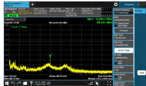
NTNV-n77(3700-3980)-PC2-30-50-L-DFT-BPSK-Inner_1RB_Left-0.15- 30-PASS
