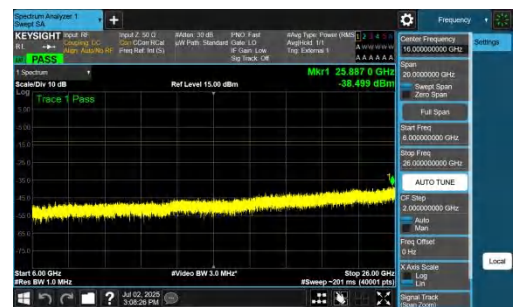
NTVN-n77(3700-3980)-PC2-30-30-H-DFT-QPSK-Inner_1RB_Left-6000-0-26000-PASS
