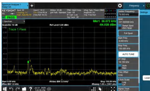
NTNV-n77(3700-3980)-PC2-30-40-L-DFT-BPSK-Inner_1RB_Left-0.00 9-0.15-PASS
