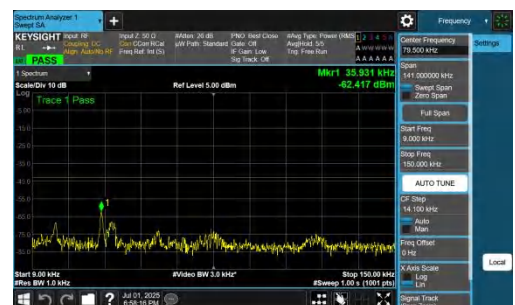
NTNV-n77(3700-3980)-PC2-30-30-H-DFT-BPSK-Inner_1RB_Right-0.0 09-0.15-PASS
