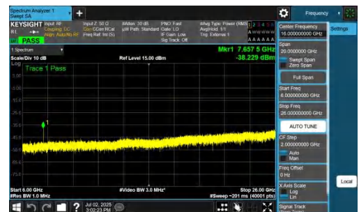
NTNV-n77(3700-3980)-PC2-30-25-M-DFT-BPSK-Inner_1RB_Left-600 0-26000-PASS
