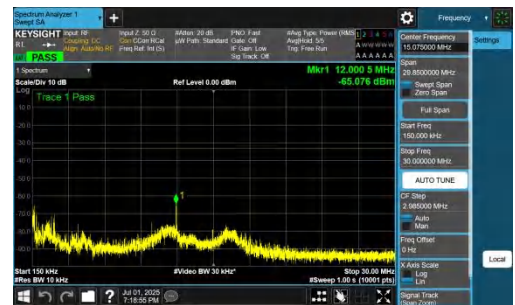
NTNV-n77(3700-3980)-PC2-30-40-H-DFT-QPSK-Inner_1RB_Left-0.15-30-PASS
