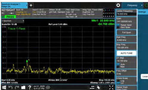
NTNV-n77(3700-3980)-PC2-30-25-H-DFT-QPSK-Inner_1RB_Left-0.009-0.15-PASS
