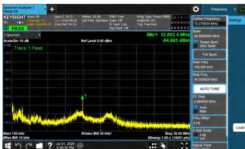
NTNV-n77(3700-3980)-PC2-30-25-H-DFT-BPSK-Inner_1RB_Right-0. 15-30-PASS
