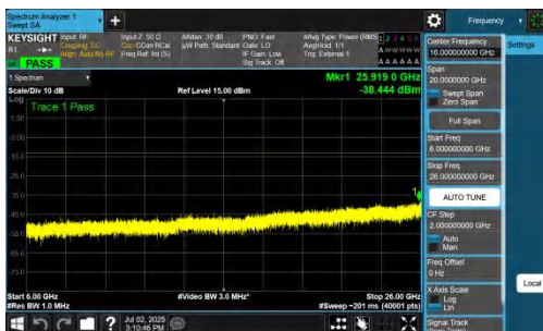
NTNV-n77(3700-3980)-PC2-30-40-M-DFT-BPSK-Inner_1RB_Right-6000-26000-PASS
