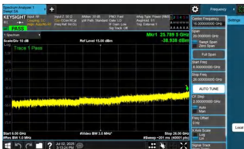
NTNV-n77(3700-3980)-PC2-30-50-L-DFT-BPSK-Inner_1RB_Right-6000-26000-PASS
