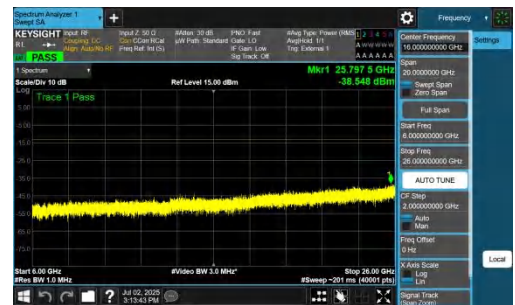
NTNV-n77(3700-3980)-PC2-30-50-L-DFT-QPSK-Inner_1RB_Left-6000-26000-PASS
