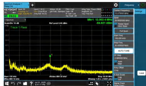
NTNV-n77(3700-3980)-PC2-30-25-H-DFT-QPSK-Inner_1RB_Left-0.15-30-PASS
