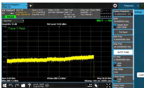
NTNV-n77(3700-3980)-PC2-30-30-H-DFT-QPSK-Inner_1RB_Right-6 000-26000-PASS
