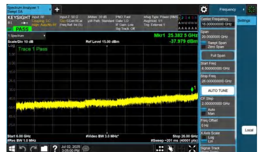
NTNV-n77(3700-3980)-PC2-30-30-L-DFT-BPSK-Inner_1RB_Left-6000 -26000-PASS
