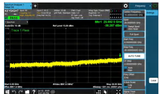
NTNV-n77(3700-3980)-PC2-30-30-H-DFT-BPSK-Inner_1RB_Left-6000 -26000-PASS
