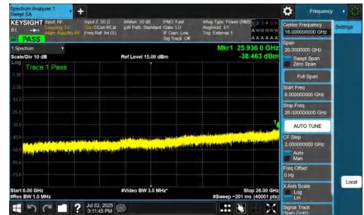
NTNV-n77(3700-3980)-PC2-30-40-H-DFT-BPSK-Inner_1RB_Left-6000 -26000-PASS
