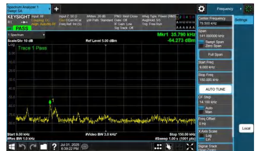
NTNV-n77(3700-3980)-PC2-30-25-H-DFT-BPSK-Inner_1RB_Right-0.0 09-0.15-PASS
