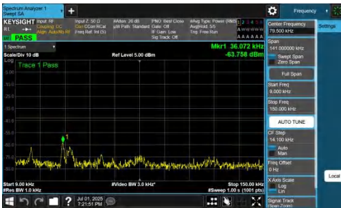
NTNV-n77(3700-3980)-PC2-30-50-L-DFT-BPSK-Inner_1RB_Left-0.00 9-0.15-PASS
