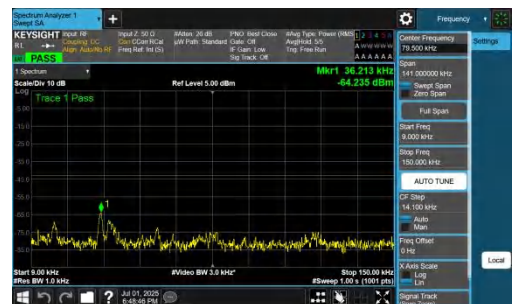
NTNV-n77(3700-3980)-PC2-30-30-L-DFT-QPSK-Inner_1RB_Right-0.09-0.15-PASS
