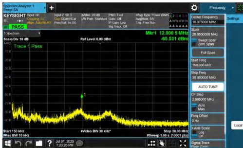
NTNV-n77(3700-3980)-PC2-30-50-L-DFT-BPSK-Inner_1RB_Right-0.15-30-PASS
