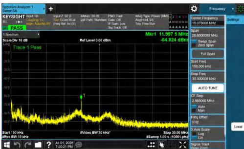
NTNV-n77(3700-3980)-PC2-30-40-H-DFT-QPSK-Inner_1RB_Right-0. 15-30-PASS
