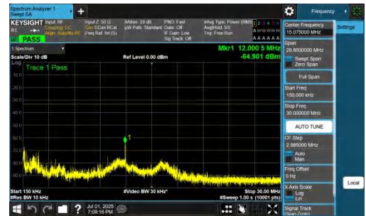
NTNV-n77(3700-3980)-PC2-30-40-M-DFT-BPSK-Inner_1RB_Left-0.15 -30-PASS
