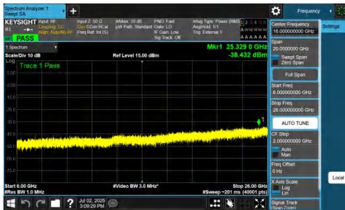
NTNV-n77(3700-3980)-PC2-30-40-L-DFT-BPSK-Inner_1RB_Right-6000-26000-PASS
