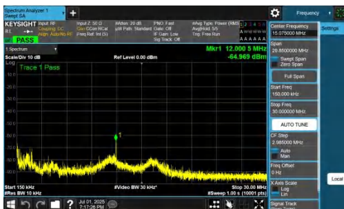
NTNV-n77(3700-3980)-PC2-30-40-H-DFT-BPSK-Inner_1RB_Right-0. 15-30-PASS
