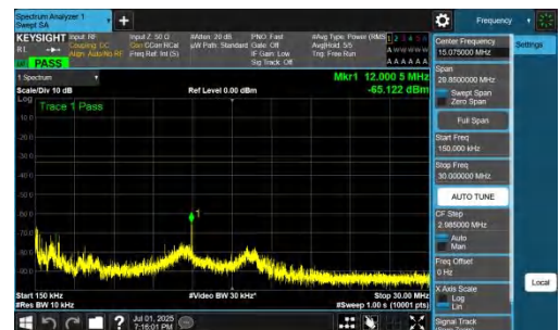
NTNV-n77(3700-3980)-PC2-30-40-H-DFT-BPSK-Inner_1RB_Left-0.15- 30-PASS
