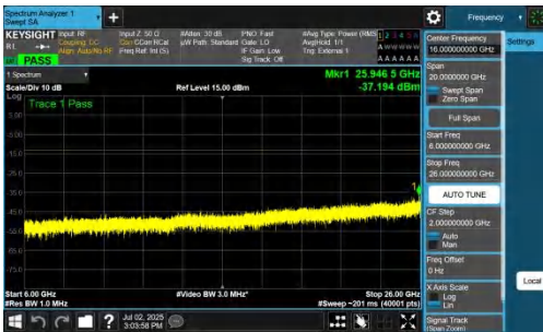
NTNV-n77(3700-3980)-PC2-30-25-H-DFT-BPSK-Inner_1RB_Right-6000-PASS
