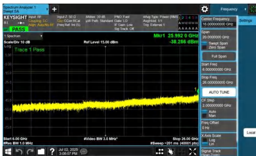
NTNV-n77(3700-3980)-PC2-30-30-L-DFT-QPSK-Inner_1RB_Right-60 00-26000-PASS
