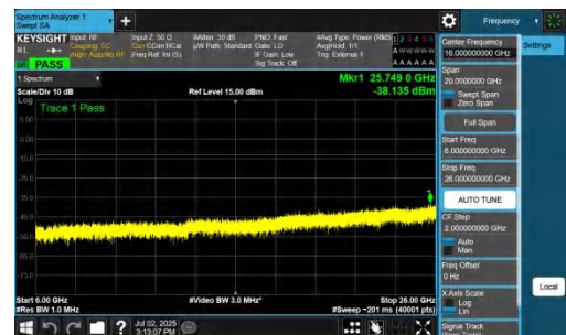
NTNV-n77(3700-3980)-PC2-30-50-L-DFT-BPSK-Inner_1RB_Left-6000 -26000-PASS
