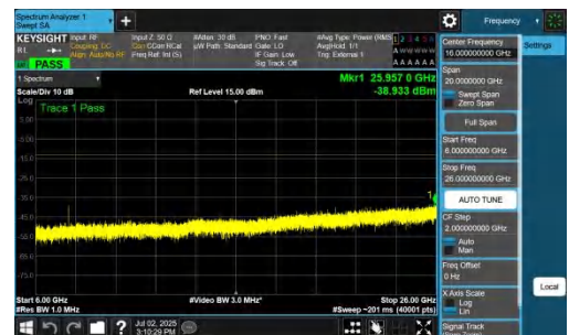
NTNV-n77(3700-3980)-PC2-30-40-M-DFT-BPSK-Inner_1RB_Left-600 0-26000-PASS
