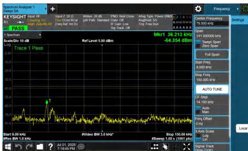
NTNV-n77(3700-3980)-PC2-30-40-H-DFT-QPSK-Inner_1RB_Left-0.009-0.15-PASS
