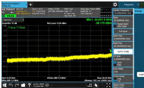
NTNV-n77(3700-3980)-PC2-30-40-H-DFT-BPSK-Inner_1RB_Right-6000-26000-PASS
