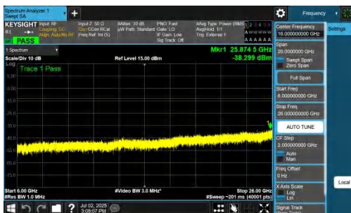
NTNV-n77(3700-3980)-PC2-30-30-H-DFT-BPSK-Inner_1RB_Right-60 00-26000-PASS
