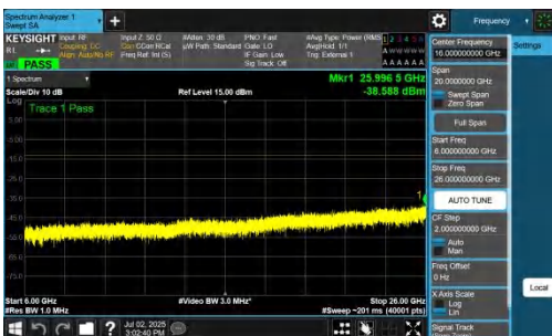
NTNV-n77(3700-3980)-PC2-30-25-M-DFT-BPSK-Inner_1RB_Right-6000-26000-PASS
