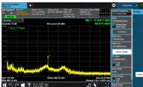
NTNV-n77(3700-3980)-PC2-30-40-L-DFT-BPSK-Inner_1RB_Right-0. 15-30-PASS
