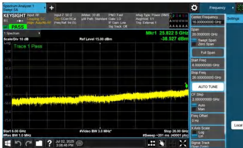
NTNV-n77(3700-3980)-PC2-30-30-M-DFT-BPSK-Inner_1RB_Right-6 000-26000-PASS
