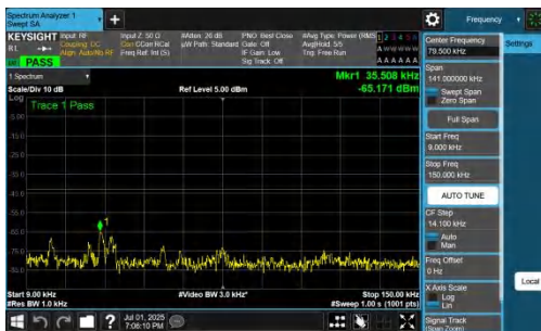
NTNV-n77(3700-3980)-PC2-30-40-L-DFT-QPSK-Inner_1RB_Left-0.009-0.15-PASS
