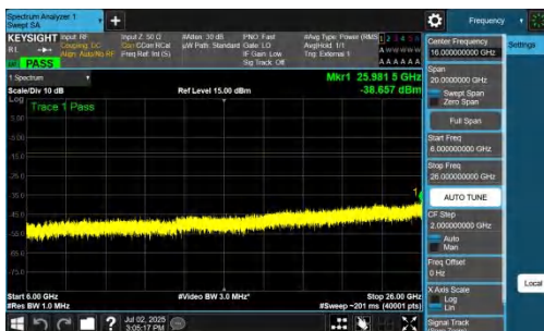
NTNV-n77(3700-3980)-PC2-30-30-L-DFT-BPSK-Inner_1RB_Right-6000-26000-PASS
