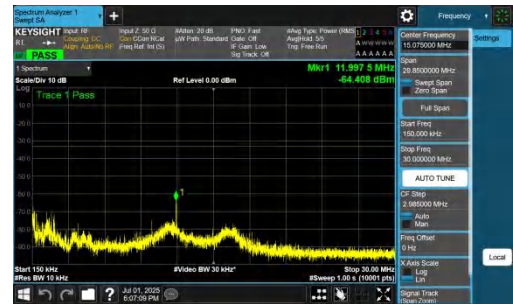
NTNV-n77(3700-3980)-PC2-30-20-L-DFT-BPSK-Inner_1RB_Left-0.15- 30-PASS
