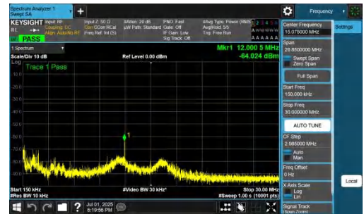
NTNV-n77(3700-3980)-PC2-30-20-H-DFT-BPSK-Inner_1RB_Left-0.15- 30-PASS
