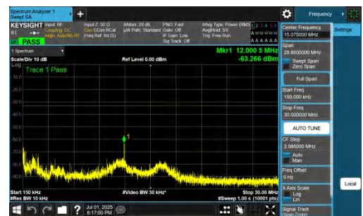
NTNV-n77(3700-3980)-PC2-30-20-M-DFT-QPSK-Inner_1RB_Left-0.15-30-PASS
