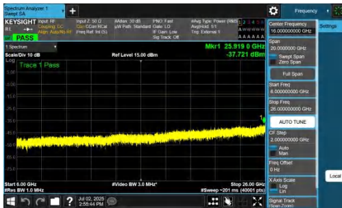
NTNV-n77(3700-3980)-PC2-30-15-H-DFT-BPSK-Inner_1RB_Right-6000-26000-PASS
