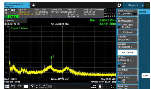
NTNV-n77(3700-3980)-PC2-30-15-H-DFT-QPSK-Inner_1RB_Left-0.15-30-PASS
