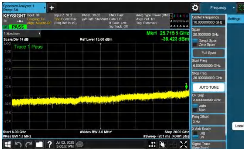
NTNV-n77(3700-3980)-PC2-30-25-L-DFT-BPSK-Inner_1RB_Right-6000-PASS
