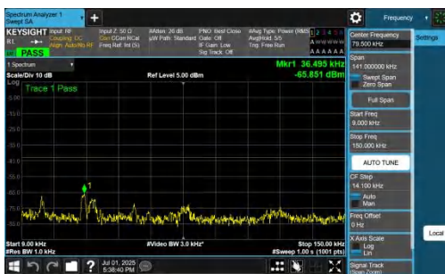
NTNV-n77(3700-3980)-PC2-30-10-M-DFT-QPSK-Inner_1RB_Left-0.009-0.15-PASS
