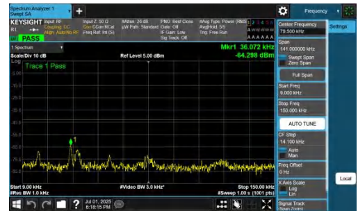
NTNV-n77(3700-3980)-PC2-30-20-M-DFT-QPSK-Inner_1RB_Right-0.0 09-0.15-PASS
