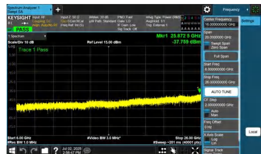
NTNV-n77(3700-3980)-PC2-30-20-L-DFT-BPSK-Inner_1RB_Left-6000 -26000-PASS
