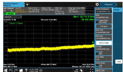
NTNV-n77(3700-3980)-PC2-30-20-H-DFT-BPSK-Inner_1RB_Left-6000 -26000-PASS
