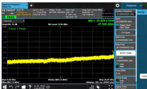
NTNV-n77(3700-3980)-PC2-30-20-H-DFT-BPSK-Inner_1RB_Right-60 00-26000-PASS
