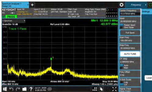
NTNV-n77(3700-3980)-PC2-30-20-L-DFT-BPSK-Inner_1RB_Right-0.15-30-PASS
