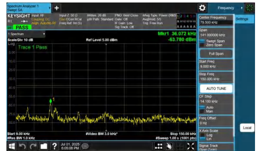
NTNV-n77(3700-3980)-PC2-30-15-H-DFT-QPSK-Inner_1RB_Right-0.09-0.15-PASS
