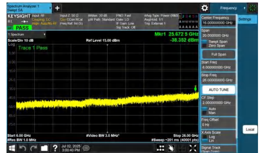
NTNV-n77(3700-3980)-PC2-30-25-L-DFT-BPSK-Inner_1RB_Left-6000 -26000-PASS
