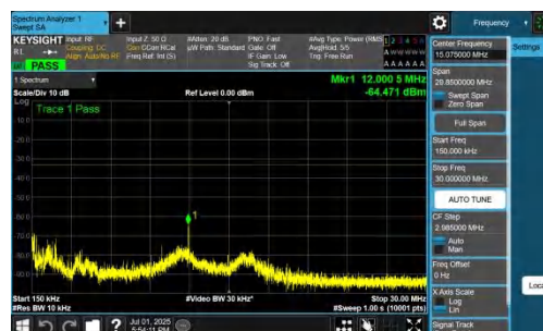
NTNV-n77(3700-3980)-PC2-30-15-M-DFT-BPSK-Inner_1RB_Left-0.15 -30-PASS
