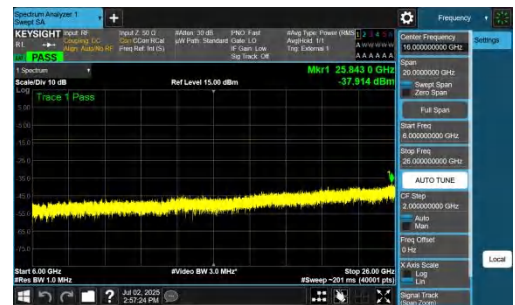
NTNV-n77(3700-3980)-PC2-30-20-L-DFT-QPSK-Inner_1RB_Left-6000-26000-PASS
