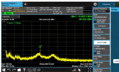
NTNV-n77(3700-3980)-PC2-30-15-L-DFT-QPSK-Inner_1RB_Right-0. 15-30-PASS
