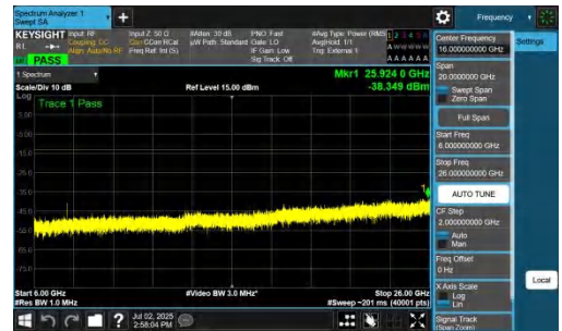
NTNV-n77(3700-3980)-PC2-30-20-M-DFT-BPSK-Inner_1RB_Left-600 0-26000-PASS
