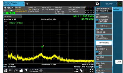
NTNV-n77(3700-3980)-PC2-30-10-H-DFT-BPSK-Inner_1RB_Left-0.15- 30-PASS
