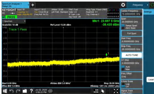
NTNV-n77(3700-3980)-PC2-30-20-M-DFT-BPSK-Inner_1RB_Right-6000-26000-PASS
