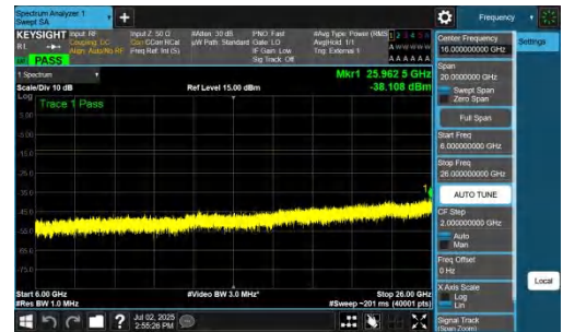
NTNV-n77(3700-3980)-PC2-30-15-H-DFT-BPSK-Inner_1RB_Left-6000 -26000-PASS
