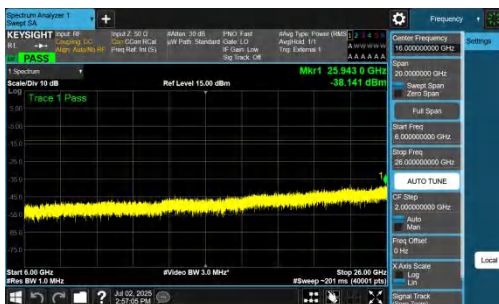
NTNV-n77(3700-3980)-PC2-30-20-L-DFT-BPSK-Inner_1RB_Right-6000-26000-PASS
