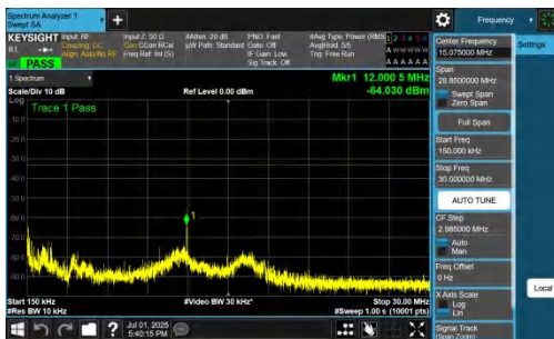
NTNV-n77(3700-3980)-PC2-30-10-M-DFT-QPSK-Inner_1RB_Right-0.15-30-PASS
