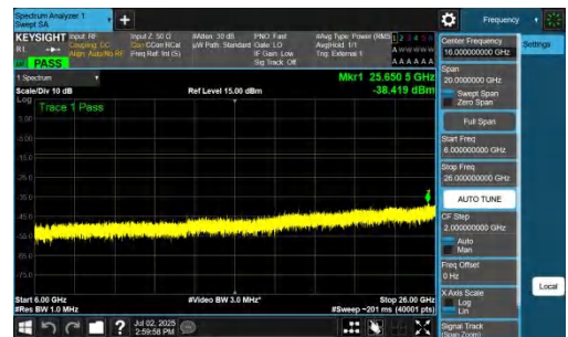
NTNV-n77(3700-3980)-PC2-30-20-H-DFT-QPSK-Inner_1RB_Left-6000-0-26000-PASS
