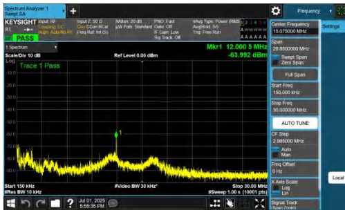
NTNV-n77(3700-3980)-PC2-30-15-M-DFT-BPSK-Inner_1RB_Right-0.15-30-PASS
