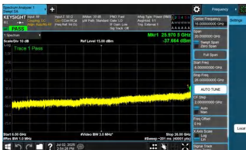
NTNV-n77(3700-3980)-PC2-30-15-M-DFT-BPSK-Inner_1RB_Right-6000-26000-PASS
