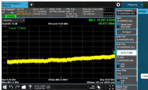
NTNV-n77(3700-3980)-PC2-30-10-M-DFT-BPSK-Inner_1RB_Right-6000-26000-PASS
