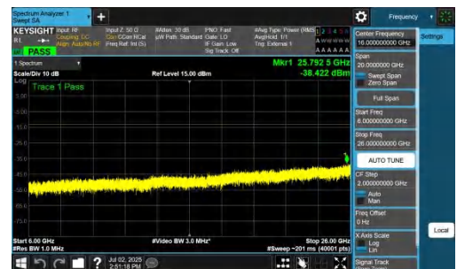
NTNV-n77(3700-3980)-PC2-30-10-H-DFT-BPSK-Inner_1RB_Left-6000 -26000-PASS
