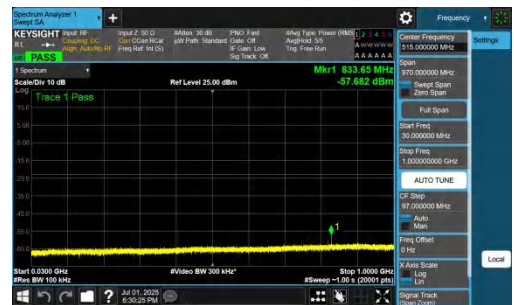
NTNV-n77(3700-3980)-PC2-30-25-L-DFT-QPSK-Inner_1RB_Right-30- 1000-PASS
