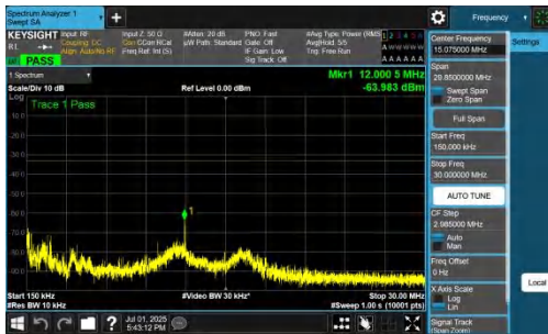
NTNV-n77(3700-3980)-PC2-30-10-H-DFT-BPSK-Inner_1RB_Right-0.15-30-PASS
