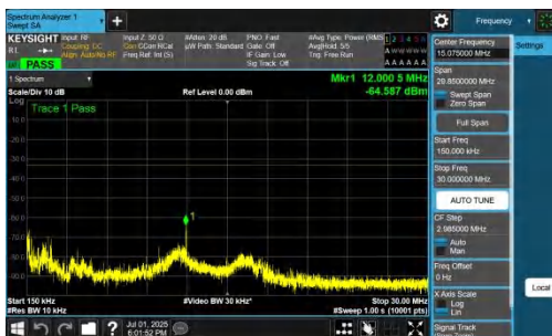
NTNV-n77(3700-3980)-PC2-30-15-H-DFT-BPSK-Inner_1RB_Right-0. 15-30-PASS
