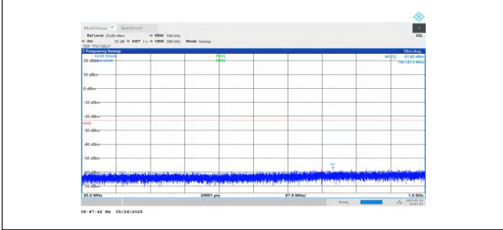
NTNV-n2-PC3-15-20-M-DFT-BPSK-Inner_1RB_Left-30-1000-PASS SS
