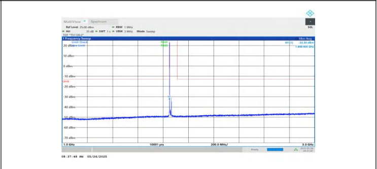
NTNV-n2-PC3-15-15-L-DFT-BPSK-Inner_1RB_Left-1000-3000-PASS
