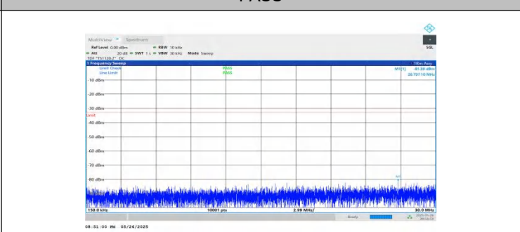
NTVN-n2-PC3-15-20-H-DFT-BPSK-Inner_1RB_Right-0.15-30-PASS
