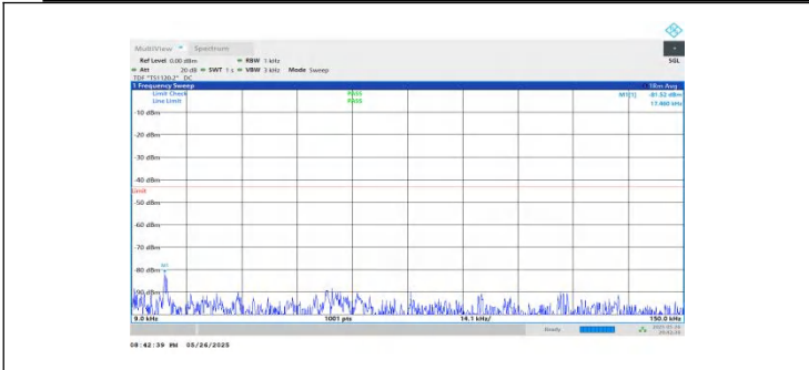
NTNV-n2-PC3-15-15-H-DFT-BPSK-Inner_1RB_Left-0.009-0.15-P ASS
