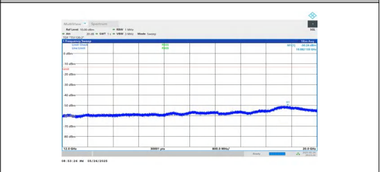
NTNV-n2-PC3-15-25-L-DFT-BPSK-Inner_1RB_Left-12000-20000- PASS
