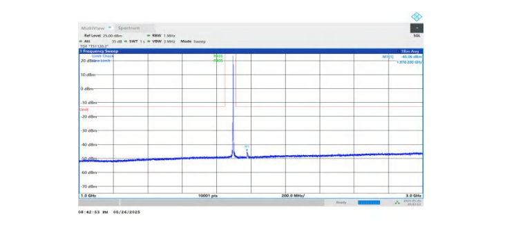
NTNV-n2-PC3-15-15-H-DFT-BPSK-Inner_1RB_Left-1000-3000-P ASS
