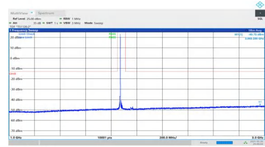
NTNV-n2-PC3-15-20-M-DFT-QPSK-Inner_1RB_Left-1000-3000-P ASS
