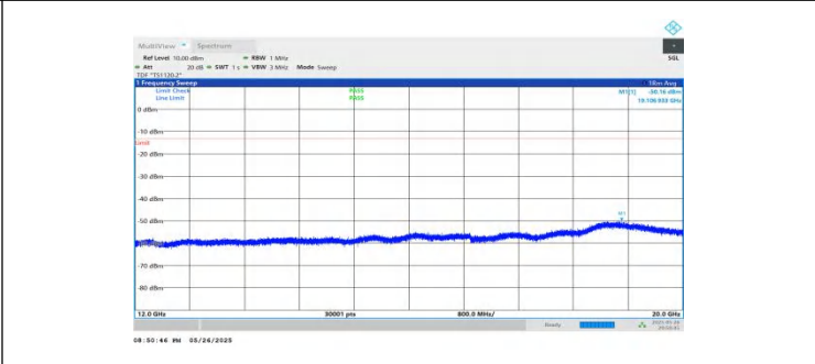
NTVN-n2-PC3-15-20-H-DFT-BPSK-Inner_1RB_Left-12000-20000-PASS
