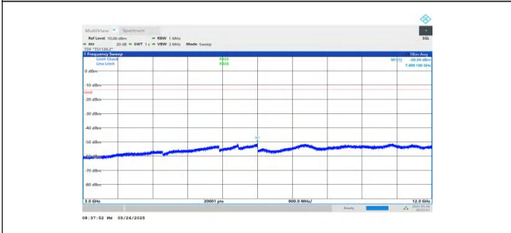
NTNV-n2-PC3-15-15-L-DFT-BPSK-Inner_1RB_Left-3000-12000-PASS
