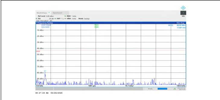
NTVN-n2-PC3-15-5-H-DFT-BPSK-Inner_1RB_Right-0.009-0.15-P ASS
