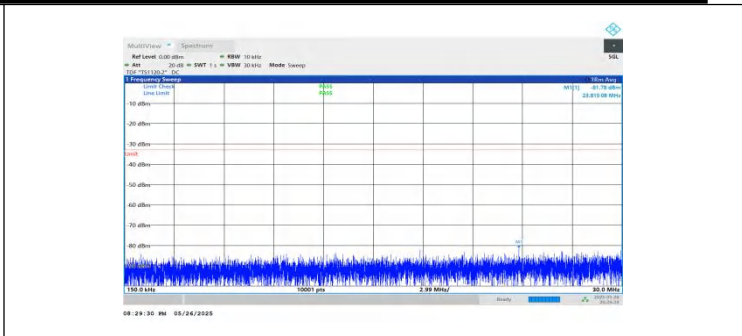
NTNV-n2-PC3-15-10-L-DFT-BPSK-Inner_1RB_Left-0.15-30-PASS
