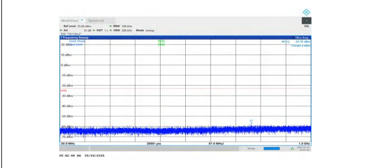
NTNV-n2-PC3-15-15-H-DFT-BPSK-Inner_1RB_Left-30-1000-PASS
