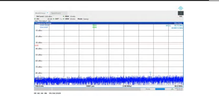
NTNV-n2-PC3-15-15-H-DFT-BPSK-Inner_1RB_Left-0.15-30-PASS
