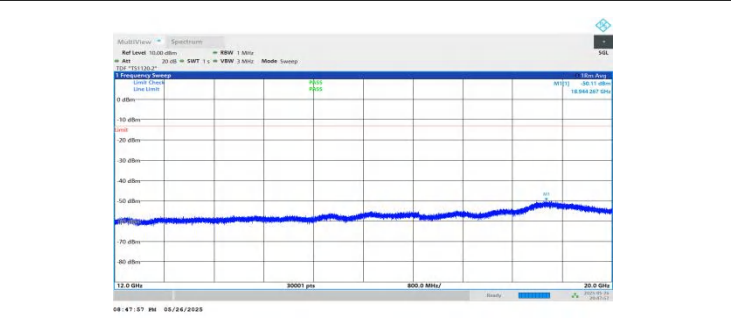
NTNV-n2-PC3-15-20-M-DFT-BPSK-Inner_1RB_Left-12000-20000-PASS PASS
