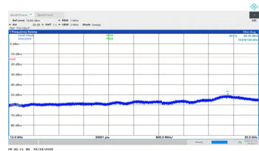
NTNV-n2-PC3-15-15-M-DFT-QPSK-Inner_1RB_Right-12000-2000 0-PASS
