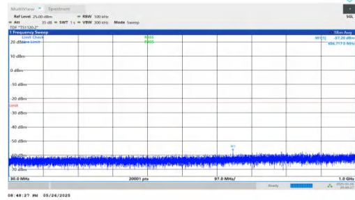
NTNV-n2-PC3-15-20-M-DFT-BPSK-Inner_1RB_Right-30-1000-P ASS
