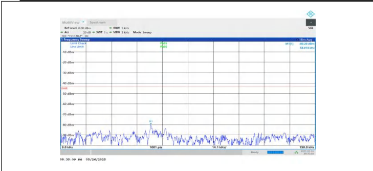
NTNV-n2-PC3-15-10-H-DFT-BPSK-Inner_1RB_Left-0.009-0.15-P ASS
