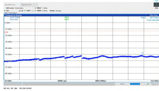
NTNV-n2-PC3-15-15-M-DFT-QPSK-Inner_1RB_Left-3000-12000 -PASS
