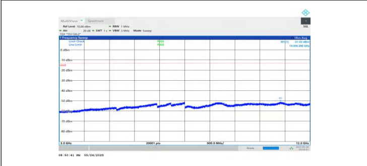
NTVN-n2-PC3-15-20-H-DFT-BPSK-Inner_1RB_Left-3000-12000-PASS
