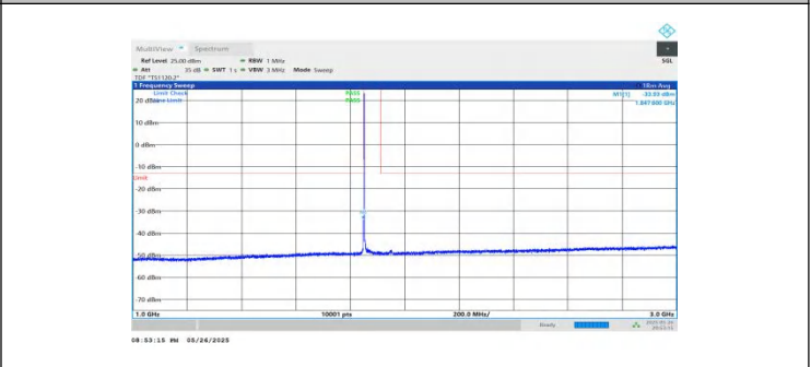
NTNV-n2-PC3-15-25-L-DFT-BPSK-Inner_1RB_Left-1000-3000-PASS S
