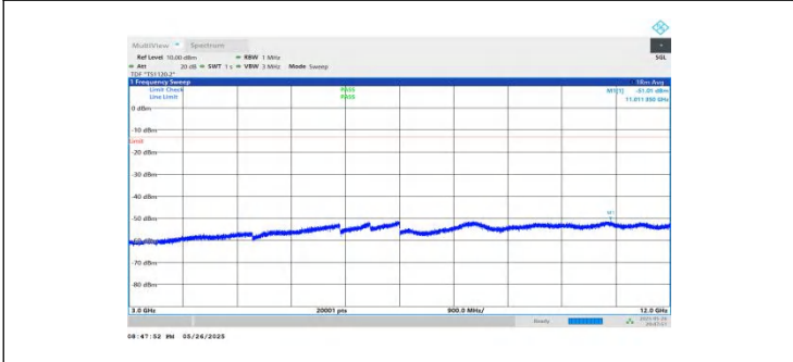
NTNV-n2-PC3-15-20-M-DFT-BPSK-Inner_1RB_Left-3000-12000-PASS PASS
