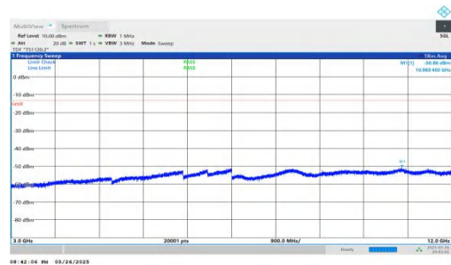
NTNV-n2-PC3-15-15-M-DFT-QPSK-Inner_1RB_Right-3000-1200 0-PASS
