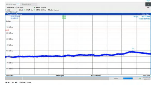
NTNV-n2-PC3-15-15-M-DFT-QPSK-Inner_1RB_Left-12000-20000 -PASS
