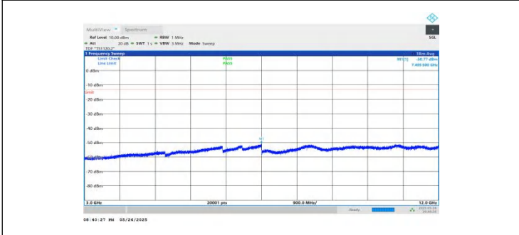
NTNV-n2-PC3-15-15-M-DFT-BPSK-Inner_1RB_Left-3000-12000-PASS PASS
