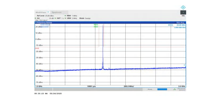
NTNV-n2-PC3-15-10-H-DFT-BPSK-Inner_1RB_Left-1000-3000-P ASS
