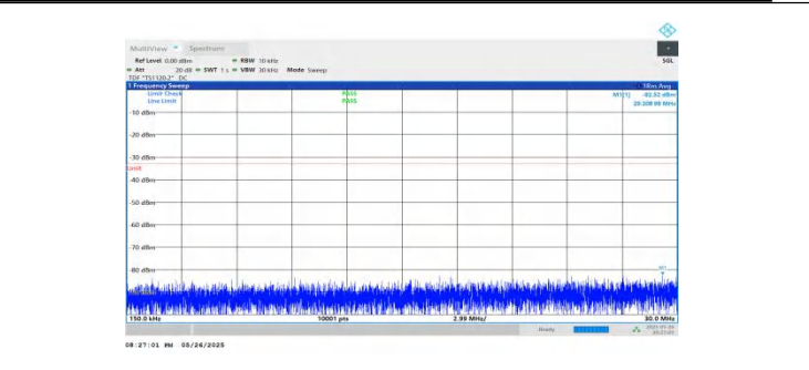
NTVN-n2-PC3-15-5-H-DFT-BPSK-Inner_1RB_Left-0.15-30-PASS
