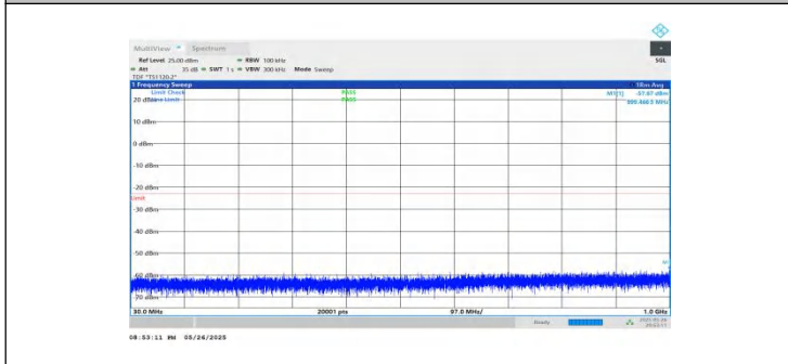
NTNV-n2-PC3-15-25-L-DFT-BPSK-Inner_1RB_Left-30-1000-PAS S
