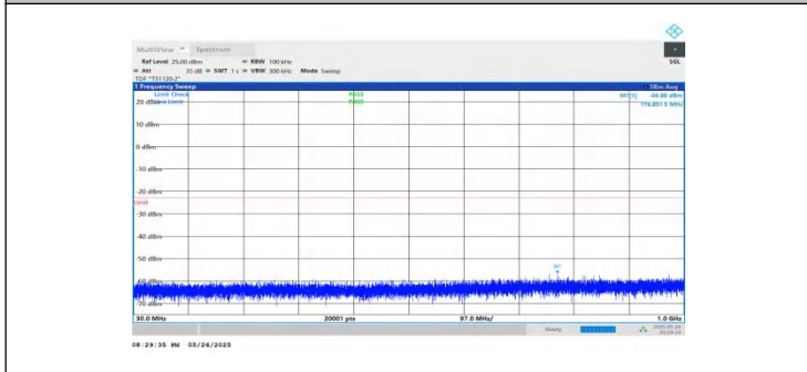
NTNV-n2-PC3-15-10-L-DFT-BPSK-Inner_1RB_Left-30-1000-PAS S
