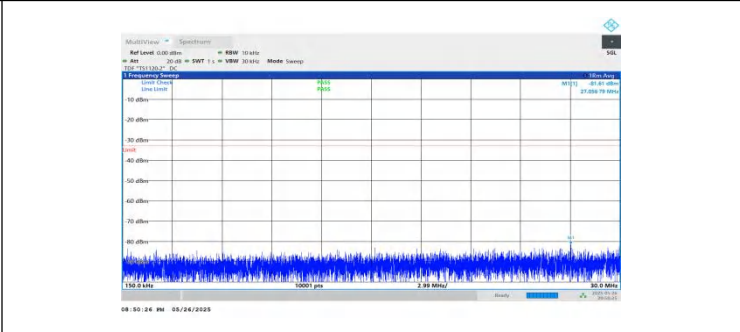
NTVN-n2-PC3-15-20-H-DFT-BPSK-Inner_1RB_Left-0.15-30-PASS
