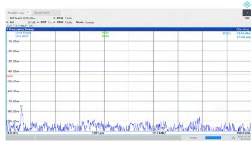
NTNV-n2-PC3-15-20-M-DFT-QPSK-Inner_1RB_Left-0.009-0.15- PASS
