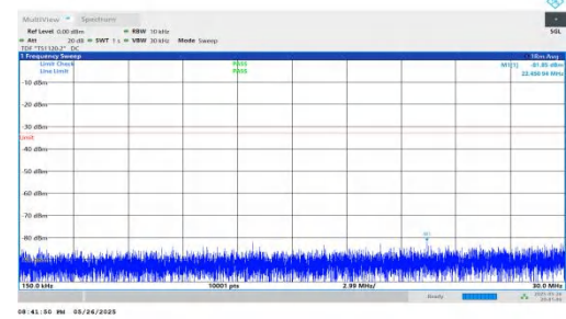
NTNV-n2-PC3-15-15-M-DFT-QPSK-Inner_1RB_Right-0.15-30-PA SS
