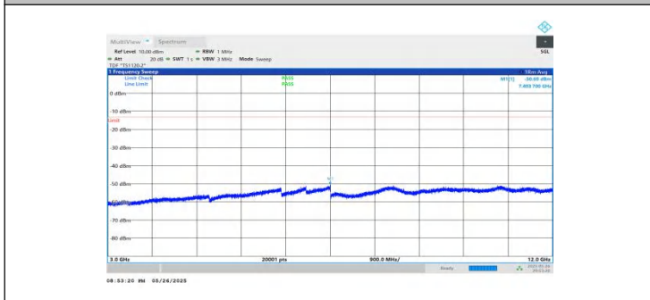
NTNV-n2-PC3-15-25-L-DFT-BPSK-Inner_1RB_Left-3000-12000- PASS
