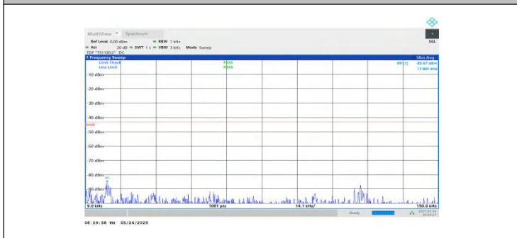
NTNV-n2-PC3-15-10-L-DFT-BPSK-Inner_1RB_Right-0.009-0.15-PASS
