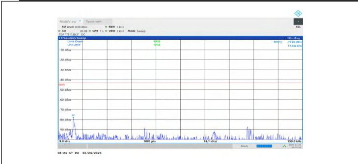
NTVN-n2-PC3-15-5-H-DFT-BPSK-Inner_1RB_Left-0.009-0.15-PA SS
