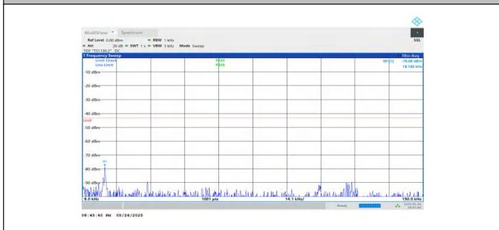
NTNV-n2-PC3-15-20-L-DFT-BPSK-Inner_1RB_Right-0.009-0.15-PASS
