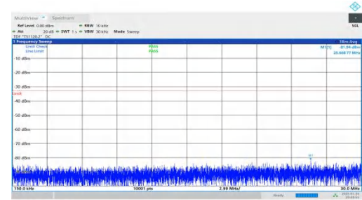
NTNV-n2-PC3-15-20-M-DFT-QPSK-Inner_1RB_Left-0.15-30-PAS S
