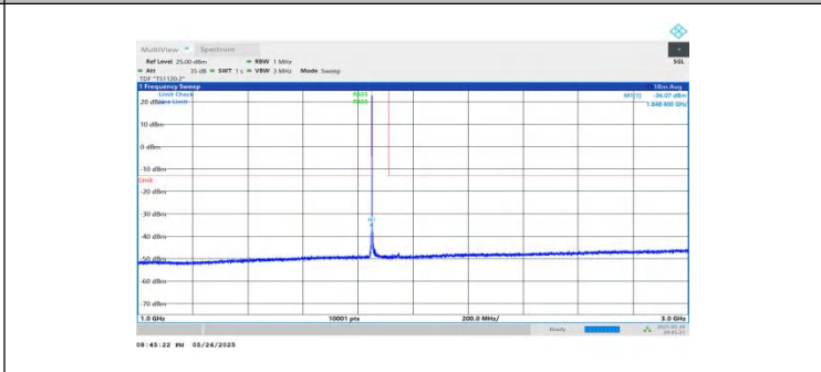
NTNV-n2-PC3-15-20-L-DFT-BPSK-Inner_1RB_Left-1000-3000-PASS S
