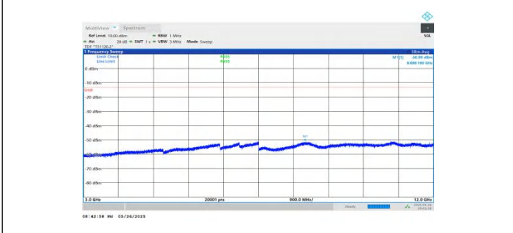
NTNV-n2-PC3-15-15-H-DFT-BPSK-Inner_1RB_Left-3000-12000-PASS
