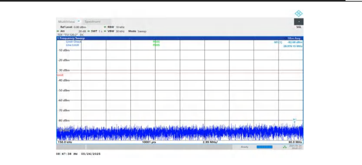
NTNV-n2-PC3-15-20-M-DFT-BPSK-Inner_1RB_Left-0.15-30-PAS S
