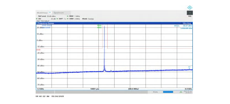
NTNV-n2-PC3-15-15-M-DFT-BPSK-Inner_1RB_Left-1000-3000-P ASS
