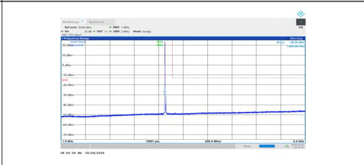
NTNV-n2-PC3-15-10-L-DFT-BPSK-Inner_1RB_Left-1000-3000-PASS
