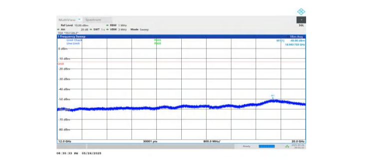
NTNV-n2-PC3-15-10-H-DFT-BPSK-Inner_1RB_Left-12000-20000-PASS
