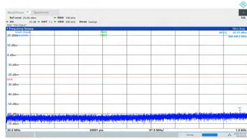
NTNV-n2-PC3-15-20-M-DFT-QPSK-Inner_1RB_Left-30-1000-PA SS
