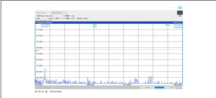
NTNV-n2-PC3-15-10-H-DFT-BPSK-Inner_1RB_Right-0.009-0.15-PASS
