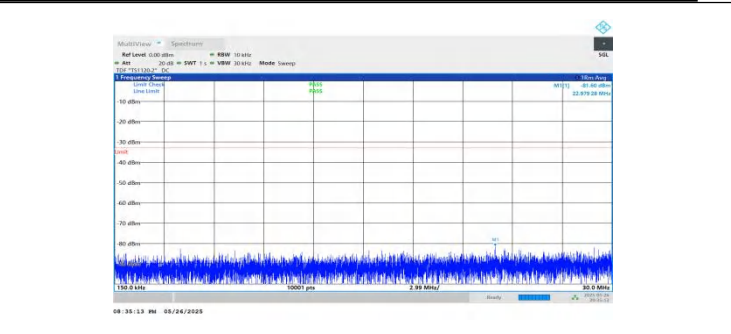
NTNV-n2-PC3-15-10-H-DFT-BPSK-Inner_1RB_Left-0.15-30-PASS
