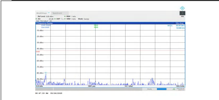
NTNV-n2-PC3-15-20-M-DFT-BPSK-Inner_1RB_Left-0.009-0.15-P ASS
