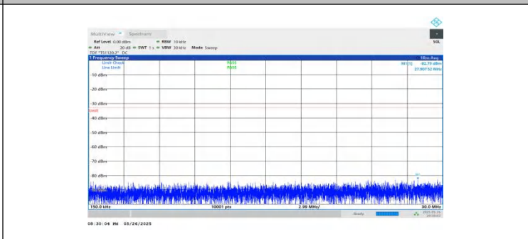
NTNV-n2-PC3-15-10-L-DFT-BPSK-Inner_1RB_Right-0.15-30-PASS
