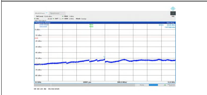
NTNV-n2-PC3-15-20-L-DFT-BPSK-Inner_1RB_Left-3000-12000-PASS
