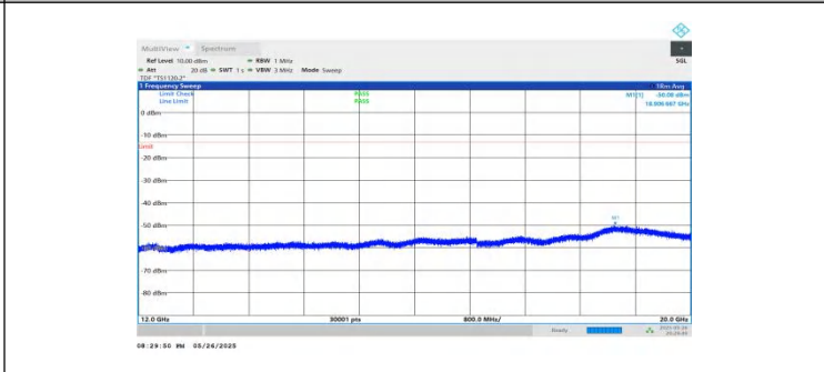
NTNV-n2-PC3-15-10-L-DFT-BPSK-Inner_1RB_Left-12000-20000-PASS
