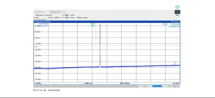
NTVN-n2-PC3-15-5-H-DFT-BPSK-Inner_1RB_Left-1000-3000-PA SS
