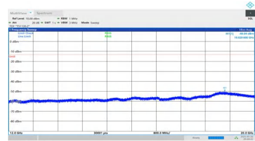
NTNV-n2-PC3-15-20-M-DFT-BPSK-Inner_1RB_Right-12000-2000 0-PASS
