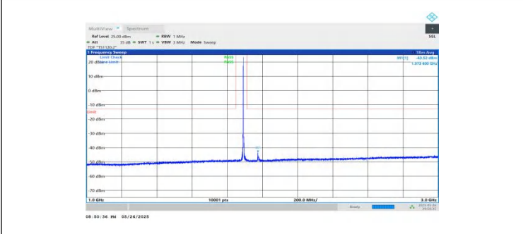
NTVN-n2-PC3-15-20-H-DFT-BPSK-Inner_1RB_Left-1000-3000-PASS
