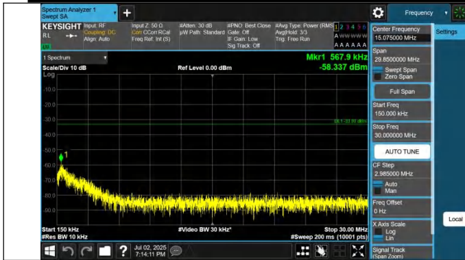
42-42-20MHz-20MHz-QPSK-QPSK-42491-42689-1RB#99-0RB# 0-0.15~30MHz-PASS
