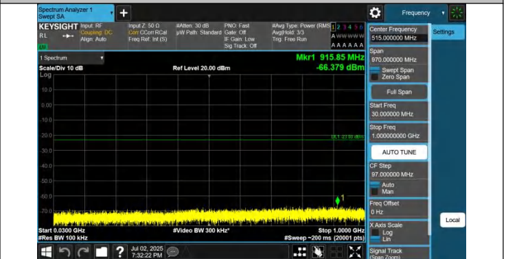
42-42-20MHz-10MHz-QPSK-QPSK-42541-42685-1RB#99-0RB# 0-30~1000MHz-PASS
