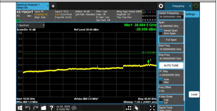
42-42-20MHz-10MHz-QPSK-QPSK-42541-42685-1RB#99-0RB# 0-18000~40000MHz-PASS
