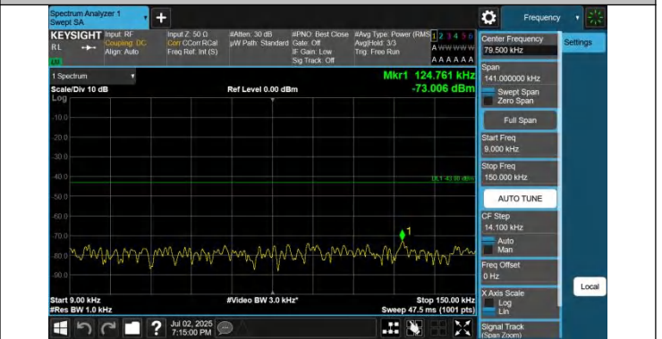
42-42-20MHz-20MHz-QPSK-QPSK-42792-42990-1RB#0-1RB#99-9-0.009~0.15MHz-PASS
