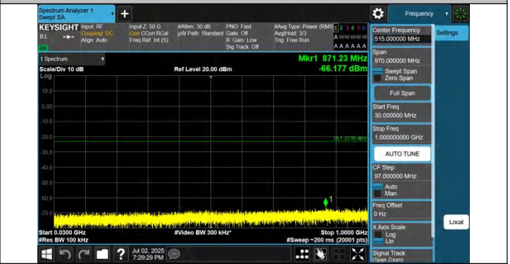
42-42-20MHz-20MHz-QPSK-QPSK-42190-42388-1RB#0-1RB#99-30~1000MHz-PASS
