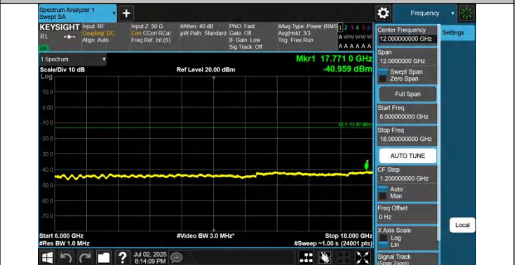
42-42-20MHz-20MHz-QPSK-QPSK-42792-42990-1RB#0-0RB#0-6000~18000MHz-PASS
