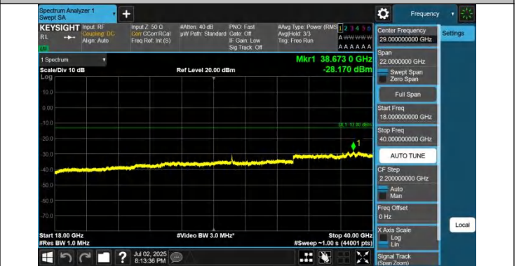
42-42-20MHz-20MHz-QPSK-QPSK-42491-42689-1RB#99-0RB# 0-18000~40000MHz-PASS
