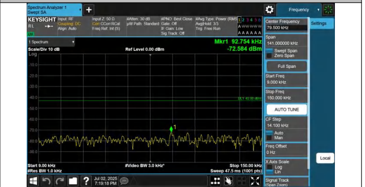
42-42-20MHz-15MHz-QPSK-QPSK-42190-42361-1RB#0-0RB#0- 0.009~0.15MHz-PASS
