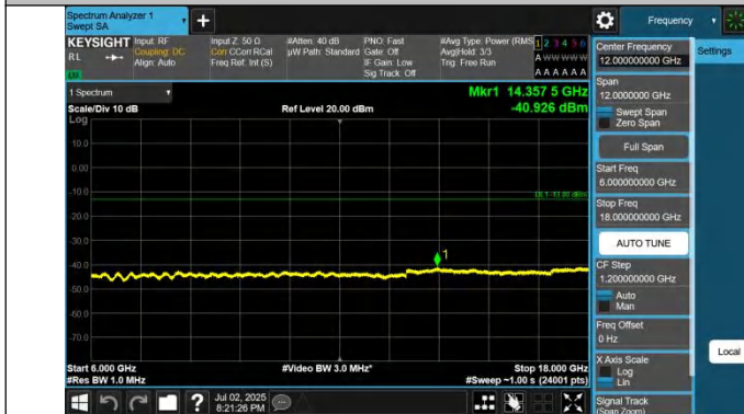
42-42-20MHz-15MHz-QPSK-QPSK-42190-42361-1RB#0-0RB#0-6000~18000MHz-PASS
