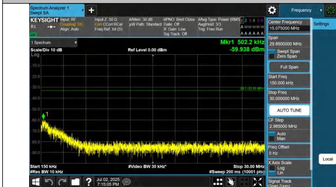
42-42-20MHz-20MHz-QPSK-QPSK-42792-42990-1RB#0-1RB#99-9-0.15~30MHz-PASS
