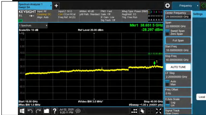
42-42-20MHz-10MHz-QPSK-QPSK-42541-42685-1RB#0-1RB#4 9-18000~40000MHz-PASS
