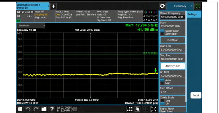
42-42-20MHz-20MHz-QPSK-QPSK-42190-42388-1RB#0-0RB#0-6000~18000MHz-PASS
