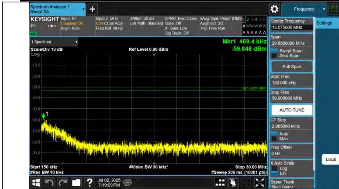
42-42-20MHz-10MHz-QPSK-QPSK-42891-43035-1RB#0-1RB#4 9-0.15~30MHz-PASS
