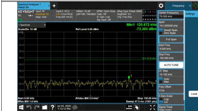
42-42-20MHz-20MHz-QPSK-QPSK-42190-42388-1RB#0-0RB#0-0.009~0.15MHz-PASS
