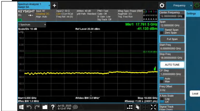
42-42-20MHz-20MHz-QPSK-QPSK-42190-42388-1RB#0-1RB#9 9-6000~18000MHz-PASS
