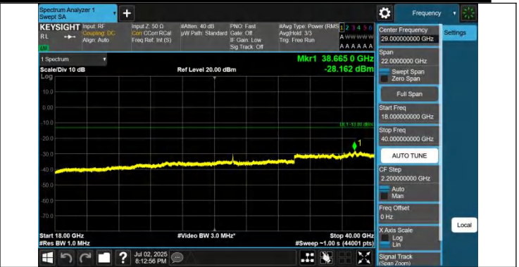
42-42-20MHz-20MHz-QPSK-QPSK-42190-42388-1RB#0-1RB#9 9-18000~40000MHz-PASS
