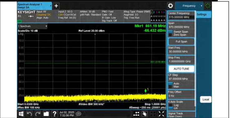
42-42-20MHz-10MHz-QPSK-QPSK-42891-43035-1RB#0-1RB#4 9-30~1000MHz-PASS
