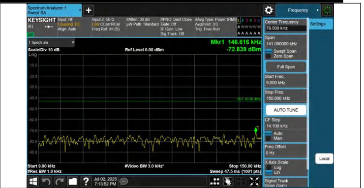
42-42-20MHz-20MHz-QPSK-QPSK-42491-42689-1RB#0-0RB#0-0.009~0.15MHz-PASS
