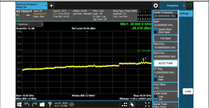
42-42-20MHz-10MHz-QPSK-QPSK-42891-43035-1RB#0-1RB#4 9-18000~40000MHz-PASS
