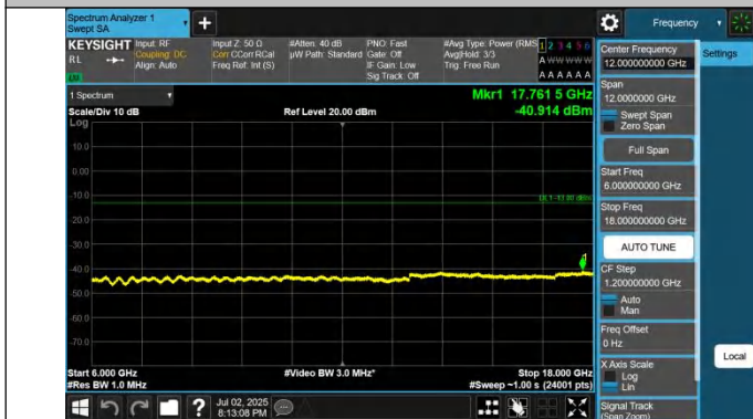
42-42-20MHz-20MHz-QPSK-QPSK-42491-42689-1RB#0-0RB#0-6000~18000MHz-PASS
