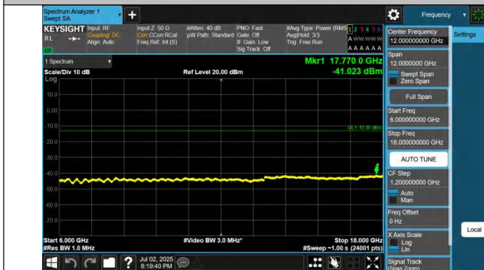
42-42-20MHz-10MHz-QPSK-QPSK-42541-42685-1RB#99-0RB# 0-6000~18000MHz-PASS
