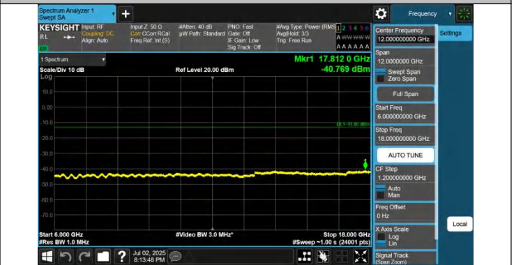
42-42-20MHz-20MHz-QPSK-QPSK-42491-42689-1RB#0-1RB#9 9-6000~18000MHz-PASS
