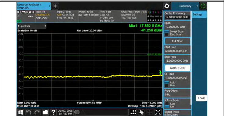
42-42-20MHz-5MHz-QPSK-QPSK-42940-43057-1RB#0-1RB#24- 6000~18000MHz-PASS
