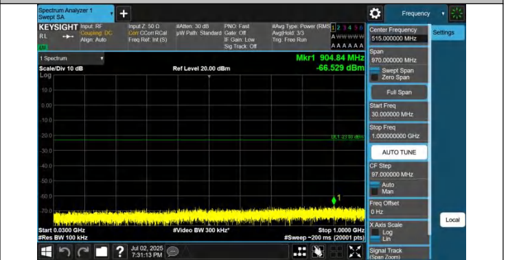
42-42-20MHz-5MHz-QPSK-QPSK-42565-42682-1RB#0-1RB#24- 30~1000MHz-PASS
