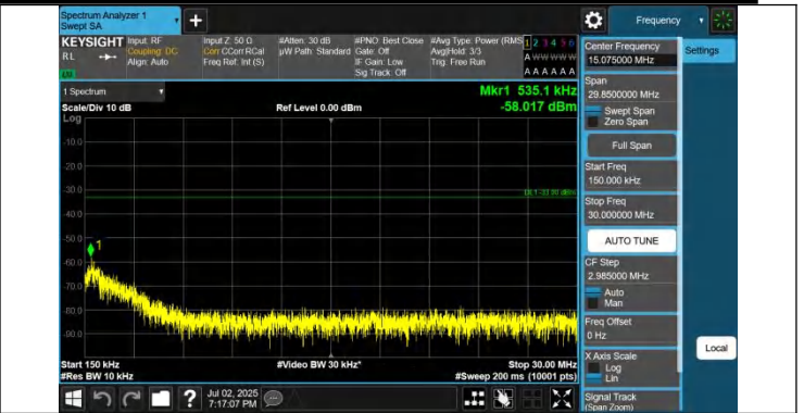
42-42-20MHz-5MHz-QPSK-QPSK-42940-43057-1RB#0-1RB#24- 0.15~30MHz-PASS
