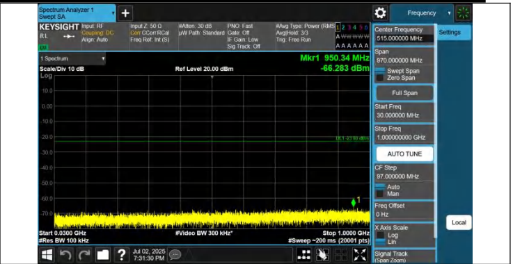
42-42-20MHz-5MHz-QPSK-QPSK-42940-43057-1RB#99-0RB#0- 30~1000MHz-PASS
