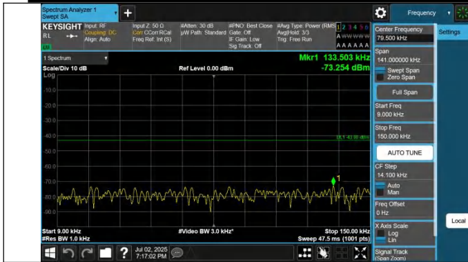
42-42-20MHz-5MHz-QPSK-QPSK-42940-43057-1RB#0-1RB#24- 0.009~0.15MHz-PASS
