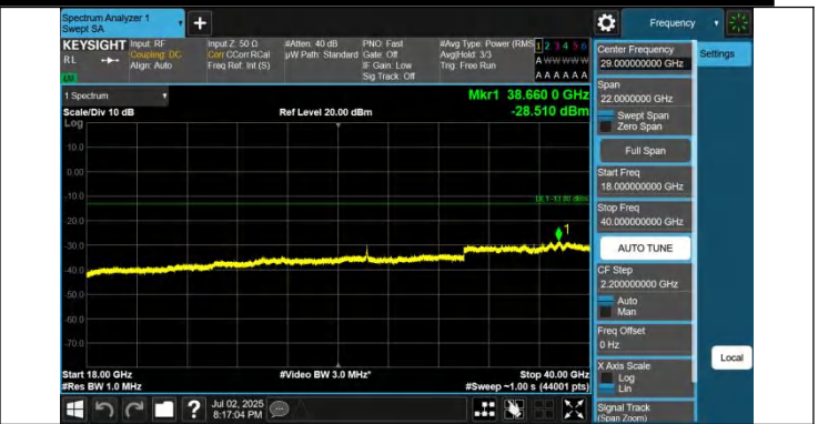
42-42-20MHz-5MHz-QPSK-QPSK-42565-42682-1RB#0-1RB#24-18000~40000MHz-PASS
