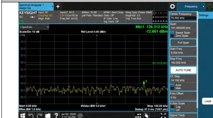
42-42-20MHz-10MHz-QPSK-QPSK-42190-42334-1RB#0-0RB#0- 0.009~0.15MHz-PASS
