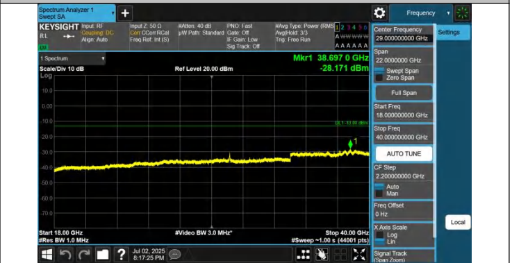
42-42-20MHz-5MHz-QPSK-QPSK-42940-43057-1RB#0-0RB#0-18000~40000MHz-PASS
