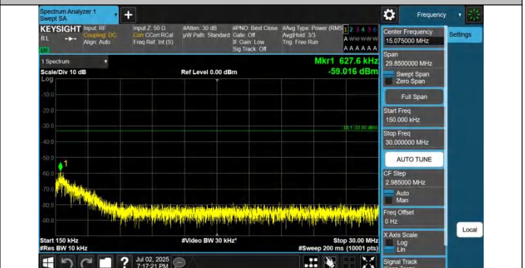
42-42-20MHz-10MHz-QPSK-QPSK-42190-42334-1RB#0-0RB#0- 0.15~30MHz-PASS
