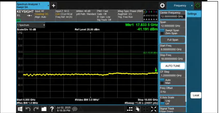
42-42-20MHz-10MHz-QPSK-QPSK-42190-42334-1RB#99-0RB# 0-6000~18000MHz-PASS
