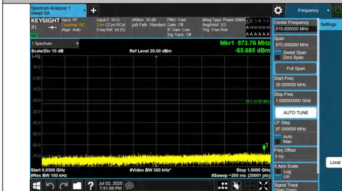
42-42-20MHz-10MHz-QPSK-QPSK-42190-42334-1RB#99-0RB# 0-30~1000MHz-PASS
