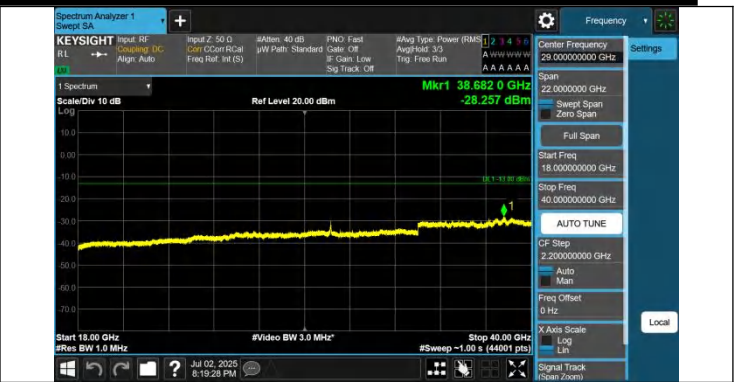
42-42-20MHz-10MHz-QPSK-QPSK-42541-42685-1RB#0-0RB#0-18000~40000MHz-PASS
