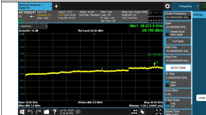
42-42-20MHz-5MHz-QPSK-QPSK-42940-43057-1RB#0-1RB#24- 18000~40000MHz-PASS
