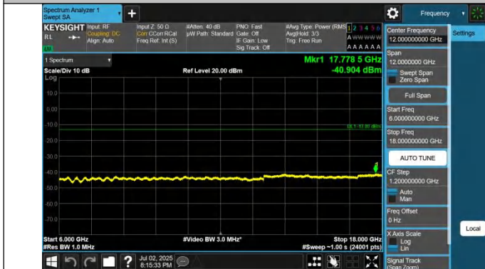
42-42-20MHz-5MHz-QPSK-QPSK-42190-42307-1RB#99-0RB#0-6000~18000MHz-PASS
