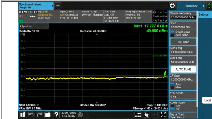
42-42-20MHz-10MHz-QPSK-QPSK-42190-42334-1RB#0-1RB#4 9-6000~18000MHz-PASS
