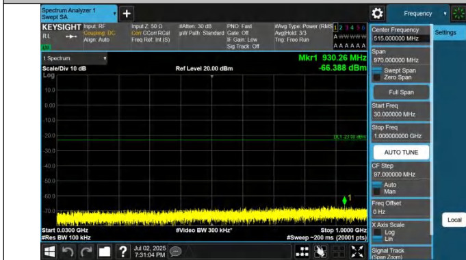
42-42-20MHz-5MHz-QPSK-QPSK-42565-42682-1RB#99-0RB#0-30~1000MHz-PASS
