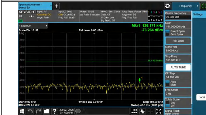
42-42-20MHz-10MHz-QPSK-QPSK-42190-42334-1RB#99-0RB# 0-0.009~0.15MHz-PASS
