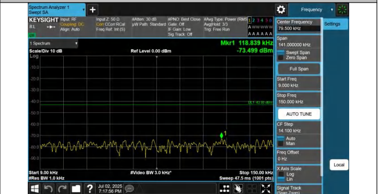
42-42-20MHz-10MHz-QPSK-QPSK-42541-42685-1RB#0-0RB#0- 0.009~0.15MHz-PASS
