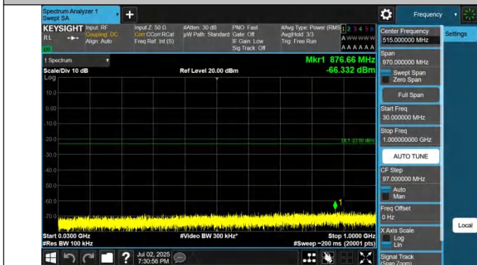
42-42-20MHz-5MHz-QPSK-QPSK-42565-42682-1RB#0-0RB#0-0-0~1000MHz-PASS
