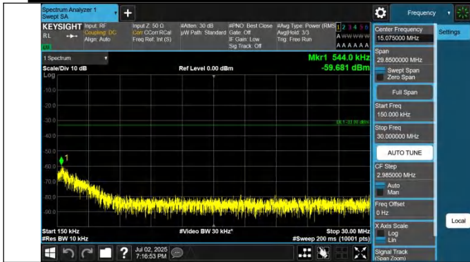
42-42-20MHz-5MHz-QPSK-QPSK-42940-43057-1RB#99-0RB#0- 0.15~30MHz-PASS
