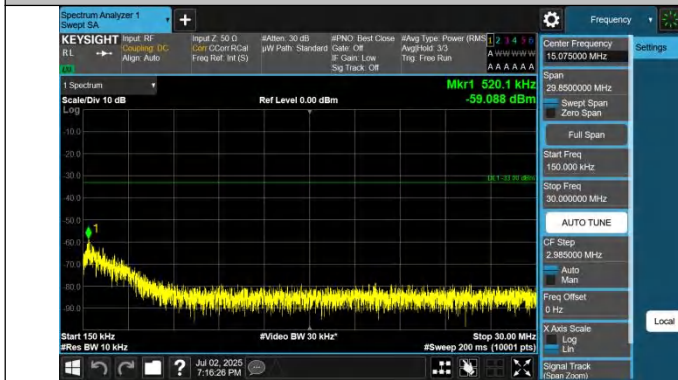
42-42-20MHz-5MHz-QPSK-QPSK-42565-42682-1RB#0-1RB#24- 0.15~30MHz-PASS
