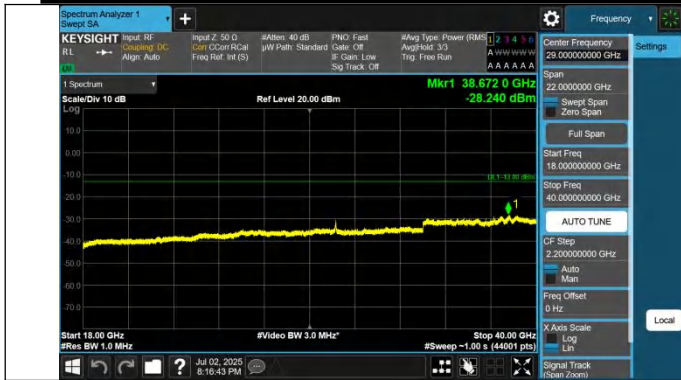
42-42-20MHz-5MHz-QPSK-QPSK-42565-42682-1RB#99-0RB#0-18000~40000MHz-PASS
