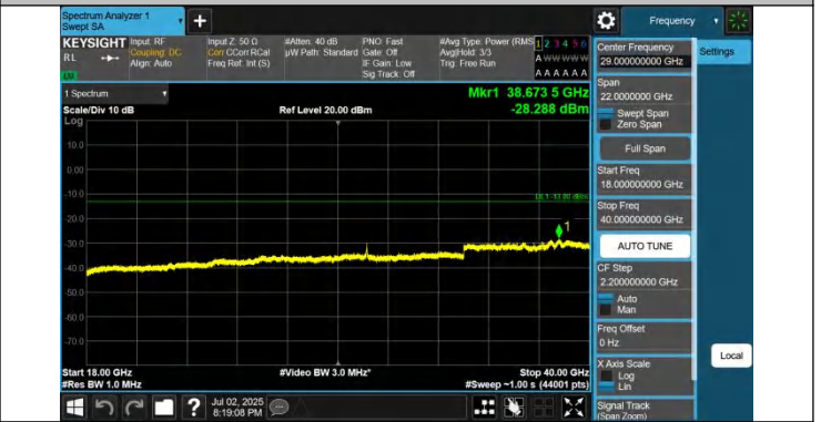
42-42-20MHz-10MHz-QPSK-QPSK-42190-42334-1RB#0-1RB#4 9-18000~40000MHz-PASS
