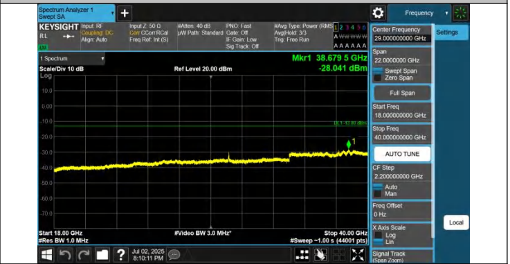
42-42-15MHz-20MHz-QPSK-QPSK-42493-42664-1RB#0-0RB#0-18000~40000MHz-PASS
