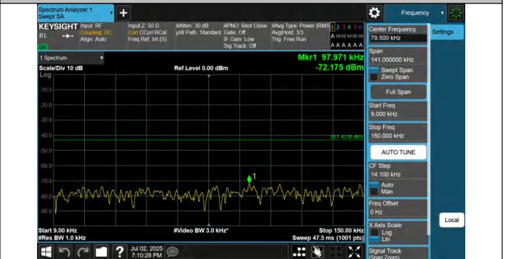
42-42-10MHz-20MHz-QPSK-QPSK-42846-42990-1RB#0-0RB#0- 0.009~0.15MHz-PASS
