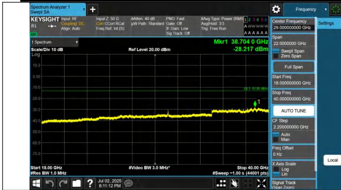
42-42-15MHz-20MHz-QPSK-QPSK-42819-42990-1RB#0-0RB#0-18000~40000MHz-PASS
