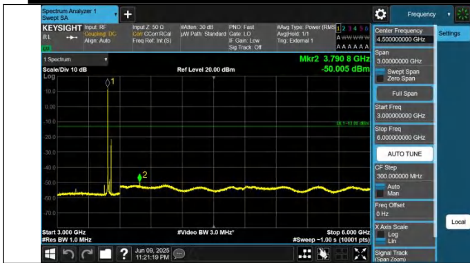
42-42-15MHz-20MHz-QPSK-QPSK-42493-42664-1RB#0-1RB#9 9-3000~6000MHz-PASS
