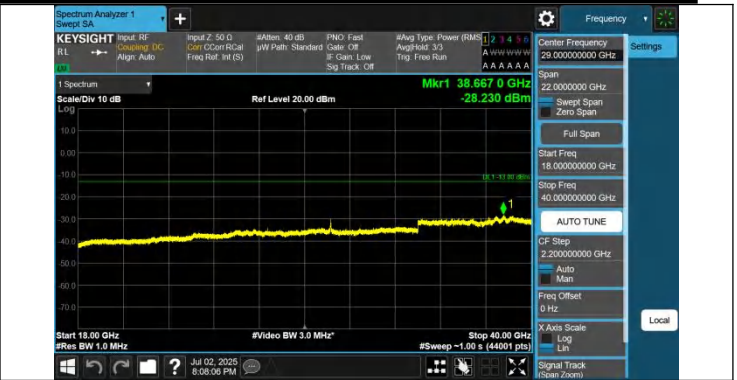
42-42-10MHz-20MHz-QPSK-QPSK-42846-42990-1RB#0-0RB#0-18000~40000MHz-PASS
