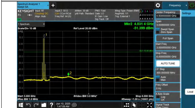
42-42-20MHz-5MHz-QPSK-QPSK-42190-42307-1RB#0-1RB#24-3000~6000MHz-PASS
