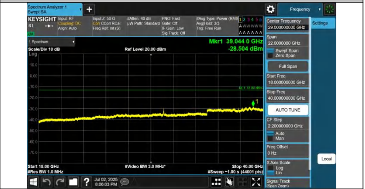
42-42-10MHz-20MHz-QPSK-QPSK-42145-42289-1RB#0-0RB#0-18000~40000MHz-PASS
