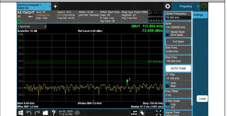
42-42-20MHz-5MHz-QPSK-QPSK-42190-42307-1RB#0-0RB#0-0 .009~0.15MHz-PASS
