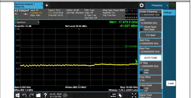
42-42-15MHz-20MHz-QPSK-QPSK-42819-42990-1RB#0-0RB#0- 6000~18000MHz-PASS
