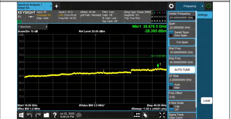
42-42-10MHz-20MHz-QPSK-QPSK-42145-42289-1RB#49-0RB# 0-18000~40000MHz-PASS
