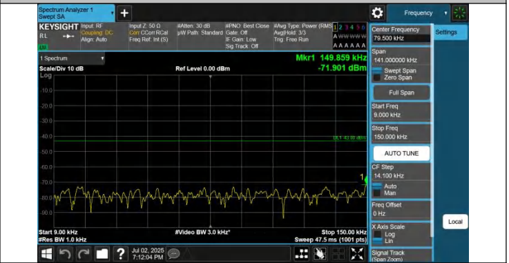
42-42-15MHz-20MHz-QPSK-QPSK-42493-42664-1RB#74-0RB# 0-0.009~0.15MHz-PASS
