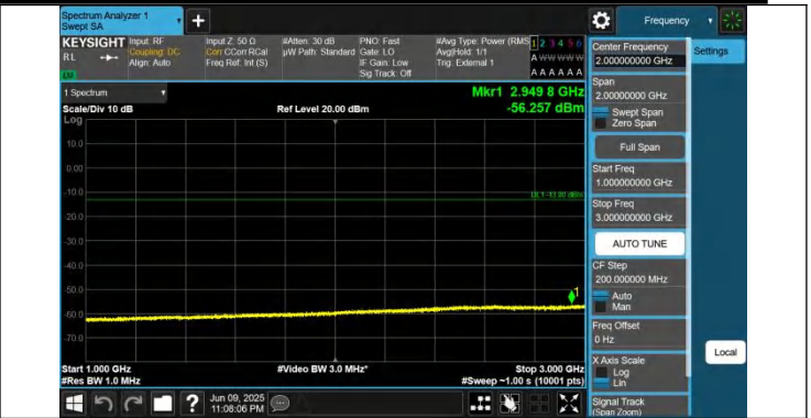
42-42-15MHz-20MHz-QPSK-QPSK-42168-42339-1RB#74-0RB# 0-1000~3000MHz-PASS
