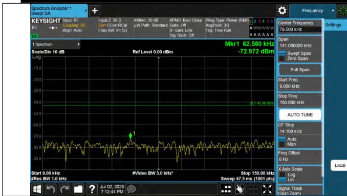
42-42-15MHz-20MHz-QPSK-QPSK-42819-42990-1RB#74-0RB# 0-0.009~0.15MHz-PASS
