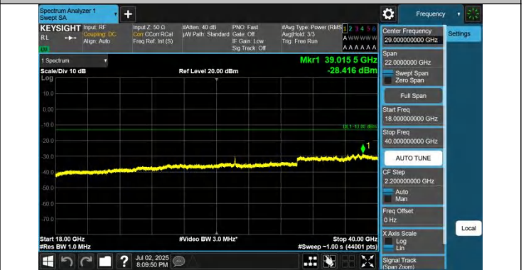
42-42-15MHz-20MHz-QPSK-QPSK-42168-42339-1RB#0-1RB#9 9-18000~40000MHz-PASS
