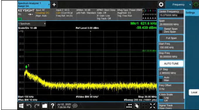
42-42-5MHz-20MHz-QPSK-QPSK-42873-42990-1RB#0-1RB#99- 0.15~30MHz-PASS
