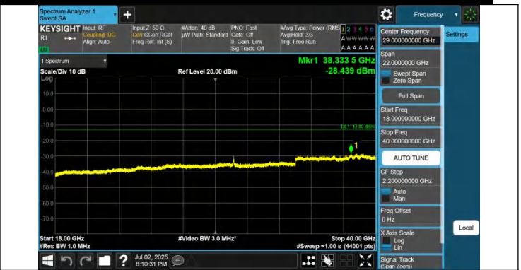
42-42-15MHz-20MHz-QPSK-QPSK-42493-42664-1RB#74-0RB# 0-18000~40000MHz-PASS
