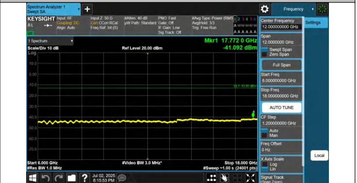
42-42-20MHz-5MHz-QPSK-QPSK-42190-42307-1RB#0-1RB#24-6000~18000MHz-PASS
