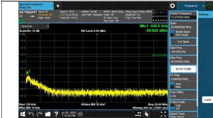
42-42-10MHz-20MHz-QPSK-QPSK-42496-42640-1RB#0-1RB#99-0.15~30MHz-PASS
