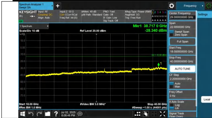
42-42-10MHz-20MHz-QPSK-QPSK-42846-42990-1RB#0-1RB#9 9-18000~40000MHz-PASS
