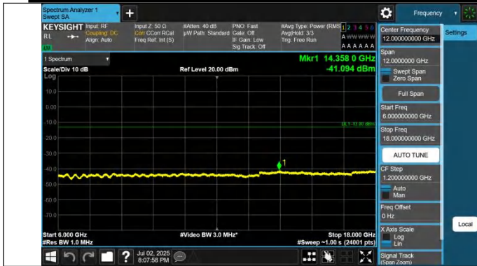
42-42-10MHz-20MHz-QPSK-QPSK-42846-42990-1RB#0-0RB#0-6000~18000MHz-PASS
