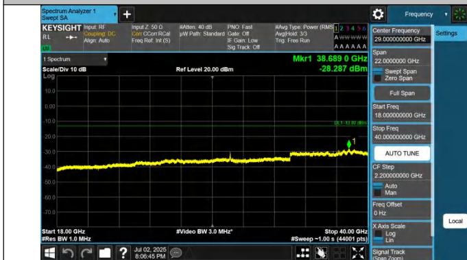
42-42-10MHz-20MHz-QPSK-QPSK-42145-42289-1RB#0-1RB#9 9-18000~40000MHz-PASS
