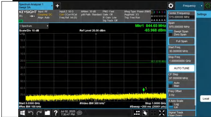
42-42-20MHz-5MHz-QPSK-QPSK-42190-42307-1RB#0-1RB#24-30~1000MHz-PASS
