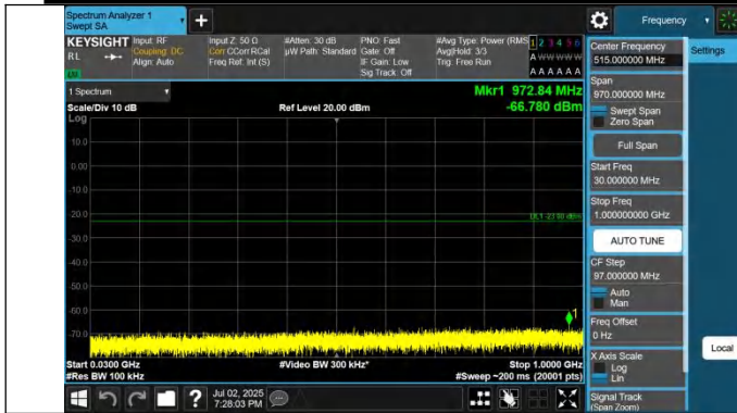
42-42-15MHz-20MHz-QPSK-QPSK-42168-42339-1RB#74-0RB# 0-30~1000MHz-PASS
