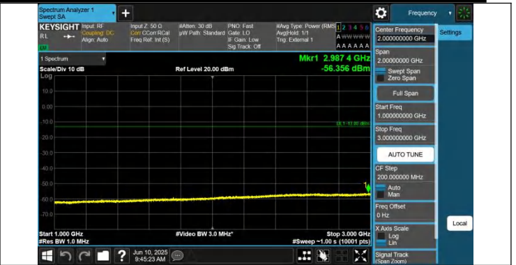
42-42-10MHz-20MHz-QPSK-QPSK-42496-42640-1RB#0-0RB#0-1000~3000MHz-PASS
