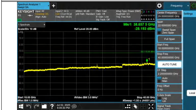
42-42-15MHz-20MHz-QPSK-QPSK-42168-42339-1RB#74-0RB# 0-18000~40000MHz-PASS
