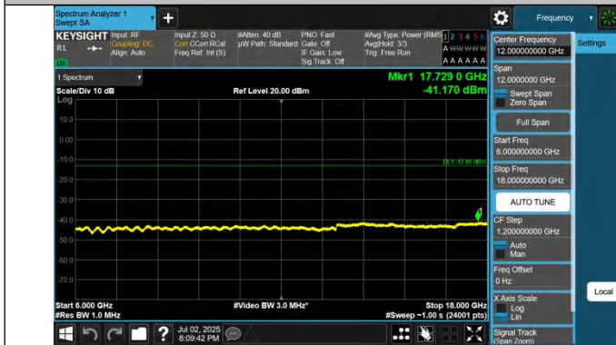
42-42-15MHz-20MHz-QPSK-QPSK-42168-42339-1RB#0-1RB#9 9-6000~18000MHz-PASS
