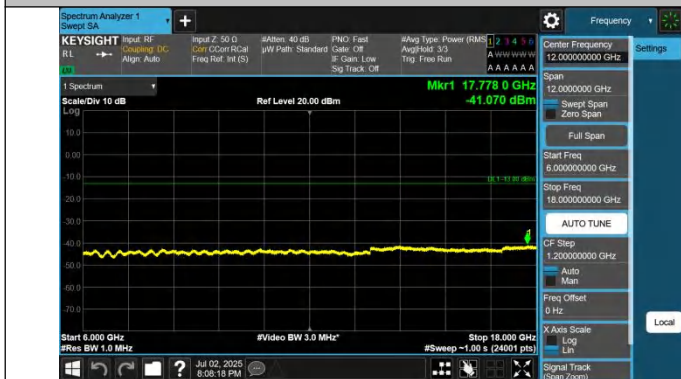
42-42-10MHz-20MHz-QPSK-QPSK-42846-42990-1RB#49-0RB# 0-6000~18000MHz-PASS
