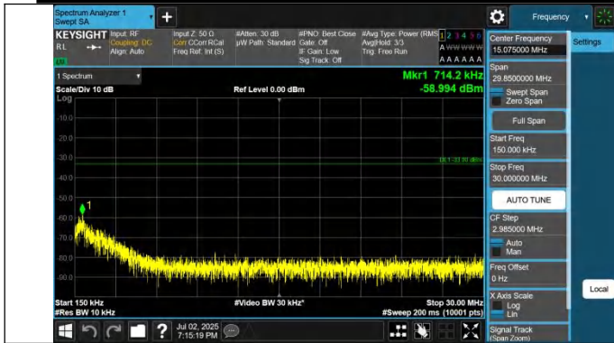
42-42-20MHz-5MHz-QPSK-QPSK-42190-42307-1RB#0-0RB#0-0 .15~30MHz-PASS
