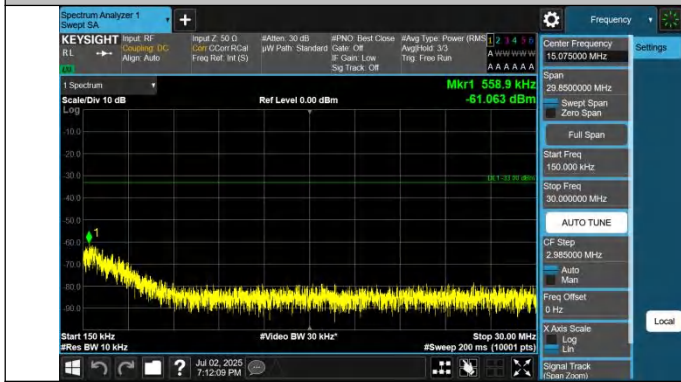
42-42-15MHz-20MHz-QPSK-QPSK-42493-42664-1RB#74-0RB# 0-0.15~30MHz-PASS
