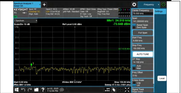
42-42-15MHz-20MHz-QPSK-QPSK-42819-42990-1RB#0-1RB#9 9-0.009~0.15MHz-PASS
