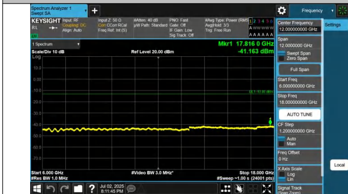
42-42-15MHz-20MHz-QPSK-QPSK-42819-42990-1RB#0-1RB#9 9-6000~18000MHz-PASS
