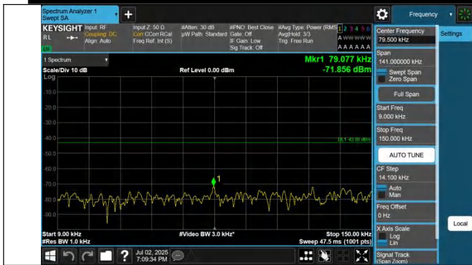
42-42-10MHz-20MHz-QPSK-QPSK-42145-42289-1RB#0-1RB#9 9-0.009~0.15MHz-PASS
