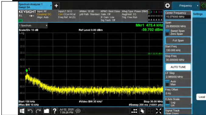
42-42-10MHz-20MHz-QPSK-QPSK-42145-42289-1RB#49-0RB# 0-0.15~30MHz-PASS
