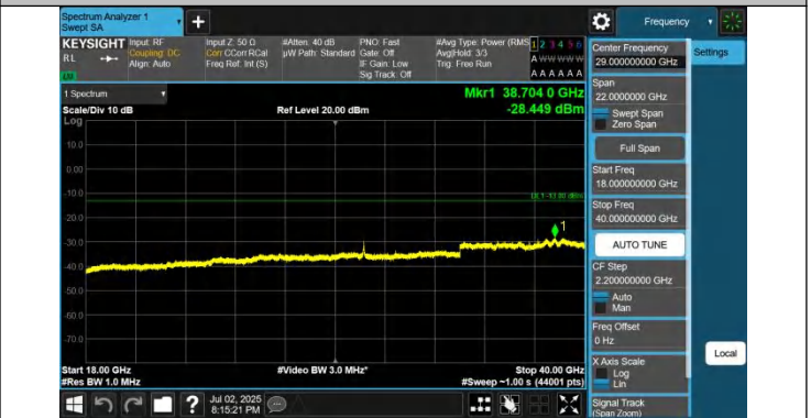
42-42-20MHz-5MHz-QPSK-QPSK-42190-42307-1RB#0-0RB#0-1 8000~40000MHz-PASS
