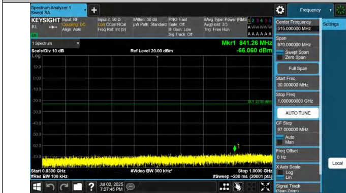
42-42-10MHz-20MHz-QPSK-QPSK-42846-42990-1RB#0-1RB#99-9-0~1000MHz-PASS
