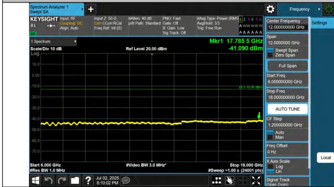
42-42-15MHz-20MHz-QPSK-QPSK-42493-42664-1RB#0-0RB#0-6000~18000MHz-PASS
