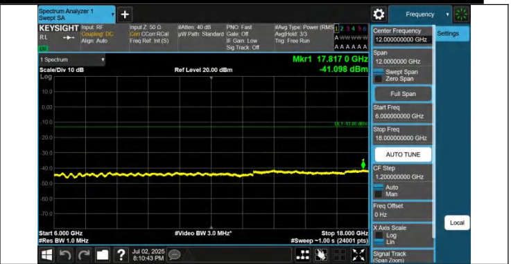
42-42-15MHz-20MHz-QPSK-QPSK-42493-42664-1RB#0-1RB#9 9-6000~18000MHz-PASS
