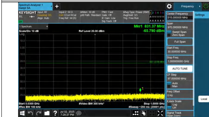
42-42-15MHz-20MHz-QPSK-QPSK-42493-42664-1RB#0-1RB#9 9-30~1000MHz-PASS
