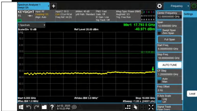
42-42-15MHz-20MHz-QPSK-QPSK-42493-42664-1RB#74-0RB# 0-6000~18000MHz-PASS
