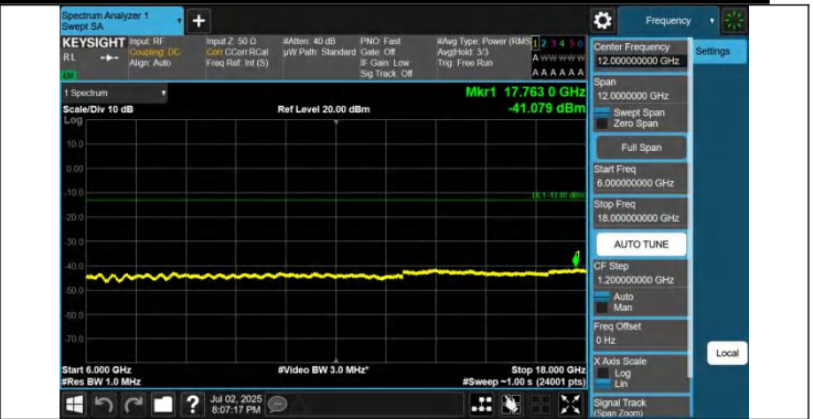
42-42-10MHz-20MHz-QPSK-QPSK-42496-42640-1RB#49-0RB# 0-6000~18000MHz-PASS
