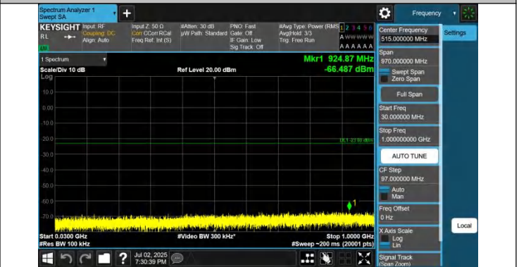
42-42-20MHz-5MHz-QPSK-QPSK-42190-42307-1RB#99-0RB#0-30~1000MHz-PASS
