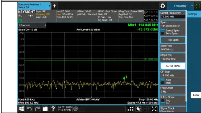
42-42-15MHz-20MHz-QPSK-QPSK-42493-42664-1RB#0-1RB#9 9-0.009~0.15MHz-PASS
