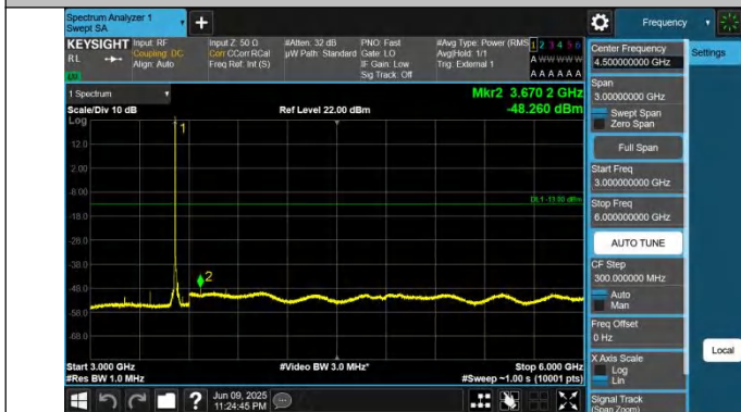
42-42-15MHz-20MHz-QPSK-QPSK-42819-42990-1RB#0-0RB#0- 3000~6000MHz-PASS
