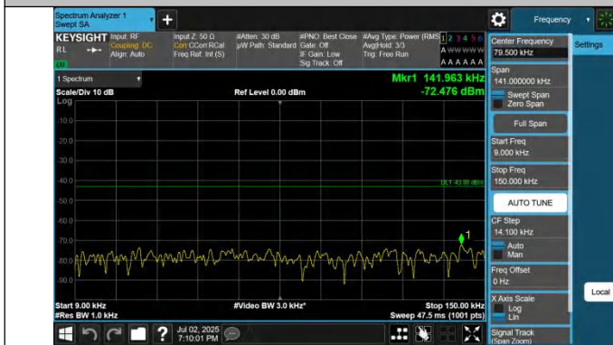
42-42-10MHz-20MHz-QPSK-QPSK-42496-42640-1RB#49-0RB# 0-0.009~0.15MHz-PASS
