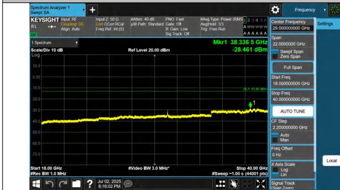
42-42-20MHz-5MHz-QPSK-QPSK-42190-42307-1RB#0-1RB#24-18000~40000MHz-PASS
