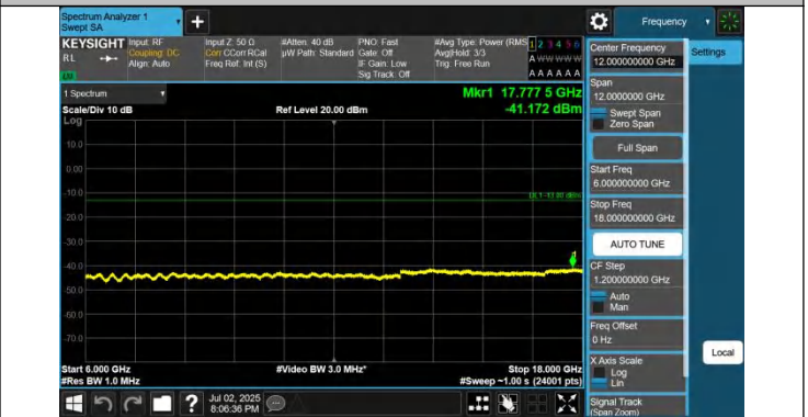
42-42-10MHz-20MHz-QPSK-QPSK-42145-42289-1RB#0-1RB#9 9-6000~18000MHz-PASS
