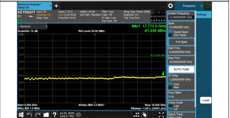
42-42-15MHz-20MHz-QPSK-QPSK-42168-42339-1RB#74-0RB# 0-6000~18000MHz-PASS
