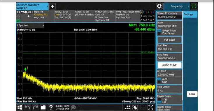
42-42-10MHz-20MHz-QPSK-QPSK-42496-42640-1RB#49-0RB# 0-0.15~30MHz-PASS
