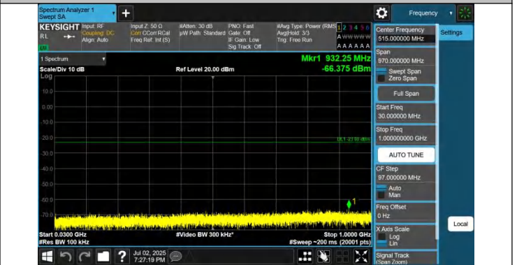
42-42-10MHz-20MHz-QPSK-QPSK-42496-42640-1RB#0-1RB#99-30~1000MHz-PASS
