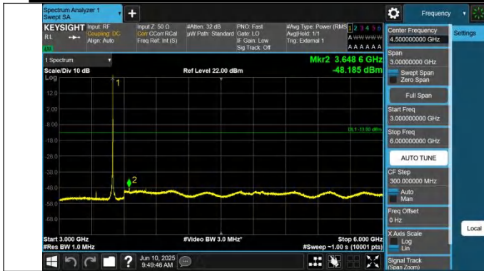
42-42-10MHz-20MHz-QPSK-QPSK-42496-42640-1RB#49-0RB# 0-3000~6000MHz-PASS
