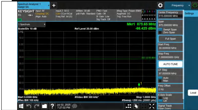
42-42-10MHz-20MHz-QPSK-QPSK-42496-42640-1RB#0-0RB#0-30~1000MHz-PASS
