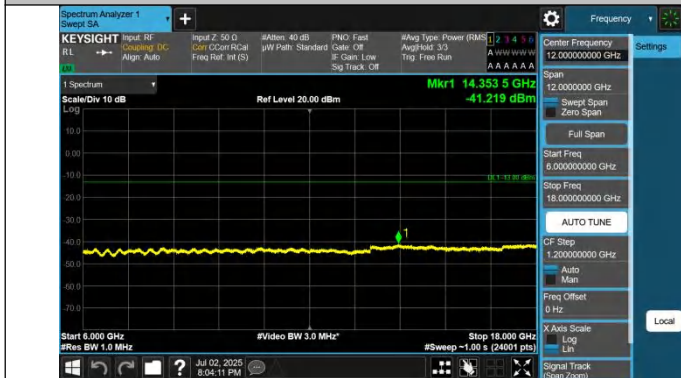
42-42-5MHz-20MHz-QPSK-QPSK-42498-42615-1RB#24-0RB#0-6000~18000MHz-PASS
