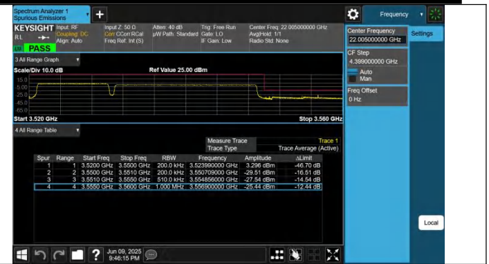
42-42-10MHz-20MHz-QPSK@QPSK-QPSK@QPSK-42846-42990 -50RB#0@50RB#0-100RB#0@100RB#0-PASS
