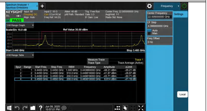
42-42-15MHz-20MHz-QPSK@QPSK-QPSK@QPSK-42168-42339 -1RB#0@75RB#0-1RB#99@100RB#0-PASS
