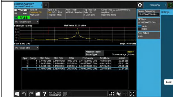
42-42-10MHz-20MHz-QPSK@QPSK-QPSK@QPSK-42145-422 89-1RB#49@50RB#0-0RB#0@100RB#0-PASS
