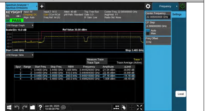
42-42-15MHz-20MHz-QPSK@QPSK-QPSK@QPSK-42168-42339 -75RB#0@75RB#0-100RB#0@100RB#0-PASS
