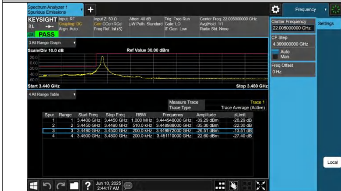
42-42-20MHz-10MHz-QPSK@QPSK-QPSK@QPSK-42190-423 34-1RB#0@100RB#0-0RB#0@50RB#0-PASS
