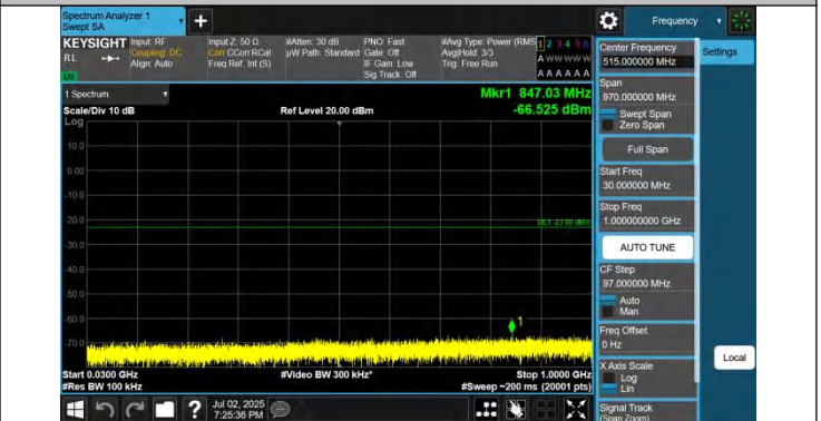
42-42-5MHz-20MHz-QPSK-QPSK-42123-42240-1RB#0-1RB#99- 30~1000MHz-PASS
