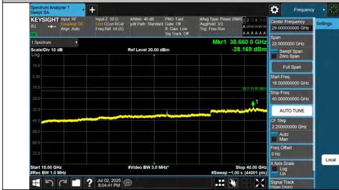
42-42-5MHz-20MHz-QPSK-QPSK-42498-42615-1RB#0-1RB#99- 18000~40000MHz-PASS
