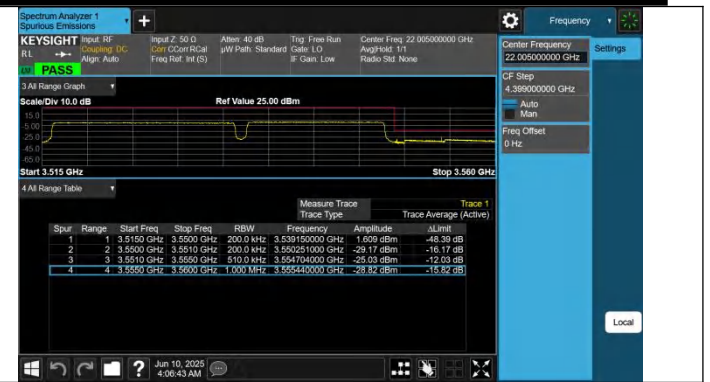
42-42-20MHz-15MHz-QPSK@QPSK-QPSK@QPSK-42841-43012 -100RB#0@100RB#0-75RB#0@75RB#0-PASS
