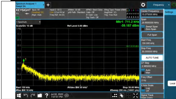
42-42-5MHz-20MHz-QPSK-QPSK-42498-42615-1RB#0-0RB#0-0 .15~30MHz-PASS
