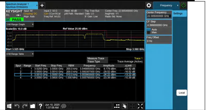
42-42-20MHz-5MHz-QPSK@QPSK-QPSK@QPSK-42940-43057- 100RB#0@100RB#0-25RB#0@25RB#0-PASS
