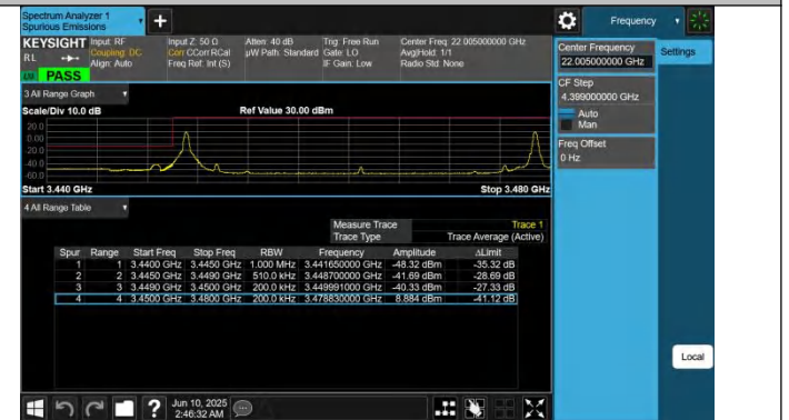
42-42-20MHz-10MHz-QPSK@QPSK-QPSK@QPSK-42190-42334 -1RB#0@100RB#0-1RB#49@50RB#0-PASS
