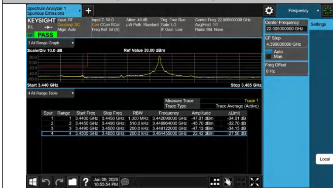
42-42-15MHz-20MHz-QPSK@QPSK-QPSK@QPSK-42168-423 39-1RB#74@75RB#0-0RB#0@100RB#0-PASS
