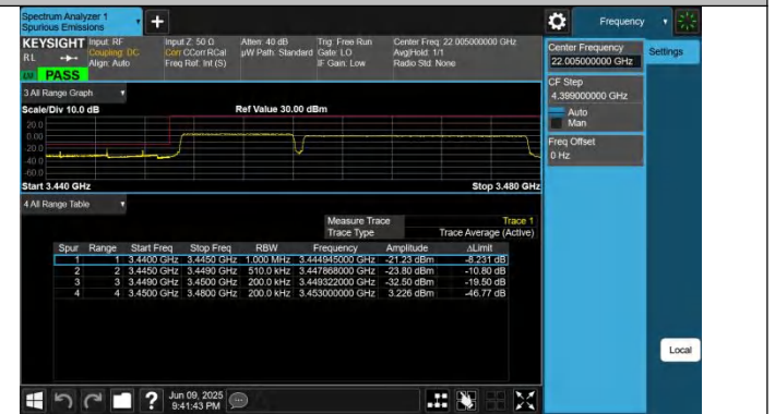
42-42-10MHz-20MHz-QPSK@QPSK-QPSK@QPSK-42145-42289 -50RB#0@50RB#0-100RB#0@100RB#0-PASS
