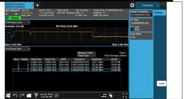
42-42-5MHz-20MHz-QPSK@QPSK-QPSK@QPSK-42873-42990- 25RB#0@25RB#0-100RB#0@100RB#0-PASS
