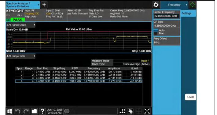
42-42-20MHz-10MHz-QPSK@QPSK-QPSK@QPSK-42190-42334 -100RB#0@100RB#0-50RB#0@50RB#0-PASS
