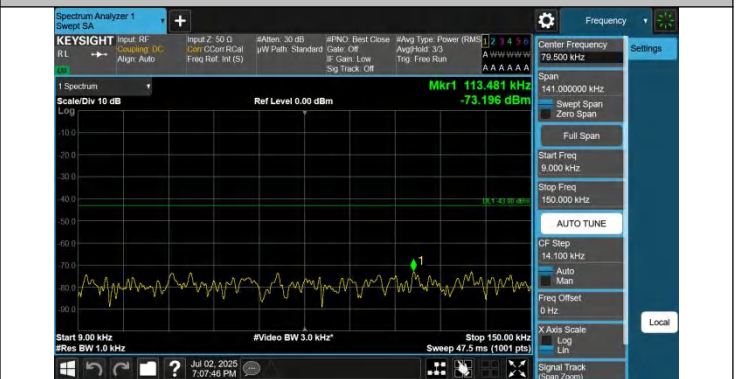
42-42-5MHz-20MHz-QPSK-QPSK-42498-42615-1RB#0-0RB#0-0 .009~0.15MHz-PASS
