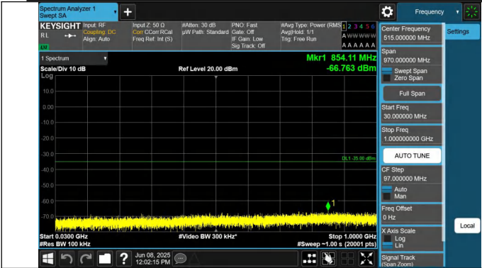
7-7-15MHz-15MHz-QPSK-QPSK-21225-21375-1RB#74-0RB#0-30~1000MHz-PASS
