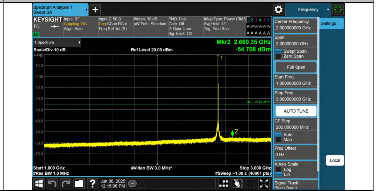
7-7-15MHz-20MHz-QPSK-QPSK-21003-21174-1RB#74-0RB#0-1 000~3000MHz-PASS
