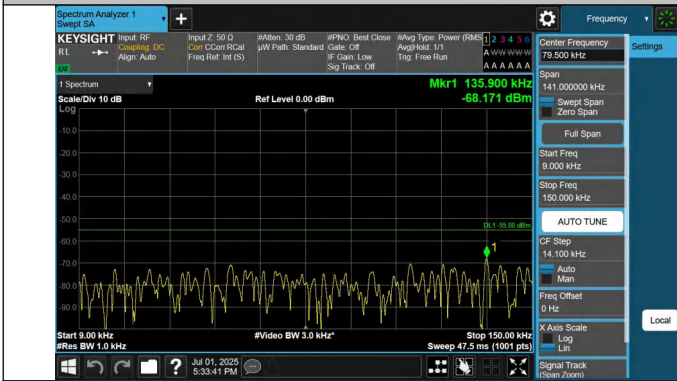
7-7-15MHz-15MHz-QPSK-QPSK-21225-21375-1RB#74-0RB#0-0.009~0.15MHz-PASS
