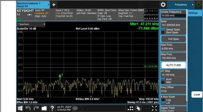
7-7-15MHz-20MHz-QPSK-QPSK-21003-21174-1RB#0-0RB#0-0.009~0.15MHz-PASS
