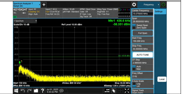
7-7-15MHz-15MHz-QPSK-QPSK-21225-21375-1RB#0-0RB#0-1 5~30MHz-PASS
