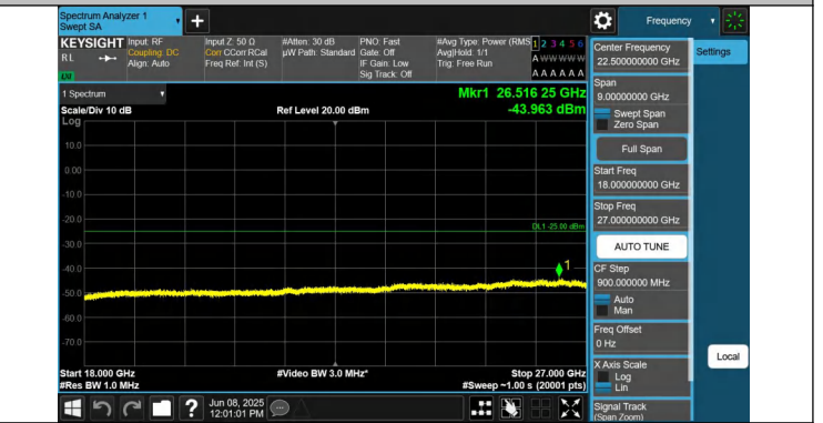
7-7-15MHz-15MHz-QPSK-QPSK-21025-21175-1RB#0-1RB#74-1 8000~27000MHz-PASS
