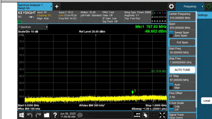
7-7-15MHz-15MHz-QPSK-QPSK-21025-21175-1RB#74-0RB#0-3 0~1000MHz-PASS
