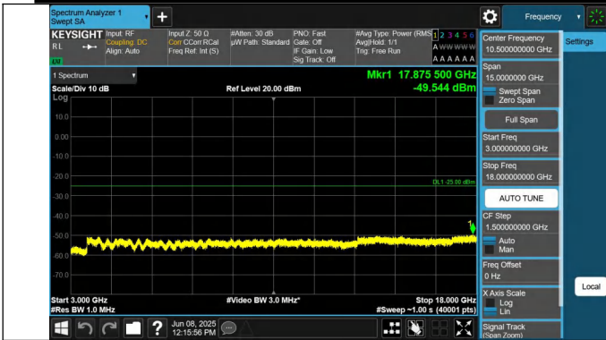
7-7-15MHz-20MHz-QPSK-QPSK-21003-21174-1RB#0-1RB#99-3 000~18000MHz-PASS
