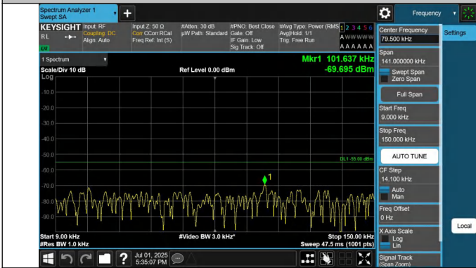
7-7-15MHz-20MHz-QPSK-QPSK-21003-21174-1RB#74-0RB#0-0 .009~0.15MHz-PASS
