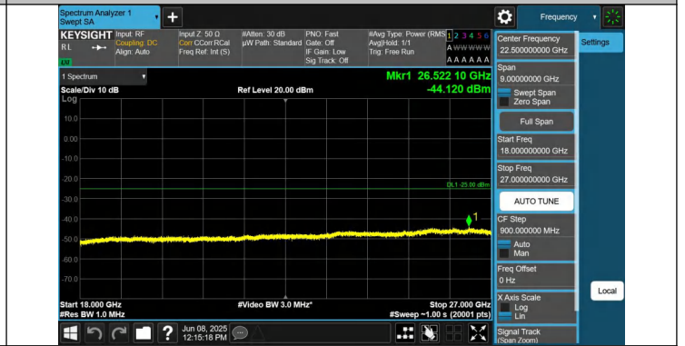
7-7-15MHz-20MHz-QPSK-QPSK-21003-21174-1RB#74-0RB#0-1 8000~27000MHz-PASS
