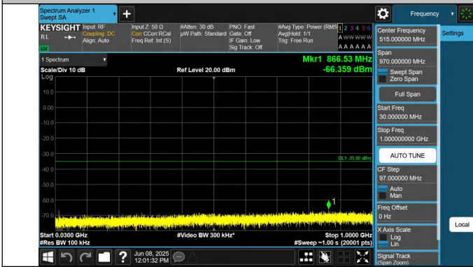
7-7-15MHz-15MHz-QPSK-QPSK-21225-21375-1RB#0-0RB#0-3 0~1000MHz-PASS
