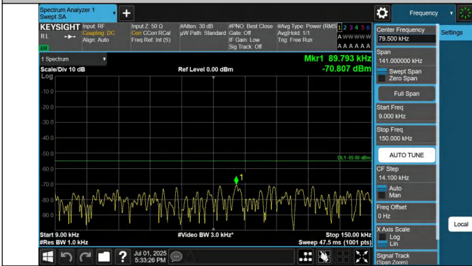
7-7-15MHz-15MHz-QPSK-QPSK-21225-21375-1RB#0-0RB#0-0. 009~0.15MHz-PASS
