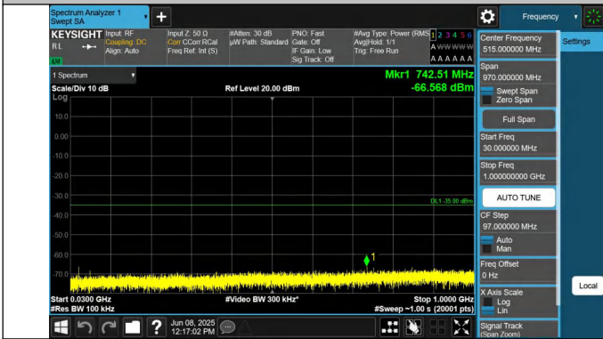
7-7-15MHz-20MHz-QPSK-QPSK-21179-21350-1RB#0-0RB#0-30 ~1000MHz-PASS
