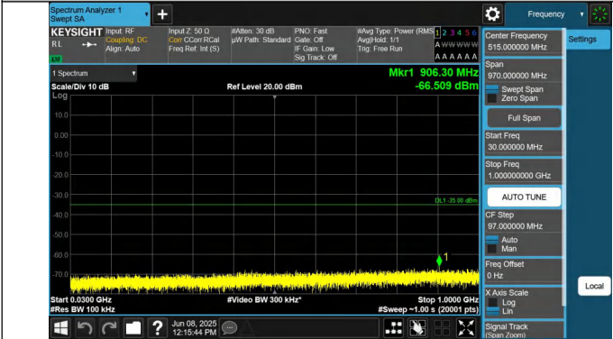
7-7-15MHz-20MHz-QPSK-QPSK-21003-21174-1RB#0-1RB#99-3 0~1000MHz-PASS
