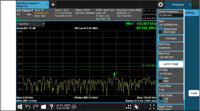
7-7-15MHz-20MHz-QPSK-QPSK-20828-20999-1RB#0-0RB#0-0.009~0.15MHz-PASS
