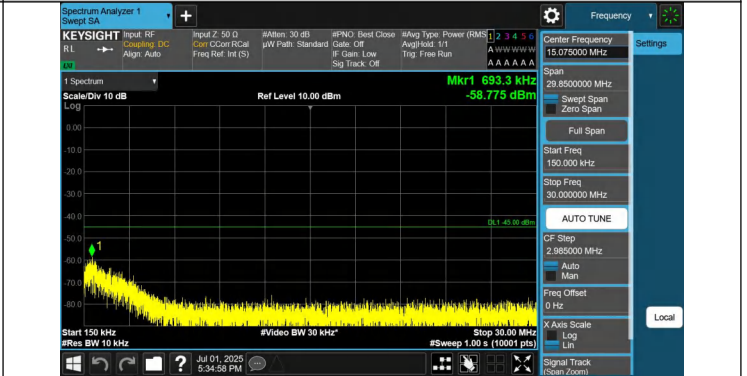
7-7-15MHz-20MHz-QPSK-QPSK-21003-21174-1RB#0-0RB#0-0.15~30MHz-PASS
