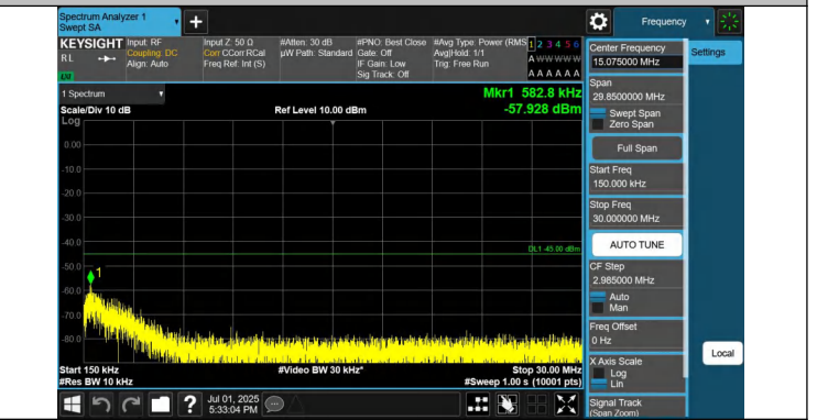
7-7-15MHz-15MHz-QPSK-QPSK-21025-21175-1RB#74-0RB#0-0. 15~30MHz-PASS
