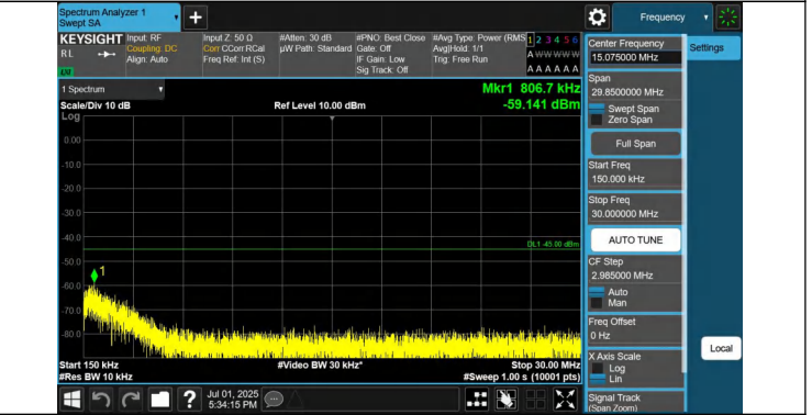
7-7-15MHz-20MHz-QPSK-QPSK-20828-20999-1RB#0-0RB#0-0.15~30MHz-PASS
