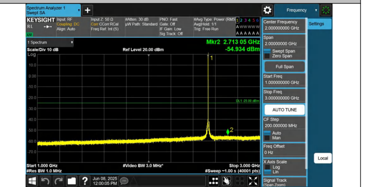
7-7-15MHz-15MHz-QPSK-QPSK-21025-21175-1RB#74-0RB#0-1 000~3000MHz-PASS
