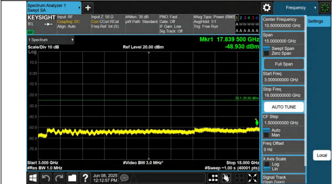
7-7-15MHz-20MHz-QPSK-QPSK-20828-20999-1RB#74-0RB#0-3000~18000MHz-PASS
