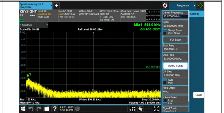
7-7-15MHz-15MHz-QPSK-QPSK-21225-21375-1RB#74-0RB#0-0.15~30MHz-PASS
