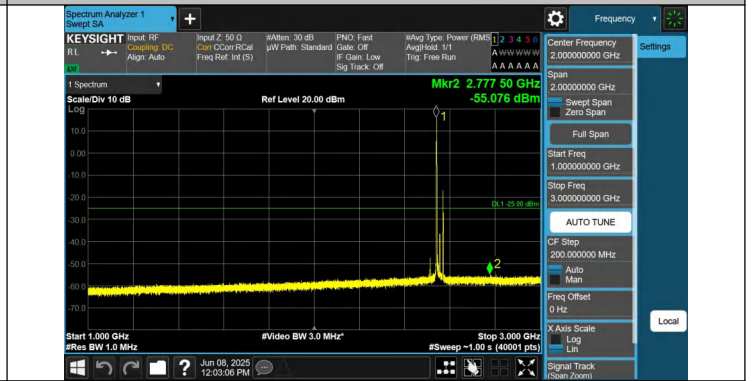
7-7-15MHz-15MHz-QPSK-QPSK-21225-21375-1RB#0-1RB#74-1000~3000MHz-PASS
