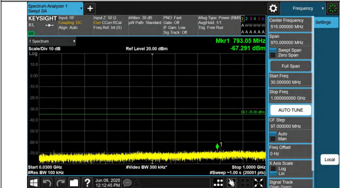
7-7-15MHz-20MHz-QPSK-QPSK-20828-20999-1RB#74-0RB#0-30~1000MHz-PASS
