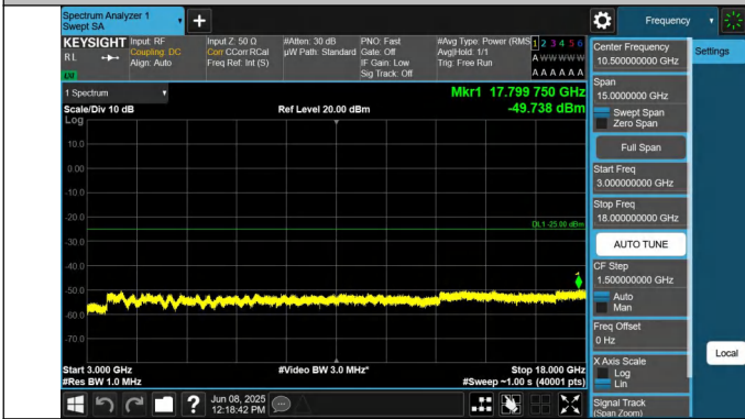
7-7-15MHz-20MHz-QPSK-QPSK-21179-21350-1RB#0-1RB#99-3 000~18000MHz-PASS
