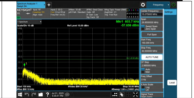
7-7-15MHz-20MHz-QPSK-QPSK-21179-21350-1RB#0-0RB#0-0.1 5~30MHz-PASS
