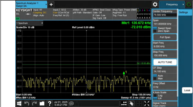
7-7-15MHz-20MHz-QPSK-QPSK-21003-21174-1RB#0-1RB#99-0 .009~0.15MHz-PASS
