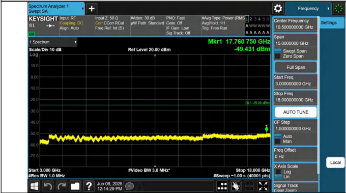
7-7-15MHz-20MHz-QPSK-QPSK-21003-21174-1RB#0-0RB#0-30 00~18000MHz-PASS
