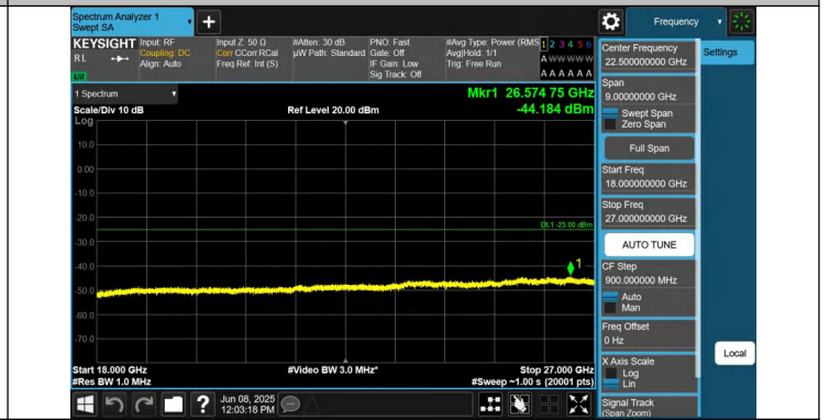
7-7-15MHz-15MHz-QPSK-QPSK-21225-21375-1RB#0-1RB#74-18000~27000MHz-PASS
