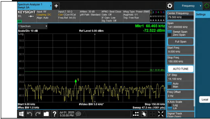
7-7-15MHz-15MHz-QPSK-QPSK-21225-21375-1RB#0-1RB#74-0.009~0.15MHz-PASS
