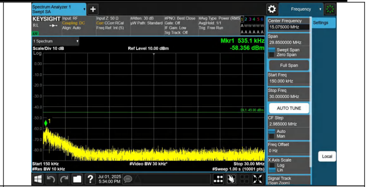
7-7-15MHz-15MHz-QPSK-QPSK-21225-21375-1RB#0-1RB#74-0.15~30MHz-PASS
