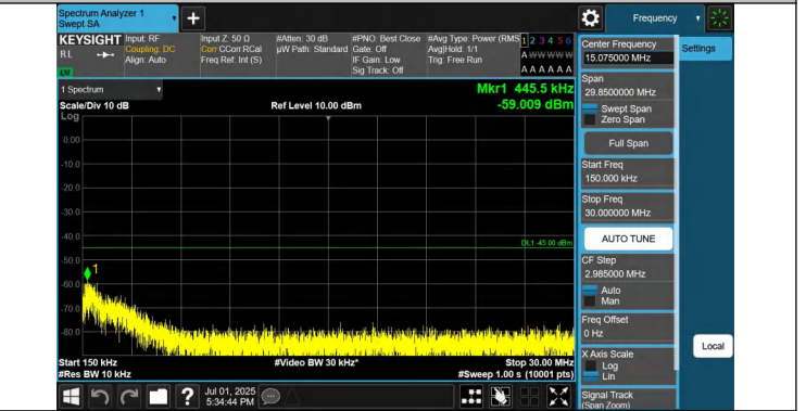
7-7-15MHz-20MHz-QPSK-QPSK-20828-20999-1RB#0-1RB#99-0. 15~30MHz-PASS
