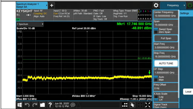
7-7-15MHz-20MHz-QPSK-QPSK-21003-21174-1RB#74-0RB#0-3 000~18000MHz-PASS
