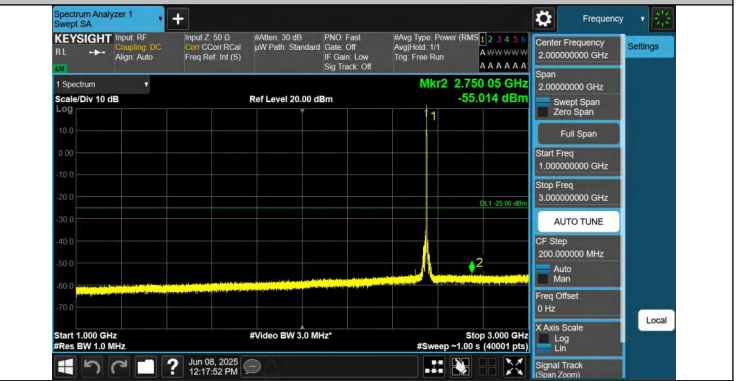
7-7-15MHz-20MHz-QPSK-QPSK-21179-21350-1RB#74-0RB#0-1 000~3000MHz-PASS
