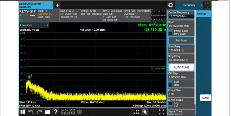
7-7-15MHz-20MHz-QPSK-QPSK-20828-20999-1RB#74-0RB#0-0.15~30MHz-PASS
