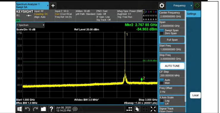
7-7-15MHz-20MHz-QPSK-QPSK-21003-21174-1RB#0-0RB#0-10 00~3000MHz-PASS
