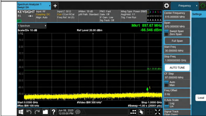
7-7-15MHz-15MHz-QPSK-QPSK-21225-21375-1RB#0-1RB#74-30~1000MHz-PASS
