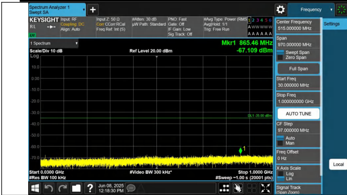
7-7-15MHz-20MHz-QPSK-QPSK-21179-21350-1RB#0-1RB#99-3 0~1000MHz-PASS
