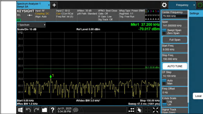
7-7-15MHz-20MHz-QPSK-QPSK-20828-20999-1RB#0-1RB#99- 0.009~0.15MHz-PASS
