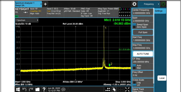
7-7-15MHz-20MHz-QPSK-QPSK-20828-20999-1RB#74-0RB#0-1000~3000MHz-PASS
