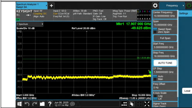
7-7-15MHz-20MHz-QPSK-QPSK-21179-21350-1RB#0-0RB#0-30 00~18000MHz-PASS
