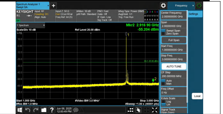
7-7-15MHz-15MHz-QPSK-QPSK-21025-21175-1RB#0-1RB#74-1 000~3000MHz-PASS
