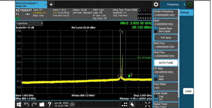
7-7-15MHz-20MHz-QPSK-QPSK-21003-21174-1RB#0-1RB#99-1 000~3000MHz-PASS
