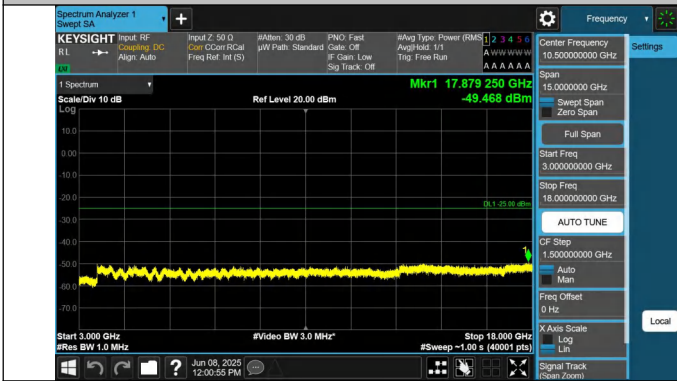
7-7-15MHz-15MHz-QPSK-QPSK-21025-21175-1RB#0-1RB#74-3 000~18000MHz-PASS
