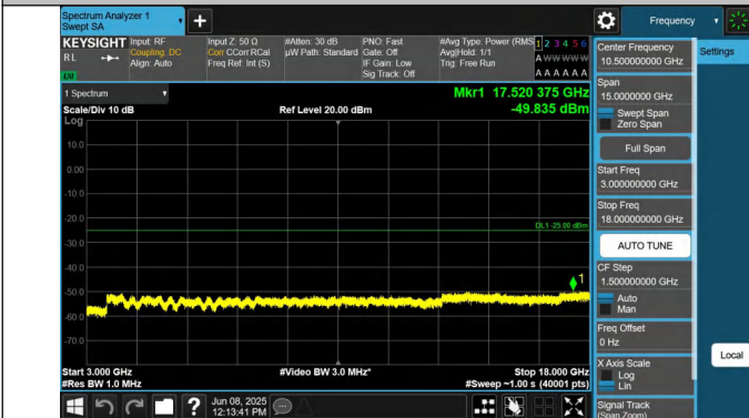
7-7-15MHz-20MHz-QPSK-QPSK-20828-20999-1RB#0-1RB#99- 3000~18000MHz-PASS
