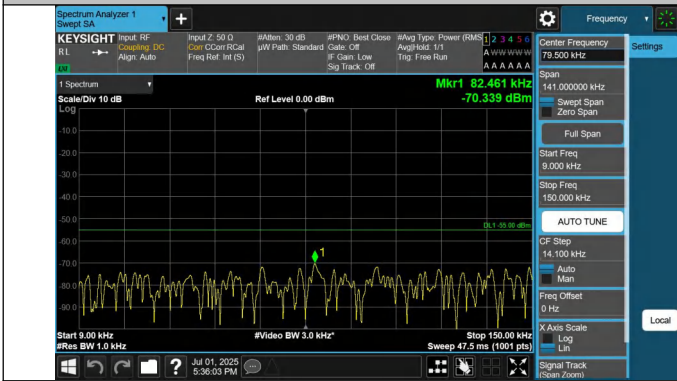
7-7-15MHz-20MHz-QPSK-QPSK-21179-21350-1RB#0-1RB#99-0 .009~0.15MHz-PASS
