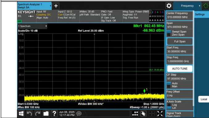
7-7-15MHz-20MHz-QPSK-QPSK-21179-21350-1RB#74-0RB#0-3 0~1000MHz-PASS
