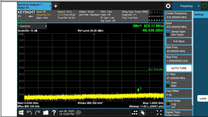
7-7-15MHz-20MHz-QPSK-QPSK-21003-21174-1RB#74-0RB#0-3 0~1000MHz-PASS
