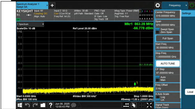
7-7-15MHz-15MHz-QPSK-QPSK-21025-21175-1RB#0-1RB#74-3 0~1000MHz-PASS
