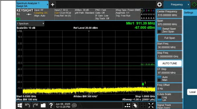
7-7-15MHz-20MHz-QPSK-QPSK-20828-20999-1RB#0-1RB#99- 30~1000MHz-PASS
