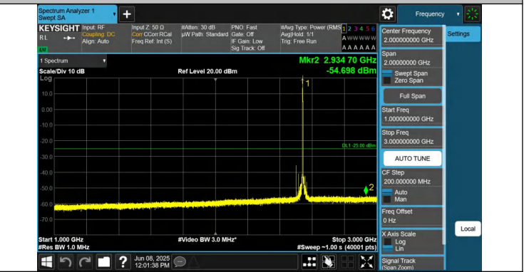
7-7-15MHz-15MHz-QPSK-QPSK-21225-21375-1RB#0-0RB#0-10 00~3000MHz-PASS
