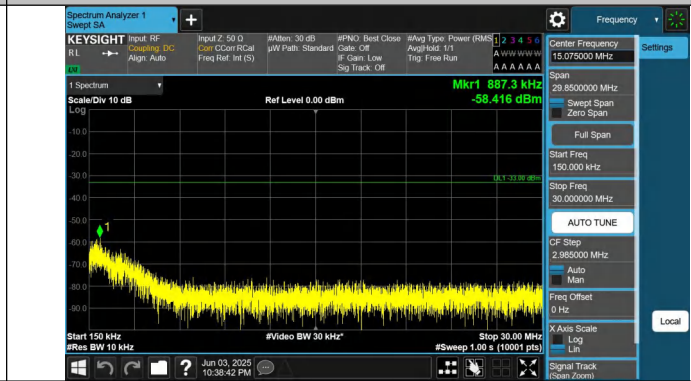
Band66-5MHz-QPSK-131997-1RB#0-0.15~30-PASS
