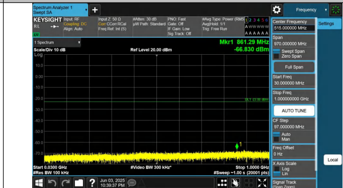
Band66-5MHz-QPSK-131997-1RB#24-30~1000-PASS
