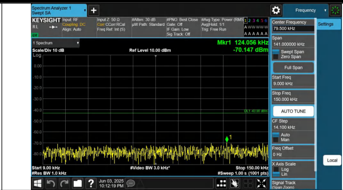
Band66-1.4MHz-QPSK-132665-1RB#5-0.009~0.15-PASS
