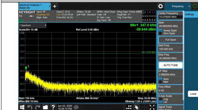
Band66-3MHz-QPSK-132322-1RB#14-0.15~30-PASS
