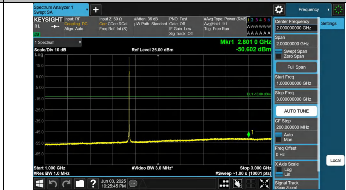
Band66-3MHz-QPSK-132322-1RB#0-1000~3000-PASS
