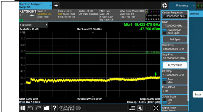
Band66-5MHz-QPSK-131997-1RB#0-3000~20000-PASS
