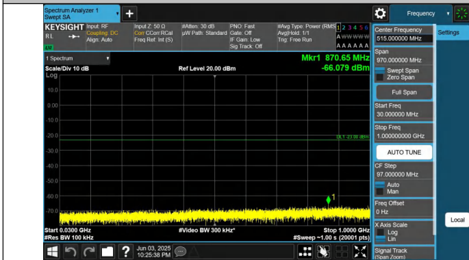
Band66-3MHz-QPSK-132322-1RB#0-30~1000-PASS
