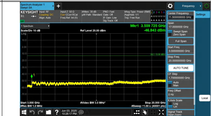
Band66-3MHz-QPSK-132657-1RB#14-3000~20000-PASS
