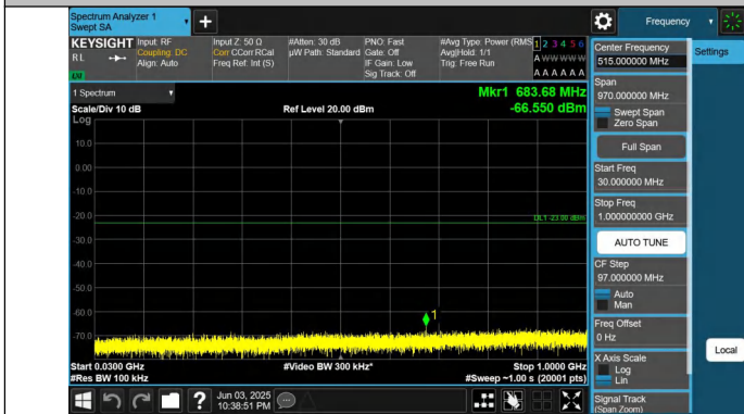
Band66-5MHz-QPSK-131997-1RB#0-30~1000-PASS
