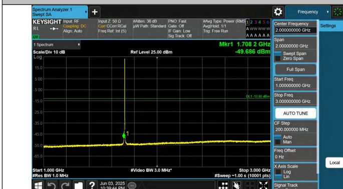
Band66-5MHz-QPSK-131997-1RB#24-1000~3000-PASS
