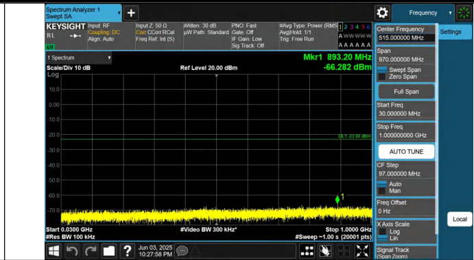
Band66-3MHz-QPSK-132657-1RB#14-30~1000-PASS
