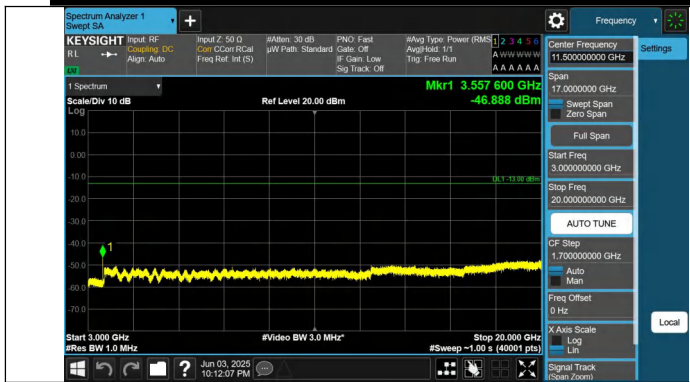
Band66-1.4MHz-QPSK-132665-1RB#0-3000~20000-PASS
