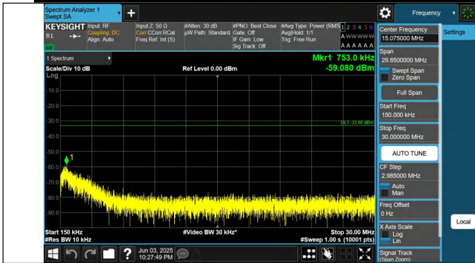
Band66-3MHz-QPSK-132657-1RB#14-0.15~30-PASS
