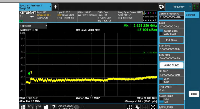
Band66-5MHz-QPSK-131997-1RB#24-3000~20000-PASS
