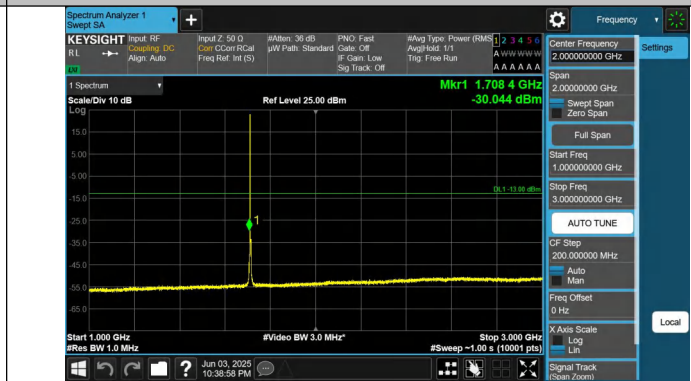
Band66-5MHz-QPSK-131997-1RB#0-1000~3000-PASS
