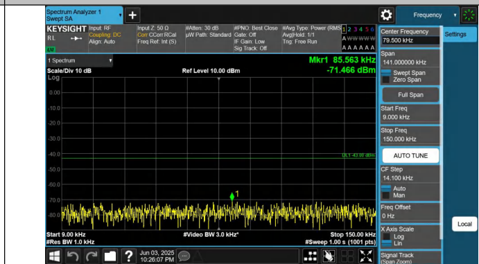
Band66-3MHz-QPSK-132322-1RB#14-0.009~0.15-PASS
