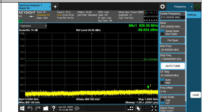
Band66-1.4MHz-QPSK-132665-1RB#5-30~1000-PASS
