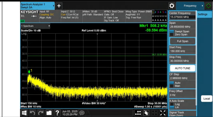
Band66-3MHz-QPSK-132322-1RB#0-0.15~30-PASS
