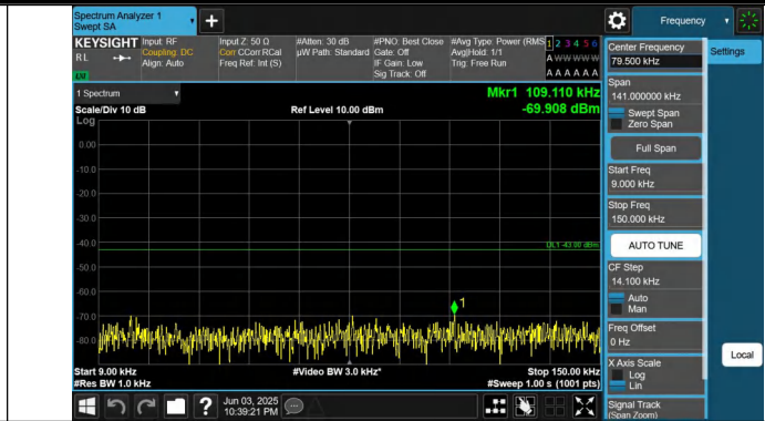
Band66-5MHz-QPSK-131997-1RB#24-0.009~0.15-PASS
