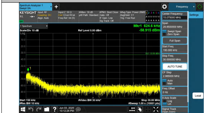
Band66-1.4MHz-QPSK-132665-1RB#5-0.15~30-PASS
