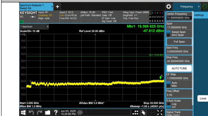
Band66-3MHz-QPSK-132322-1RB#0-3000~20000-PASS
