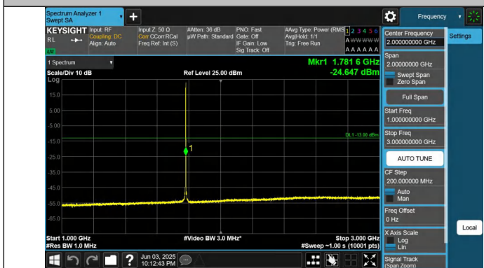
Band66-1.4MHz-QPSK-132665-1RB#5-1000~3000-PASS
