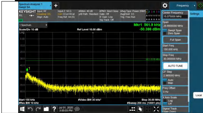
Band42(3450-3550)-15MHz-QPSK-43015-1RB#74-0.15~30-PAS S
