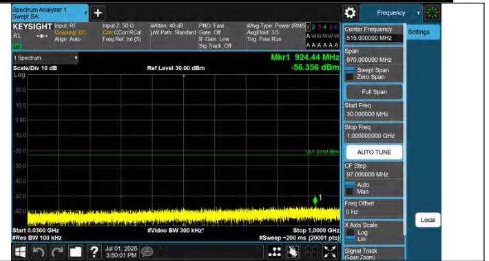
Band42(3450-3550)-15MHz-QPSK-42165-1RB#74-30~1000-PASS
