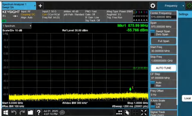
Band42(3450-3550)-20MHz-QPSK-42590-1RB#0-30~1000-PASS
