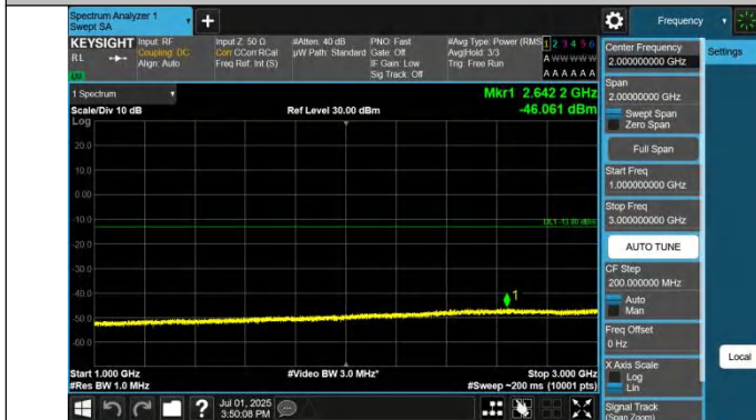
Band42(3450-3550)-15MHz-QPSK-42165-1RB#74-1000~3000-P
