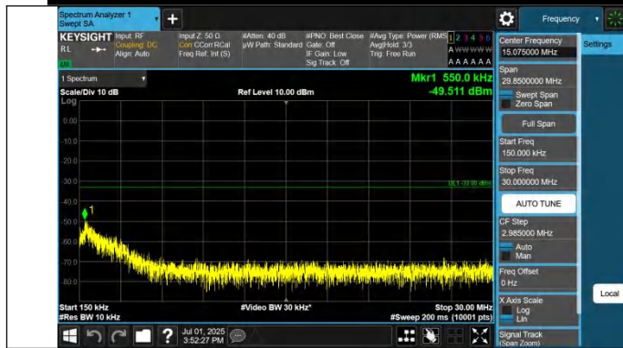
Band42(3450-3550)-15MHz-QPSK-42590-1RB#74-0.15~30-PAS
