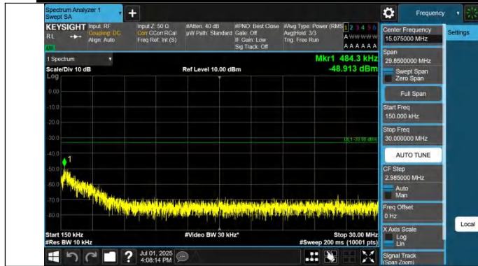
Band42(3450-3550)-20MHz-QPSK-42590-1RB#99-0.15~30-PAS
