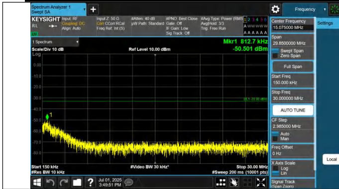
Band42(3450-3550)-15MHz-QPSK-42165-1RB#74-0.15~30-PAS
