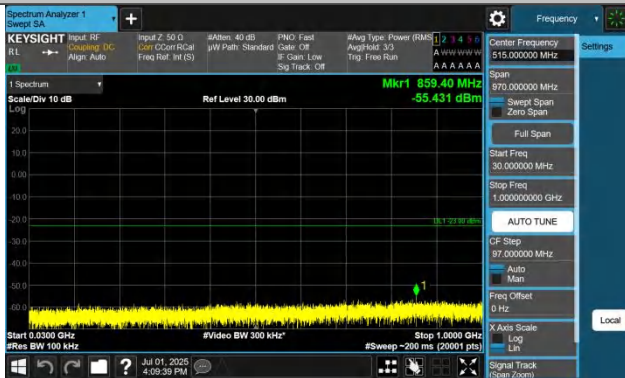
Band42(3450-3550)-20MHz-QPSK-42990-1RB#0-30~1000-PASS
