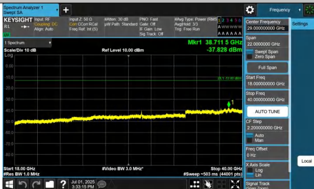
Band42(3450-3550)-10MHz-QPSK-42590-1RB#0-18000~40000-P
