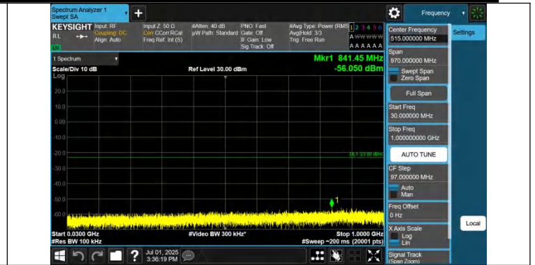
Band42(3450-3550)-10MHz-QPSK-43040-1RB#49-30~1000-PASS
