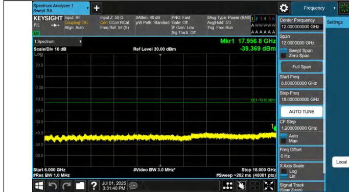
Band42(3450-3550)-10MHz-QPSK-42140-1RB#49-6000~18000-P
