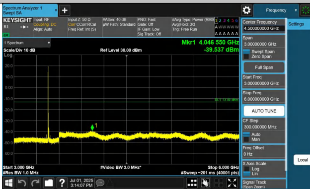
Band42(3450-3550)-15MHz-QPSK-42165-1RB#0-3000~6000-PA
