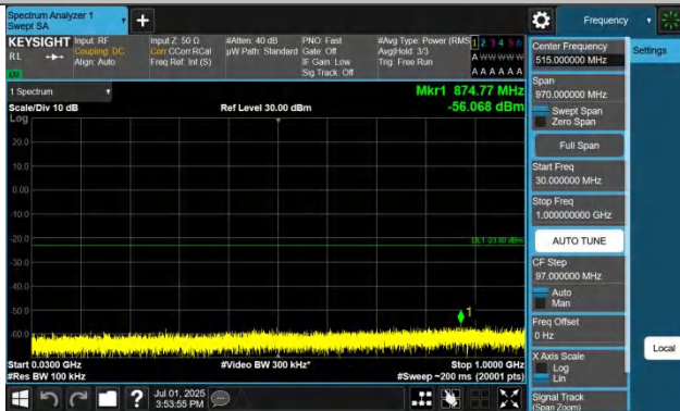
Band42(3450-3550)-15MHz-QPSK-43015-1RB#0-30~1000-PASS
