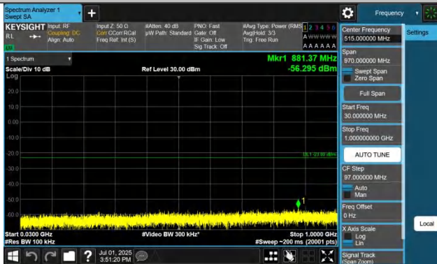
Band42(3450-3550)-15MHz-QPSK-42590-1RB#0-30~1000-PASS
