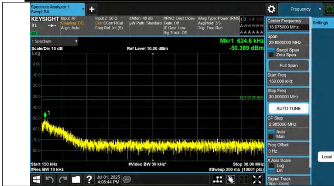
Band42(3450-3550)-20MHz-QPSK-42190-1RB#99-0.15~30-PAS
