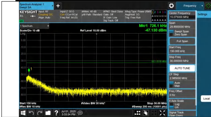
Band42(3450-3550)-10MHz-QPSK-42590-1RB#49-0.15~30-PAS
