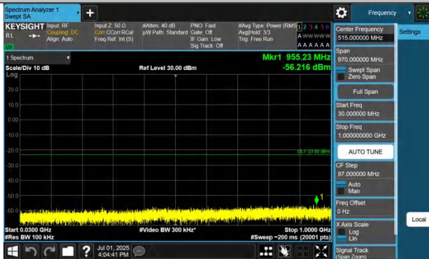
Band42(3450-3550)-20MHz-QPSK-42190-1RB#0-30~1000-PASS
