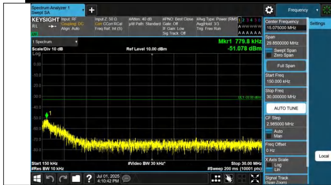
Band42(3450-3550)-20MHz-QPSK-42990-1RB#99-0.15~30-PAS
