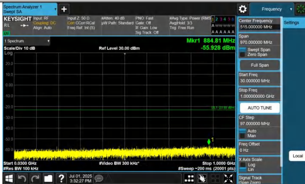
Band42(3450-3550)-10MHz-QPSK-42590-1RB#0-30~1000-PASS
