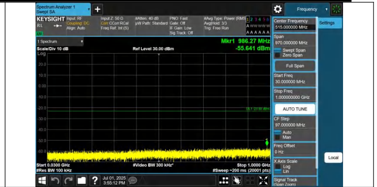
Band42(3450-3550)-15MHz-QPSK-43015-1RB#74-30~1000-PASS
