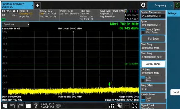
Band42(3450-3550)-15MHz-QPSK-42165-1RB#0-30~1000-PASS
