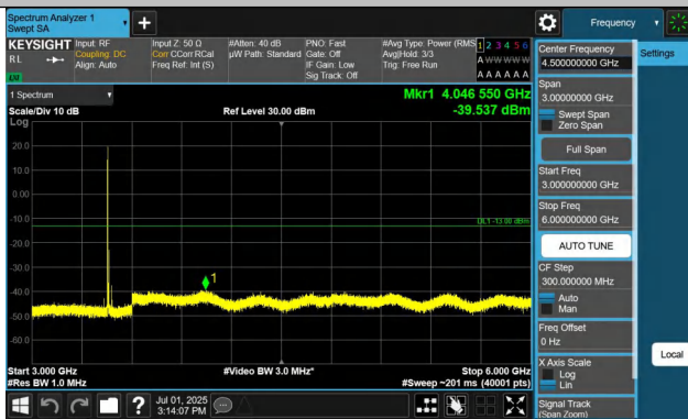
Band42(3450-3550)-15MHz-QPSK-43015-1RB#0-3000~6000-PA
