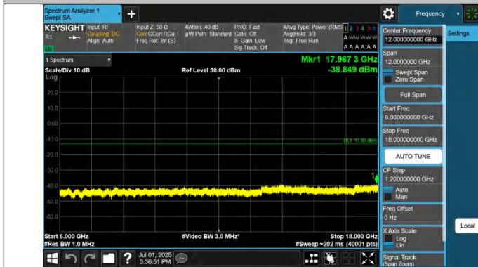
Band42(3450-3550)-10MHz-QPSK-43040-1RB#49-6000~18000-P ASS
