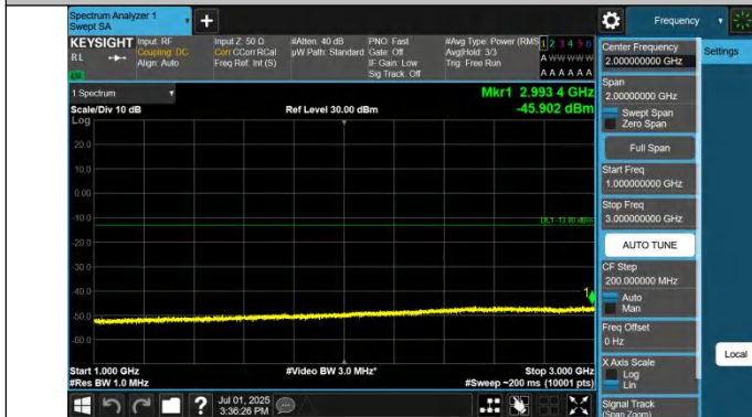
Band42(3450-3550)-10MHz-QPSK-43040-1RB#49-1000~3000-P ASS
