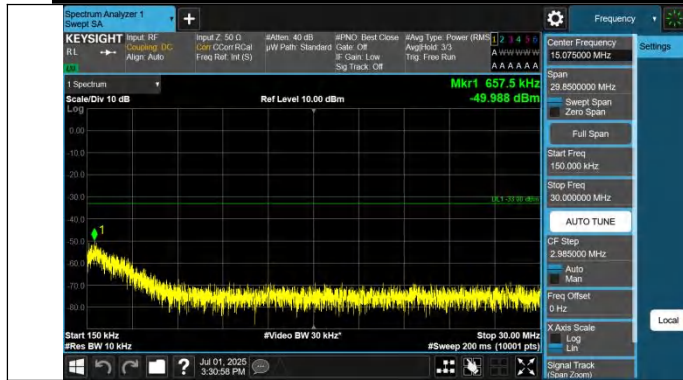
Band42(3450-3550)-10MHz-QPSK-42140-1RB#49-0.15~30-PAS
