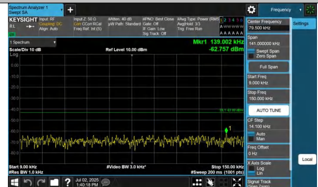
Band42(3450-3550)-10MHz-QPSK-42590-1RB#49-0.009~0.15-PA
