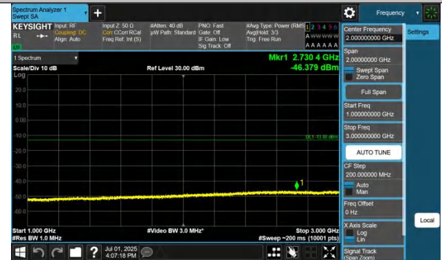
Band42(3450-3550)-20MHz-QPSK-42590-1RB#0-1000~3000-PAS
