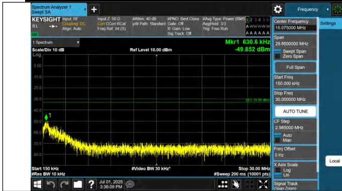
Band42(3450-3550)-10MHz-QPSK-43040-1RB#49-0.15~30-PAS S
