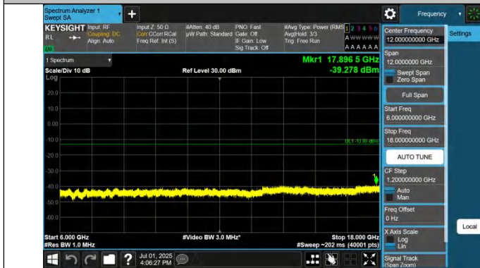
Band42(3450-3550)-20MHz-QPSK-42190-1RB#99-6000~18000-P
