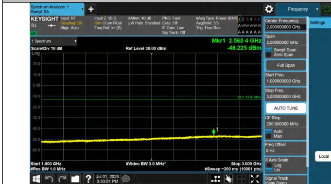
Band42(3450-3550)-10MHz-QPSK-42590-1RB#49-1000~3000-P
