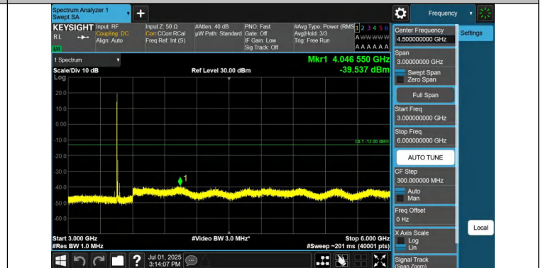
Band42(3450-3550)-10MHz-QPSK-42140-1RB#49-3000~6000-PA
