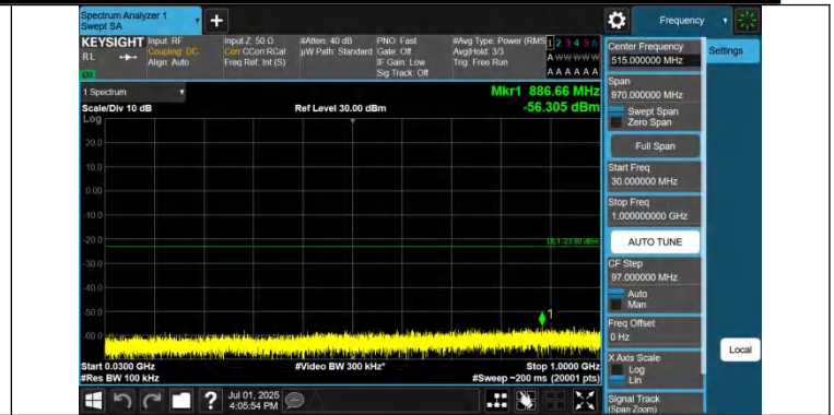
Band42(3450-3550)-20MHz-QPSK-42190-1RB#99-30~1000-PASS
