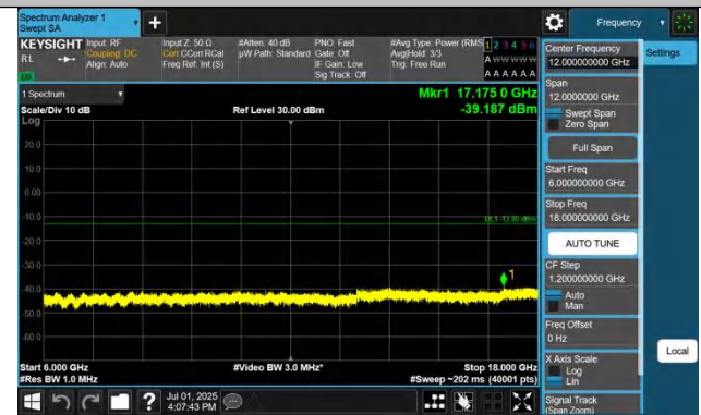
Band42(3450-3550)-20MHz-QPSK-42590-1RB#0-6000~18000-PA
