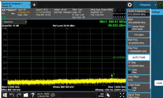
Band42(3450-3550)-10MHz-QPSK-43040-1RB#0-30~1000-PASS
