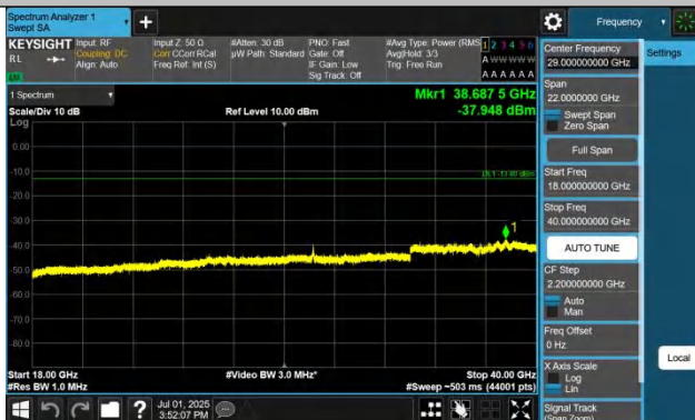
Band42(3450-3550)-15MHz-QPSK-42590-1RB#0-18000~40000-P
