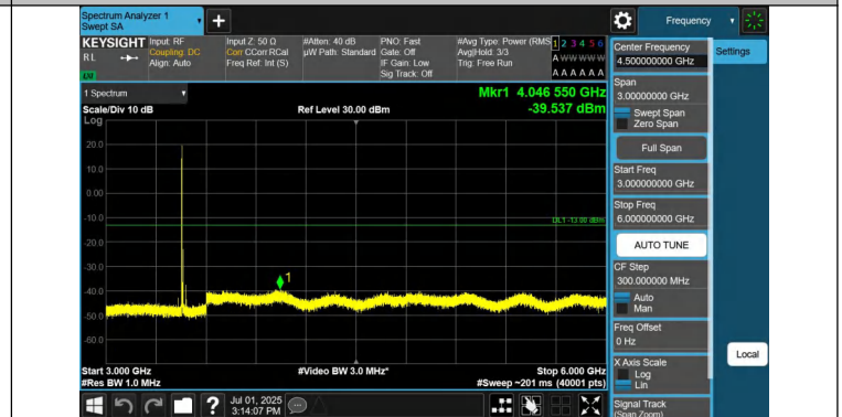
Band42(3450-3550)-20MHz-QPSK-42190-1RB#99-3000~6000-PA
