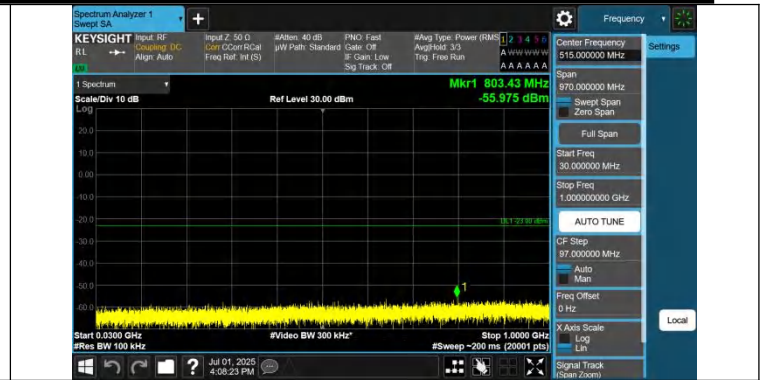
Band42(3450-3550)-20MHz-QPSK-42590-1RB#99-30~1000-PASS
