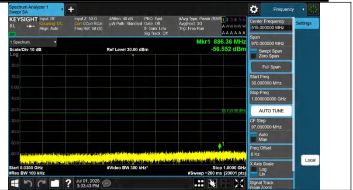
Band42(3450-3550)-10MHz-QPSK-42590-1RB#49-30~1000-PASS
