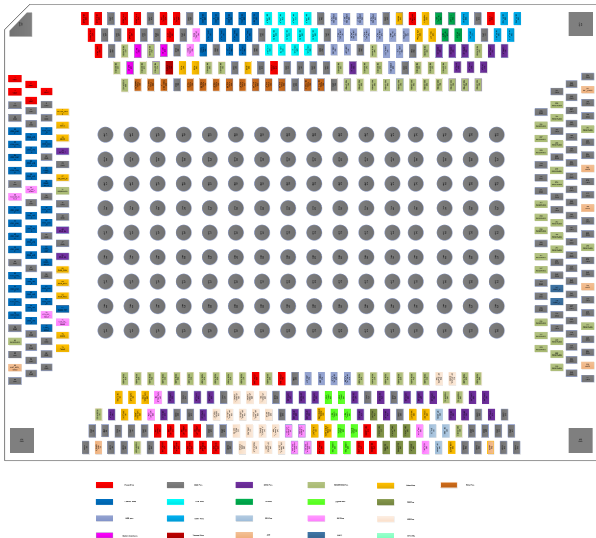
Figure 3: Pin Assignment
