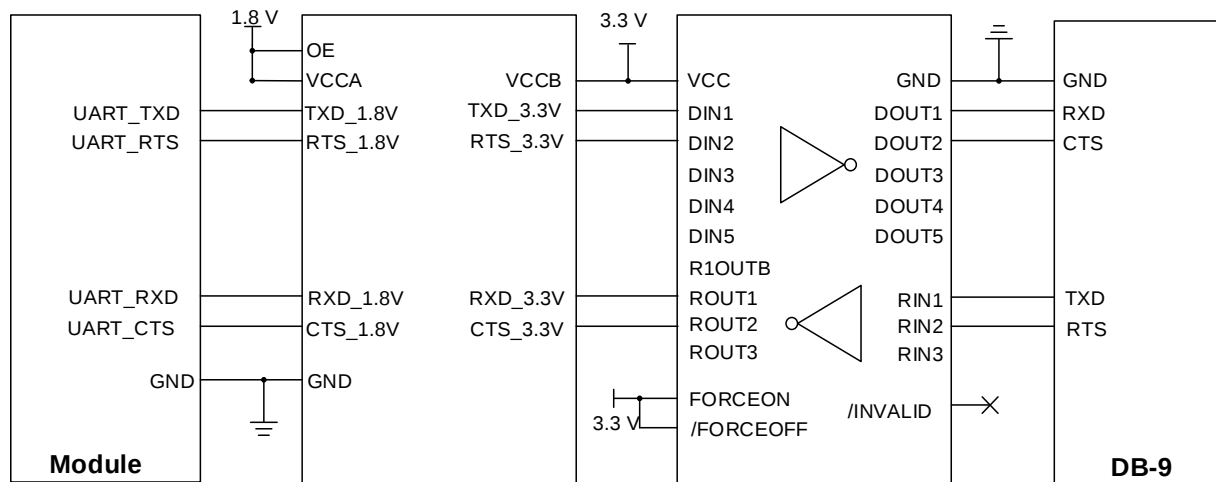
Figure 21: Reference Circuit with RS232 Level-Shifting Chip (for UART)
