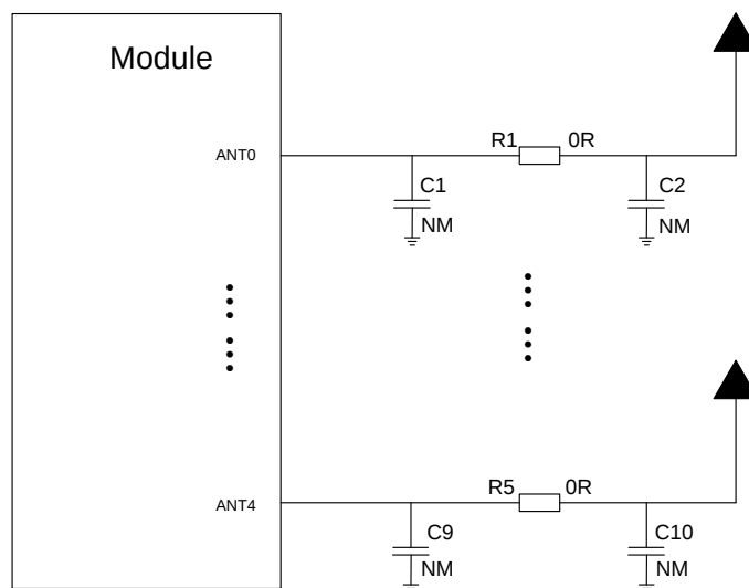
Figure 28: Reference Circuit for RF Antenna Interfaces
