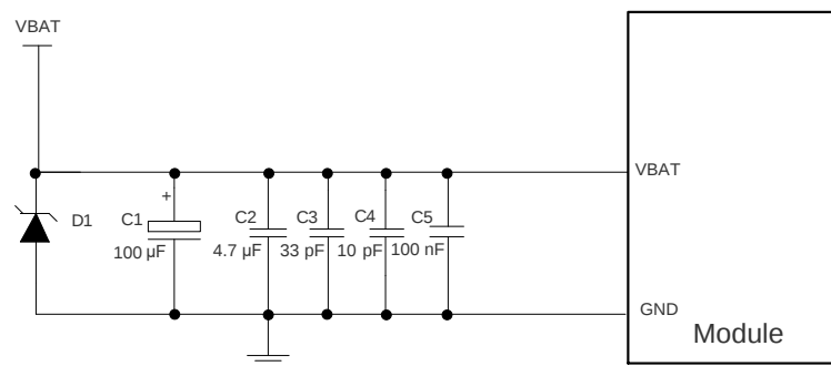
Figure 7: Structure of Power Supply
