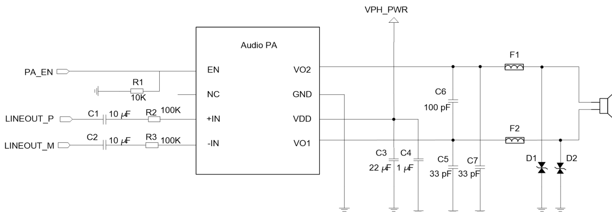
Figure 27: Reference Circuit Design for Lineout Interface
