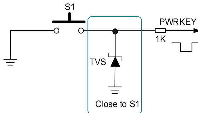
Figure 7: Turn On Module Using Button
