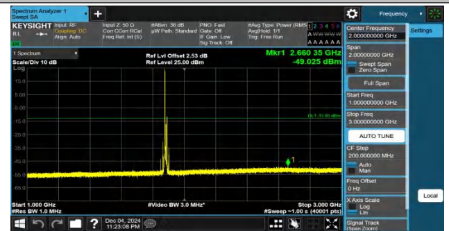
Band25-15MHz-QPSK-26365-1RB#0-1000~3000-PASS
