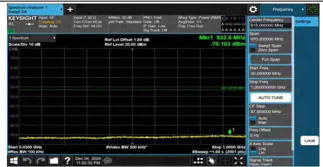
Band25-5MHz-QPSK-26065-1RB#24-30~1000-PASS
