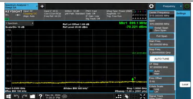
Band25-5MHz-QPSK-26665-1RB#24-30~1000-PASS
