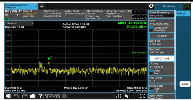
Band25-5MHz-QPSK-26065-1RB#24-0.009~0.15-PASS
