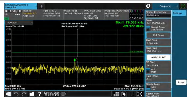
Band25-15MHz-QPSK-26365-1RB#74-0.009~0.15-PASS
