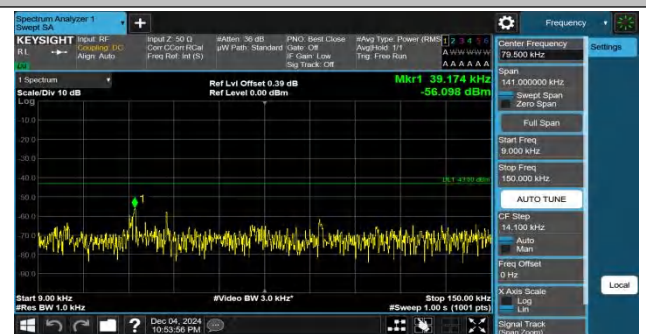
Band25-3MHz-QPSK-26365-1RB#14-0.009~0.15-PASS
