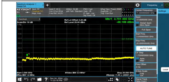
Band25-15MHz-QPSK-26365-1RB#0-3000~20000-PASS
