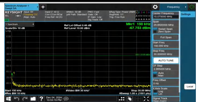
Band25-3MHz-QPSK-26365-1RB#0-0.15~30-PASS
