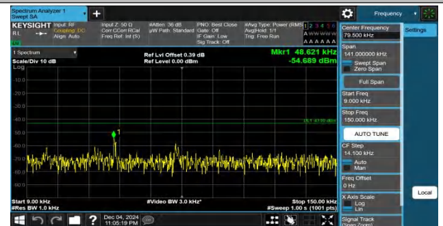
Band25-5MHz-QPSK-26665-1RB#24-0.009~0.15-PASS
