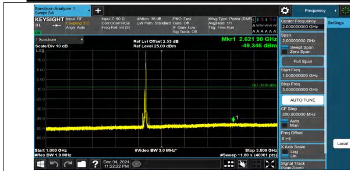
Band25-15MHz-QPSK-26115-1RB#74-1000~3000-PASS
