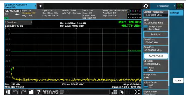
Band25-5MHz-QPSK-26365-1RB#0-0.15~30-PASS
