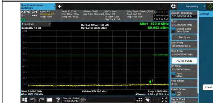
Band25-3MHz-QPSK-26365-1RB#0-30~1000-PASS
