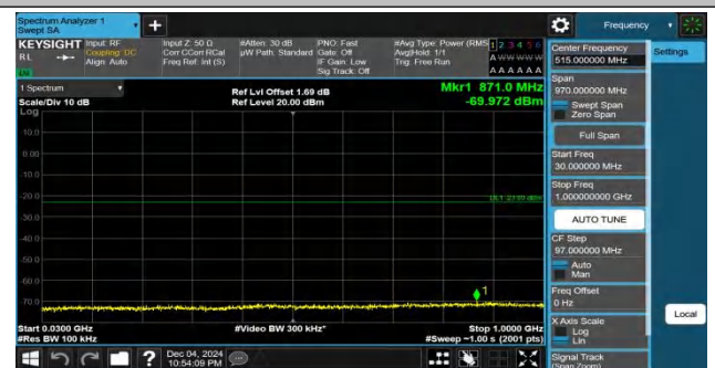
Band25-3MHz-QPSK-26365-1RB#14-30~1000-PASS
