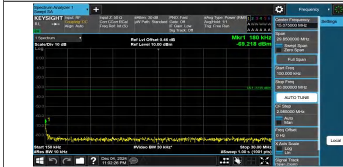
Band25-5MHz-QPSK-26065-1RB#24-0.15~30-PASS
