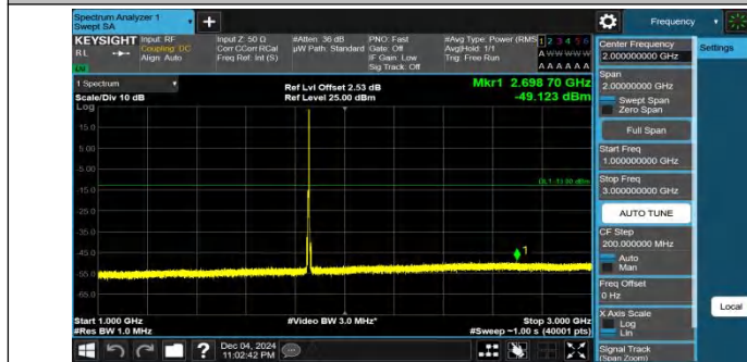
Band25-5MHz-QPSK-26065-1RB#24-1000~3000-PASS
