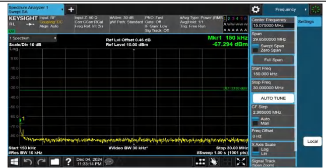
Band25-20MHz-QPSK-26590-1RB#0-0.15~30-PASS
