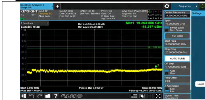
Band25-5MHz-QPSK-26065-1RB#0-3000~20000-PASS
