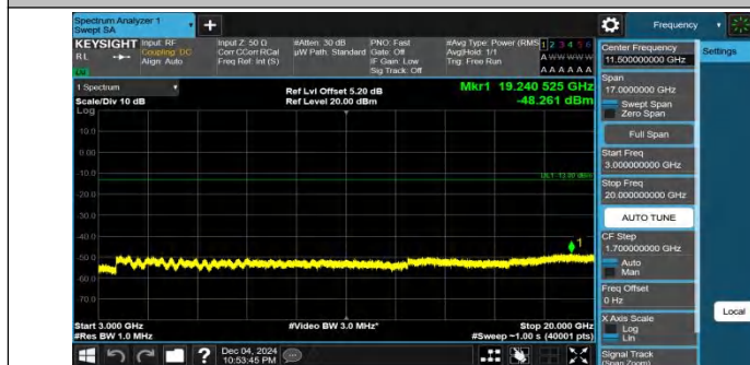
Band25-3MHz-QPSK-26365-1RB#0-3000~20000-PASS
