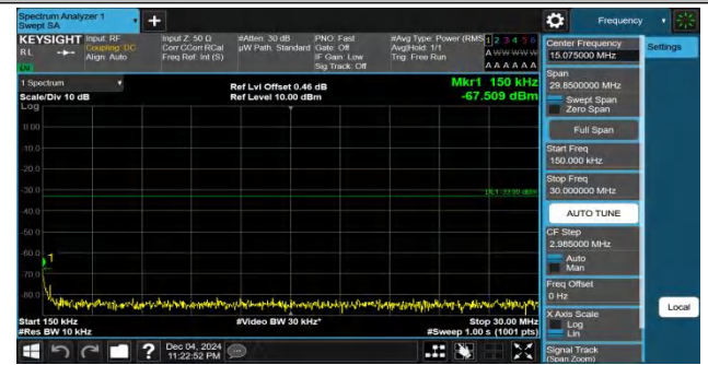
Band25-15MHz-QPSK-26365-1RB#0-0.15~30-PASS
