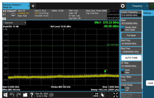
BLE_1M-Ant1-2440-30~1000-PASS
