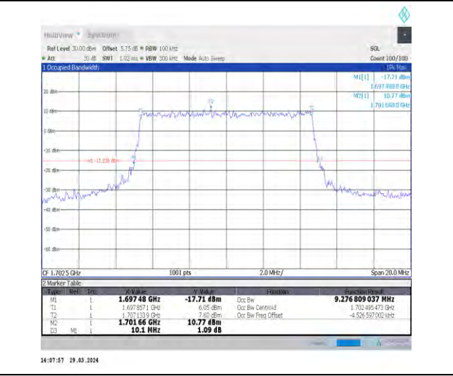
1-N70-15-10-M-7-CP-16QAM-Outer_Full-52@0-Ant1 -9.277-10.100-≤10-PASS
