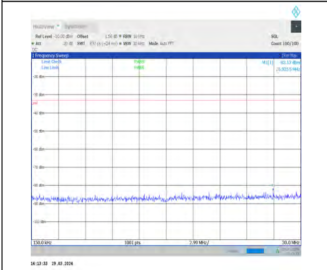
1-N70-15-15-M-1-DFT-PI2BPSK-Inner_1RB_Left-1 @1-0.15-30-Ant1-26.93--83.13--33-PASS
