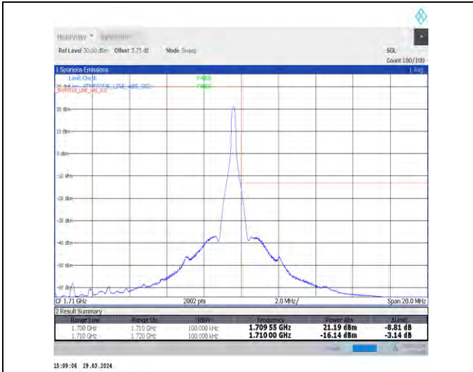
1-N70-15-10-H-2-DFT-PI2BPSK-Edge_1RB_Right-1@51-Ant1-1-seegraph-PASS-see graph
