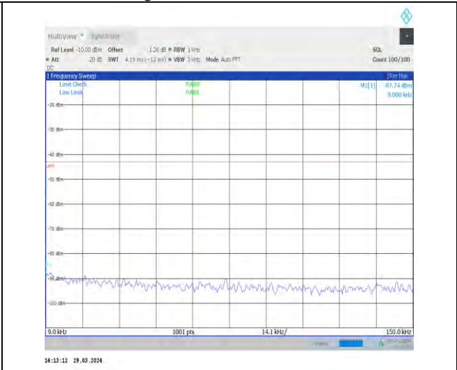
1-N70-15-15-M-1-DFT-PI2BPSK-Inner_1RB_Left-1@ 1-0.009-0.15-Ant1-0.01--87.74--43-PASS
