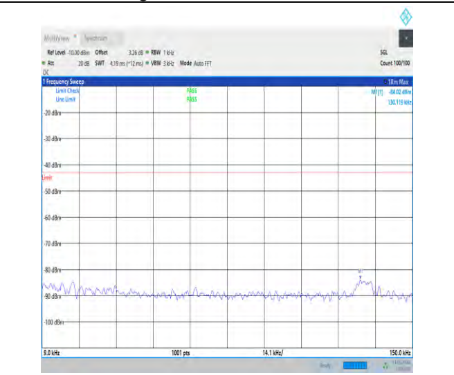
1-N70-15-15-M-1-DFT-PI2BPSK-Inner_1RB_Left-1 @1-0.009-0.15-Ant1-0.13--84.02--43-PASS
