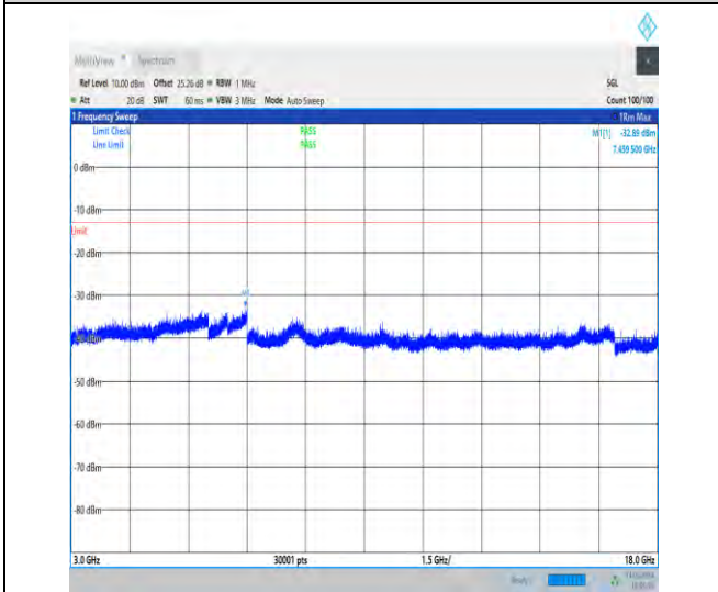
1-N70-15-15-H-1-DFT-PI2BPSK-Inner_1RB_Left-1@ 1-3000-18000-Ant1-7459.50--32.89--13-PASS
