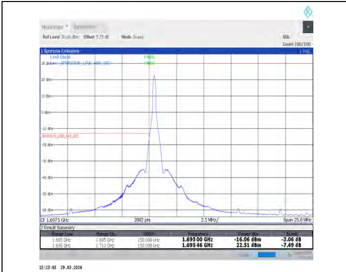
1-N70-15-15-L-1-DFT-PI2BPSK-Edge_1RB_Left-1@0-Ant1-1-seegraph-PASS-see graph
