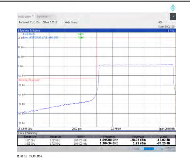
1-N70-15-10-L-6-CP-QPSK-Outer_Full-52@0-Ant1-1-seegraph-PASS-see graph
