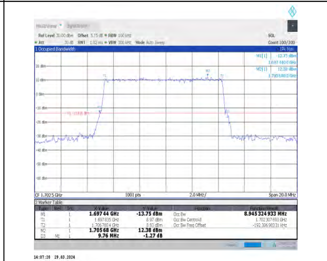
1-N70-15-10-M-3-DFT-16QAM-Outer_Full-50@0-Ant 1-8.945-9.760-≤10-PASS
