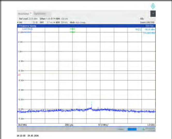
1-N70-15-15-M-1-DFT-PI2BPSK-Inner_1RB_Left-1@ 1-30-1000-Ant1-551.86--56.16--23-PASS
