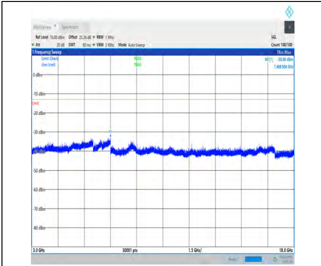
1-N70-15-15-L-1-DFT-PI2BPSK-Inner_1RB_Left-1@ 1-3000-18000-Ant1-7498.50--33.09--13-PASS
