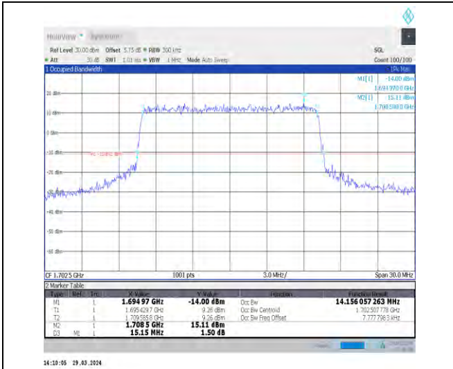
1-N70-15-15-M-7-CP-16QAM-Outer_Full-79@0-Ant 1-14.156-15.150≤15-PASS
