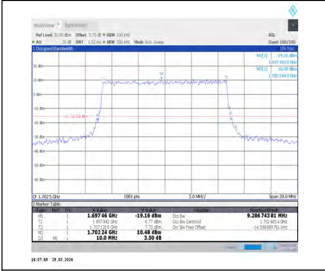
1-N70-15-10-M-6-CP-QPSK-Outer_Full-52@0-Ant1 9.287-10.000-≤10-PASS
