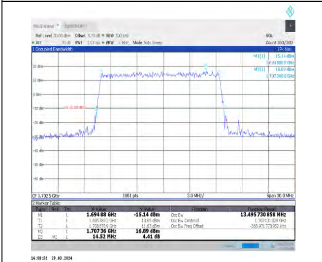
1-N70-15-15-M-1-DFT-QPSK-Outer_Full-75@0-Ant1 -13.496-14.520-≤15-PASS
