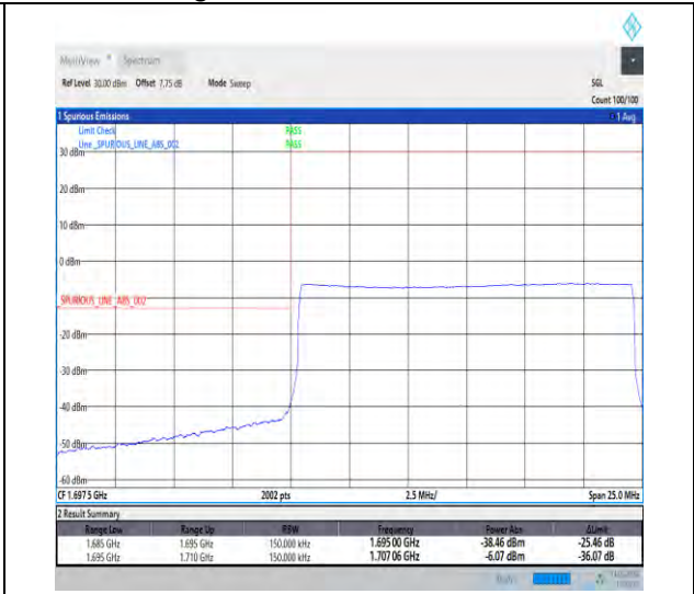
1-N70-15-15-L-6-CP-QPSK-Outer_Full-79@0-Ant1 1-1-seegraph-PASS-see graph
