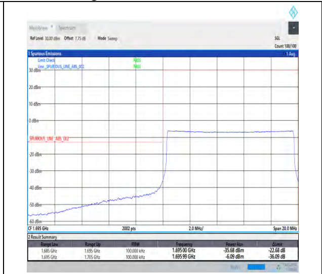
1-N70-15-10-L-6-CP-QPSK-Outer_Full-52@0-Ant1 1-1-seegraph-PASS-see graph
