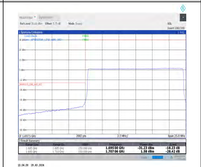
1-N70-15-15-L-6-CP-QPSK-Outer_Full-79@0-Ant1-1-seegraph-PASS-see graph
