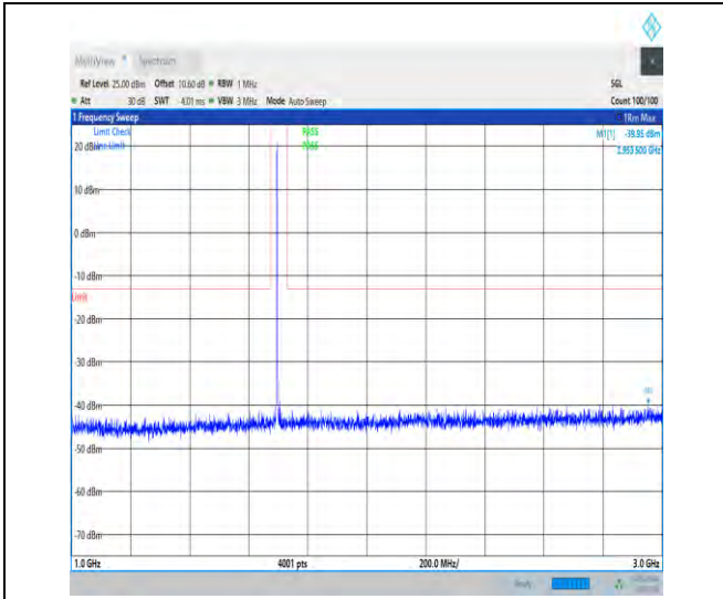
1-N70-15-15-M-1-DFT-PI2BPSK-Inner_1RB_Left-1 @1-1000-3000-Ant1-2953.50--39.95--13-PASS
