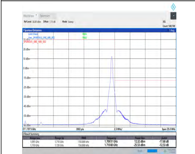
1-N70-15-15-H-5-CP-QPSK-Edge_1RB_Right-1@78-Ant1 -1-seegraph-PASS-see graph
