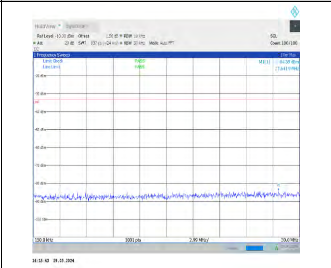
1-N70-15-15-H-1-DFT-PI2BPSK-Inner_1RB_Left-1 @ 1-0.15-30-Ant1-27.64--84.39--33-PASS
