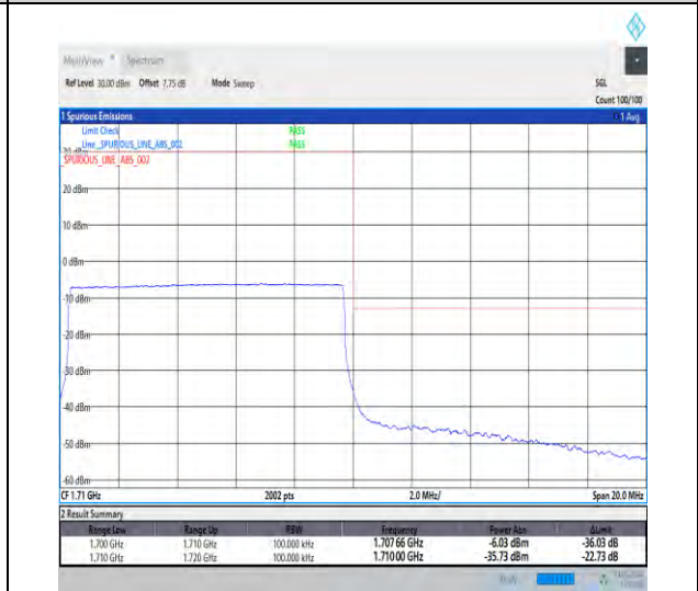
1-N70-15-10-H-6-CP-QPSK-Outer_Full-52@0-Ant1 1-1-seegraph-PASS-see graph
