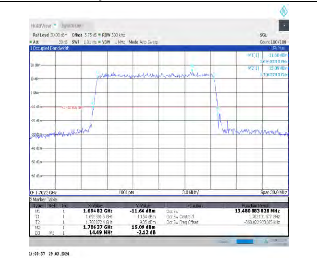
1-N70-15-15-M-4-DFT-64QAM-Outer_Full-75@0-Ant 1-13.481-14.490-≤15-PASS
