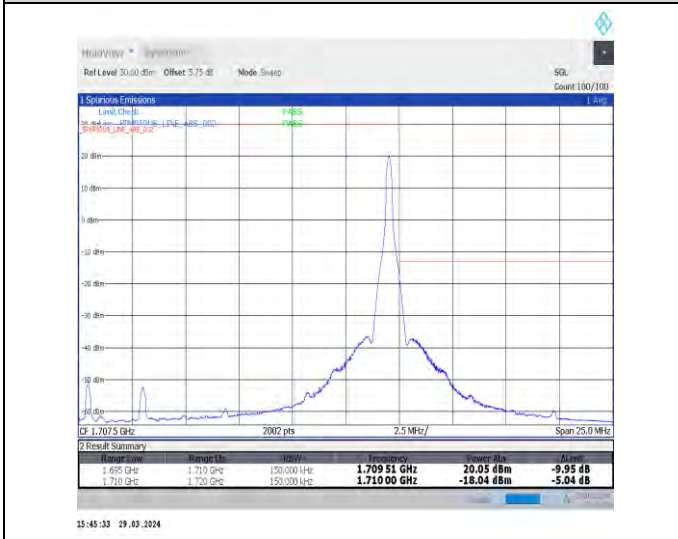
1-N70-15-15-H-5-CP-QPSK-Edge_1RB_Right-1@78-Ant1-1-seegraph-PASS-see graph
