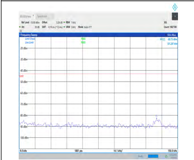
1-N70-15-15-H-1-DFT-PI2BPSK-Inner_1RB_Left-1@ 1-0.009-0.15-Ant1-0.13--83.75--43-PASS
