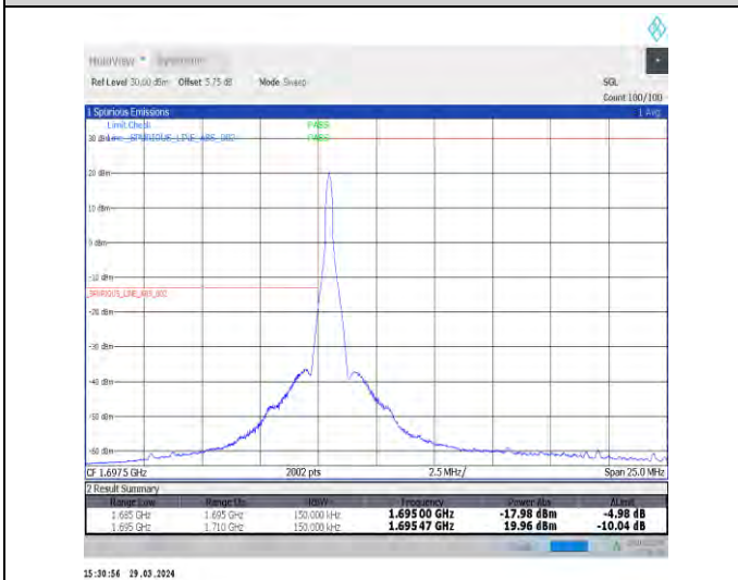
1-N70-15-15-L-4-CP-QPSK-Edge_1RB_Left-1@0-Ant1-1-seegraph-PASS-see graph
