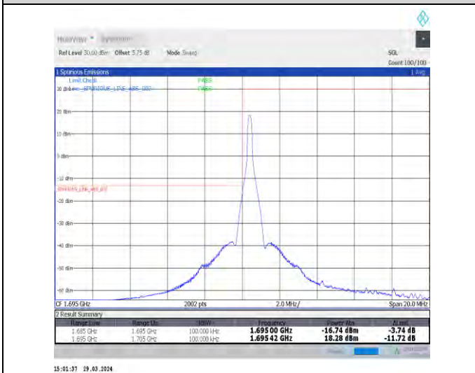
1-N70-15-10-L-4-CP-QPSK-Edge_1RB_Left-1@0-Ant1-1-seegraph-PASS-see graph
