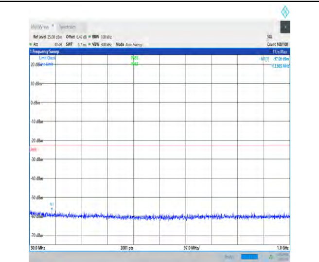
1-N70-15-15-M-1-DFT-PI2BPSK-Inner_1RB_Left-1 @1-30-1000-Ant1-112.94--57.06--23-PASS
