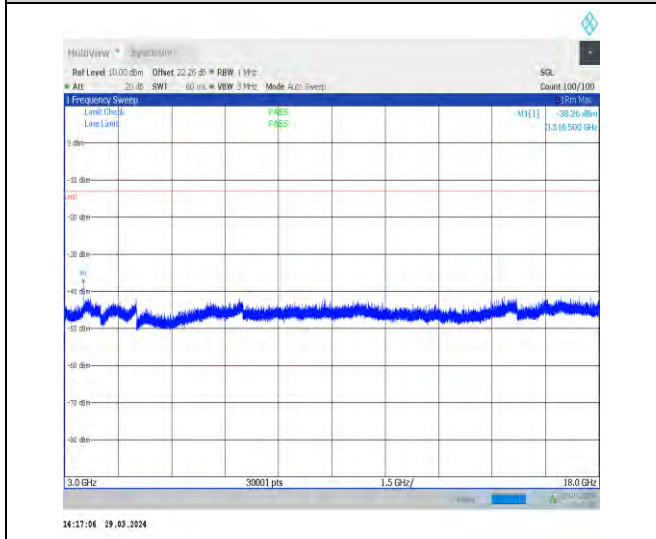
1-N70-15-15-H-1-DFT-PI2BPSK-Inner_1RB_Left-1 @1-3000-18000-Ant1-3516.50--38.26--13-PASS
