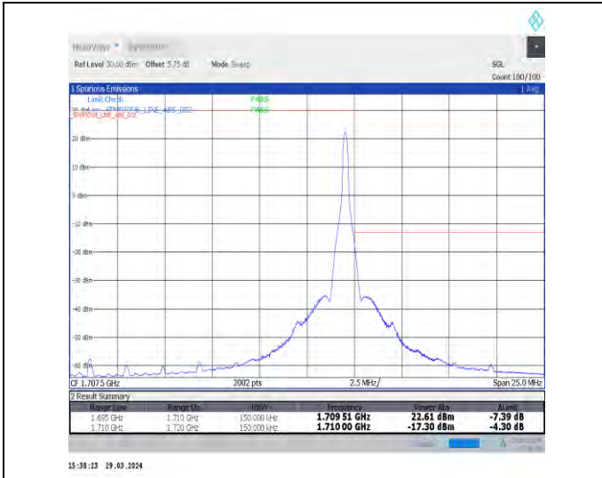
1-N70-15-15-H-2-DFT-PI2BPSK-Edge_1RB_Right-1@78-Ant1-1-seegraph-PASS-see graph
