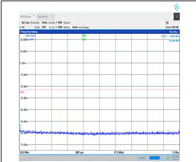
1-N70-15-15-H-1-DFT-PI2BPSK-Inner_1RB_Left-1@ 1-30-1000-Ant1-35.34--56.83--23-PASS
