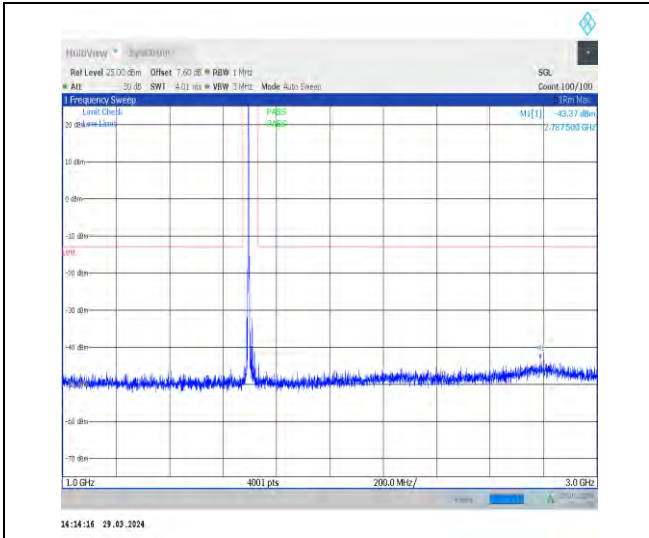
1-N70-15-15-M-1-DFT-PI2BPSK-Inner_1RB_Left-1 @1-1000-3000-Ant1-2787.50--43.37--13-PASS
