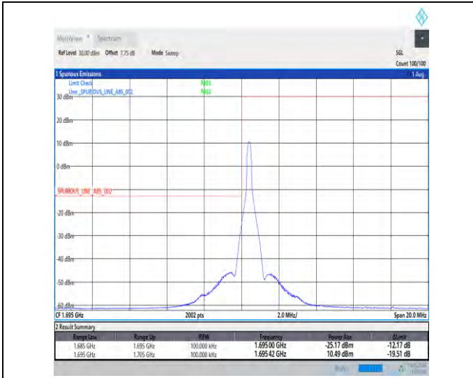
1-N70-15-10-L-4-CP-QPSK-Edge_1RB_Left-1@0-Ant1 -1-seegraph-PASS-see graph
