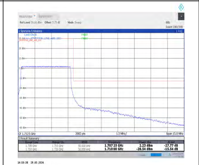
1-N70-15-5-H-6-CP-QPSK-Outer_Full-25@0-Ant1 -1-seegraph-PASS-see graph
