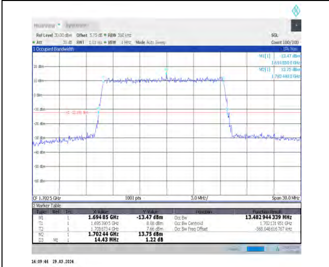
1-N70-15-15-M-5-DFT-256QAM-Outer_Full-75@0-Ant 1-13.483-14.430-≤15-PASS
