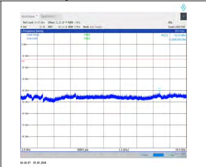
1-N70-15-15-M-1-DFT-PI2BPSK-Inner_1RB_Left-1 @ 1-3000-18000-Ant1-15568.50--41.59--13-PASS
