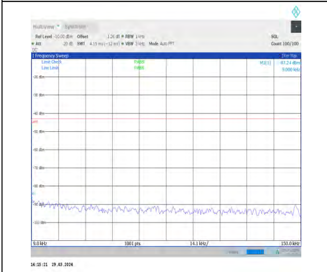
1-N70-15-15-H-1-DFT-PI2BPSK-Inner_1RB_Left-1 @1-0.009-0.15-Ant1-0.01--87.24--43-PASS
