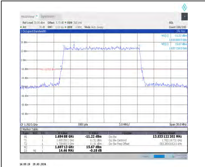
1-N70-15-15-M-3-DFT-16QAM-Outer_Full-75@0-Ant 1-13.533-14.460-≤15-PASS
