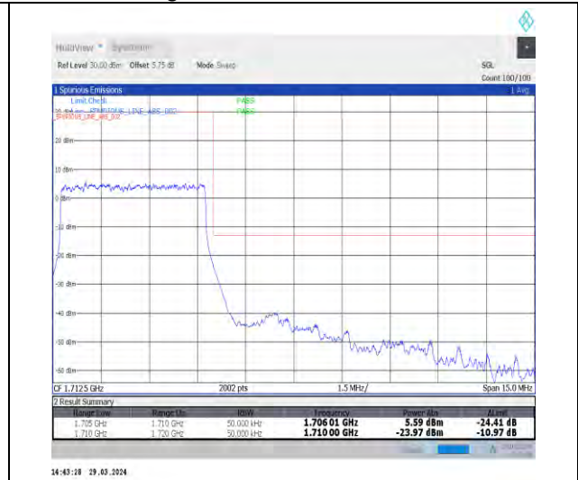
1-N70-15-5-H-3-DFT-PI2BPSK-Outer_Full-25@0-Ant1-1-seegraph-PASS-see graph
