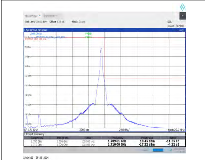
1-N70-15-10-H-5-CP-QPSK-Edge_1RB_Right-1@51-Ant1-1-seegraph-PASS-see graph
