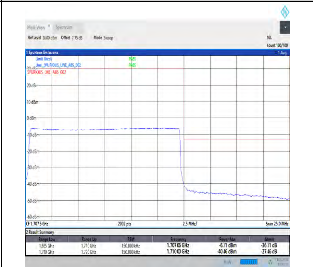
1-N70-15-15-H-6-CP-QPSK-Outer_Full-79@0-Ant1 1-1-seegraph-PASS-see graph
