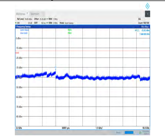
1-N70-15-15-M-1-DFT-PI2BPSK-Inner_1RB_Left-1 @1-3000-18000-Ant1-7484.00--32.92--13-PASS
