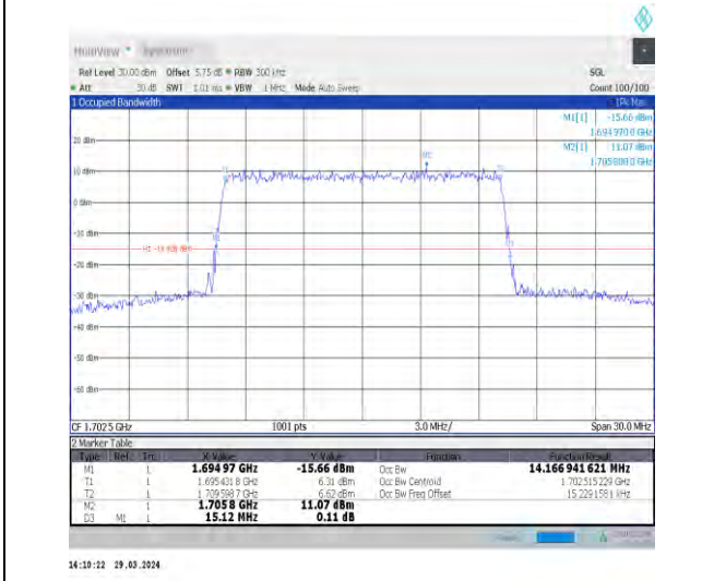
1-N70-15-15-M-9-CP-256QAM-Outer_Full-79@0-An t1-14.167-15.120≤15-PASS
