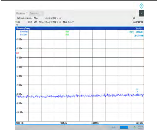
1-N70-15-15-M-1-DFT-PI2BPSK-Inner_1RB_Left-1 @1-0.15-30-Ant1-28.48--78.54--33-PASS
