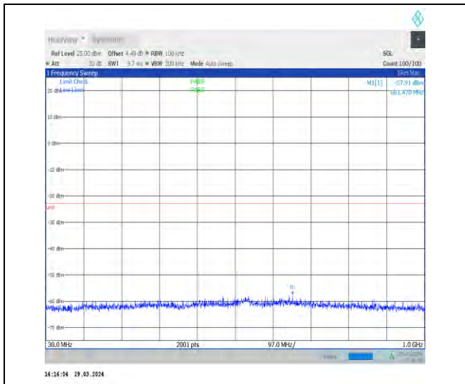
1-N70-15-15-H-1-DFT-PI2BPSK-Inner_1RB_Left-1 @1-30-1000-Ant1-661.47--57.91--23-PASS
