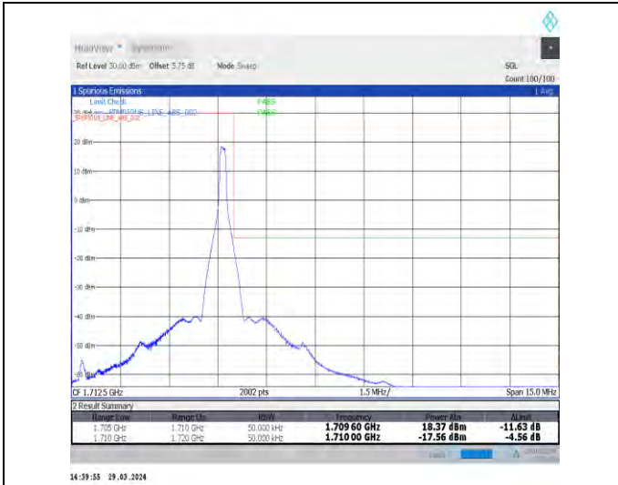
1-N70-15-5-H-2-DFT-PI2BPSK-Edge_1RB_Right-1@2 4-Ant1-1-seegraph-PASS-see graph
