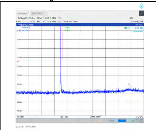
1-N70-15-15-H-1-DFT-PI2BPSK-Inner_1RB_Left-1@ 1-1000-3000-Ant1-2771.00--43.12--13-PASS
