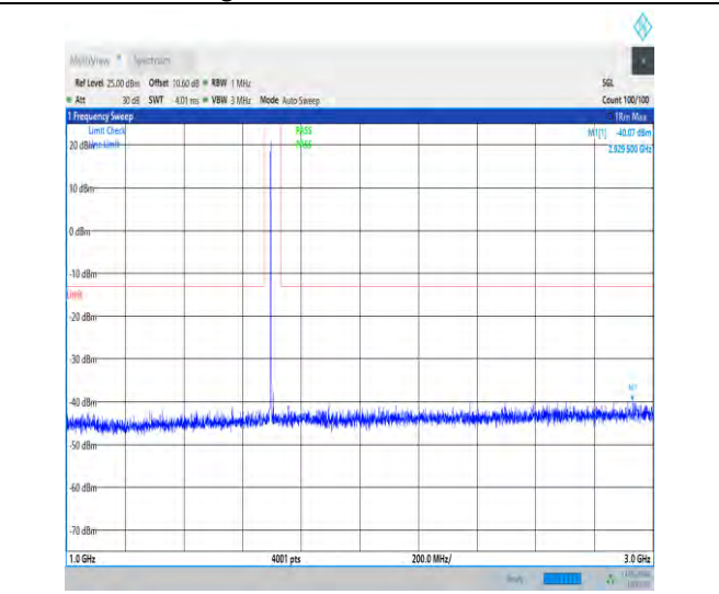
1-N70-15-15-H-1-DFT-PI2BPSK-Inner_1RB_Left-1@ 1-1000-3000-Ant1-2929.50--40.07--13-PASS
