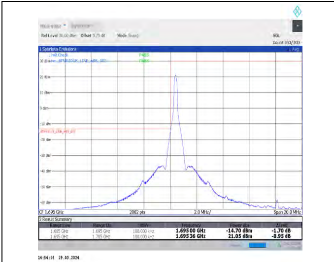
1-N70-15-10-L-1-DFT-PI2BPSK-Edge_1RB_Left-1@0-Ant1-1-seegraph-PASS-see graph
