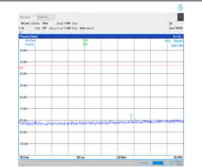
1-N70-15-15-H-1-DFT-PI2BPSK-Inner_1RB_Left-1@ 1-0.15-30-Ant1-20.51--78.64--33-PASS
