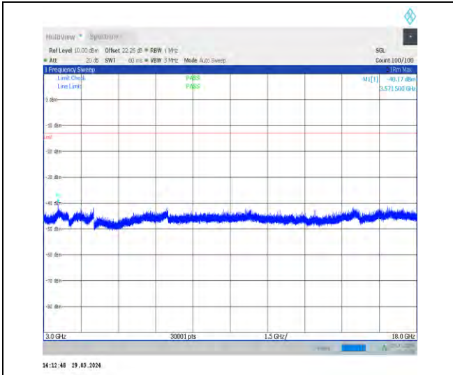
1-N70-15-15-L-1-DFT-PI2BPSK-Inner_1RB_Left-1@ 1-3000-18000-Ant1-3571.50--40.17--13-PASS
