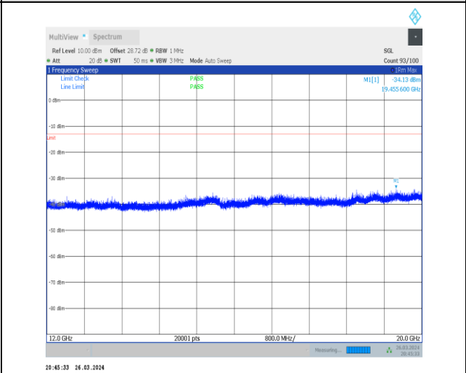
1-N13-15-10-H-1-DFT-PI2BPSK-Inner_1RB_Left-1 @ 1-12000-20000-Ant1-19455.60--34.13--13-PASS
