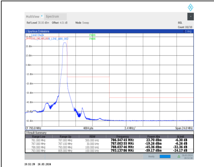
1-N13-15-5-H-2-DFT-PI2BPSK-Edge_1RB_Right-1@2 4-Ant1-1--PASS-see graph
