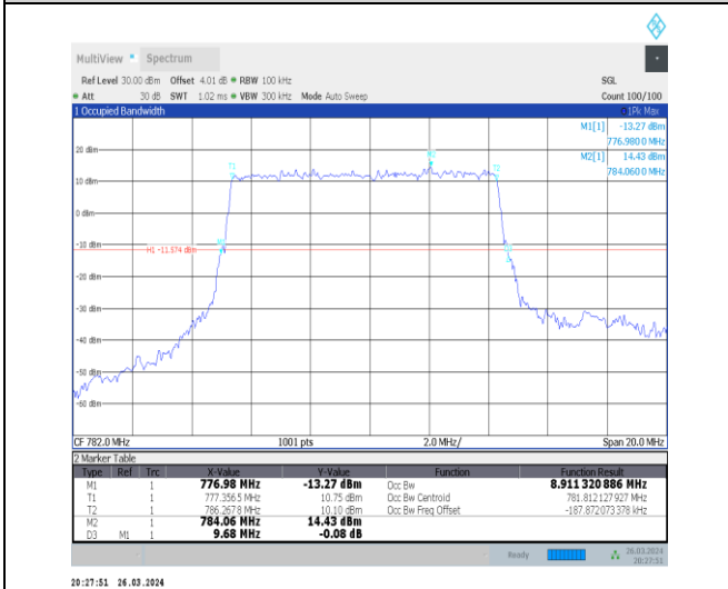
1-N13-15-10-M-2-DFT-16QAM-Outer_Full-50@0-Ant1 -8.911-9.680-≤10-PASS
