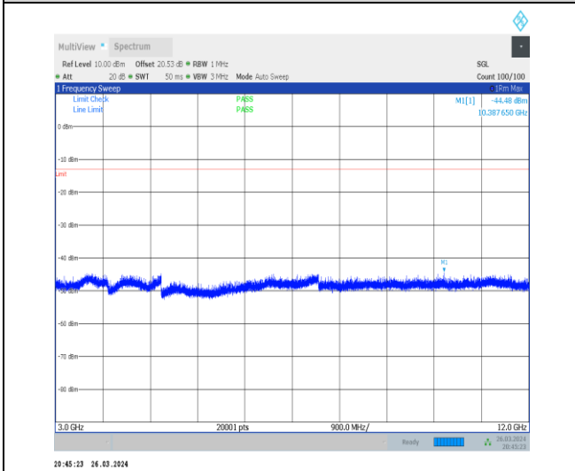
1-N13-15-10-H-1-DFT-PI2BPSK-Inner_1RB_Left-1 @ 1-3000-12000-Ant1-10387.65--44.48--13-PASS
