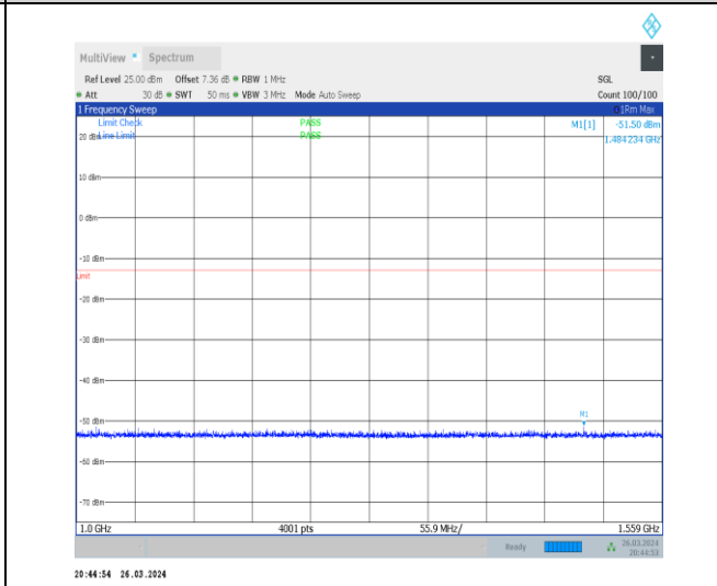
1-N13-15-10-H-1-DFT-PI2BPSK-Inner_1RB_Left-1 @ 1-1000-1559-Ant1-1484.23--51.50--13-PASS
