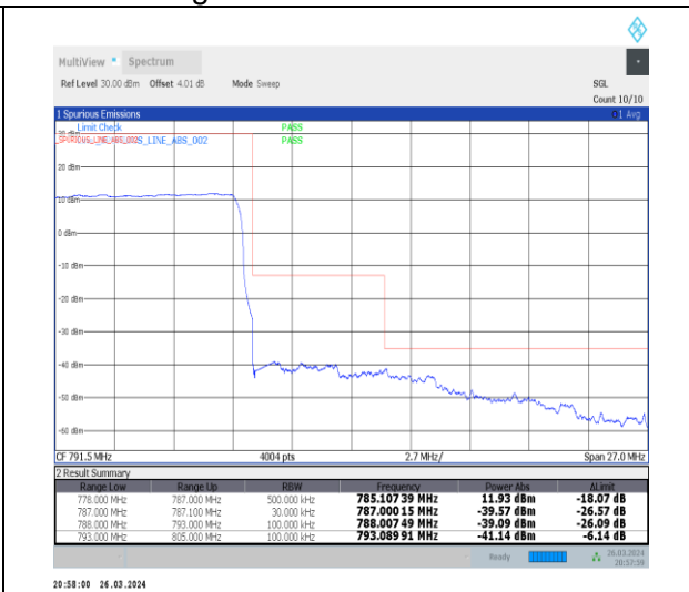
1-N13-15-10-H-3-DFT-PI2BPSK-Outer_Full-50@0-Ant1-1--PASS-see graph
