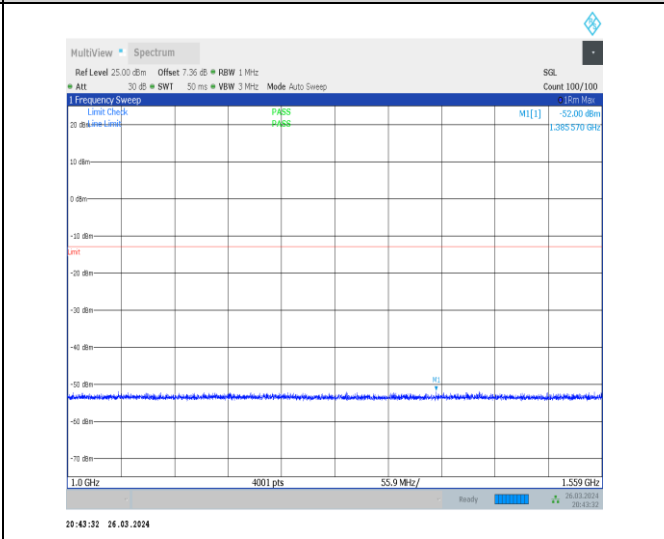
1-N13-15-10-M-1-DFT-PI2BPSK-Inner_1RB_Left-1 @ 1-1000-1559-Ant1-1385.57--52.00--13-PASS
