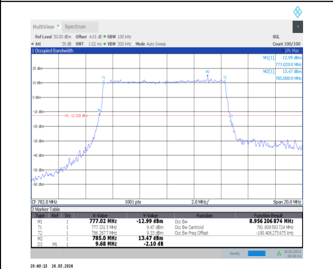
1-N13-15-10-M-3-DFT-16QAM-Outer_Full-50@0-Ant 1-8.956-9.680-≤10-PASS
