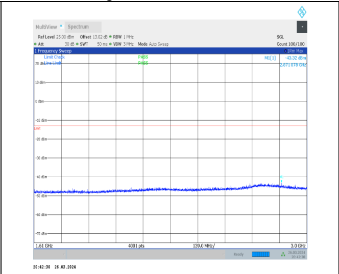
1-N13-15-10-L-1-DFT-PI2BPSK-Inner_1RB_Left-1 @ 1-1610-3000-Ant1-2871.08--43.32--13-PASS
