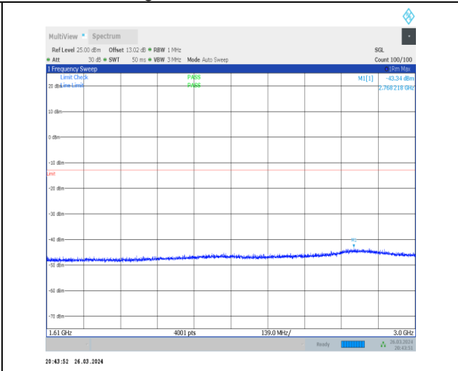
1-N13-15-10-M-1-DFT-PI2BPSK-Inner_1RB_Left-1 @ 1-1610-3000-Ant1-2768.22--43.34--13-PASS
