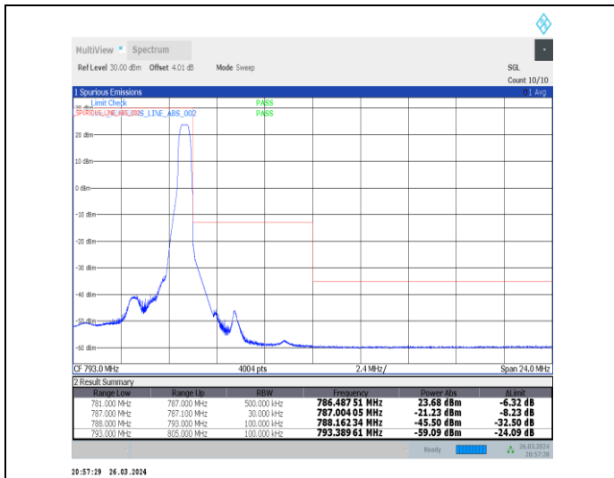
1-N13-15-10-H-2-DFT-PI2BPSK-Edge_1RB_Right-1@51-Ant1-1--PASS-see graph
