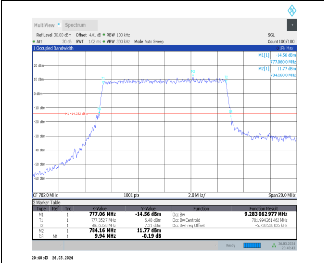
1-N13-15-10-M-6-CP-QPSK-Outer_Full-52@0-Ant1 9.283-9.940-≤10-PASS
