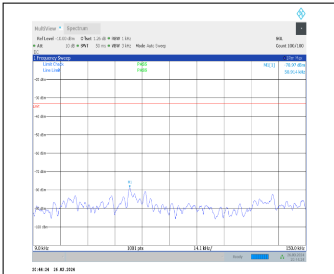
1-N13-15-10-H-1-DFT-PI2BPSK-Inner_1RB_Left-1 @ 1-0.009-0.15-Ant1-0.06--78.97--33-PASS
