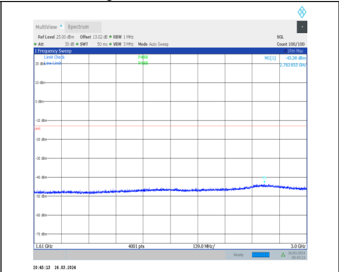
1-N13-15-10-H-1-DFT-PI2BPSK-Inner_1RB_Left-1 @ 1-1610-3000-Ant1-2783.86--43.38--13-PASS
