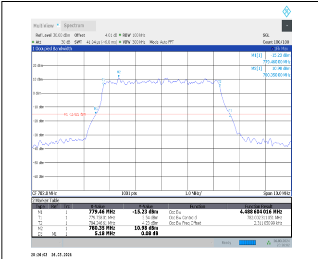
1-N13-15-5-M-9-CP-256QAM-Outer_Full-25@0-Ant1 -4.489-5.180-≤5-PASS
