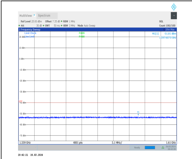
1-N13-15-10-L-1-DFT-PI2BPSK-Inner_1RB_Left-1 @ 1-1559-1610-Ant1-1597.61--51.81--40-PASS
