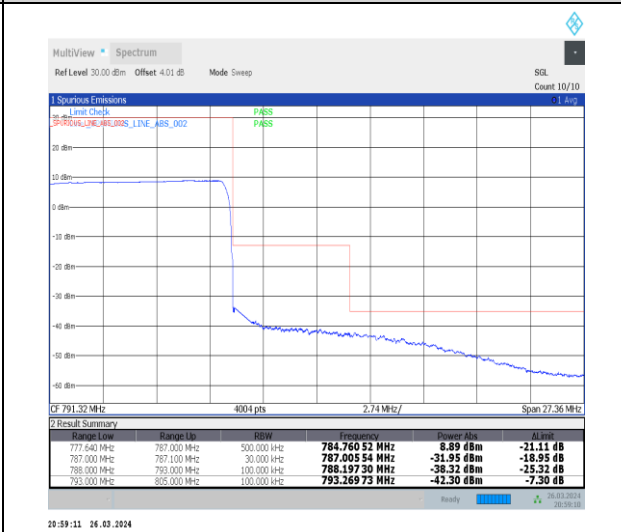
1-N13-15-10-H-6-CP-QPSK-Outer_Full-52@0-Ant1-1--PASS-see graph
