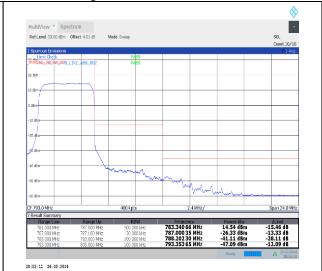
1-N13-15-5-H-3-DFT-PI2BPSK-Outer_Full-25@0- Ant1-1--PASS-see graph
