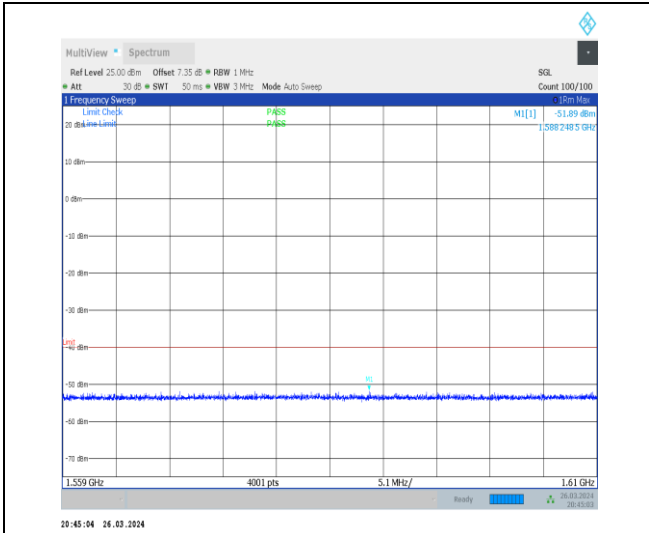
1-N13-15-10-H-1-DFT-PI2BPSK-Inner_1RB_Left-1 @ 1-1559-1610-Ant1-1588.25--51.89--40-PASS
