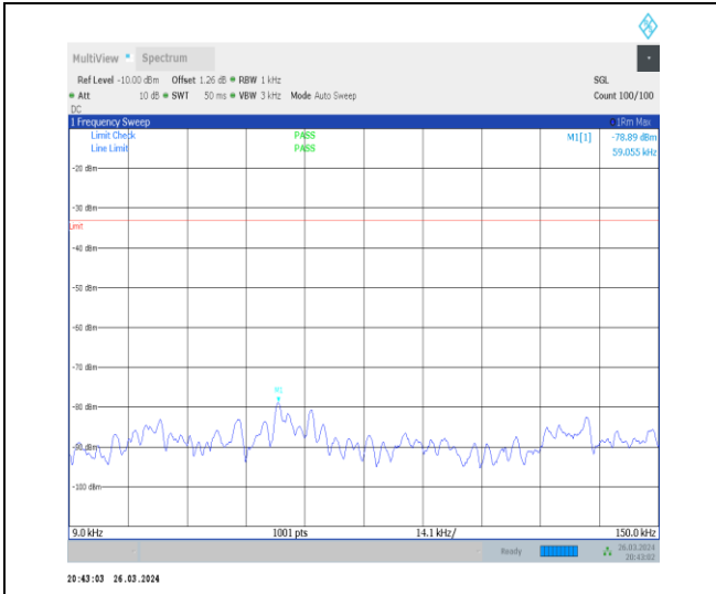
1-N13-15-10-M-1-DFT-PI2BPSK-Inner_1RB_Left-1 @ 1-0.009-0.15-Ant1-0.06--78.89--33-PASS
