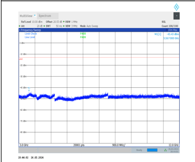
1-N13-15-10-M-1-DFT-PI2BPSK-Inner_1RB_Left-1 @ 1-3000-12000-Ant1-3567.00--43.43--13-PASS
