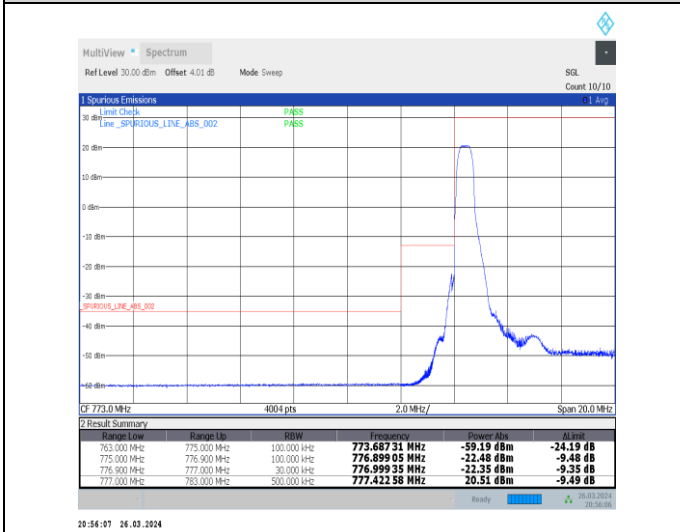
1-N13-15-10-L-4-CP-QPSK-Edge_1RB_Left-1@0-Ant1-1--PASS-see graph
