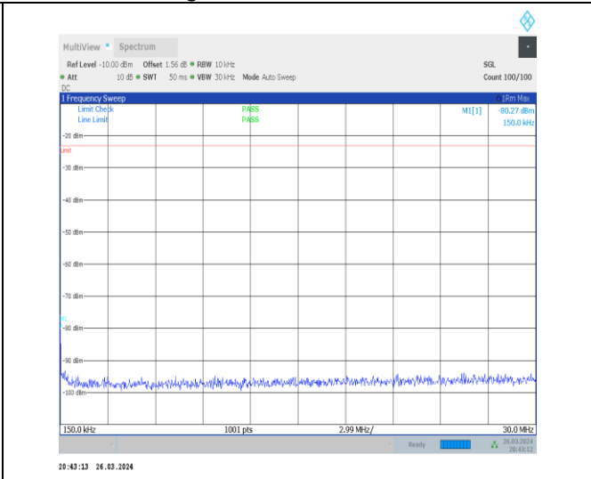
1-N13-15-10-M-1-DFT-PI2BPSK-Inner_1RB_Left-1 @ 1-0.15-30-Ant1-0.15--80.27--23-PASS
