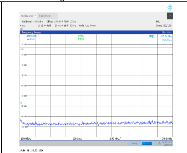
1-N13-15-10-H-1-DFT-PI2BPSK-Inner_1RB_Left-1 @ 1-0.15-30-Ant1-0.15--80.04--23-PASS
