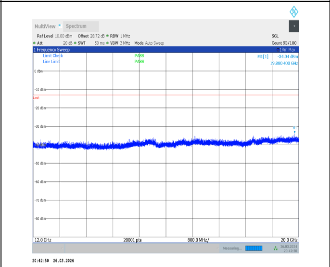
1-N13-15-10-L-1-DFT-PI2BPSK-Inner_1RB_Left-1 @ 1-12000-20000-Ant1-19880.40--34.04--13-PASS
