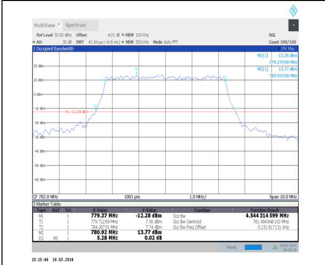
1-N13-15-5-M-7-CP-16QAM-Outer_Full-25@0-Ant1- 4.544-5.280-≤5-PASS
