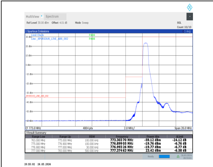
1-N13-15-10-L-1-DFT-PI2BPSK-Edge_1RB_Left-1@0-Ant1-1--PASS-see graph
