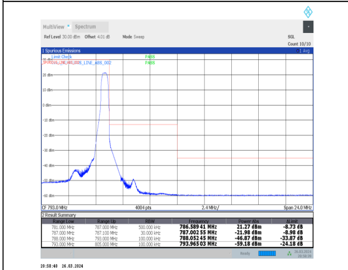
1-N13-15-10-H-5-CP-QPSK-Edge_1RB_Right-1@51-Ant1-1--PASS-see graph
