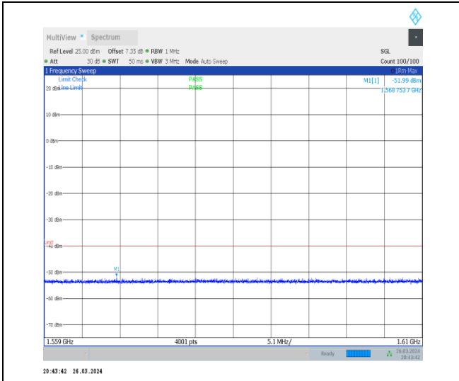
1-N13-15-10-M-1-DFT-PI2BPSK-Inner_1RB_Left-1 @ 1-1559-1610-Ant1-1568.75--51.99--40-PASS
