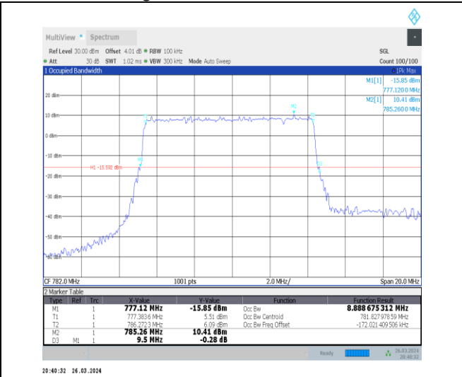
1-N13-15-10-M-5-DFT-256QAM-Outer_Full-50@0-A nt1-8.889-9.500-≤10-PASS
