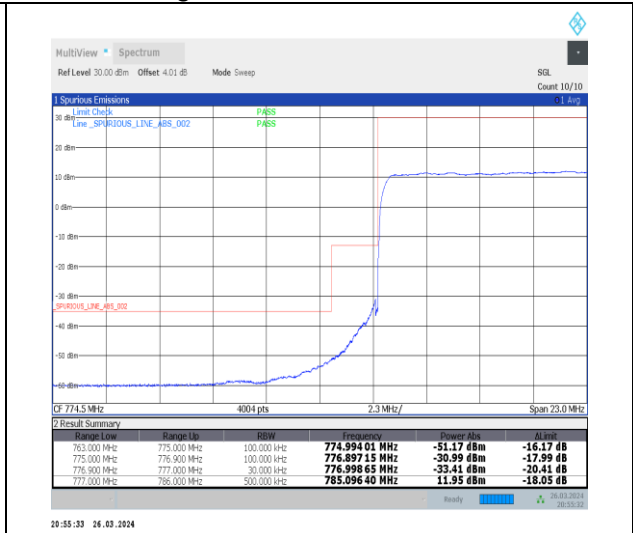
1-N13-15-10-L-3-DFT-PI2BPSK-Outer_Full-50@0-Ant1-1--PASS-see graph
