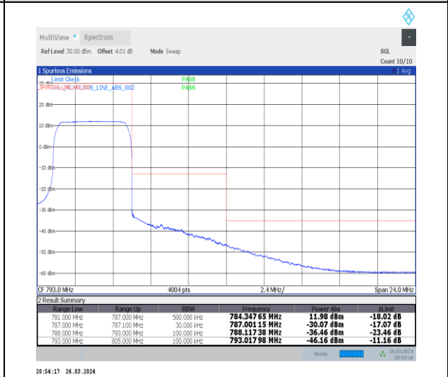
1-N13-15-5-H-6-CP-QPSK-Outer_Full-25@0-Ant1 -1--PASS-see graph
