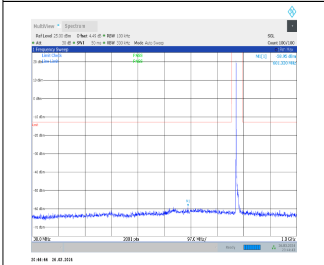
1-N13-15-10-H-1-DFT-PI2BPSK-Inner_1RB_Left-1 @ 1-30-1000-Ant1-601.33--58.95--13-PASS
