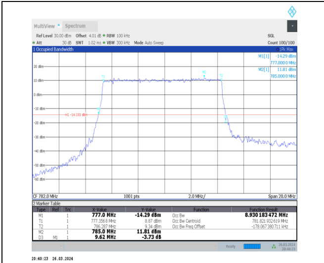
1-N13-15-10-M-4-DFT-64QAM-Outer_Full-50@0-Ant 1-8.93-9.620-≤10-PASS
