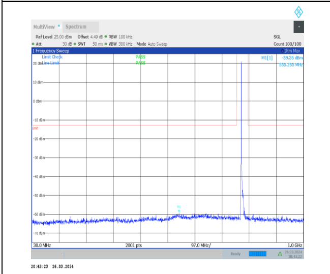
1-N13-15-10-M-1-DFT-PI2BPSK-Inner_1RB_Left-1 @ 1-30-1000-Ant1-555.26--59.35--13-PASS
