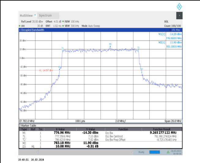
1-N13-15-10-M-7-CP-16QAM-Outer_Full-52@0-Ant1 -9.265-10.080-≤10-PASS
