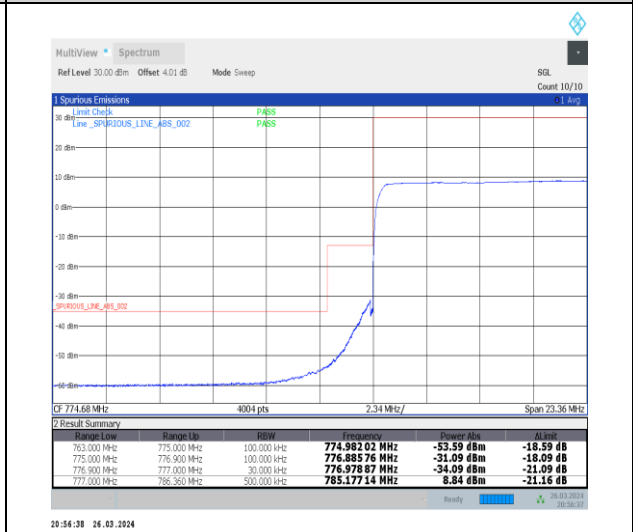
1-N13-15-10-L-6-CP-QPSK-Outer_Full-52@0-Ant1-1--PASS-see graph
