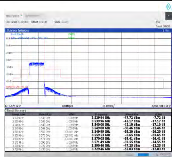
1-N48-30-20-L-3-DFT-PI2BPSK-Outer_Full-50@0-Ant1-1--PASS-see graph
