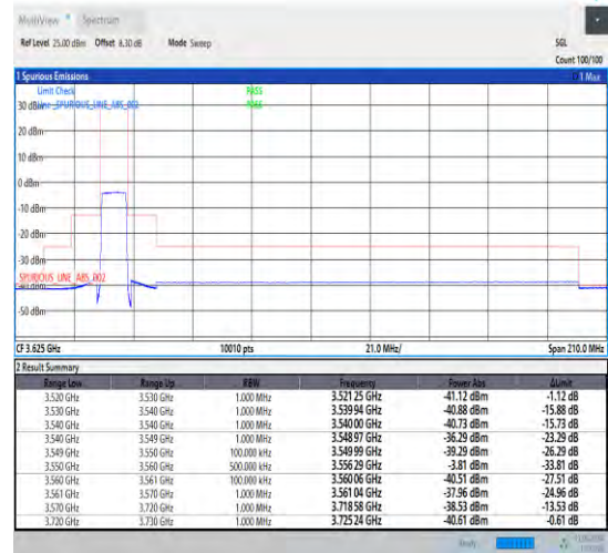
1-N48-30-10-L-3-CP-QPSK-Outer_Full-24@0-Ant1 -1--PASS-see graph
