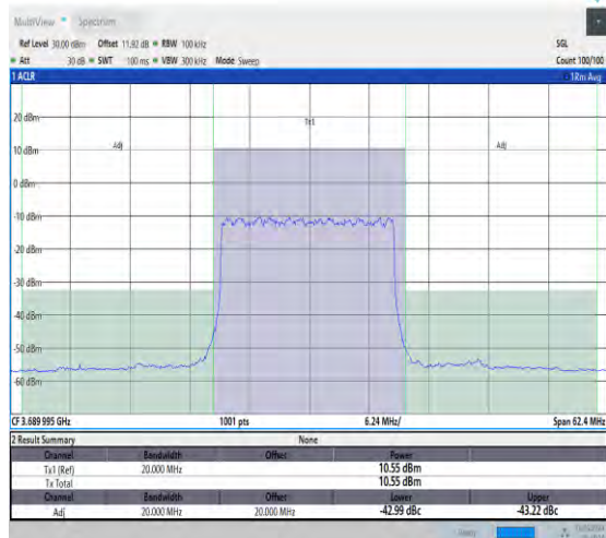
NTNV_N48_30_20_H_TID1_#1_-20_20
