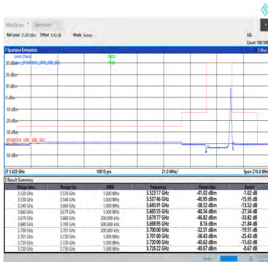
1-N48-30-20-H-2-CP-QPSK-Edge_1RB_Right-1@50-Ant1 -1--PASS-see graph
