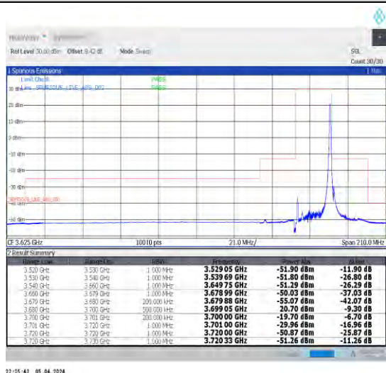
1-N48-30-20-H-5-CP-QPSK-Edge_1RB_Right-1@50-Ant1-1--PASS-see graph
