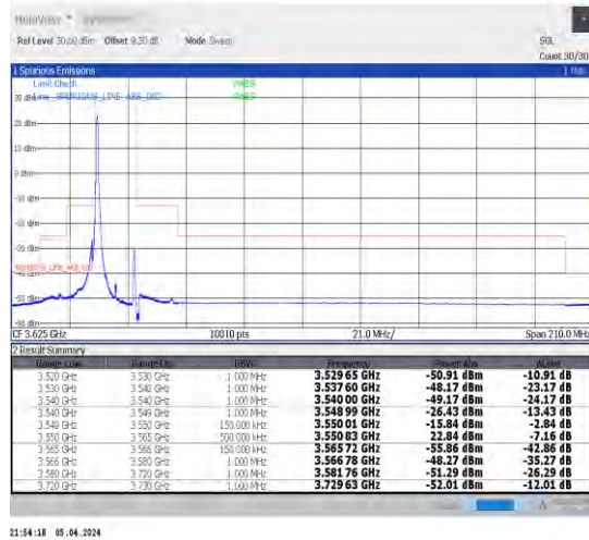
1-N48-30-15-L-1-DFT-PI2BPSK-Edge_1RB_Left-1@0-Ant1-1--PASS-see graph
