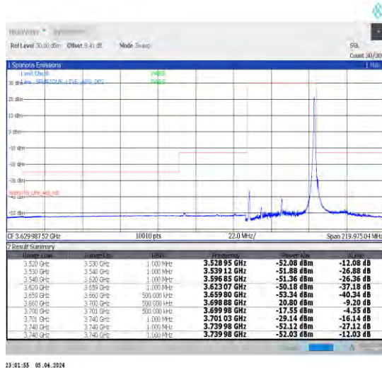
1-N48-30-40-H-5-CP-QPSK-Edge_1RB_Right-1@105-Ant1-1--PASS-see graph
