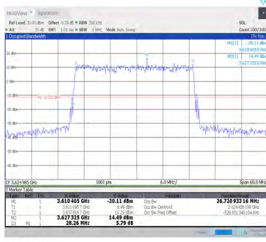
1-N48-30-30-M-1-DFT-QPSK-Outer_Full-75@0-Ant1 -26.721-28.260-≤30-PASS
