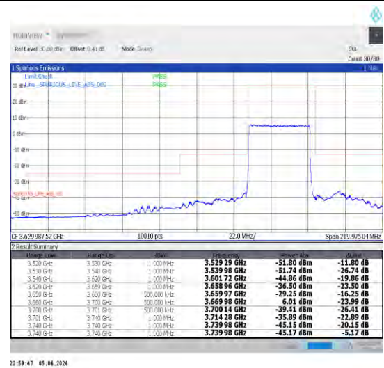
1-N48-30-40-H-3-DFT-PI2BPSK-Outer_Full-100@0-Ant1-1--PASS-see graph
