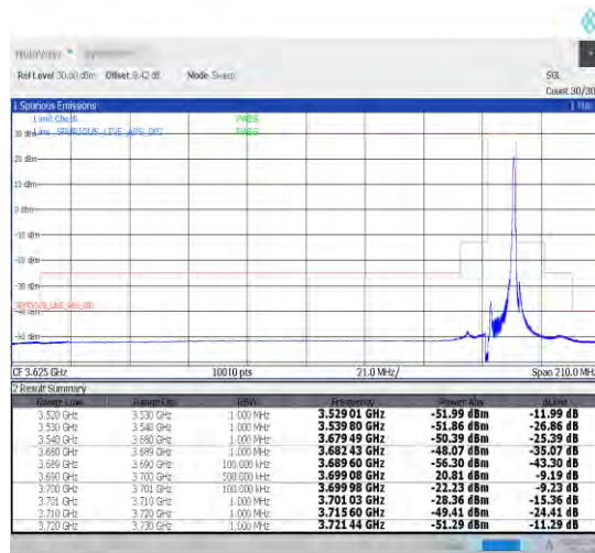
1-N48-30-10-H-2-DFT-PI2BPSK-Edge_1RB_Right-1@23-Ant1-1--PASS-see graph
