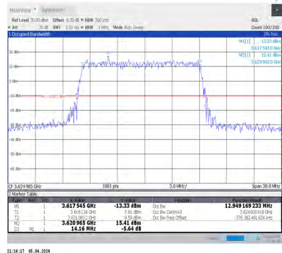
1-N48-30-15-M-3-DFT-16QAM-Outer_Full-36@0-Ant 1-12.949-14.160-<15-PASS
