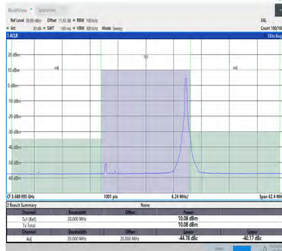
NTNV_N48_30_20_H_TID3_#1_-20_20
