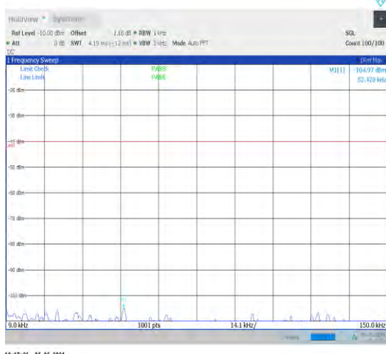
1-N48-30-40-H-1-DFT-PI2BPSK-Inner_1RB_Left-1@ 1-0.009-0.15-Ant1-0.05--104.97--40-PASS
