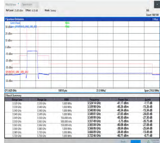
1-N48-30-15-L-3-CP-QPSK-Outer_Full-38@0-Ant1 -1--PASS-see graph
