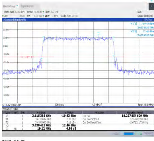
1-N48-30-20-M-7-CP-16QAM-Outer_Full-51@0-Ant 1-18.228-19.120-≤20-PASS
