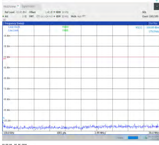
1-N48-30-40-M-1-DFT-PI2BPSK-Inner_1RB_Left-1 @1-0.15-30-Ant1-0.30--100.80--40-PASS
