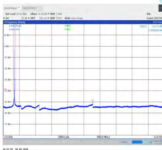
1-N48-30-40-M-1-DFT-PI2BPSK-Inner_1RB_Left-1 @1-3000-12000-Ant1-7998.60--51.73--40-PASS
