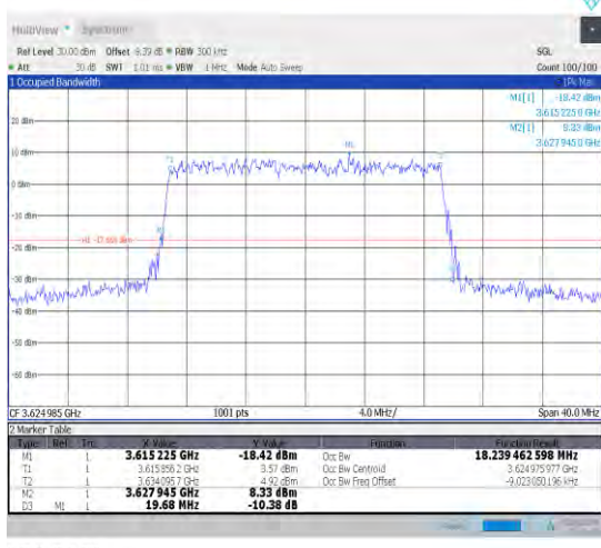
1-N48-30-20-M-9-CP-256QAM-Outer_Full-51@0-An t1-18.239-19.680-≤20-PASS
