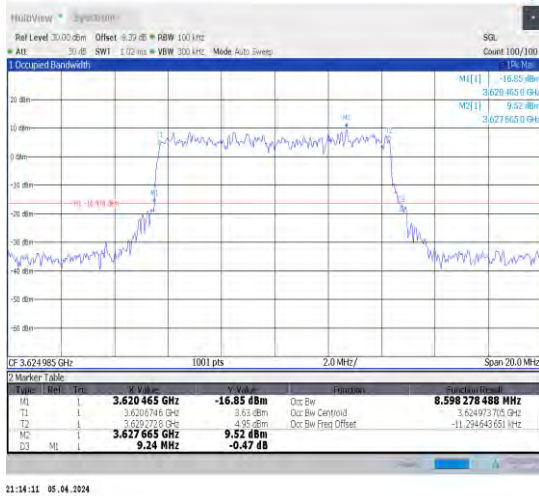
1-N48-30-10-M-5-DFT-256QAM-Outer_Full-24@0-A nt1-8.598-9.240-≤10-PASS
