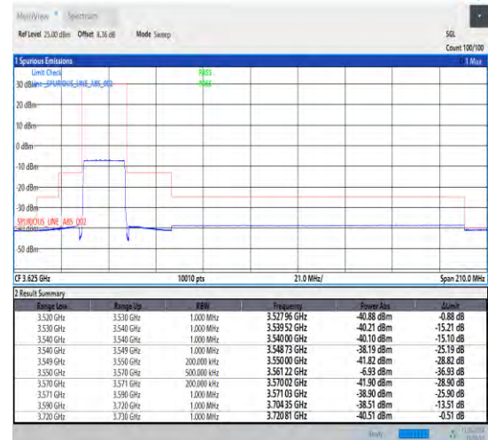
1-N48-30-20-L-3-CP-QPSK-Outer_Full-51@0-Ant1 1-1--PASS-see graph
