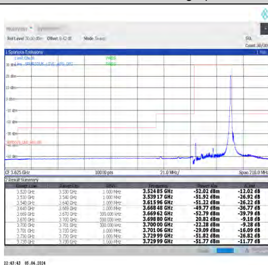
1-N48-30-30-H-5-CP-QPSK-Edge_1RB_Right-1@77-Ant1-1--PASS-see graph
