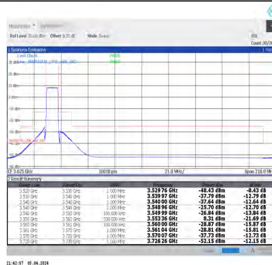
1-N48-30-10-L-6-CP-QPSK-Outer_Full-24@0-Ant1-1--PASS-see graph
