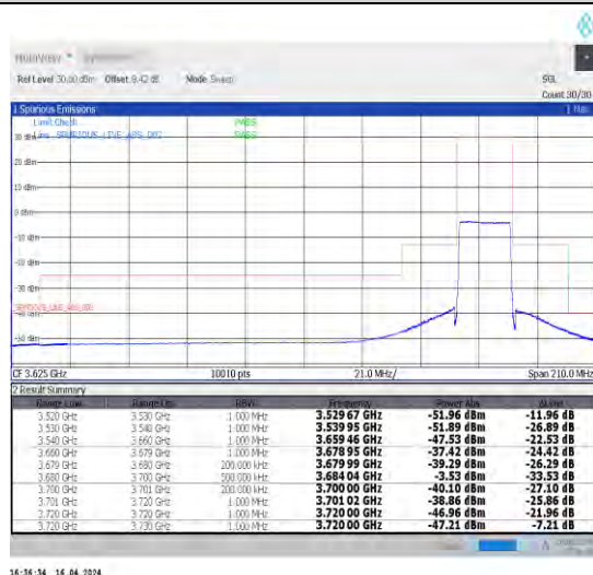
1-N48-30-20-H-6-CP-QPSK-Outer_Full-51@0-Ant1-1--PASS-see graph
