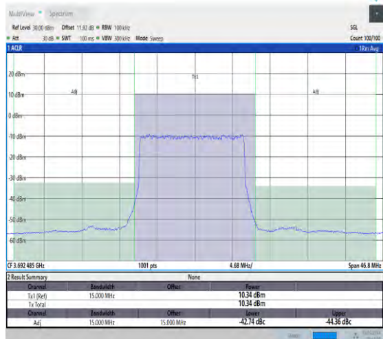
NTNV_N48_30_15_H_TID1_#1_-15_15
