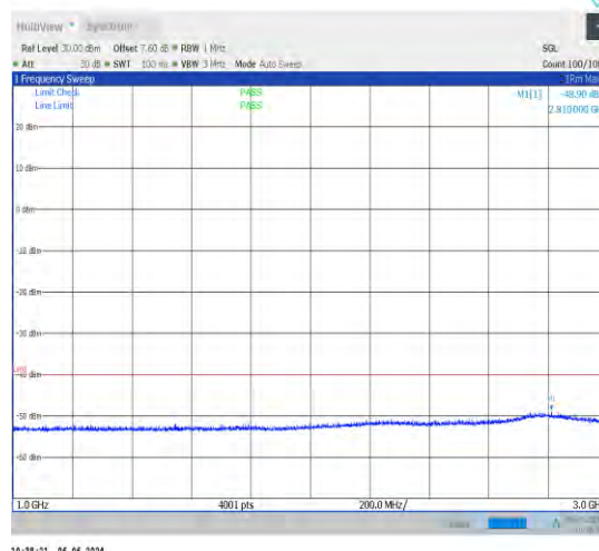
1-N48-30-40-H-1-DFT-PI2BPSK-Inner_1RB_Left-1@ 1-1000-3000-Ant1-2724.50--48.90--40-PASS
