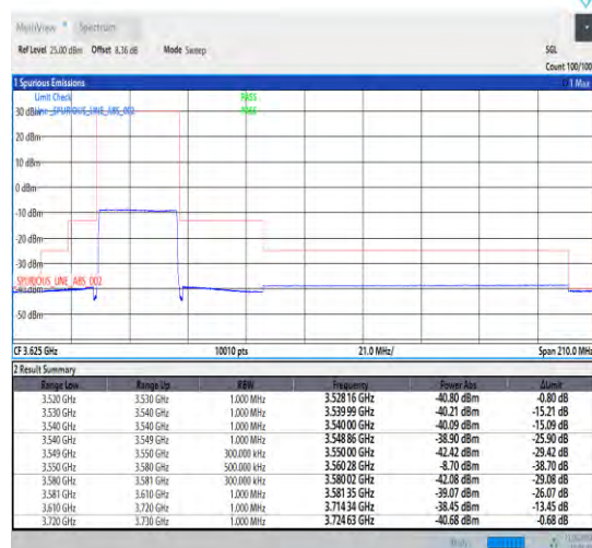
1-N48-30-30-L-3-CP-QPSK-Outer_Full-78@0-Ant1 1-1--PASS-see graph
