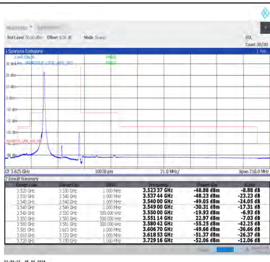
1-N48-30-30-L-1-DFT-PI2BPSK-Edge_1RB_Left-1@0-Ant1-1--PASS-see graph
