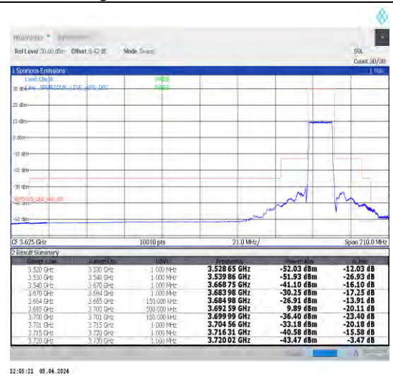
1-N48-30-15-H-3-DFT-PI2BPSK-Outer_Full-36@0-Ant1-1--PASS-see graph
