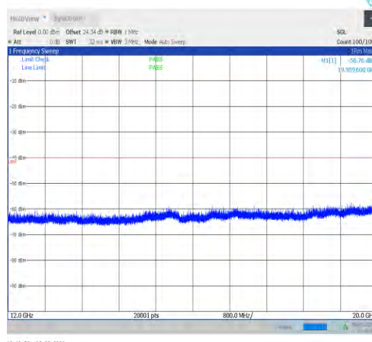
1-N48-30-40-H-1-DFT-PI2BPSK-Inner_1RB_Left-1@ 1-12000-20000-Ant1-19959.60--56.76--40-PASS
