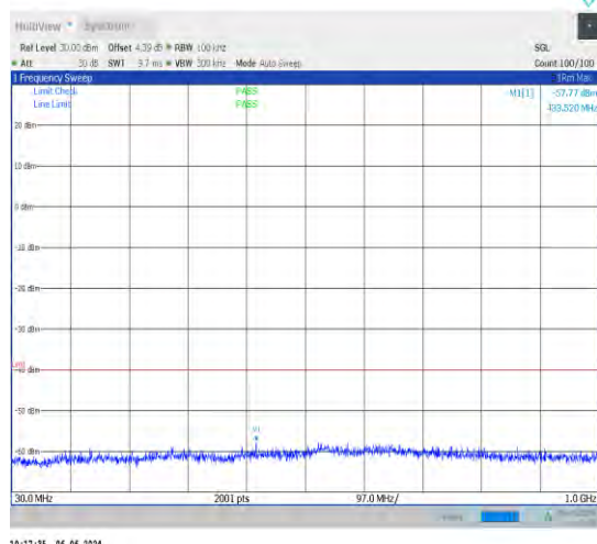
1-N48-30-40-H-1-DFT-PI2BPSK-Inner_1RB_Left-1@ 1-30-1000-Ant1-433.52--57.77--40-PASS
