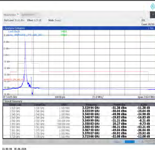
1-N48-30-10-L-4-CP-QPSK-Edge_1RB_Left-1@0-Ant1-1--PASS-see graph
