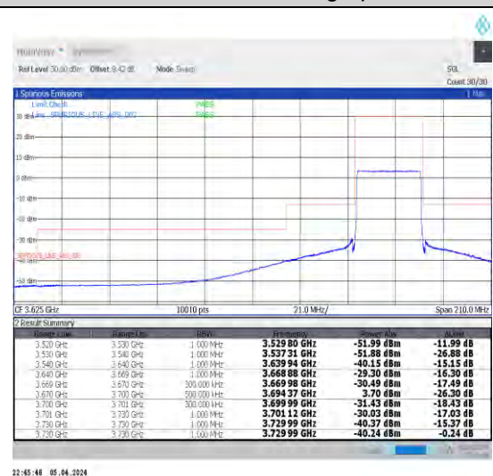
1-N48-30-30-H-6-CP-QPSK-Outer_Full-78@0-Ant1-1--PASS-see graph
