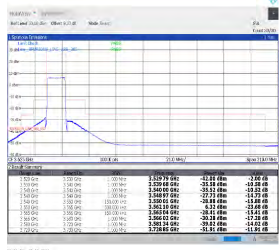
1-N48-30-15-L-6-CP-QPSK-Outer_Full-38@0-Ant1-1--PASS-see graph
