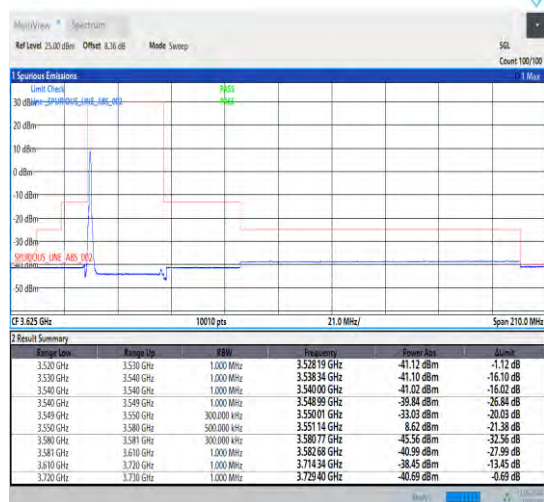
1-N48-30-30-L-1-CP-QPSK-Edge_1RB_Left-1@0-Ant1 -1--PASS-see graph
