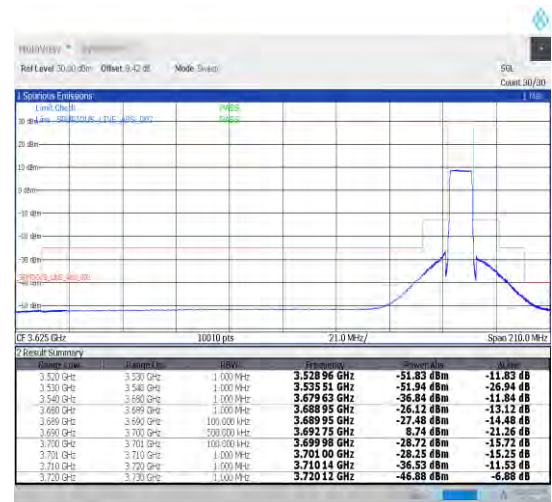
1-N48-30-10-H-3-DFT-PI2BPSK-Outer_Full-24@0-Ant1-1--PASS-see graph
