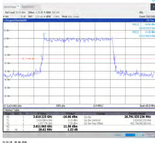
1-N48-30-30-M-3-DFT-16QAM-Outer_Full-75@0-Ant 1-26.793-28.620-≤30-PASS
