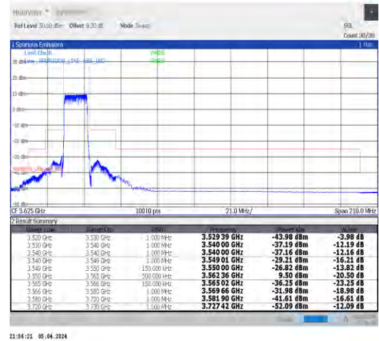
1-N48-30-15-L-3-DFT-PI2BPSK-Outer_Full-36@0-Ant1-1--PASS-see graph
