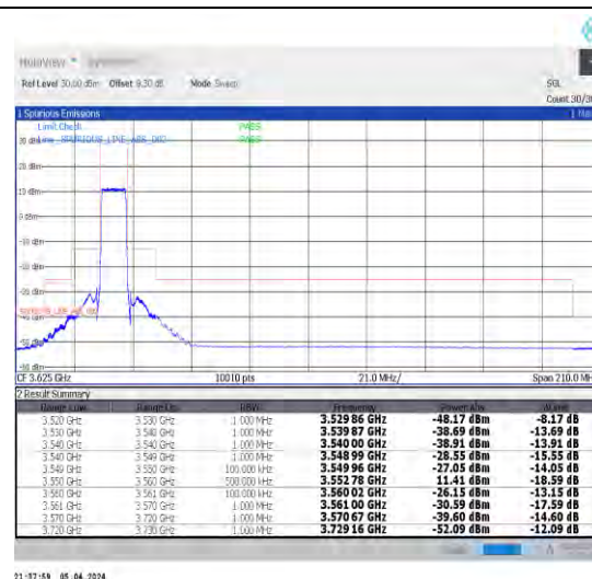
1-N48-30-10-L-3-DFT-PI2BPSK-Outer_Full-24@0-Ant1-1--PASS-see graph
