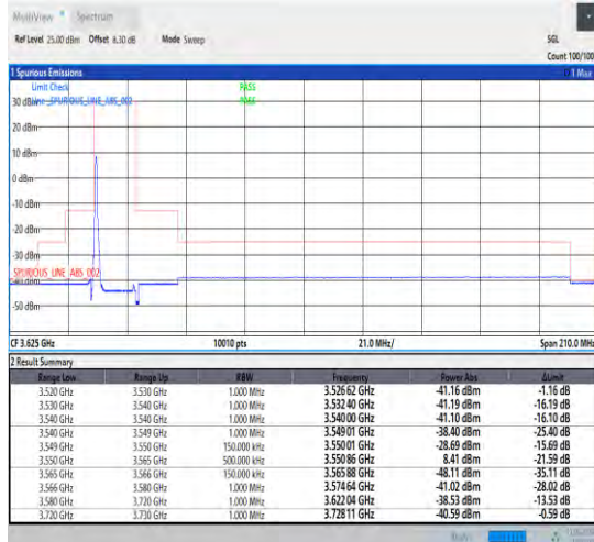
1-N48-30-15-L-1-CP-QPSK-Edge_1RB_Left-1@0-Ant1 -1--PASS-see graph
