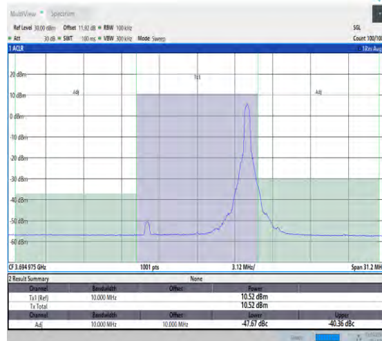
NTNV_N48_30_10_H_TID3_#1_-10_10
