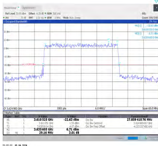
1-N48-30-30-M-9-CP-256QAM-Outer_Full-78@0-Ant1-27.859-29.160-≤30-PASS
