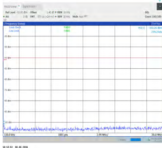
1-N48-30-40-M-1-DFT-PI2BPSK-Inner_1RB_Left-1 @1-0.15-30-Ant1-0.30--102.26--40-PASS
