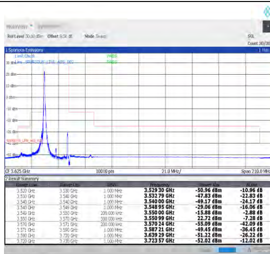
1-N48-30-20-L-1-DFT-PI2BPSK-Edge_1RB_Left-1@0-Ant1-1--PASS-see graph
