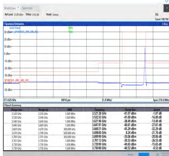
1-N48-30-30-H-2-CP-QPSK-Edge_1RB_Right-1@77-Ant1 1-1--PASS-see graph
