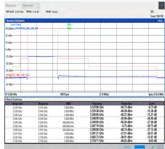
1-N48-30-40-L-3-CP-QPSK-Outer_Full-106@0-Ant1 t1-1--PASS-see graph
