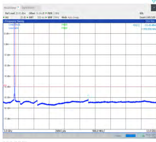
1-N48-30-40-H-1-DFT-PI2BPSK-Inner_1RB_Left-1@ 1-3000-12000-Ant1-7993.20--51.49--40-PASS
