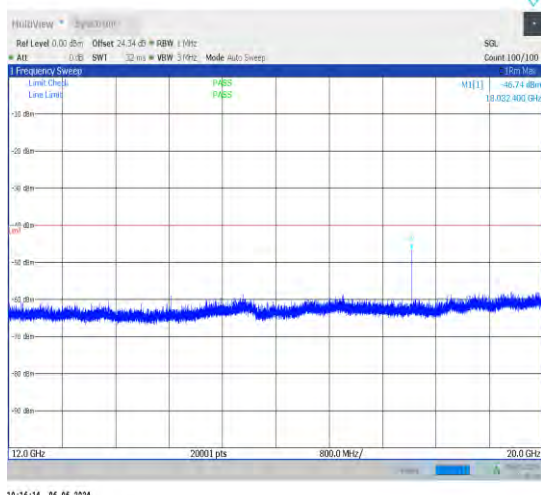
1-N48-30-40-M-1-DFT-PI2BPSK-Inner_1RB_Left-1 @1-12000-20000-Ant1-18032.40--46.74--40-PASS
