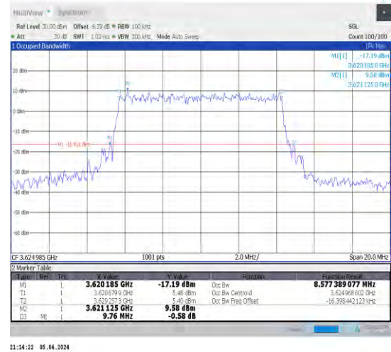
1-N48-30-10-M-6-CP-QPSK-Outer_Full-24@0-Ant1- 8.577-9.760-≤10-PASS
