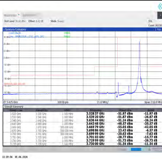
1-N48-30-30-H-2-DFT-PI2BPSK-Edge_1RB_Right-1@77-Ant1-1--PASS-see graph
