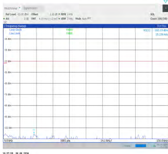
1-N48-30-40-H-1-DFT-PI2BPSK-Inner_1RB_Left-1@ 1-0.009-0.15-Ant1-0.05--105.19--40-PASS
