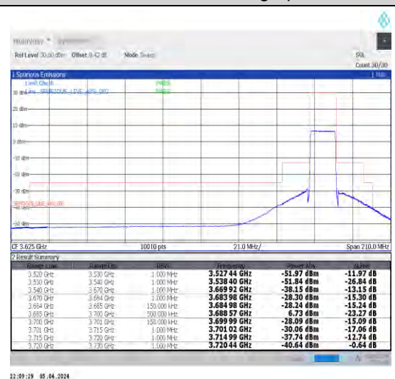
1-N48-30-15-H-6-CP-QPSK-Outer_Full-38@0-Ant1-1--PASS-see graph
