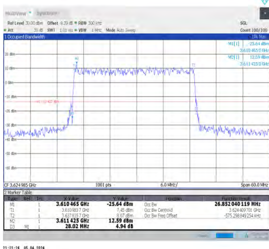
1-N48-30-30-M-4-DFT-64QAM-Outer_Full-75@0-Ant 1-26.852-28.020-≤30-PASS
