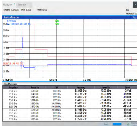
1-N48-30-20-L-1-CP-QPSK-Edge_1RB_Left-1@0-Ant1 -1--PASS-see graph
