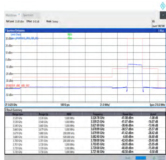
1-N48-30-20-H-3-CP-QPSK-Outer_Full-51@0-Ant1 1-1--PASS-see graph
