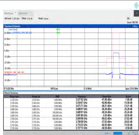
1-N48-30-10-H-3-CP-QPSK-Outer_Full-24@0-Ant1 -1--PASS-see graph
