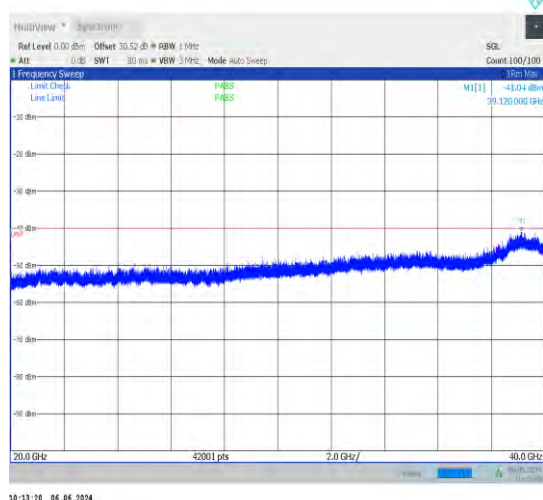
1-N48-30-40-L-1-DFT-PI2BPSK-Inner_1RB_Left-1@ 1-20000-40000-Ant1-39120.00--41.04--40-PASS
