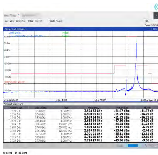
1-N48-30-15-H-2-DFT-PI2BPSK-Edge_1RB_Right-1@37-Ant1-1--PASS-see graph
