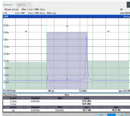
NTNV_N48_30_40_H_TID3_#1_-40_40
