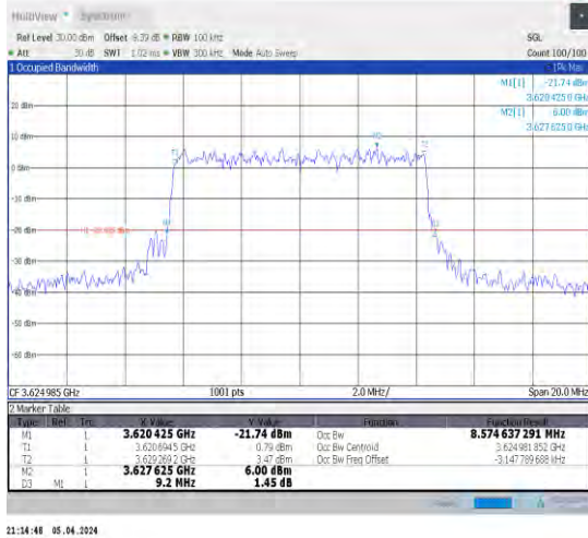
1-N48-30-10-M-9-CP-256QAM-Outer_Full-24@0-An t1-8.575-9.200-<10-PASS
