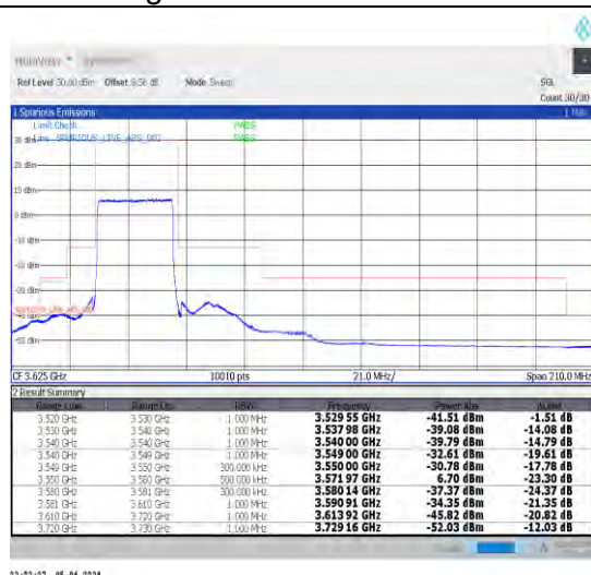
1-N48-30-30-L-3-DFT-PI2BPSK-Outer_Full-75@0-Ant1-1--PASS-see graph
