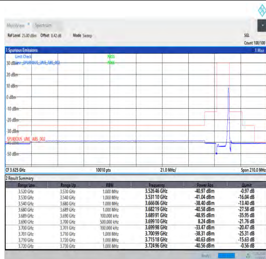
1-N48-30-10-H-2-CP-QPSK-Edge_1RB_Right-1@23-Ant1 -1--PASS-see graph
