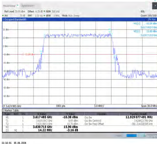
1-N48-30-15-M-2-DFT-PI2BPSK-Outer_Full-36@0-A nt1-12.929-14.220-<15-PASS
