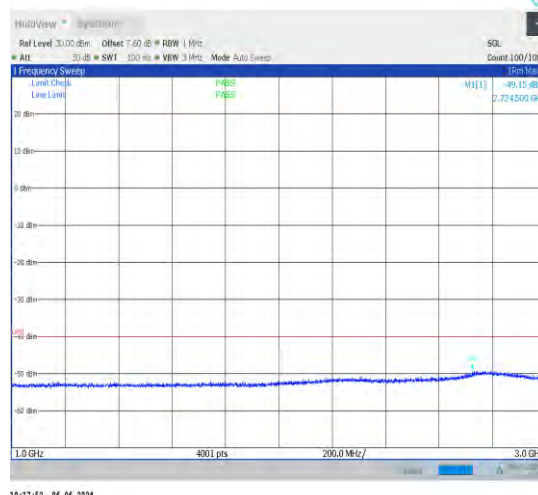
1-N48-30-40-H-1-DFT-PI2BPSK-Inner_1RB_Left-1@ 1-1000-3000-Ant1-2724.50--49.15--40-PASS
