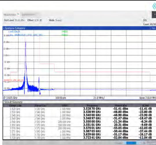
1-N48-30-20-L-1-DFT-PI2BPSK-Edge_1RB_Left-1@0-Ant1-1--PASS-see graph
