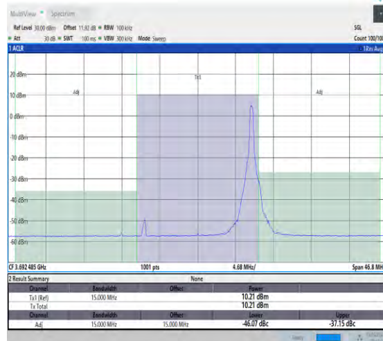
NTNV_N48_30_15_H_TID3_#1_-15_15
