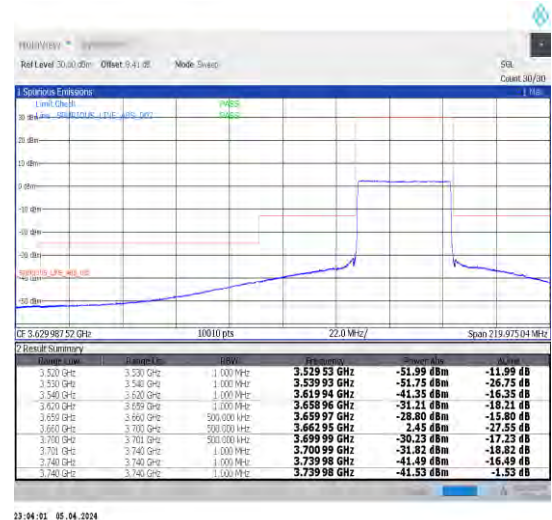
1-N48-30-40-H-6-CP-QPSK-Outer_Full-106@0-Ant1-1--PASS-see graph
