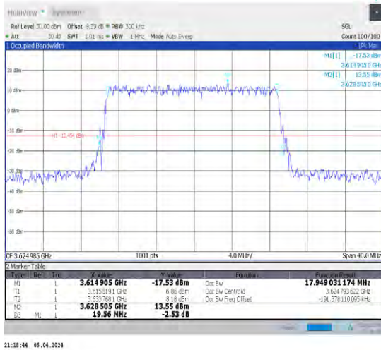
1-N48-30-20-M-3-DFT-16QAM-Outer_Full-50@0-Ant 1-17.949-19.560-≤20-PASS
