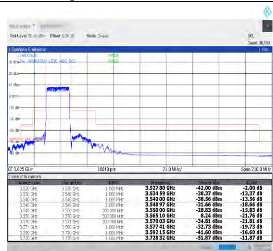
1-N48-30-20-L-3-DFT-PI2BPSK-Outer_Full-50@0-Ant1-1--PASS-see graph
