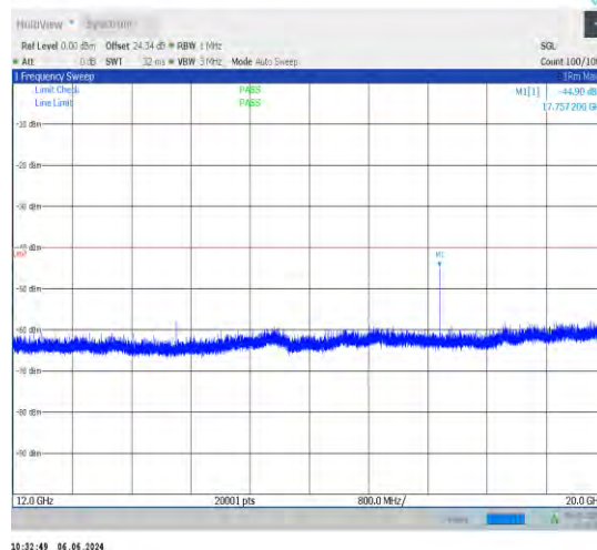
1-N48-30-40-L-1-DFT-PI2BPSK-Inner_1RB_Left-1@ 1-12000-20000-Ant1-17758.00--44.90--40-PASS
