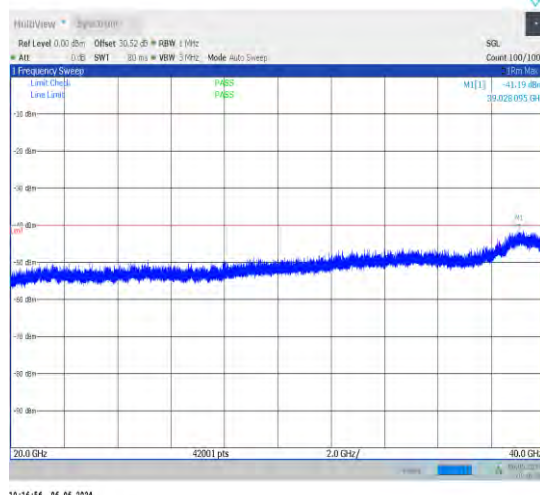
1-N48-30-40-M-1-DFT-PI2BPSK-Inner_1RB_Left-1 @1-20000-40000-Ant1-39028.10--41.19--40-PASS
