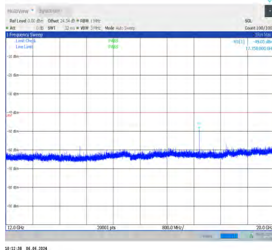
1-N48-30-40-L-1-DFT-PI2BPSK-Inner_1RB_Left-1@ 1-12000-20000-Ant1-17758.00--49.05--40-PASS
