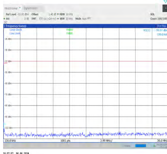
1-N48-30-40-H-1-DFT-PI2BPSK-Inner_1RB_Left-1@ 1-0.15-30-Ant1-0.18--99.97--40-PASS
