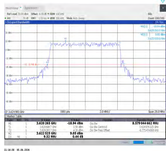
1-N48-30-10-M-8-CP-64QAM-Outer_Full-24@0-Ant1 -8.579-9.520-≤10-PASS
