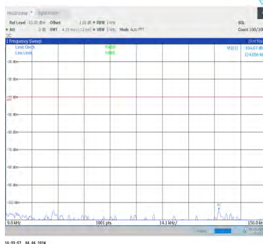
1-N48-30-40-M-1-DFT-PI2BPSK-Inner_1RB_Left-1 @1-0.009-0.15-Ant1-0.02--104.67--40-PASS
