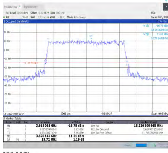
1-N48-30-20-M-8-CP-64QAM-Outer_Full-51@0-Ant1 -18.227-19.720-≤20-PASS
