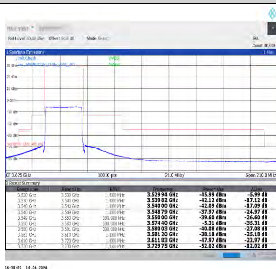
1-N48-30-30-L-6-CP-QPSK-Outer_Full-78@0-Ant1-1--PASS-see graph
