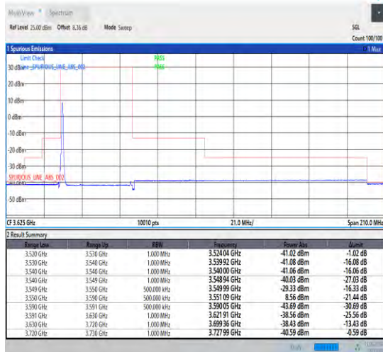
1-N48-30-40-L-1-CP-QPSK-Edge_1RB_Left-1@0-Ant1 -1--PASS-see graph
