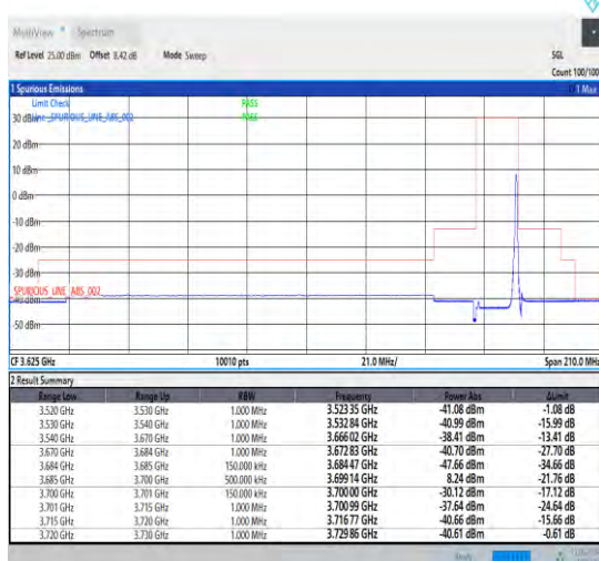
1-N48-30-15-H-2-CP-QPSK-Edge_1RB_Right-1@37-Ant1 -1--PASS-see graph
