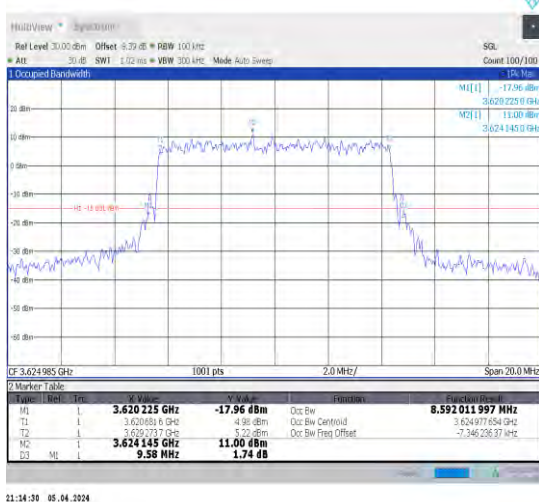
1-N48-30-10-M-7-CP-16QAM-Outer_Full-24@0-Ant 1-8.592-9.580-≤10-PASS
