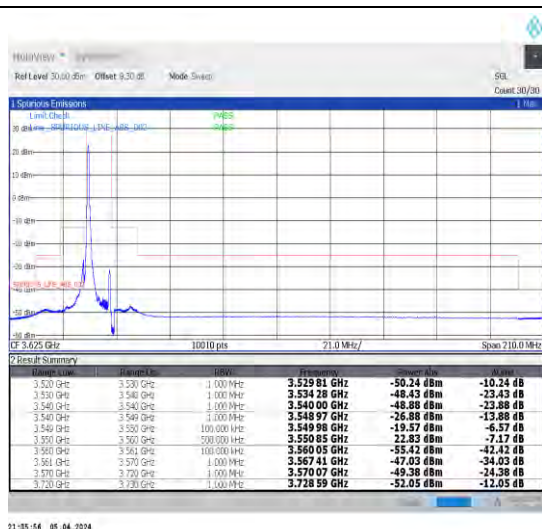
1-N48-30-10-L-1-DFT-PI2BPSK-Edge_1RB_Left-1@0-Ant1-1--PASS-see graph
