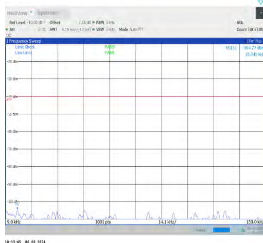
1-N48-30-40-M-1-DFT-PI2BPSK-Inner_1RB_Left-1 @1-0.009-0.15-Ant1-0.02--104.77--40-PASS
