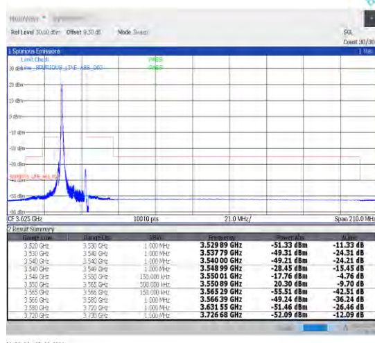
1-N48-30-15-L-4-CP-QPSK-Edge_1RB_Left-1@0-Ant1-1--PASS-see graph
