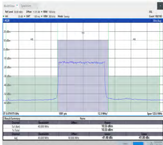
NTNV_N48_30_40_H_TID1_#1_-40_40
