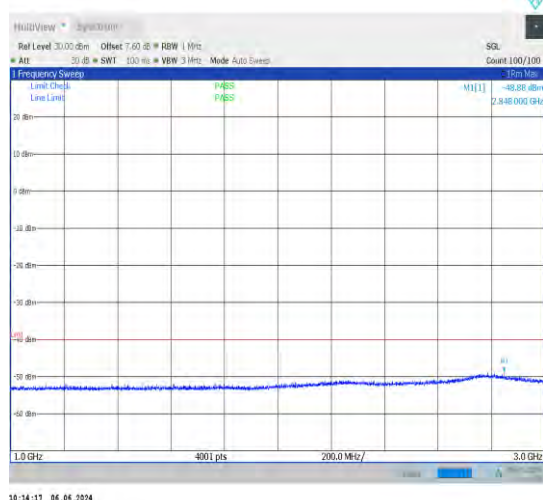
1-N48-30-40-M-1-DFT-PI2BPSK-Inner_1RB_Left-1 @1-1000-3000-Ant1-2848.00--48.88--40-PASS
