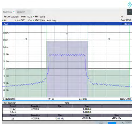
NTNV_N48_30_10_H_TID16_#1_-10_10
