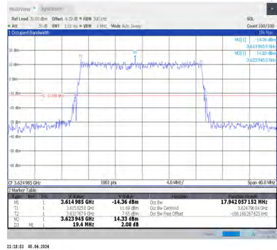
1-N48-30-20-M-4-DFT-64QAM-Outer_Full-50@0-Ant 1-17.942-19.400-≤20-PASS
