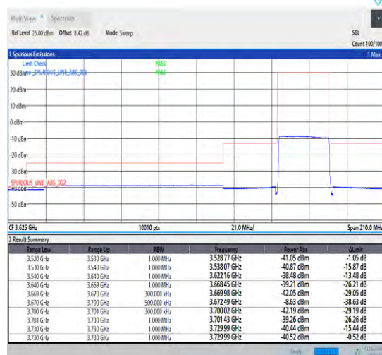
1-N48-30-30-H-3-CP-QPSK-Outer_Full-78@0-Ant1 1-1--PASS-see graph
