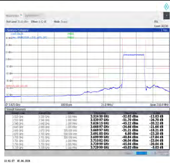
1-N48-30-30-H-3-DFT-PI2BPSK-Outer_Full-75@0-Ant1-1--PASS-see graph
