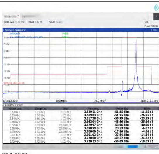
1-N48-30-20-H-2-DFT-PI2BPSK-Edge_1RB_Right-1@50-Ant1-1--PASS-see graph
