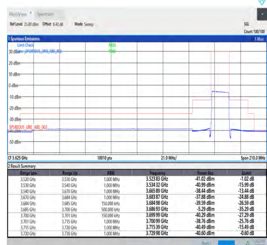
1-N48-30-15-H-3-CP-QPSK-Outer_Full-38@0-Ant1 -1--PASS-see graph
