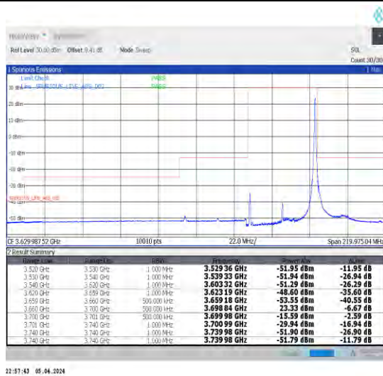
1-N48-30-40-H-2-DFT-PI2BPSK-Edge_1RB_Right-1@105-Ant1-1--PASS-see graph
