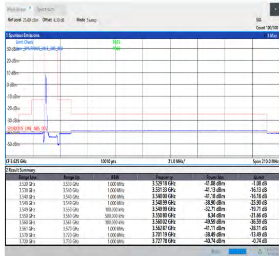
1-N48-30-10-L-1-CP-QPSK-Edge_1RB_Left-1@0-Ant1 -1--PASS-see graph
