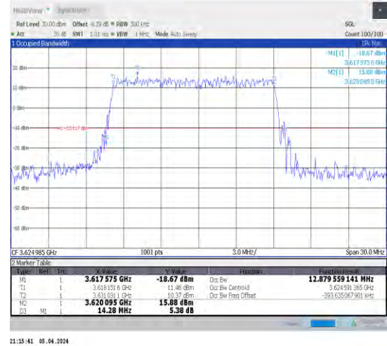
1-N48-30-15-M-1-DFT-QPSK-Outer_Full-36@0-Ant1 -12.88-14.280-<15-PASS
