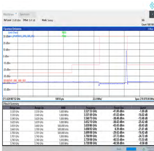
1-N48-30-40-H-2-CP-QPSK-Edge_1RB_Right-1@105-Ant1 -1--PASS-see graph
