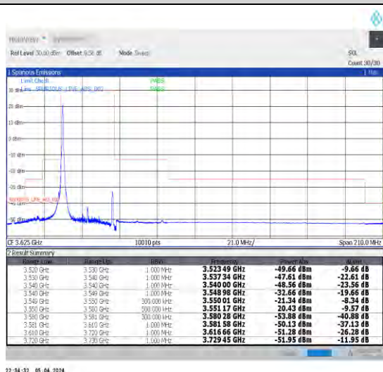
1-N48-30-30-L-4-CP-QPSK-Edge_1RB_Left-1@0-Ant1-1--PASS-see graph
