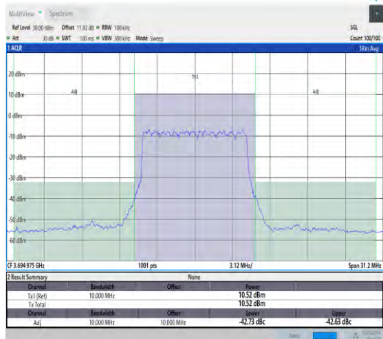
NTNV_N48_30_10_H_TID1_#1_-10_10
