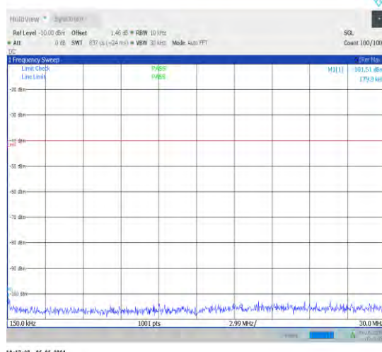
1-N48-30-40-H-1-DFT-PI2BPSK-Inner_1RB_Left-1@ 1-0.15-30-Ant1-0.18--101.51--40-PASS
