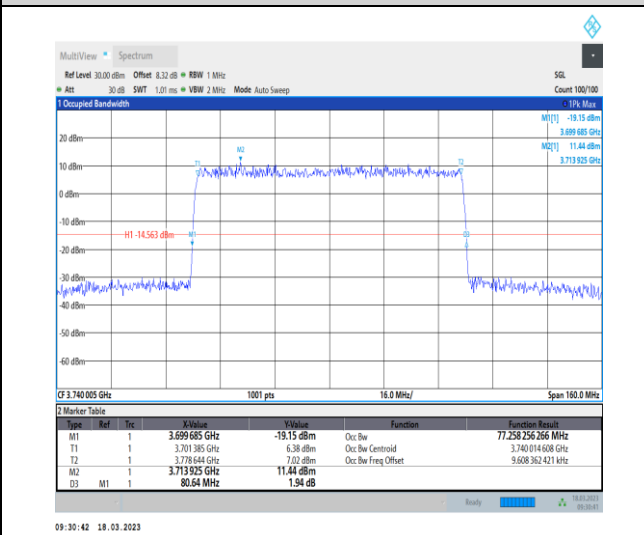
1-N78-3700-3800-30-80-L-6-CP-QPSK-Outer_Full-2 17@0-Ant0-77.258-80.640-<80-PASS
