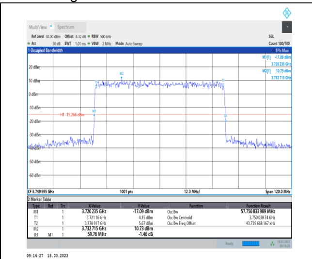
1-N78-3700-3800-30-60-M-1-DFT-QPSK-Outer_Full -162@0-Ant0-57.757-59.760-≤60-PASS
