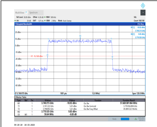
1-N78-3700-3800-30-60-H-3-DFT-16QAM-Outer_Ful I-162@0-Ant0-57.669-59.640-≤60-PASS
