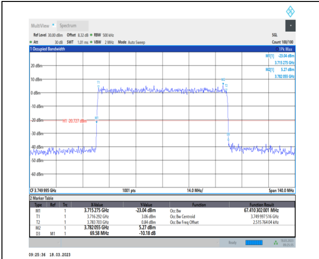
1-N78-3700-3800-30-70-M-9-CP-256QAM-Outer_Ful I-189@0-Ant0-67.41-69.580-≤70-PASS
