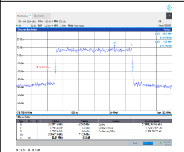
1-N78-3700-3800-30-60-M-3-DFT-16QAM-Outer_Full -162@0-Ant0-57.808-59.640-≤60-PASS
