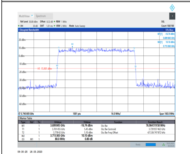
1-N78-3700-3800-30-80-L-5-DFT-256QAM-Outer_Fu ll-216@0-Ant0-76.965-80.000-<80-PASS
