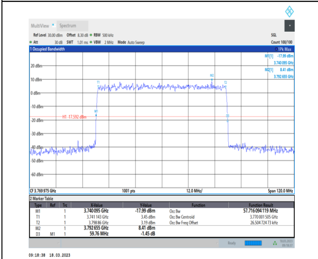
1-N78-3700-3800-30-60-H-5-DFT-256QAM-Outer_Full-162@0-Ant0-57.716-59.760-≤60-PASS
