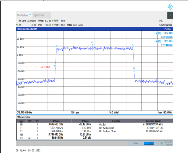
1-N78-3700-3800-30-80-L-8-CP-64QAM-Outer_Full-217@0-Ant0-77.604-80.640-≤80-PASS
