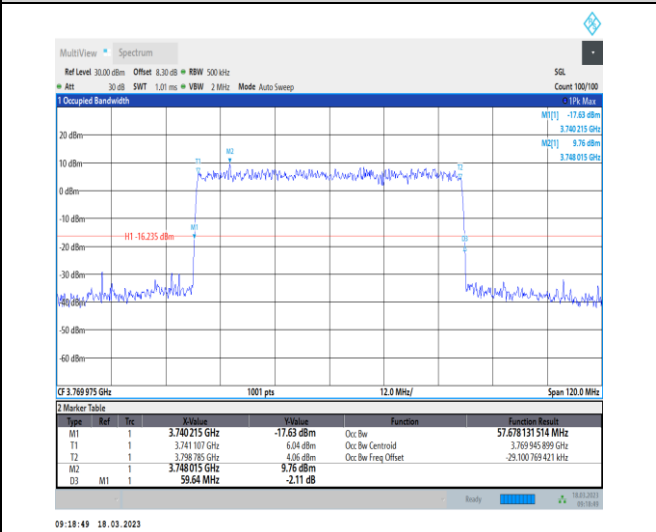
1-N78-3700-3800-30-60-H-6-CP-QPSK-Outer_Full-162@0-Ant0-57.678-59.640-≤60-PASS
