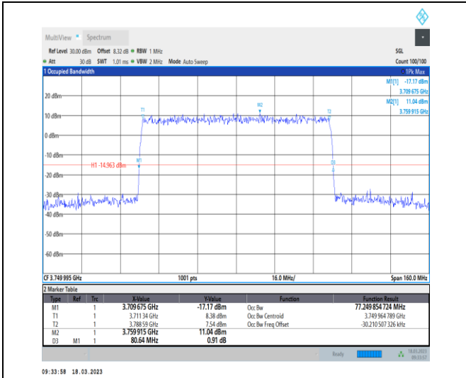
1-N78-3700-3800-30-80-M-6-CP-QPSK-Outer_Full-2 17@0-Ant0-77.25-80.640-≤80-PASS
