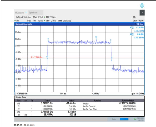
1-N78-3700-3800-30-70-H-6-CP-QPSK-Outer_Full-189@0-Ant0-67.438-69.580-≤70-PASS
