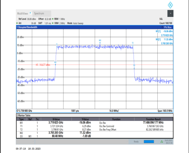
1-N78-3700-3800-30-80-H-8-CP-64QAM-Outer_Full-217@0-Ant0-77.486-80.480-≤80-PASS
