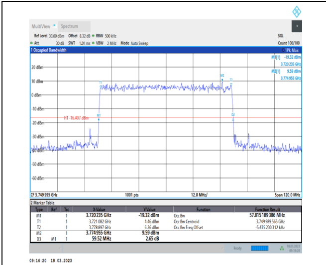
1-N78-3700-3800-30-60-M-8-CP-64QAM-Outer_Full-162@0-Ant0-57.815-59.520-≤60-PASS
