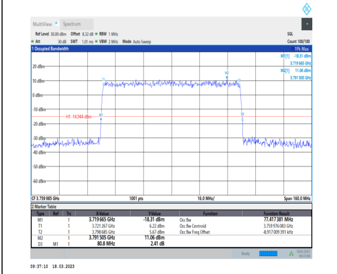
1-N78-3700-3800-30-80-H-7-CP-16QAM-Outer_Full-217@0-Ant0-77.417-80.800-≤80-PASS
