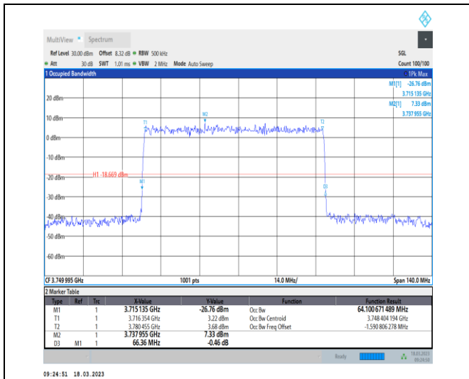
1-N78-3700-3800-30-70-M-5-DFT-256QAM-Outer_Full-180@0-Ant0-64.101-66.360-≤70-PASS
