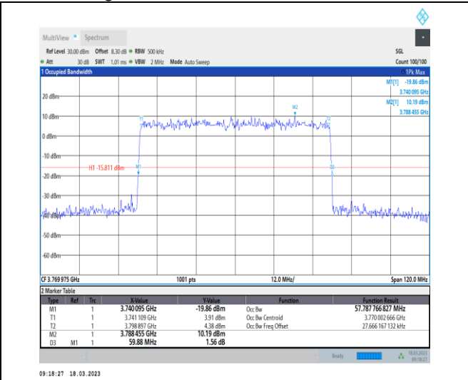
1-N78-3700-3800-30-60-H-4-DFT-64QAM-Outer_Ful I-162@0-Ant0-57.788-59.880-≤60-PASS
