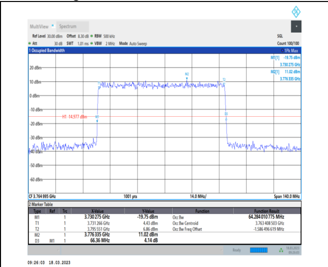
1-N78-3700-3800-30-70-H-1-DFT-QPSK-Outer_Full-180@0-Ant0-64.284-66.360-≤70-PASS
