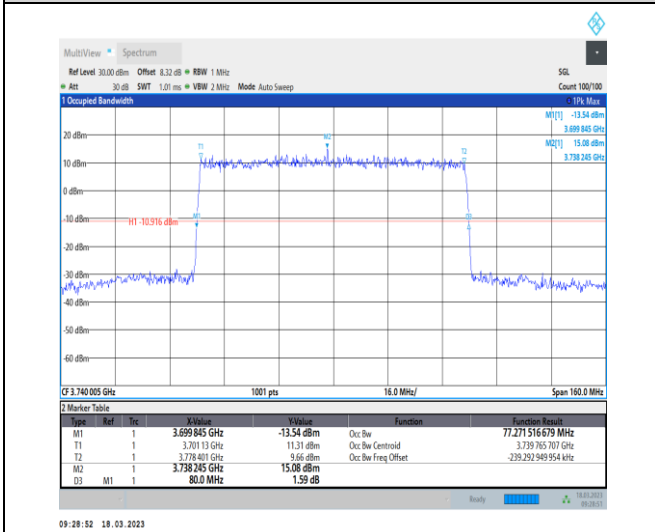
1-N78-3700-3800-30-80-L-1-DFT-QPSK-Outer_Full-216@0-Ant0-77.272-80.000-<math>\leq 80</math>-PASS
