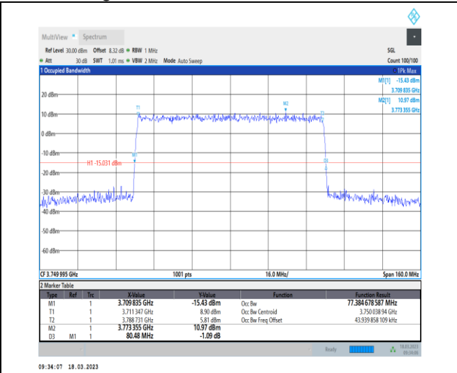
1-N78-3700-3800-30-80-M-7-CP-16QAM-Outer_Full-217@0-Ant0-77.385-80.480-≤80-PASS
