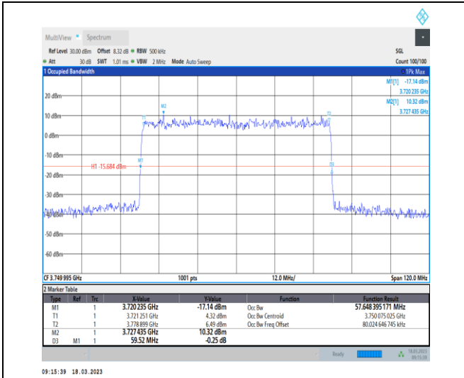
1-N78-3700-3800-30-60-M-4-DFT-64QAM-Outer_Ful I-162@0-Ant0-57.648-59.520-≤60-PASS
