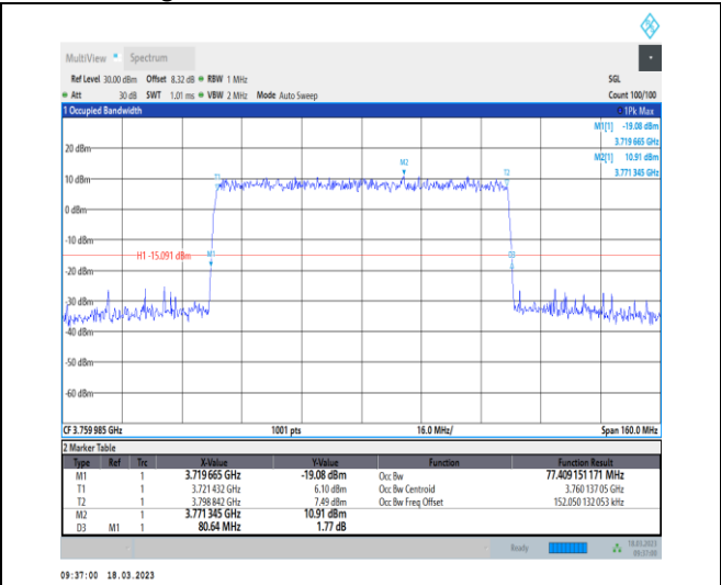
1-N78-3700-3800-30-80-H-6-CP-QPSK-Outer_Full-217@0-Ant0-77.409-80.640-≤80-PASS
