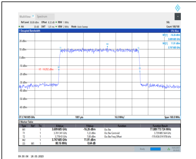
1-N78-3700-3800-30-80-L-3-DFT-16QAM-Outer_Full -216@0-Ant0-77.09-80.160-<80-PASS
