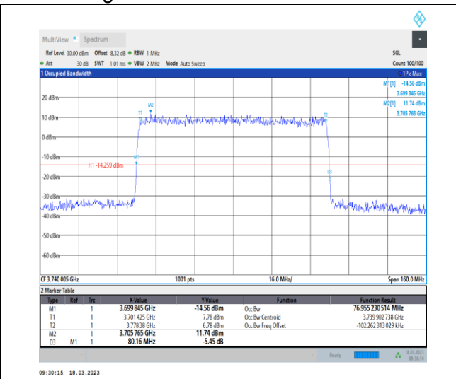
1-N78-3700-3800-30-80-L-4-DFT-64QAM-Outer_Full -216@0-Ant0-76.955-80.160-<80-PASS
