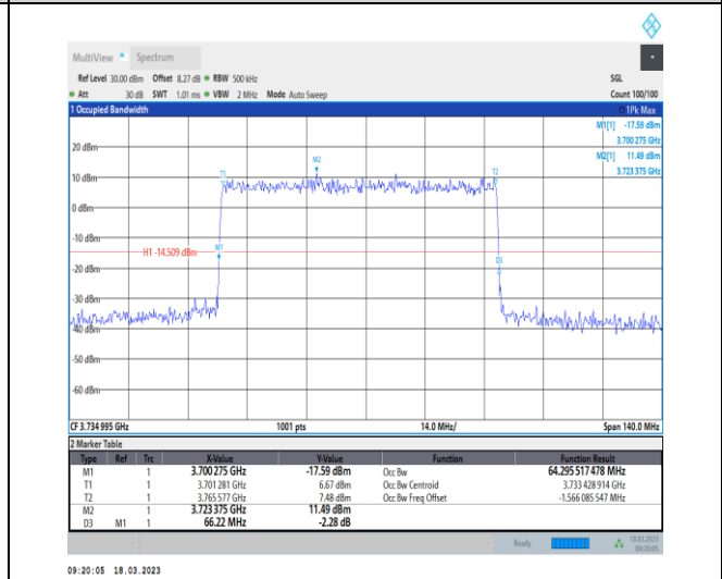
1-N78-3700-3800-30-70-L-1-DFT-QPSK-Outer_Full-180@0-Ant0-64.296-66.220-≤70-PASS
