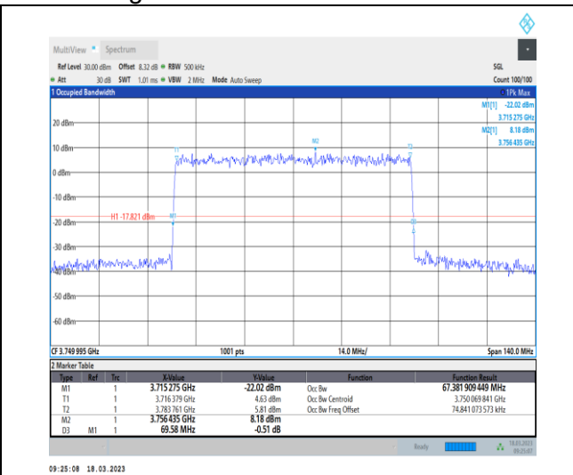
1-N78-3700-3800-30-70-M-6-CP-QPSK-Outer_Full-189@0-Ant0-67.382-69.580-≤70-PASS
