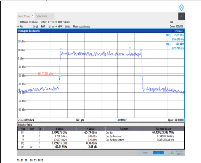
1-N78-3700-3800-30-70-L-7-CP-16QAM-Outer_Full-189@0-Ant0-67.458-69.440-≤70-PASS
