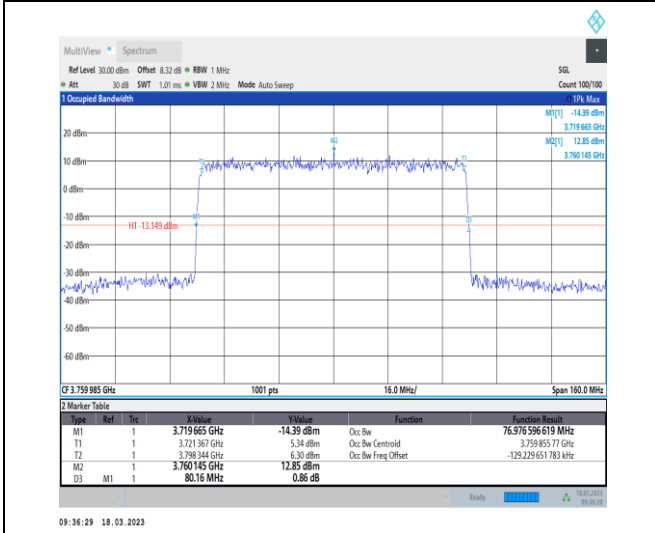
1-N78-3700-3800-30-80-H-3-DFT-16QAM-Outer_Full-216@0-Ant0-76.977-80.160-≤80-PASS
