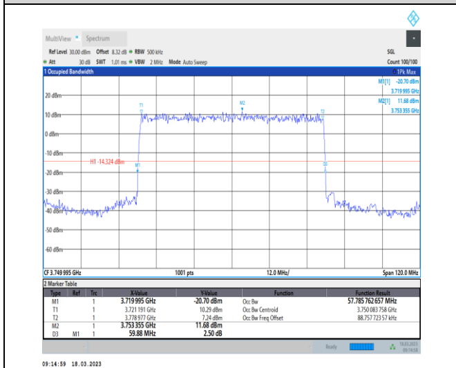
1-N78-3700-3800-30-60-M-2-DFT-PI2BPSK-Outer_Full -162@0-Ant0-57.786-59.880-≤60-PASS
