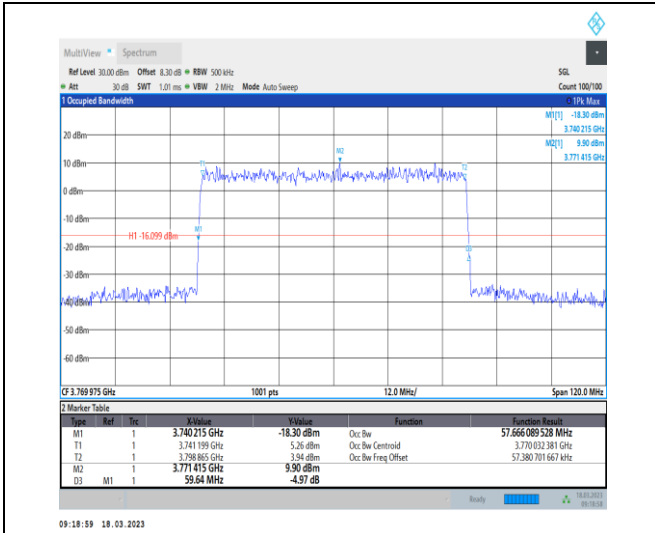
1-N78-3700-3800-30-60-H-7-CP-16QAM-Outer_Full-162@0-Ant0-57.666-59.640-≤60-PASS
