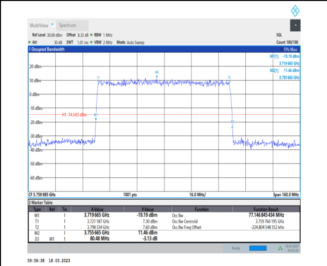
1-N78-3700-3800-30-80-H-4-DFT-64QAM-Outer_Full-216@0-Ant0-77.147-80.480-≤80-PASS
