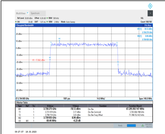
1-N78-3700-3800-30-70-H-8-CP-64QAM-Outer_Full-189@0-Ant0-67.295-69.440-<math>\leq 70</math>-PASS
