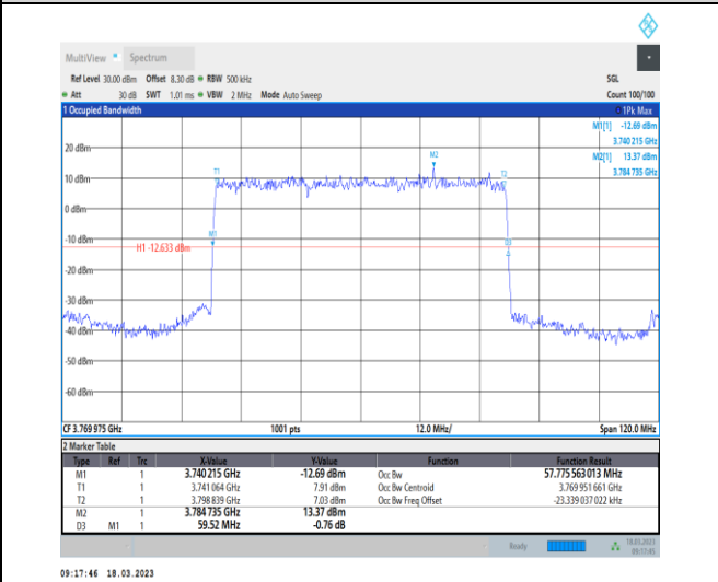
1-N78-3700-3800-30-60-H-2-DFT-PI2BPSK-Outer_Full-162@0-Ant0-57.776-59.520-≤60-PASS
