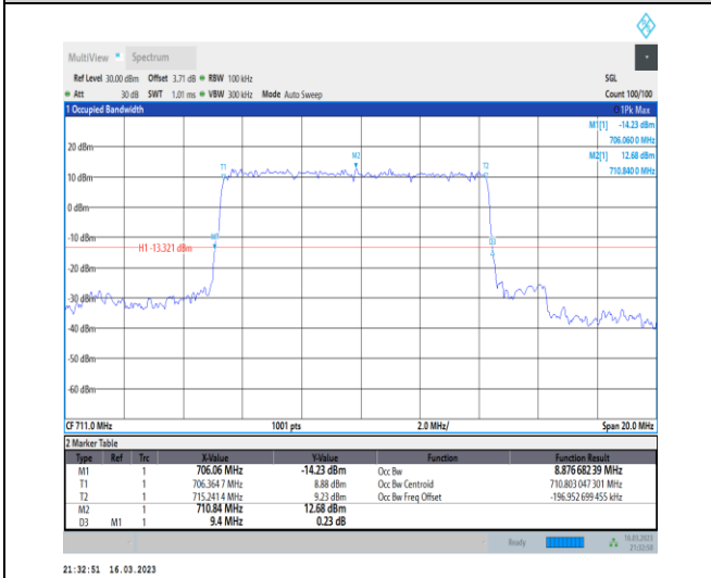
1-N12-PC3-15-10-H-2-DFT-PI2BPSK-Outer_Full-50@0-Ant7-8.877-9.400-≤10-PASS
