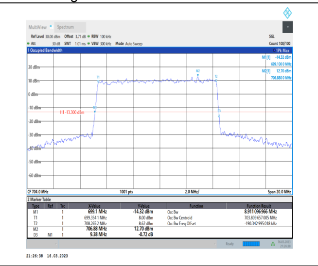
1-N12-PC3-15-10-L-3-DFT-16QAM-Outer_Full-50 @0-Ant7-8.911-9.380-≤10-PASS
