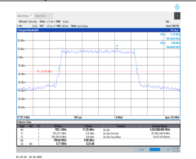
1-N12-PC3-15-5-M-5-DFT-256QAM-Outer_Full-25@0-Ant7-4.452-4.770-≤5-PASS
