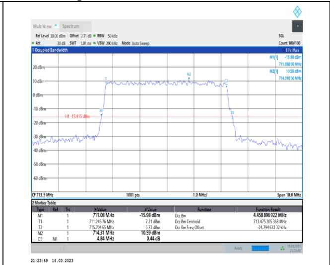
1-N12-PC3-15-5-H-4-DFT-64QAM-Outer_Full-25@0-Ant7-4.459-4.840-≤5-PASS
