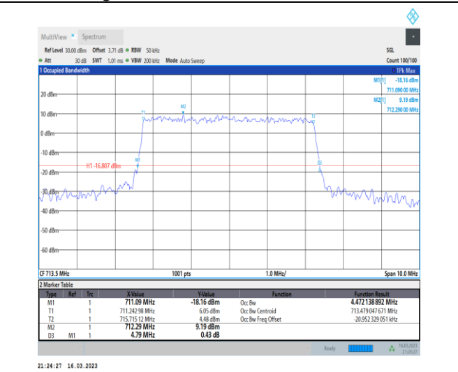
1-N12-PC3-15-5-H-8-CP-64QAM-Outer_Full-25@0-Ant7-4.472-4.790-≤5-PASS
