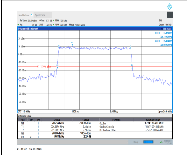
1-N12-PC3-15-10-H-6-CP-QPSK-Outer_Full-52@0-Ant7-9.274-9.680-≤10-PASS
