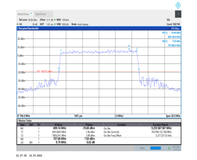
1-N12-PC3-15-10-L-9-CP-256QAM-Outer_Full-52@0-Ant7-9.256-9.740-≤10-PASS
