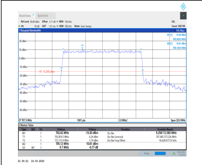
1-N12-PC3-15-10-M-7-CP-16QAM-Outer_Full-52@0 -Ant7-9.258-9.700-≤10-PASS
