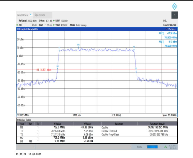
1-N12-PC3-15-10-M-8-CP-64QAM-Outer_Full-52@0 -Ant7-9.285-9.780-≤10-PASS
