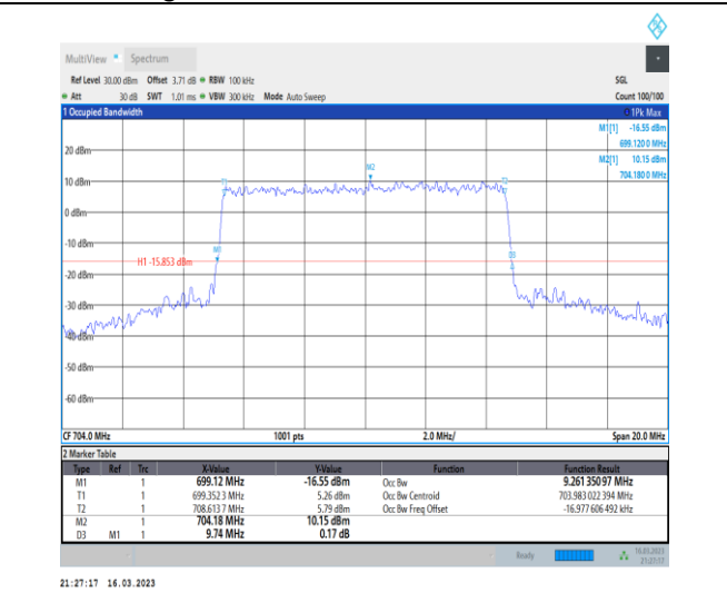
1-N12-PC3-15-10-L-7-CP-16QAM-Outer_Full-52@0-Ant7-9.261-9.740-≤10-PASS
