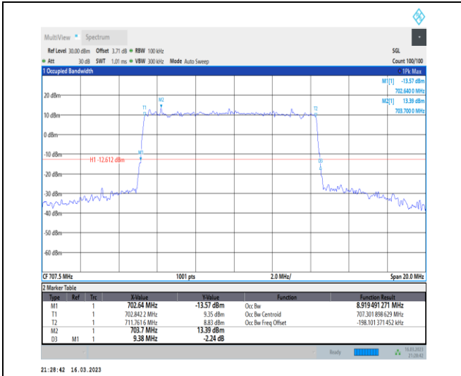
1-N12-PC3-15-10-M-1-DFT-QPSK-Outer_Full-50@0 -Ant7-8.919-9.380-≤10-PASS
