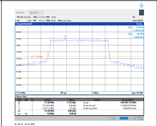
1-N12-PC3-15-5-H-6-CP-QPSK-Outer_Full-25@0-Ant7-4.462-4.800-≤5-PASS
