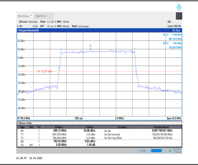
1-N12-PC3-15-10-L-5-DFT-256QAM-Outer_Full-50 @0-Ant7-8.908-9.340-≤10-PASS
