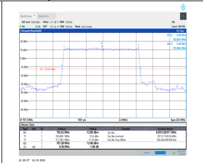
1-N12-PC3-15-10-M-2-DFT-PI2BPSK-Outer_Full-50@0-Ant7-8.936-9.380-≤10-PASS
