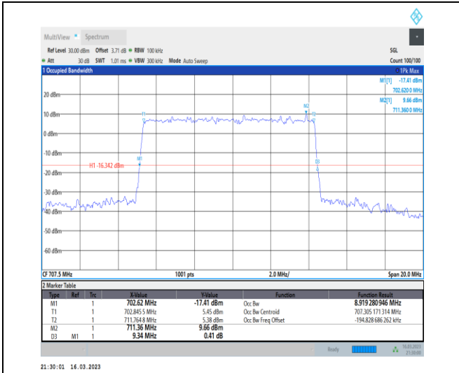
1-N12-PC3-15-10-M-5-DFT-256QAM-Outer_Full-50 @0-Ant7-8.919-9.340-≤10-PASS
