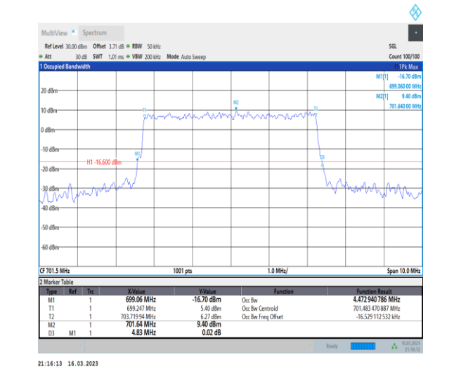
1-N12-PC3-15-5-L-8-CP-64QAM-Outer_Full-25@0-Ant7-4.473-4.830-≤5-PASS
