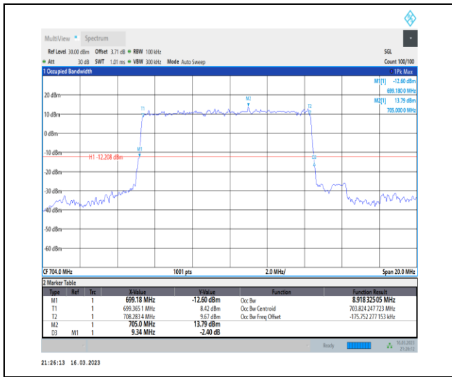
1-N12-PC3-15-10-L-2-DFT-PI2BPSK-Outer_Full-50 @0-Ant7-8.918-9.340-≤10-PASS
