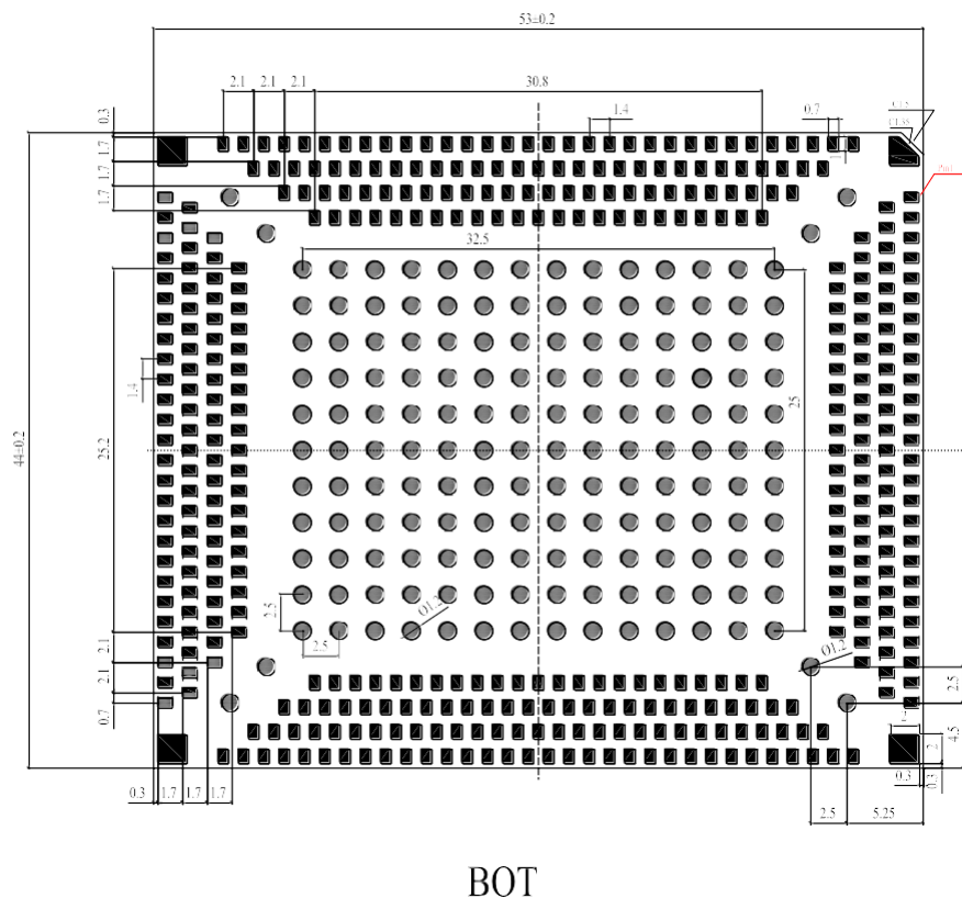
Figure 47: Bottom Dimensions
