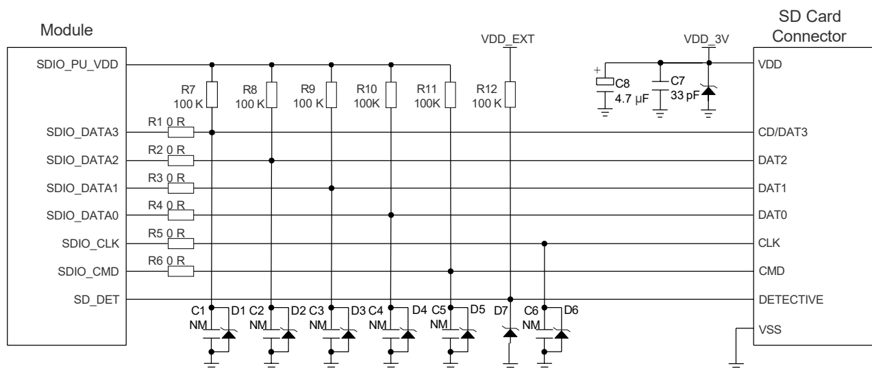
Figure 20: Reference Design of SDIO Interface
