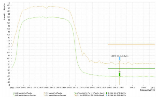
Wi-Fi2.4G_11N40_2452
