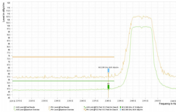
Wi-Fi2.4G_11N20_2412
