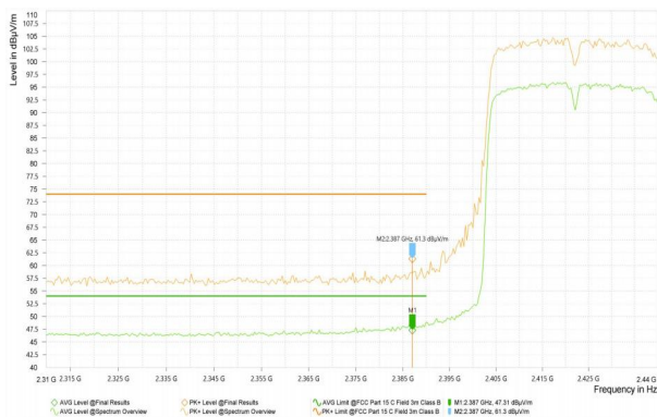
Wi-Fi2.4G_11N40_2422
