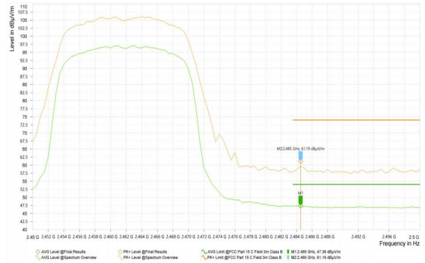
Wi-Fi2.4G_11N20_2462
