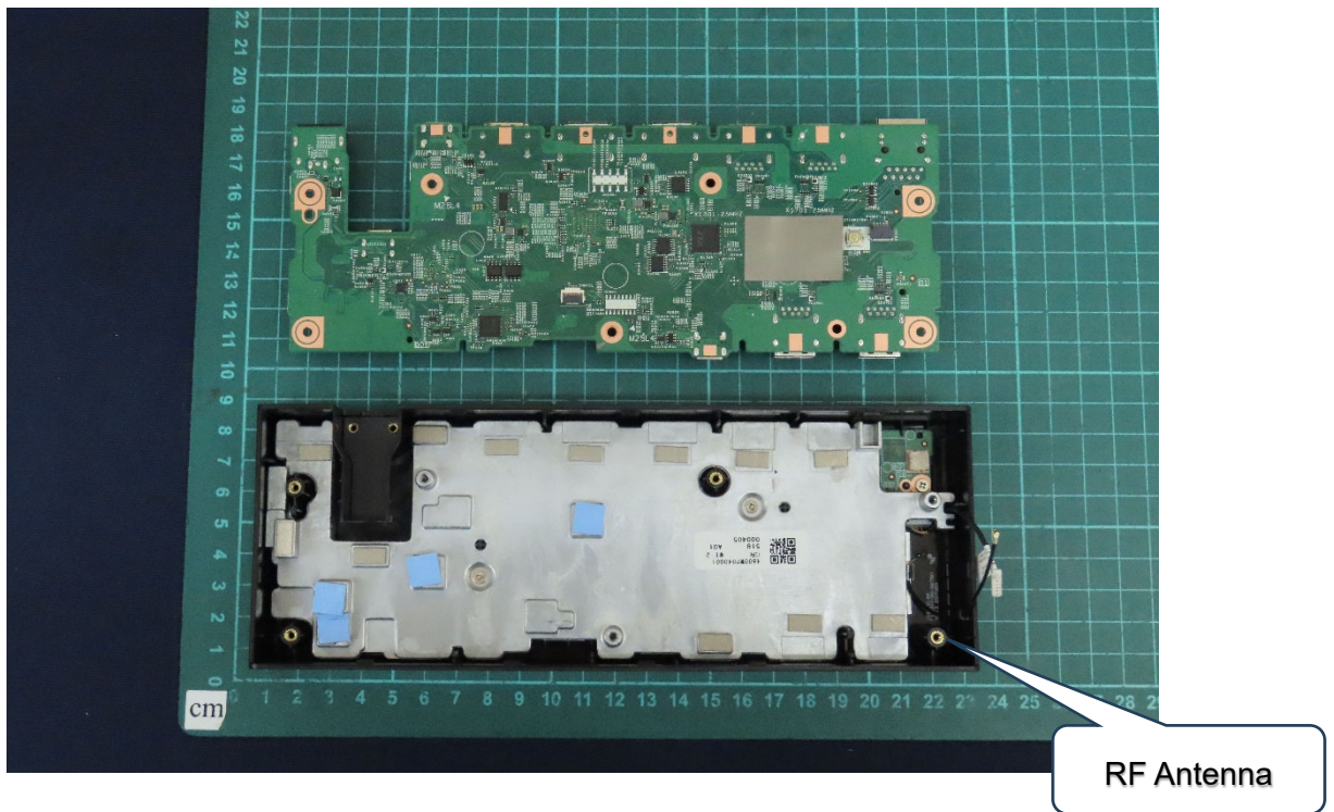
(11) EUT Photo
