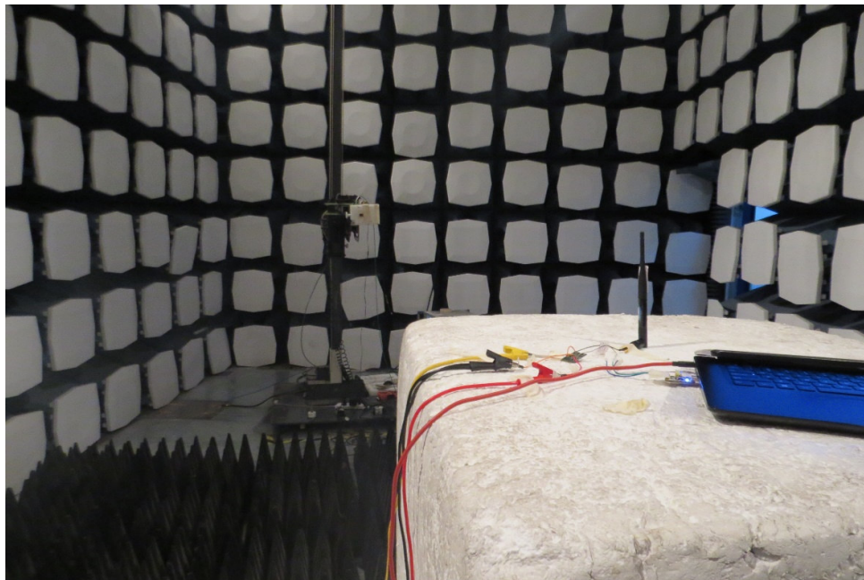
Picture 1 Radiated Emission Test Setup
