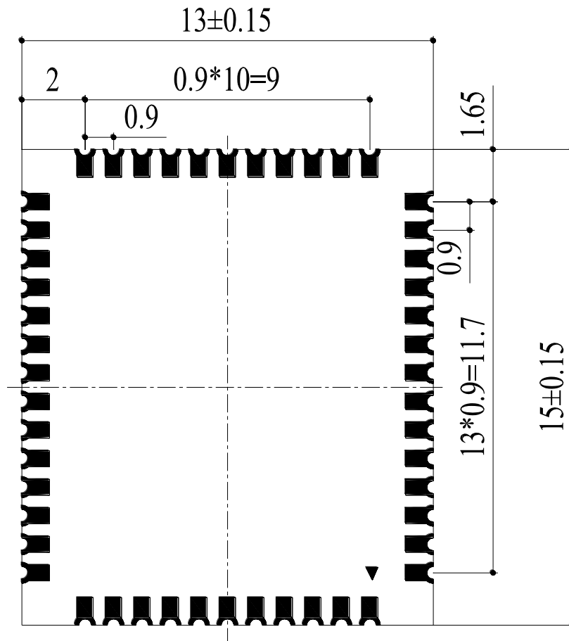
Figure 19: Bottom Dimensions (Bottom View)
