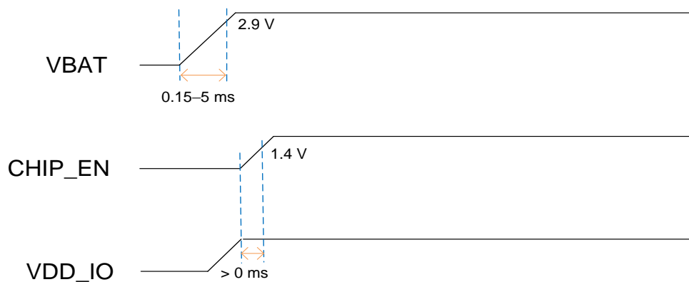
Figure 3: Power-up Timing
