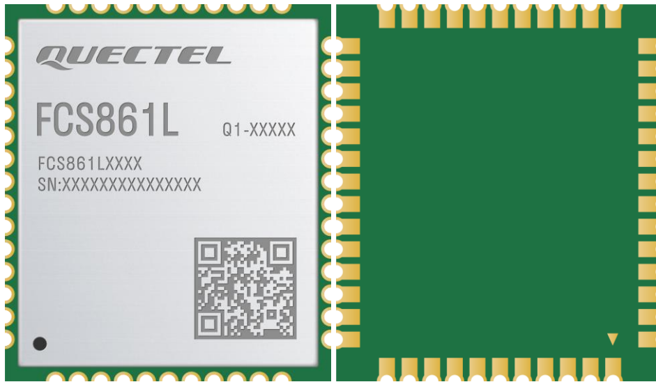
Figure 21: Top and Bottom Views
