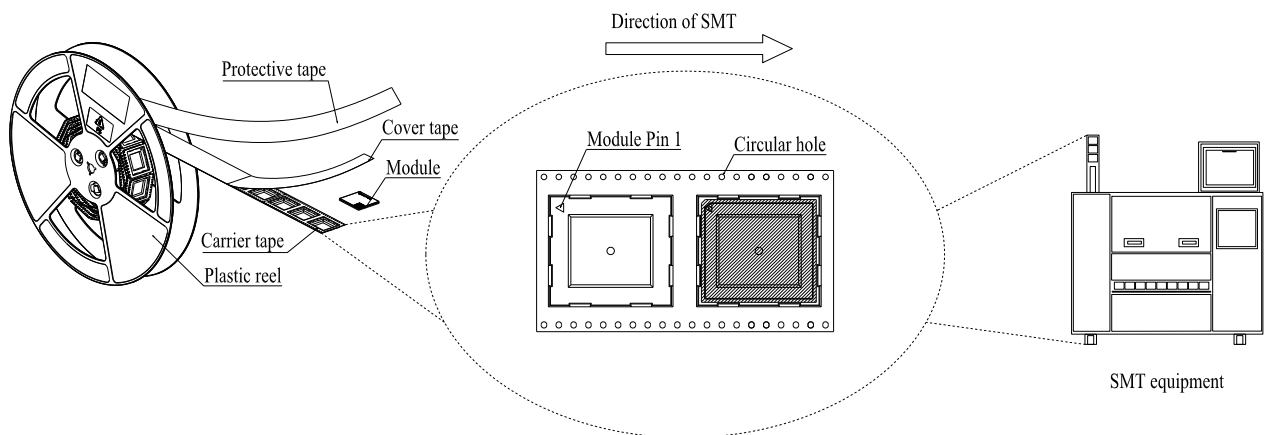
Figure 25: Mounting Direction
