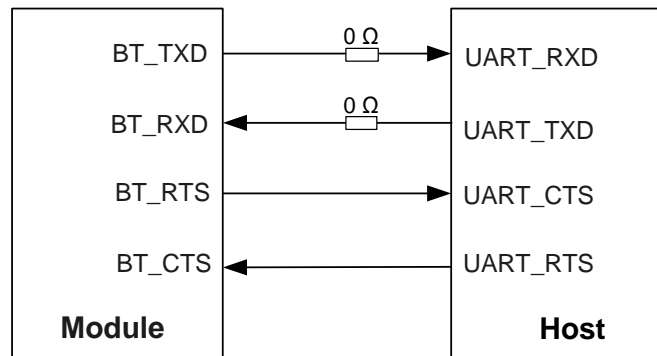
Figure 8: UART Connection
