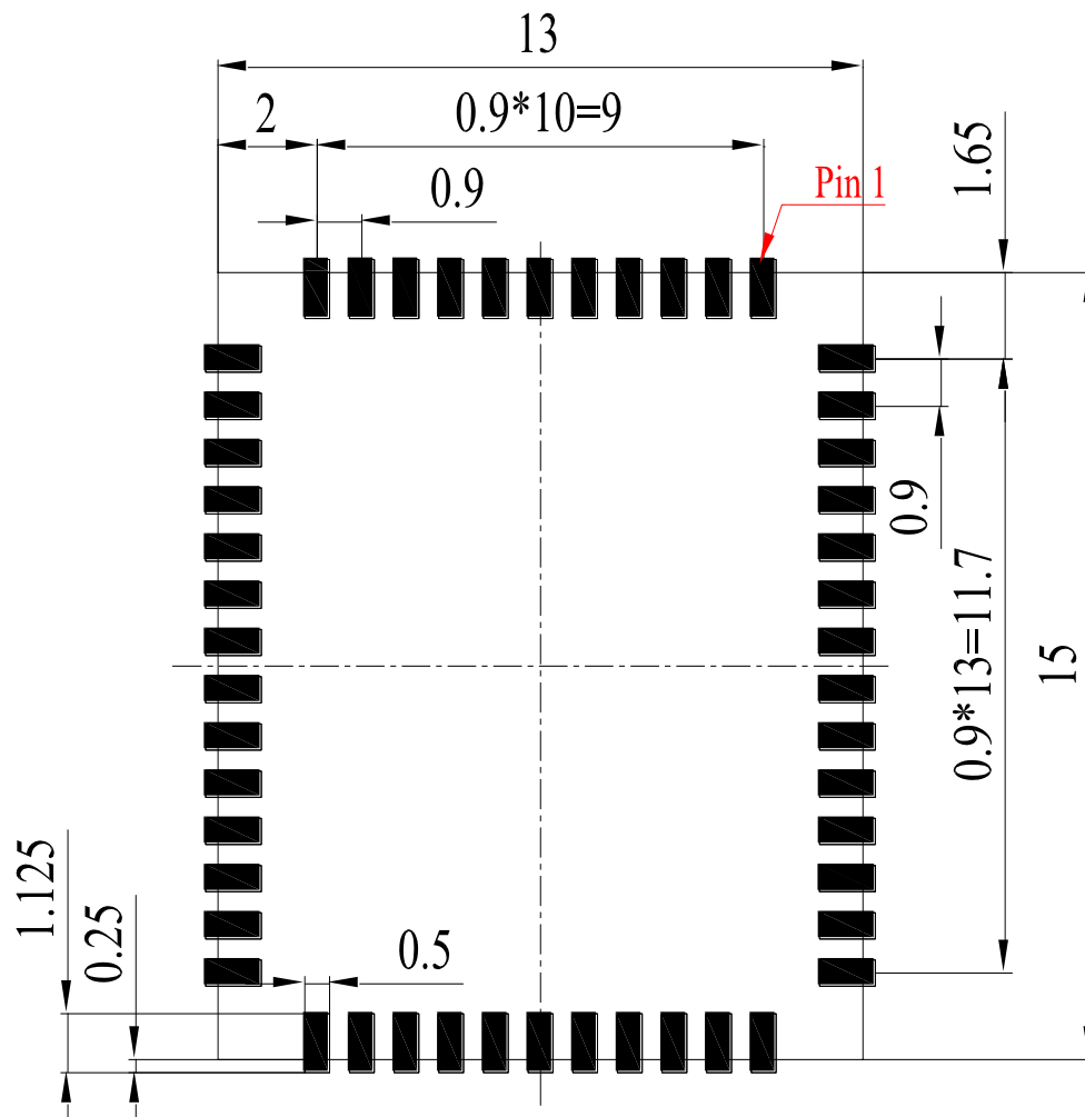
Figure 20: Recommended Footprint
