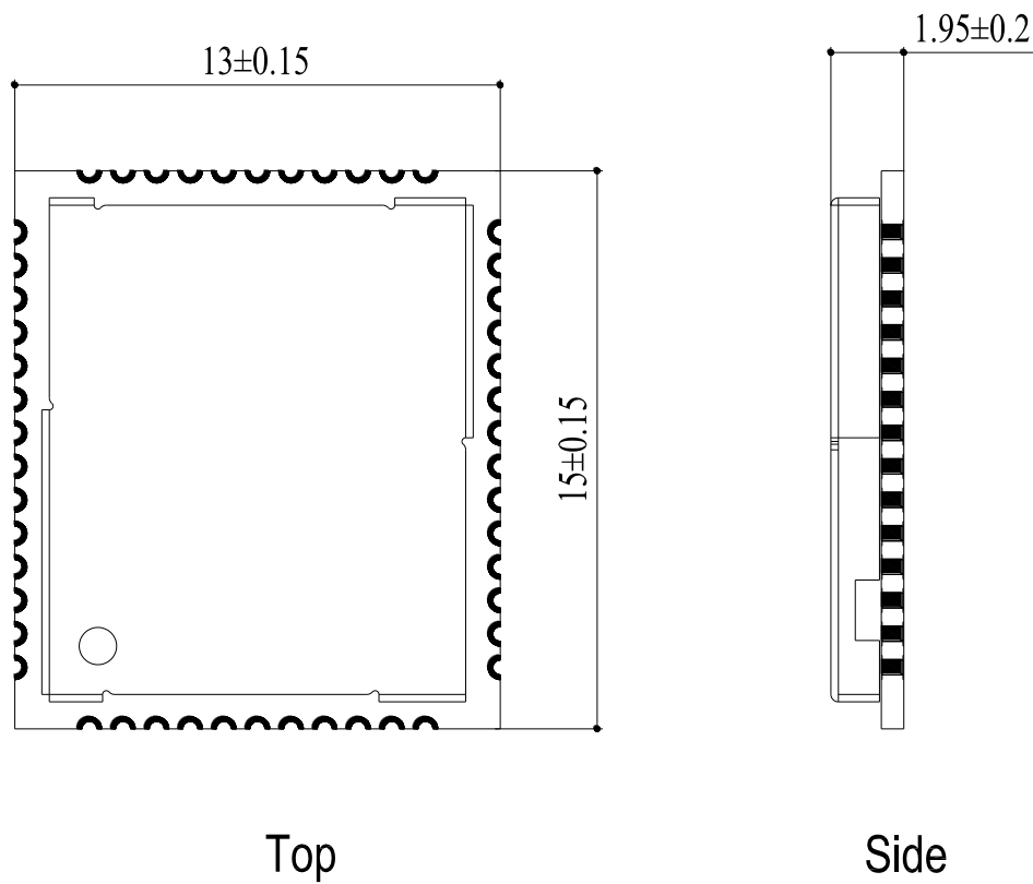
Figure 18: Top and Side Dimensions
