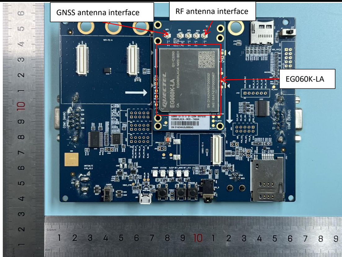
EG060K-LA + EVB _Top
