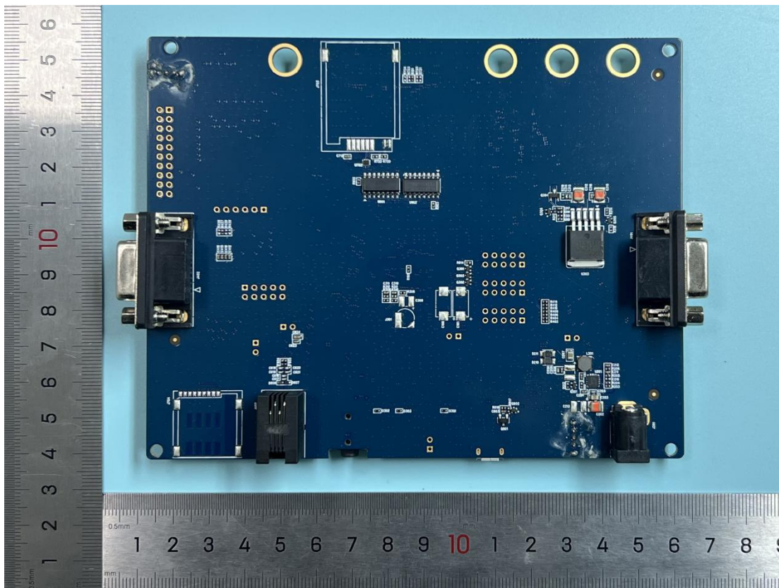
EG060K-LA + EVB _Bottom
