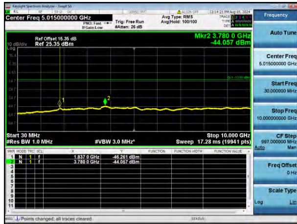
QPSK Middle channel-30MHz~10GHz
