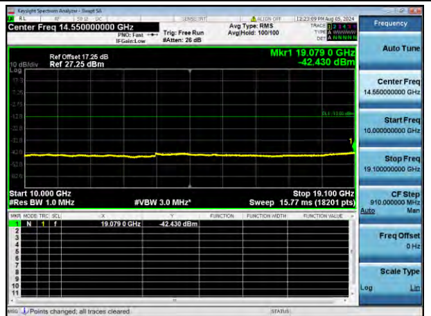
QPSK High channel-10GHz~20GHz
