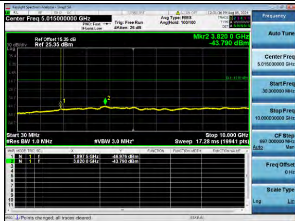
QPSK High channel-30MHz~10GHz
