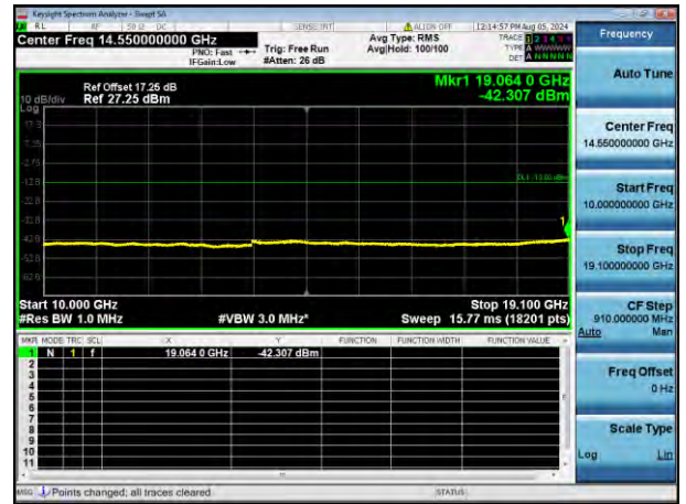
QPSK Middle channel-10GHz~20GHz
