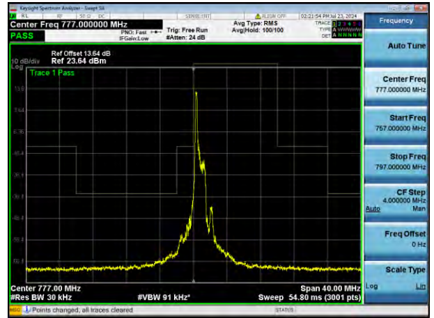
16QAM Low channel-5 RB offset 0
