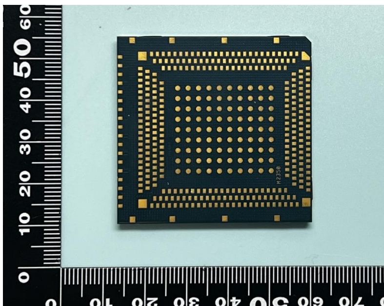
AG568N-NA_Bottom
