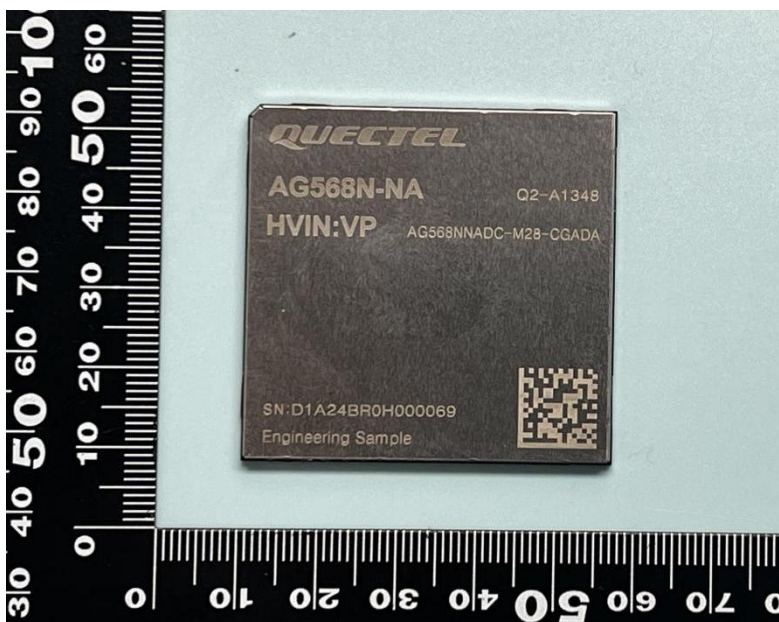
AG568N-NA_Top
