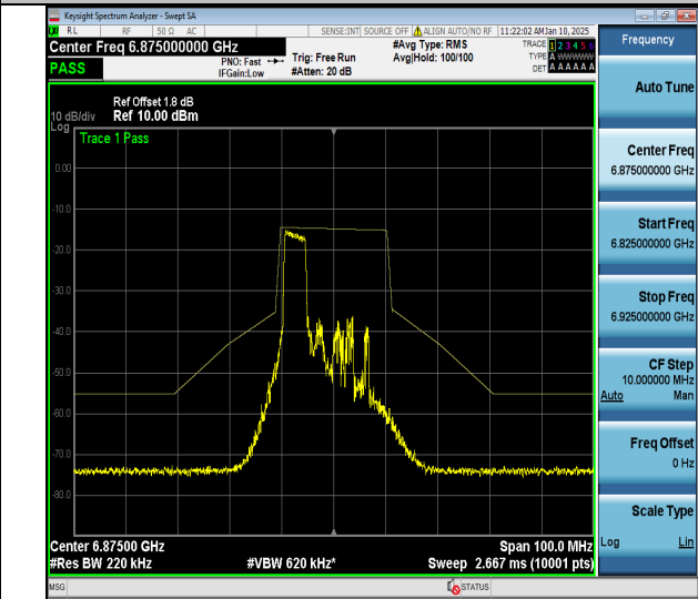
NTVN-11ax20MIMO-Ant2-6875-52Tone-RU37-PASS
