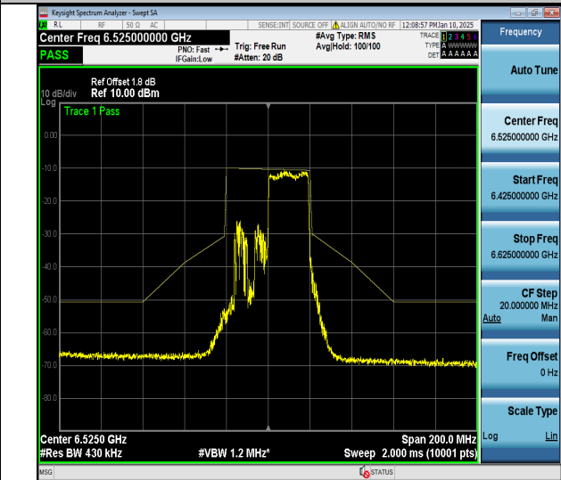
NTNV-11ax40MIMO-Ant2-6525-242Tone-RU62-PASS
