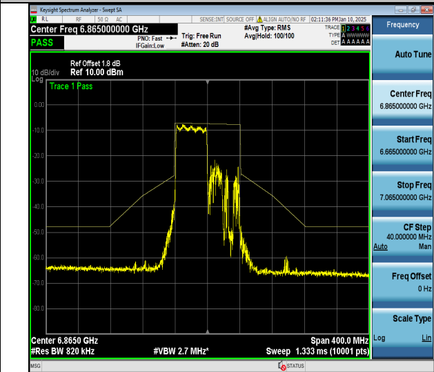
NTNV-11ax80MIMO-Ant2-6865-484Tone-RU65-PASS
