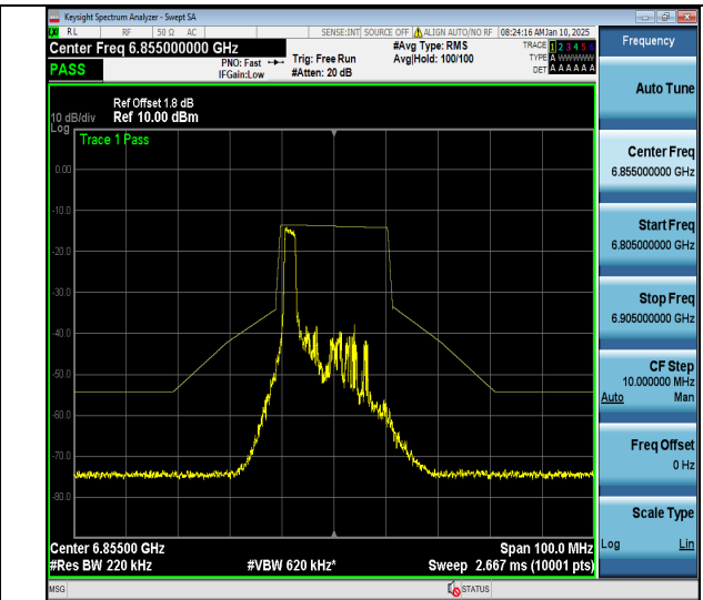
NTNV-11ax20MIMO-Ant2-6855-26Tone-RU0-PASS
