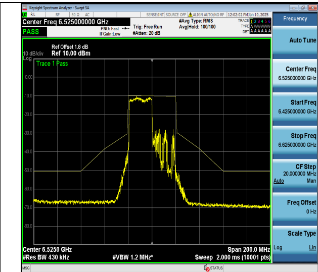
NTNV-11ax40MIMO-Ant2-6525-242Tone-RU61-PASS
