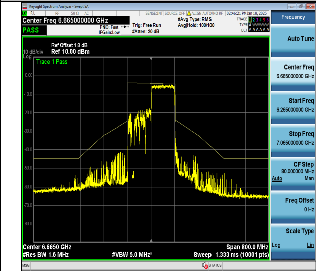
NTNV-11ax160MIMO-Ant2-6665-996Tone-RU68-PASS
