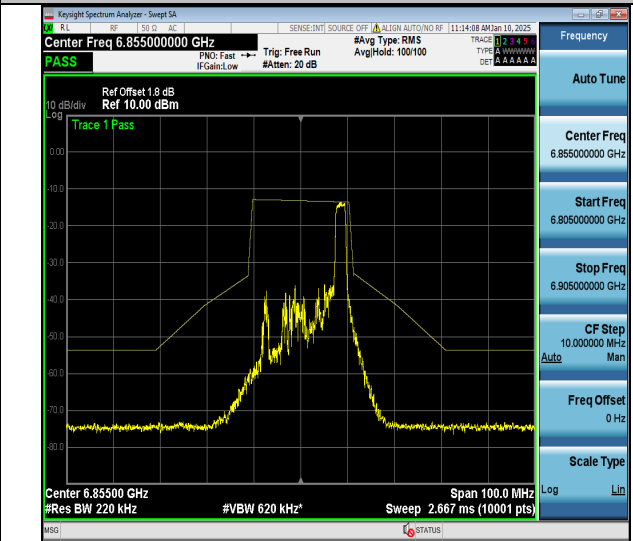
NTNV-11ax20MIMO-Ant2-6855-26Tone-RU8-PASS
