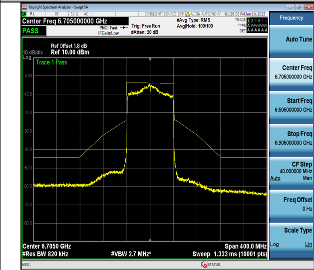
NTVN-11ax80MIMO-Ant2-6705-PASS
