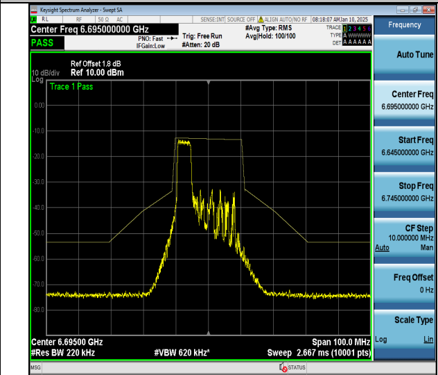
NTVN-11ax20MIMO-Ant2-6695-52Tone-RU37-PASS
