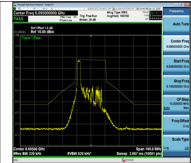
NTVN-11ax20MIMO-Ant2-6695-26Tone-RU0-PASS
