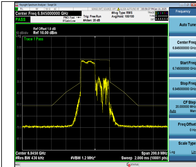
NTNV-11ax40MIMO-Ant1-6845-242Tone-RU61-PASS
