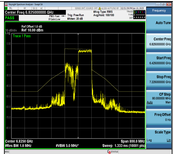
NTNV-11ax160MIMO-Ant2-6825-996Tone-RU68-PASS
