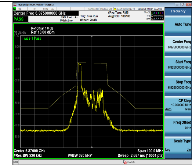
NTVN-11ax20MIMO-Ant2-6875-26Tone-RU0-PASS
