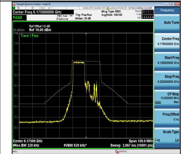
NTNV-11ax20MIMO-Ant2-6175-106Tone-RU53-PASS
