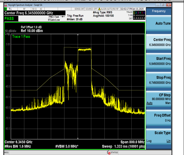
NTNV-11ax160MIMO-Ant2-6345-996Tone-RU68-PASS
