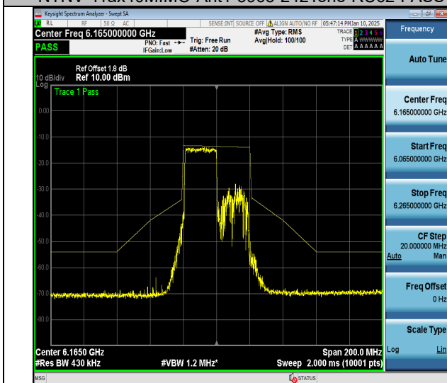
NTNV-11ax40MIMO-Ant1-6165-242Tone-RU61-PASS
