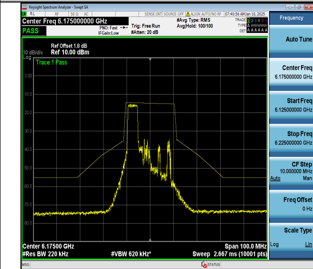
NTVN-11ax20MIMO-Ant2-6175-52Tone-RU37-PASS
