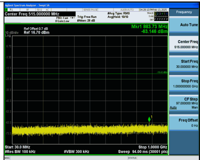
3DH5-Ant1-2480-30~1000-PASS
