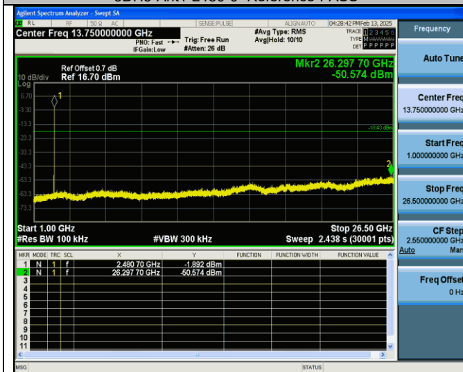
3DH5-Ant1-2480-1000~26500-PASS
