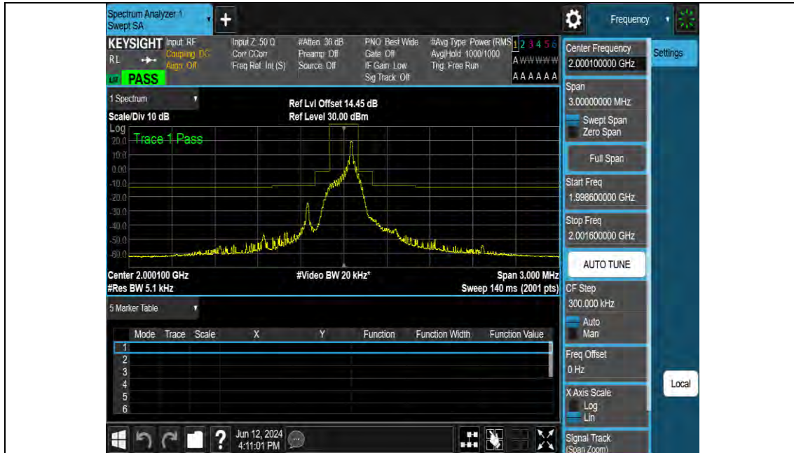
Band23-15kHz-MASK-L-BPSK-1@1
