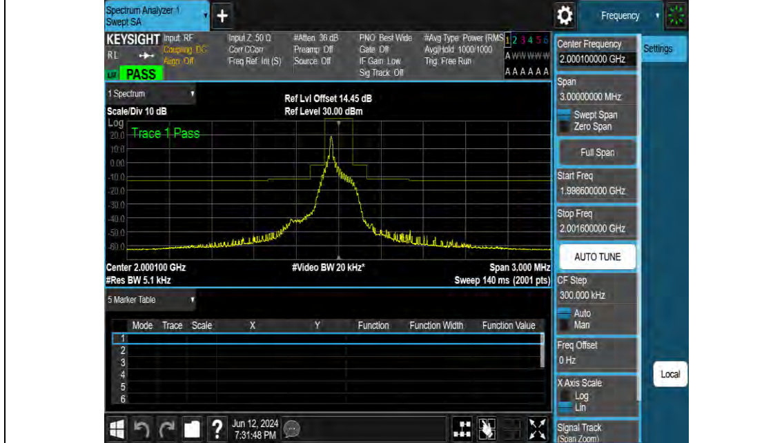
Band23-15kHz-MASK-L-BPSK-1@1
