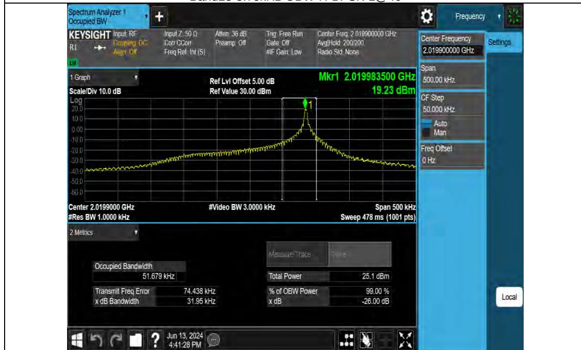
Band23-3.75kHz-OBW-H-BPSK-1@46
