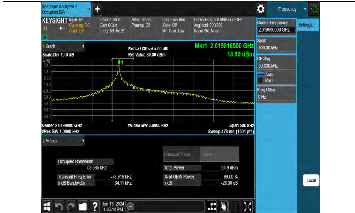
Band23-3.75kHz-OBW-H-BPSK-1@46
