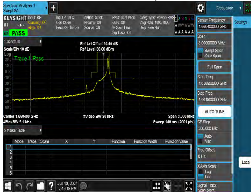
Band255-3.75kHz-MASK-H-BPSK-1@1
