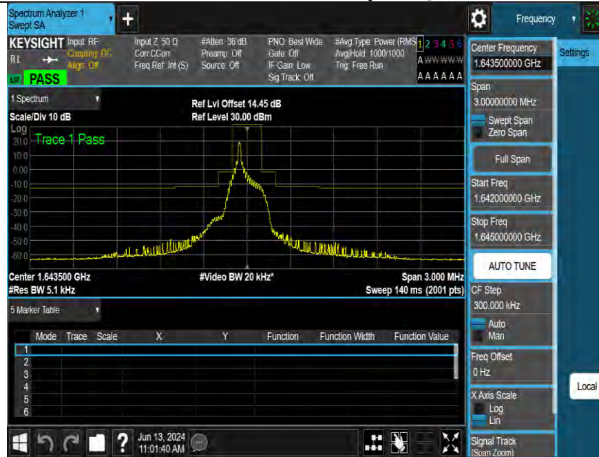
Band255-15kHz-MASK-M-QPSK-1@10
