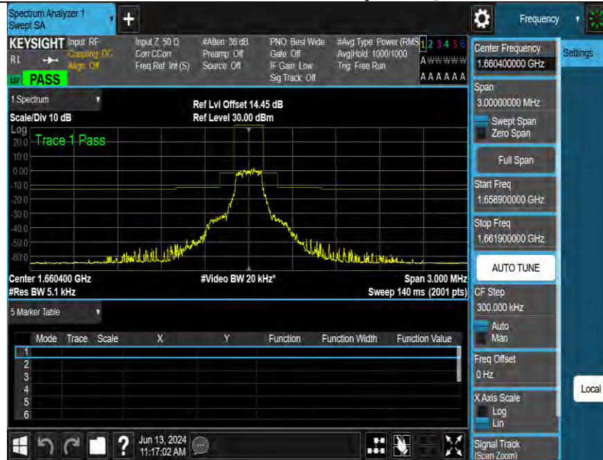
Band255-15kHz-MASK-H-QPSK-1@1
