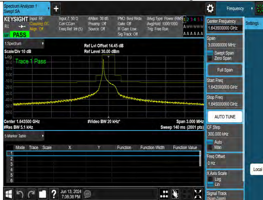
Band255-3.75kHz-MASK-M-BPSK-1@1
