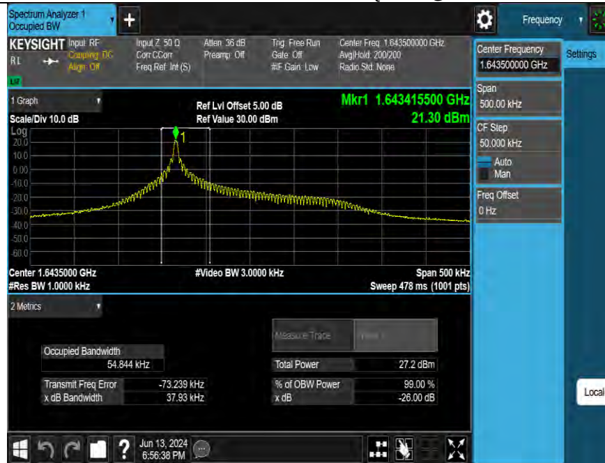
Band255-3.75kHz-OBW-M-QPSK-1@1
