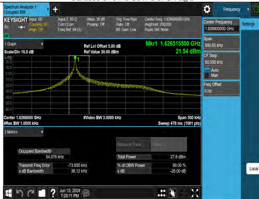
Band255-3.75kHz-OBW-L-BPSK-1@1
