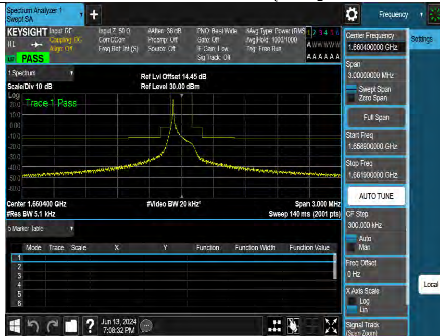
Band255-3.75kHz-MASK-H-QPSK-1@1
