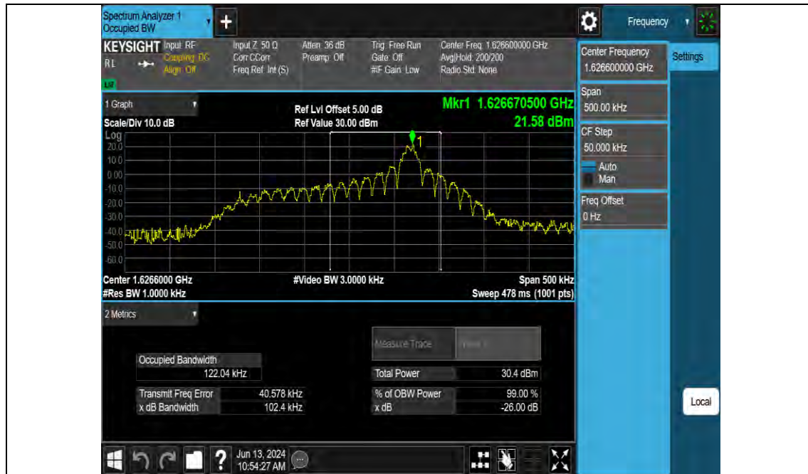
Band255-15kHz-OBW-L-BPSK-1@1
