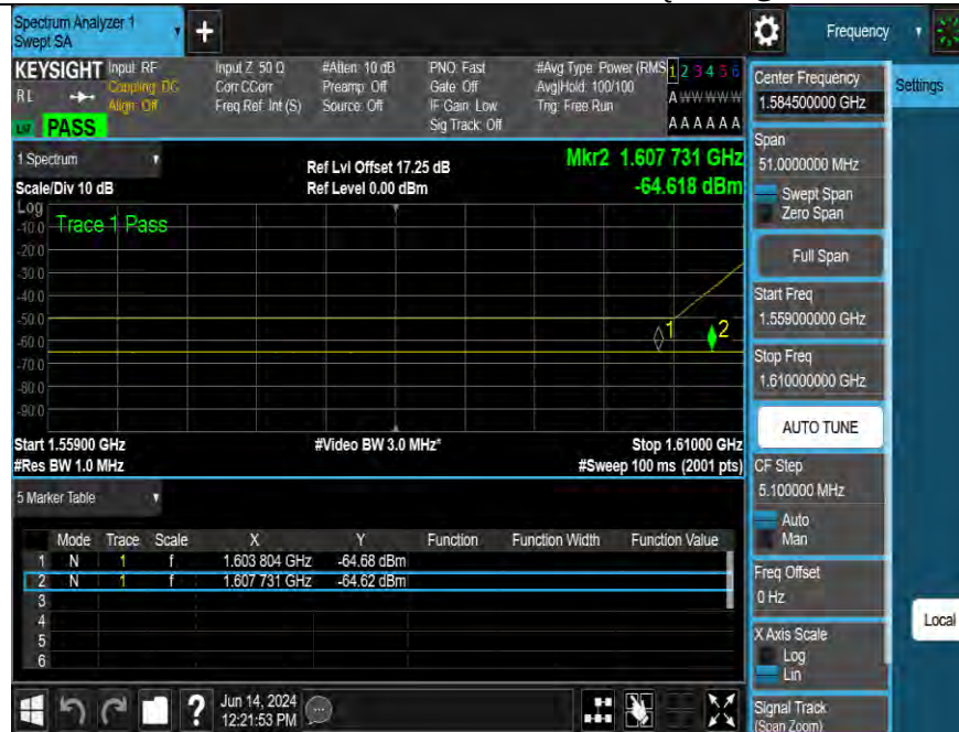
Band255-3.75kHz-Discrete emission-H-QPSK-1@1
