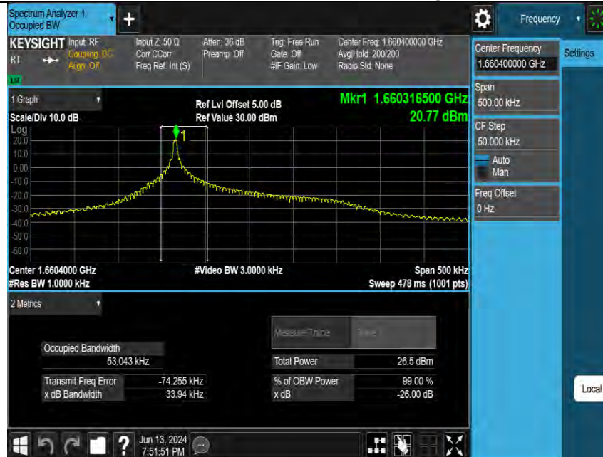
Band255-3.75kHz-OBW-H-BPSK-1@1
