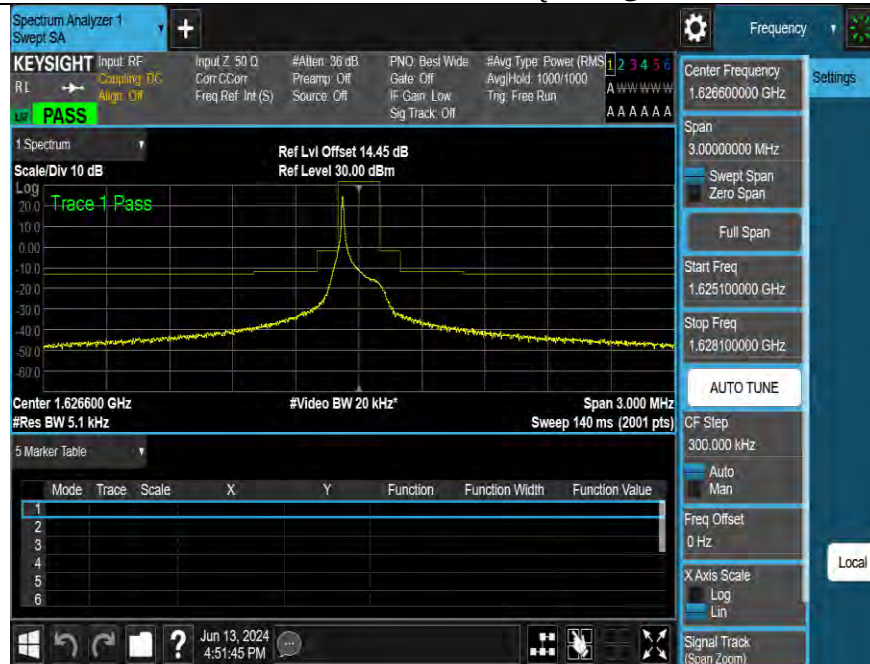
Band255-3.75kHz-MASK-L-QPSK-1@1
