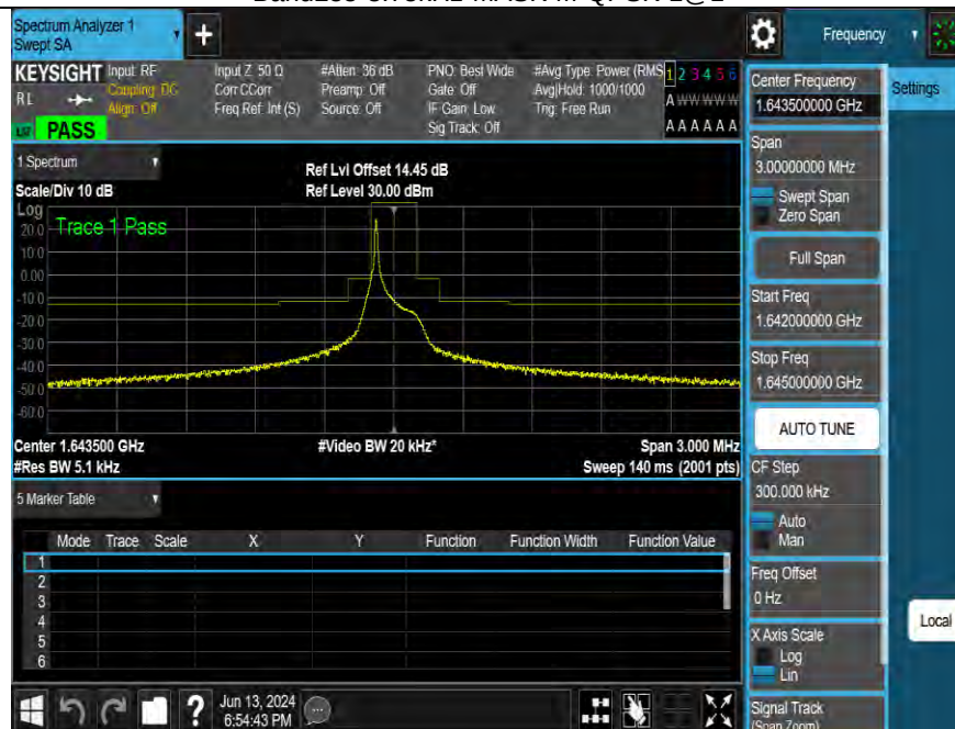
Band255-3.75kHz-MASK-M-QPSK-1@1
