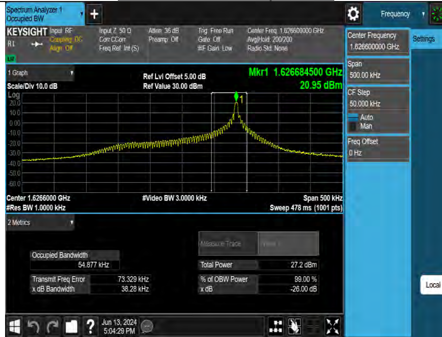
Band255-3.75kHz-OBW-L-BPSK-1@1
