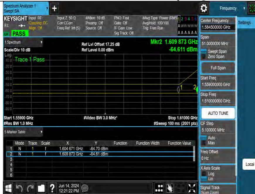
Band255-3.75kHz-Discrete emission-M-QPSK-1@1
