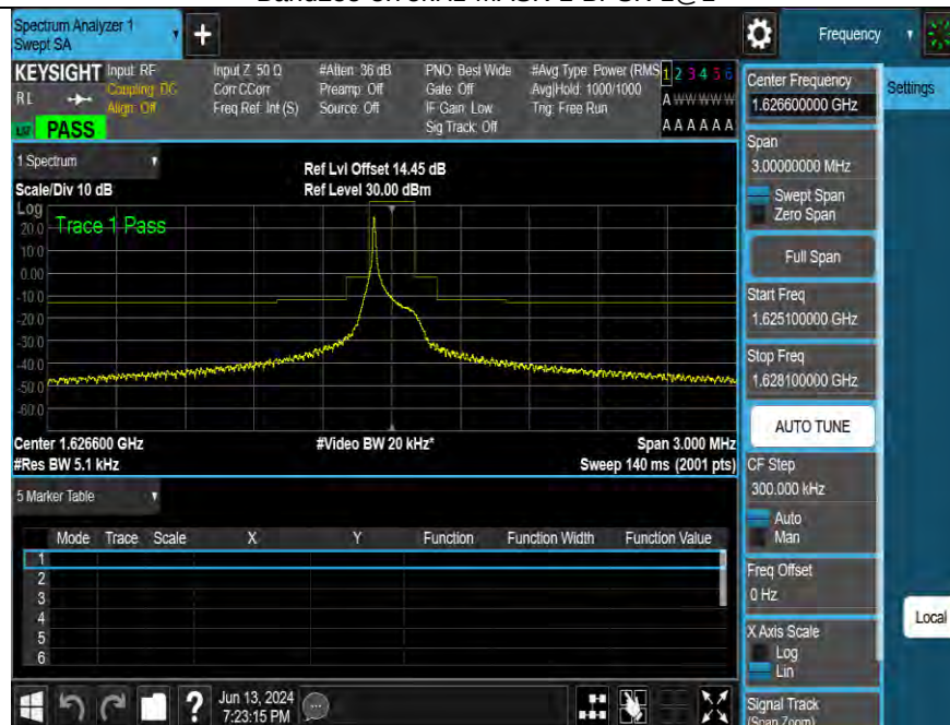
Band255-3.75kHz-MASK-L-BPSK-1@1
