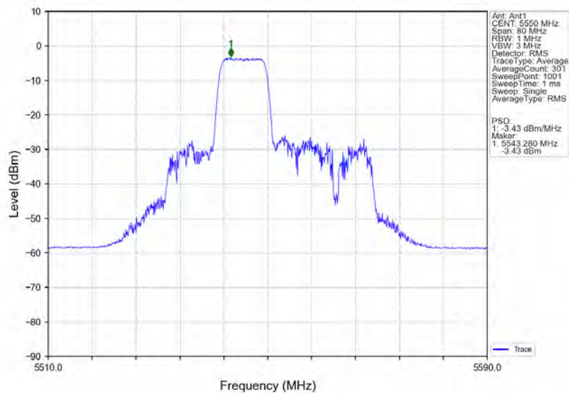
802.11ax(HE40) MCH_5550MHz_RU106_Mid_Ant1_NTNV
