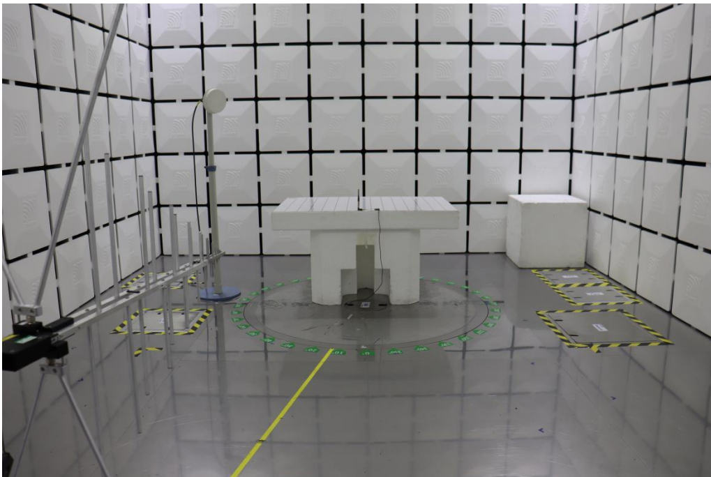
Bluetooth_30MHz to 1GHz
