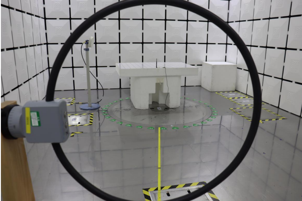
Bluetooth_9KHz to 30MHz
