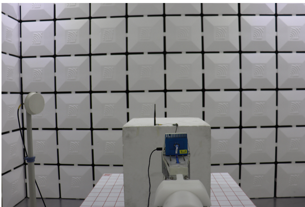
Bluetooth_Above 18GHz
