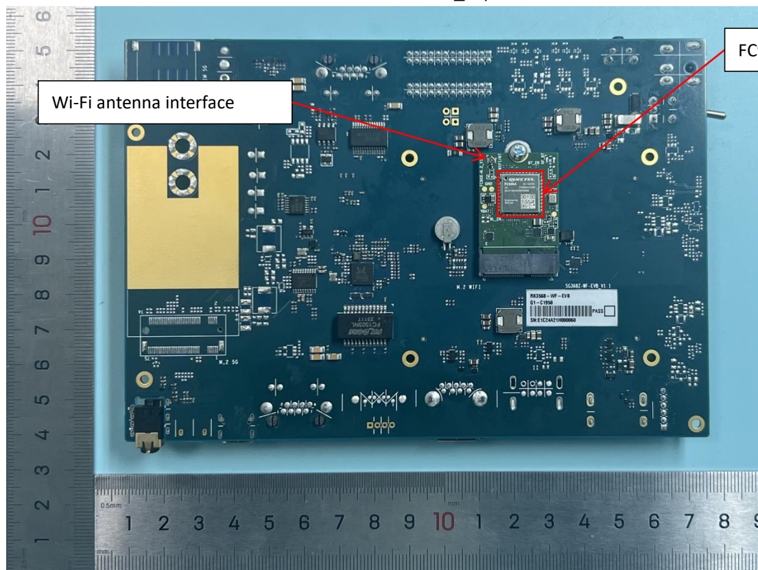
FC906A -Wi-Fi + EVB _Bottom
