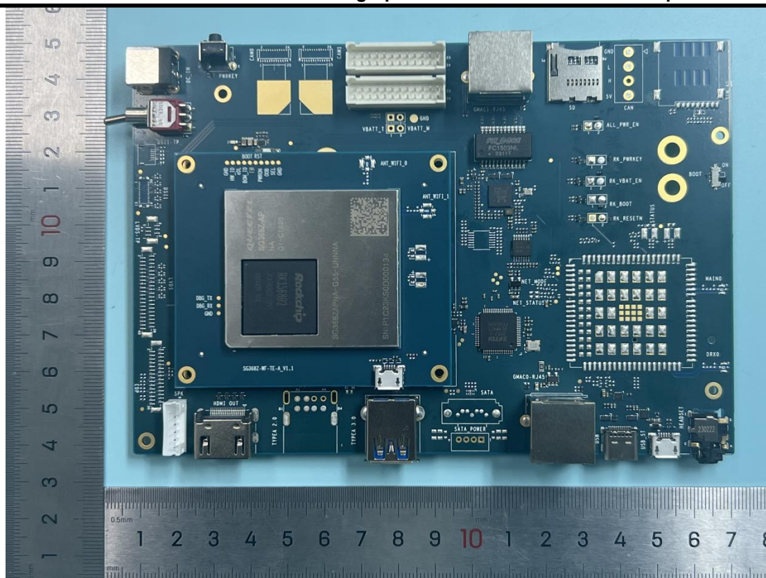
FC906A -Wi-Fi+ EVB _Top
