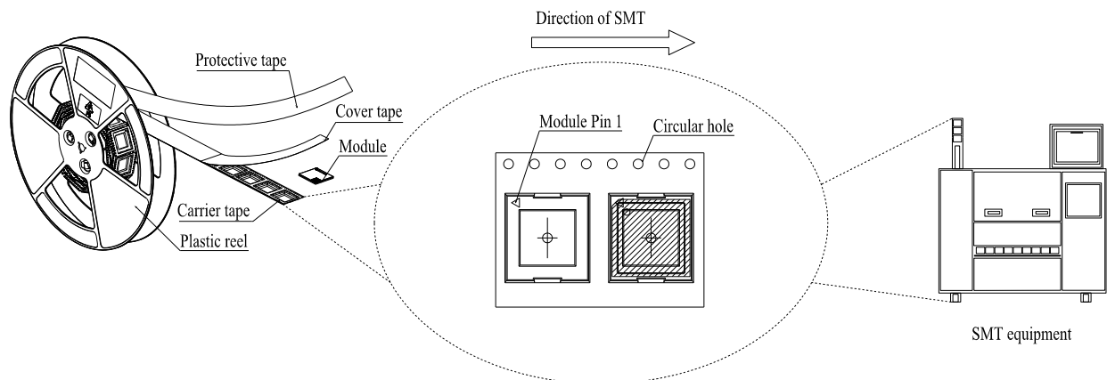
Figure 27: Mounting Direction
