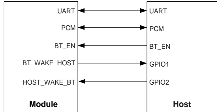
Figure 8: Bluetooth Application Interface Connection
