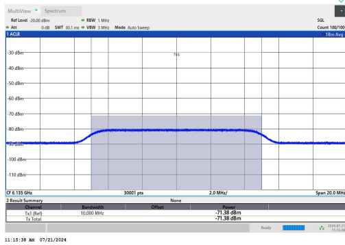
11AX20SISO-Ant1-6135-Center-6135-Minimal
