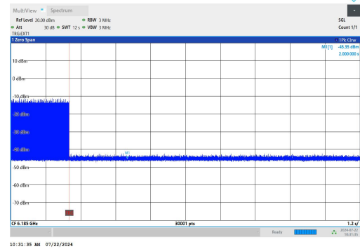
11AX160SISO-Ant1-6185-High-6258.5307-OFF-PASS
