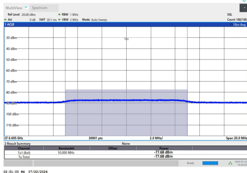
11AX20SISO-Ant1-6695-Center-6695-Minimal
