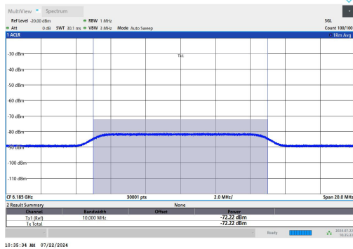
11AX160SISO-Ant1-6185-High-6258.5307-Minimal
