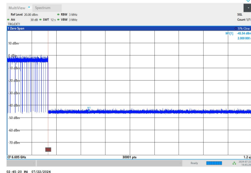
11AX20SISO-Ant1-6695-Center-6695-Minimal
