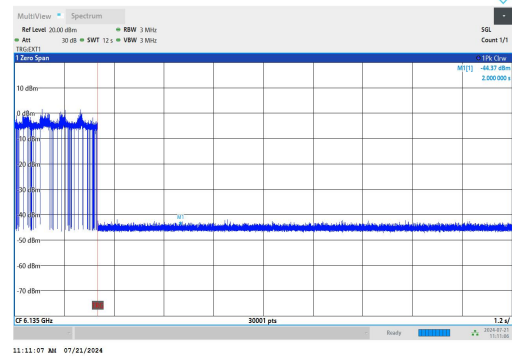
11AX20SISO-Ant1-6135-Center-6135-Minimal
