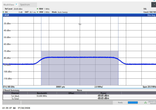
11AX160SISO-Ant1-6185-High-6258.5307-OFF-PASS
