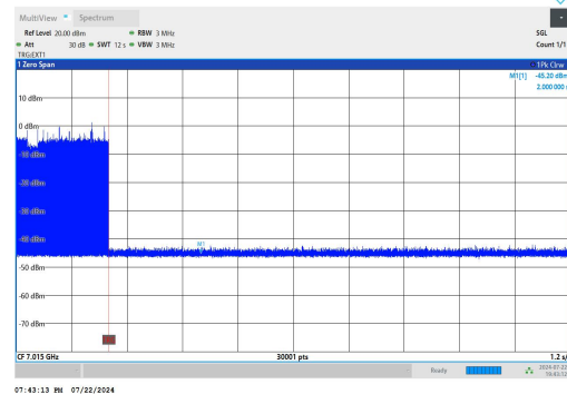
11AX20SISO-Ant1-7015-Center-7015-Minimal
