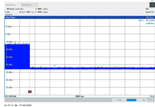
11AX160SISO-Ant1-6185-High-6258.5307-Minimal
