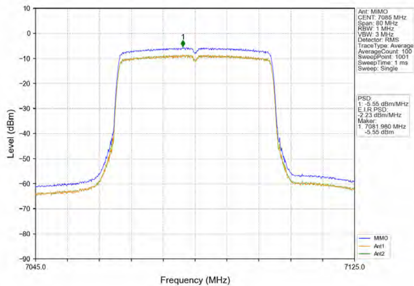
802.11ax(HEW40)_HCH_7085MHz_RU484_Left_MIMO_NTNV
