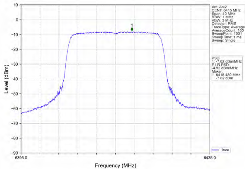
802.11ax(HEW20)_HCH_6415MHz_RU242_Left_Ant2_NTNV
