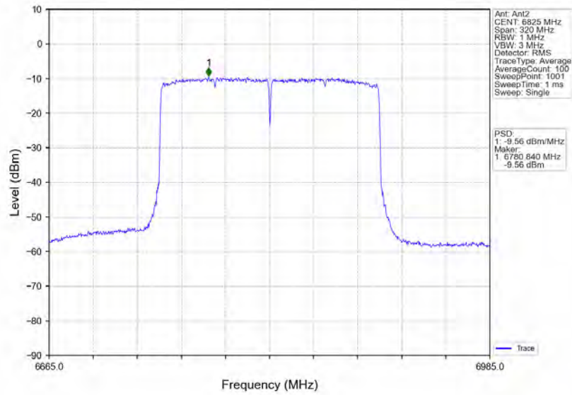
802.11ax(HEW160)_HCH_6825MHz_2xRU996_Left_MIMO_NTNV
