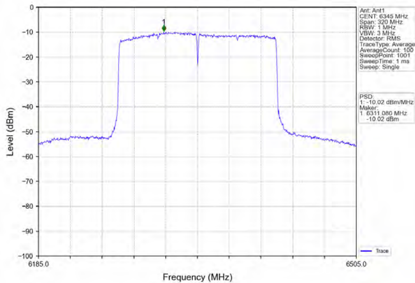
802.11ax(HEW160)_HCH_6345MHz_2xRU996_Left_Ant1_NTNV
