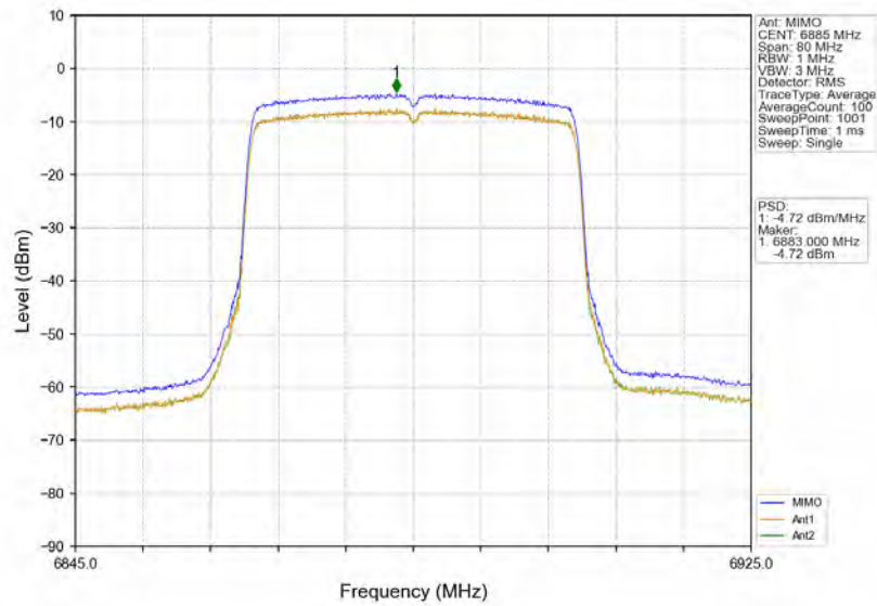
802.11ax(HEW40)_HCH_6885MHz_RU484_Left_MIMO_NTNV
