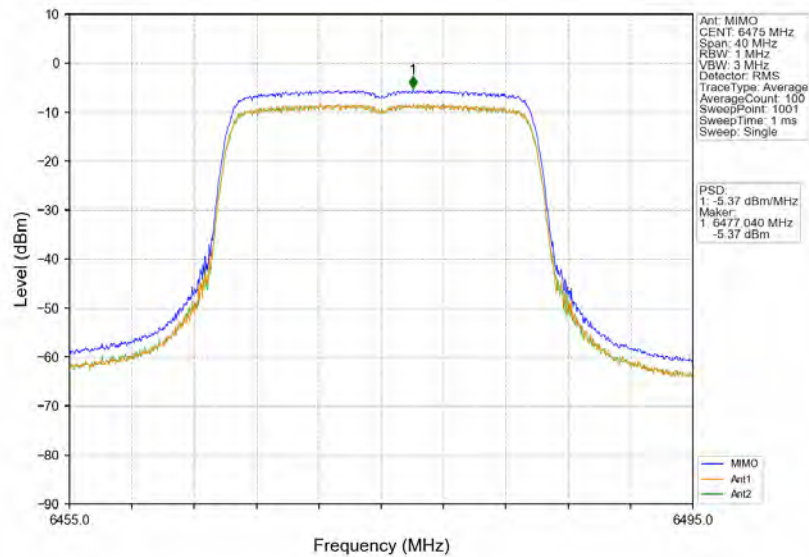
802.11ax(HEW20)_MCH_6475MHz_RU242_Left_MIMO_NTNV
