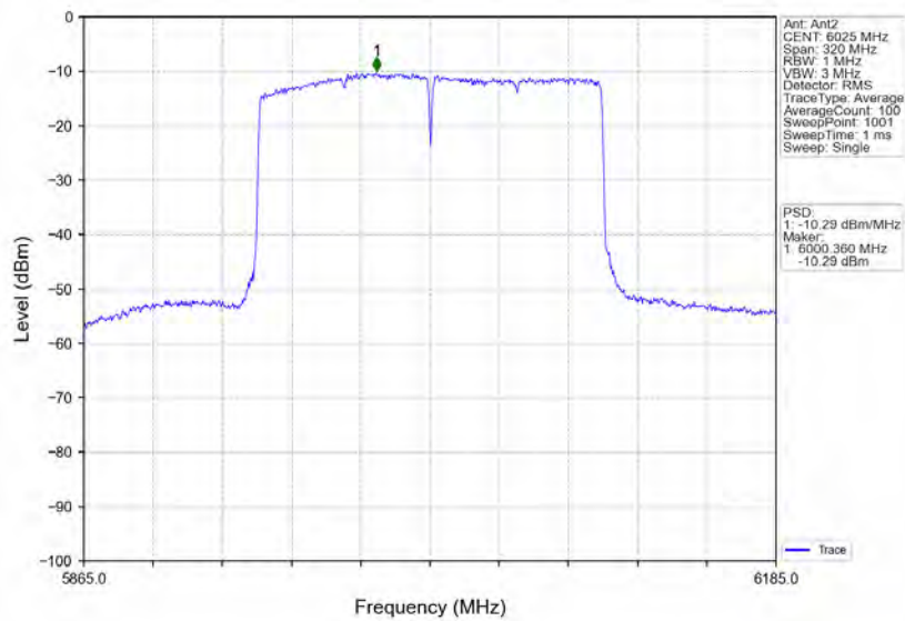
802.11ax(HEW160)_LCH_6025MHz_2xRU996_Left_MIMO_NTNV
