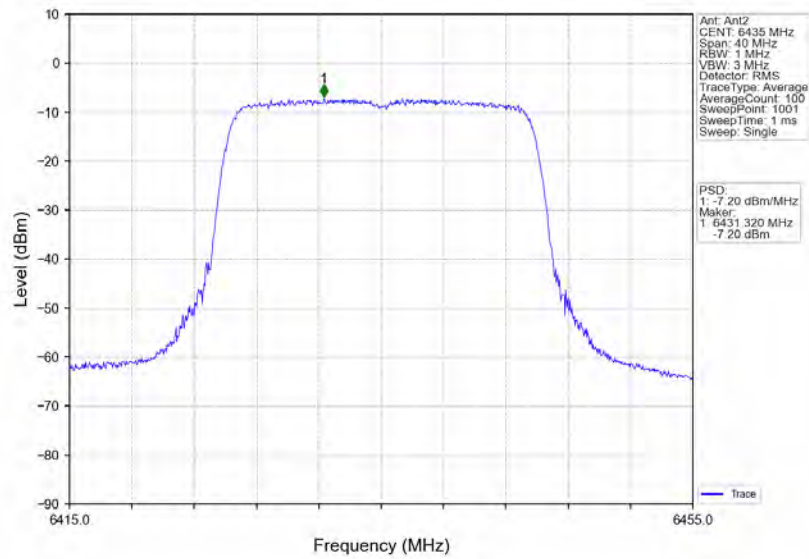
802.11ax(HEW20)_LCH_6435MHz_RU242_Left_Ant2_NTNV
