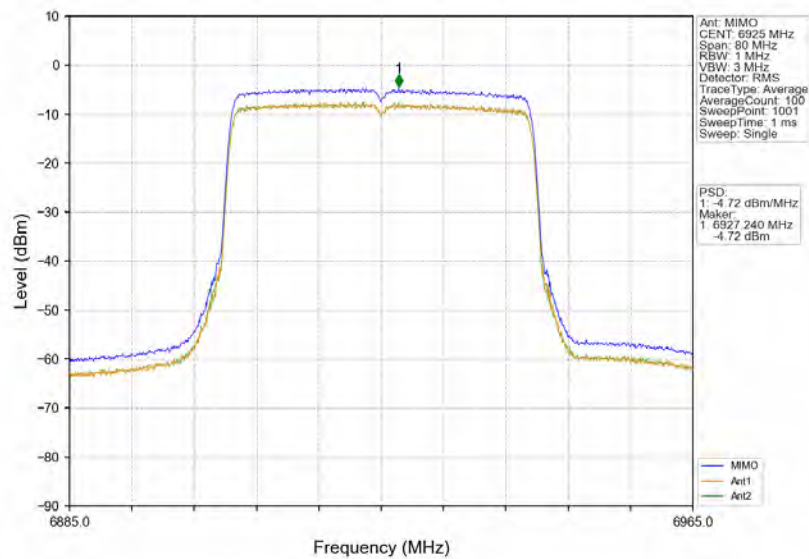
802.11ax(HEW40)_LCH_6925MHz_RU484_Left_MIMO_NTNV
