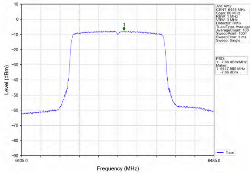
802.11ax(HEW40)_LCH_6445MHz_RU484_Left_MIMO_NTNV
