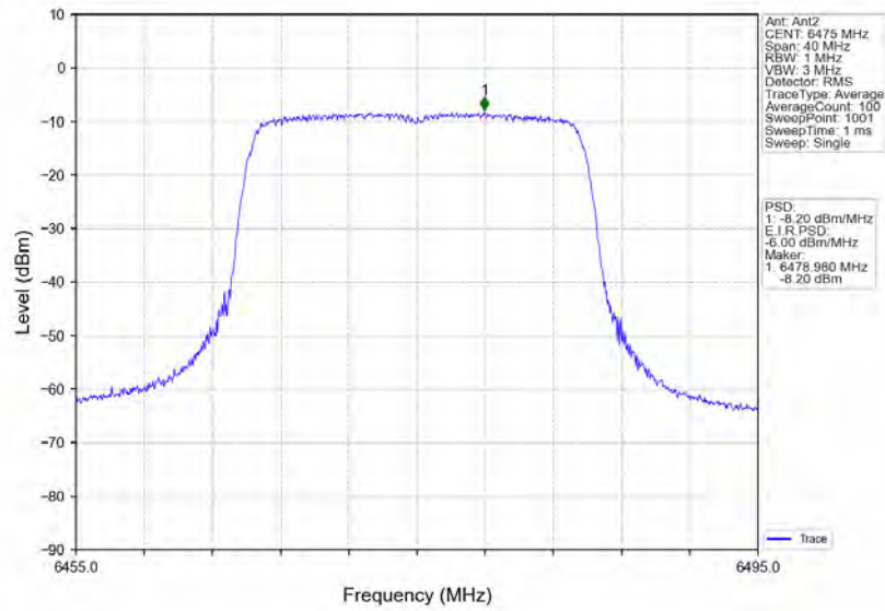
802.11ax(HEW20)_MCH_6475MHz_RU242_Left_MIMO_NTNV
