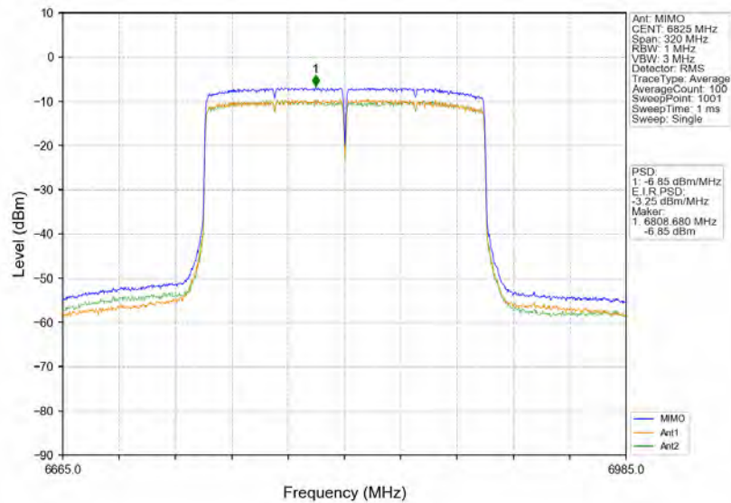
802.11ax(HEW160)_HCH_6825MHz_2xRU996_Left_MIMO_NTNV
