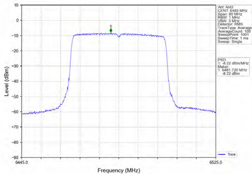
802.11ax(HEW40)_MCH_6485MHz_RU484_Left_Ant2_NTNV
