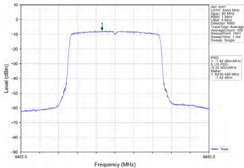
802.11ax(HEW40)_LCH_6445MHz_RU484_Left_Ant1_NTNV
