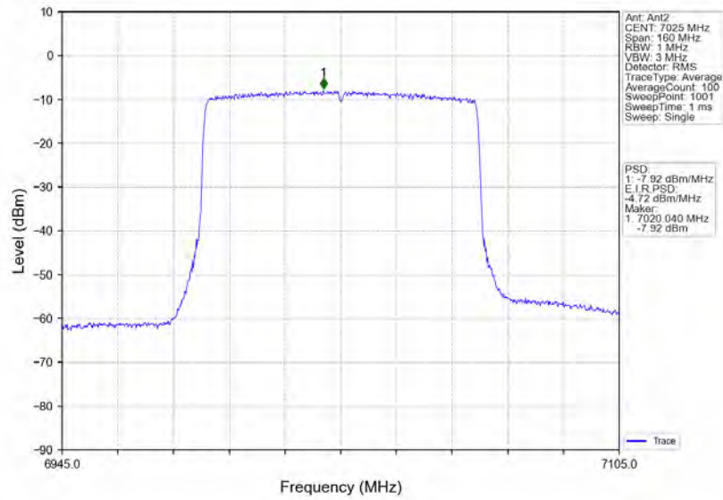
802.11ax(HEW80)_HCH_7025MHz_RU996_Left_MIMO_NTNV
