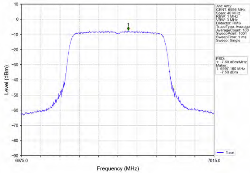
802.11ax(HEW20)_MCH_6995MHz_RU242_Left_MIMO_NTNV
