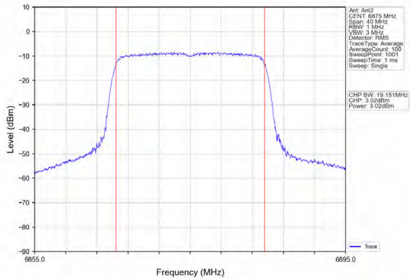
802.11ax(HEW20)_HCH_6875MHz_RU242_Left_Ant2_NTNV
