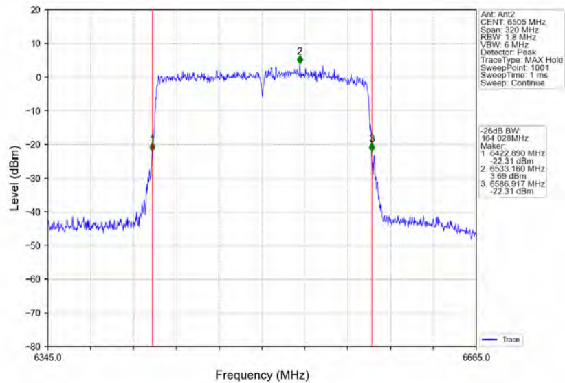
802.11ax(HEW160)_HCH_6505MHz_2xRU996_Left_Ant2_NTNV
