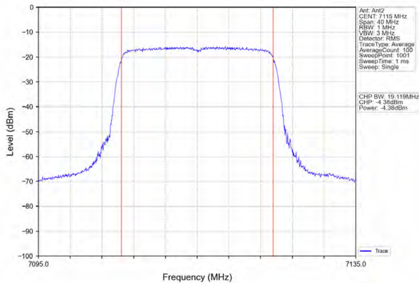
802.11ax(HEW20)_HCH_7115MHz_RU242_Left_Ant2_NTNV
