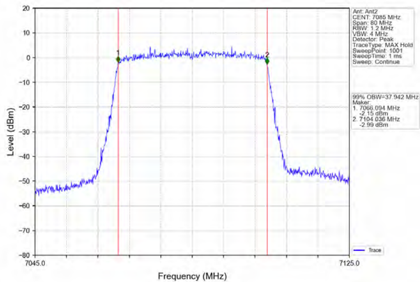
802.11ax(HEW40)_HCH_7085MHz_RU484_Left_Ant2_NTNV
