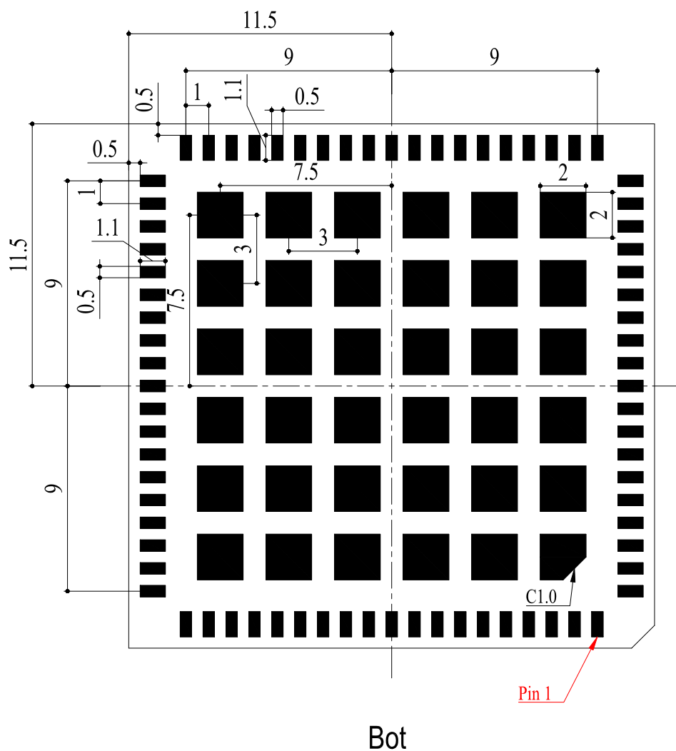
Figure 23: Bottom Dimensions (Bottom View)
