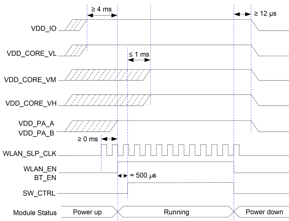
Figure 6: Timing of Power Up and Power Down
