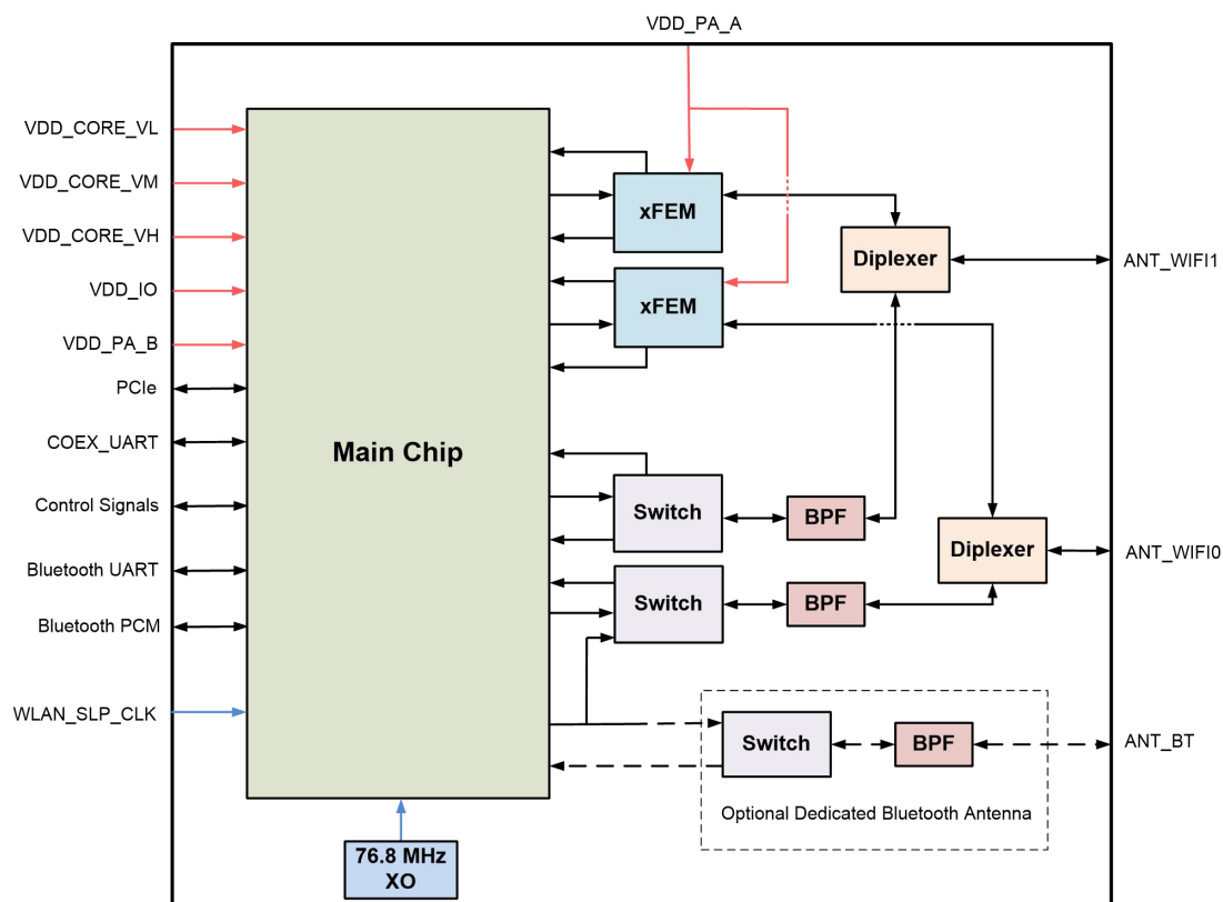
Figure 1: Functional Diagram
