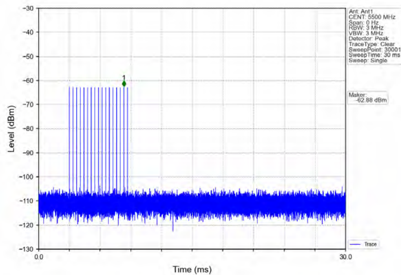
Signal Calibration_802.11a_2C_5500MHz_RadarType3_Trial0
