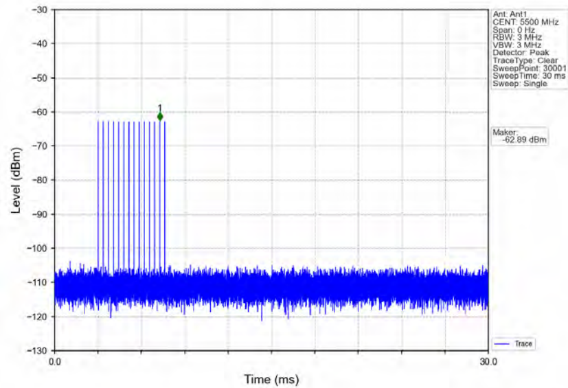
Signal Calibration_802.11a_2C_5500MHz_RadarType5_Trial0
