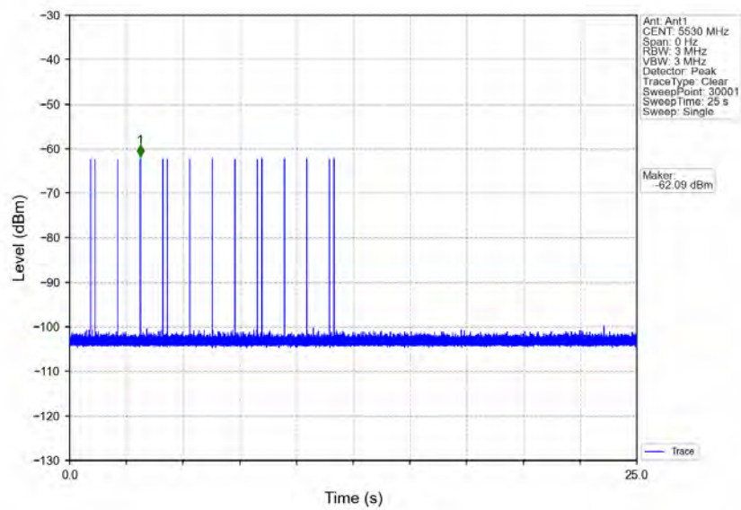
Signal Calibration_802.11ac(VHT80)_2C_5530MHz_RadarType5_Trial0
