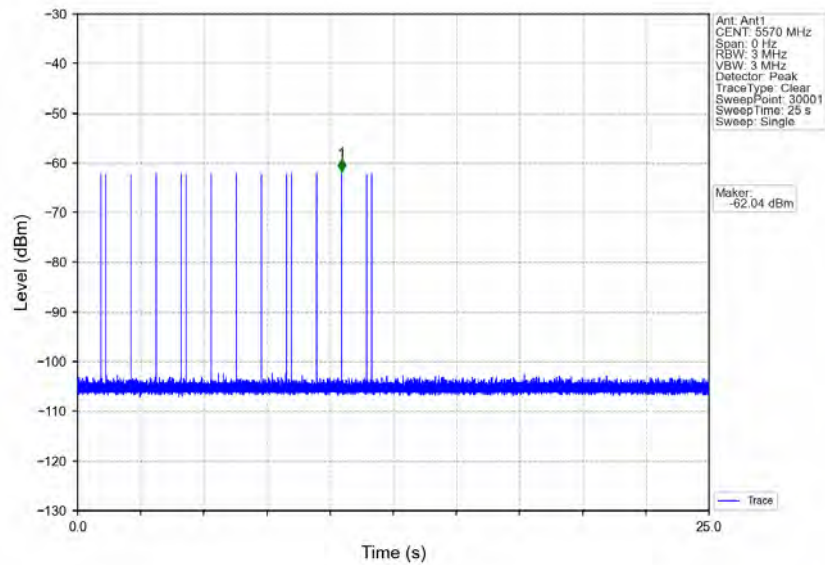
Signal Calibration 802.11ax(HEW160) 2C 5570MHz RadarType6 Trial0
