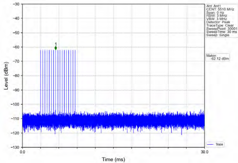
Signal Calibration_802.11n(HT40)_2C_5510MHz_RadarType4_Trial0
