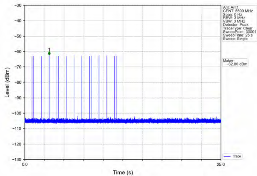
Signal Calibration_802.11a_2C_5500MHz_RadarType5_Trial0
