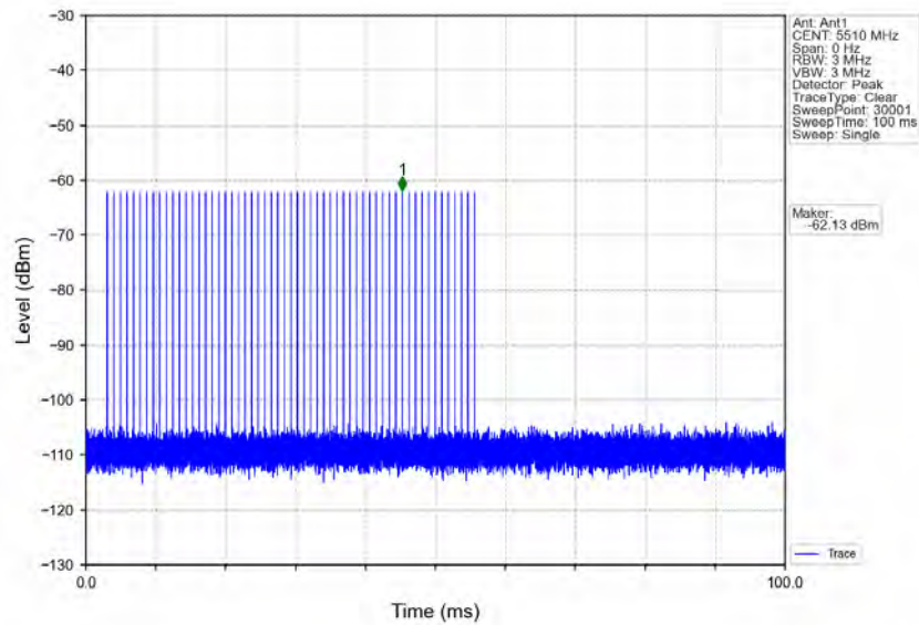
Signal Calibration_802.11n(HT40)_2C_5510MHz_RadarType2_Trial0
