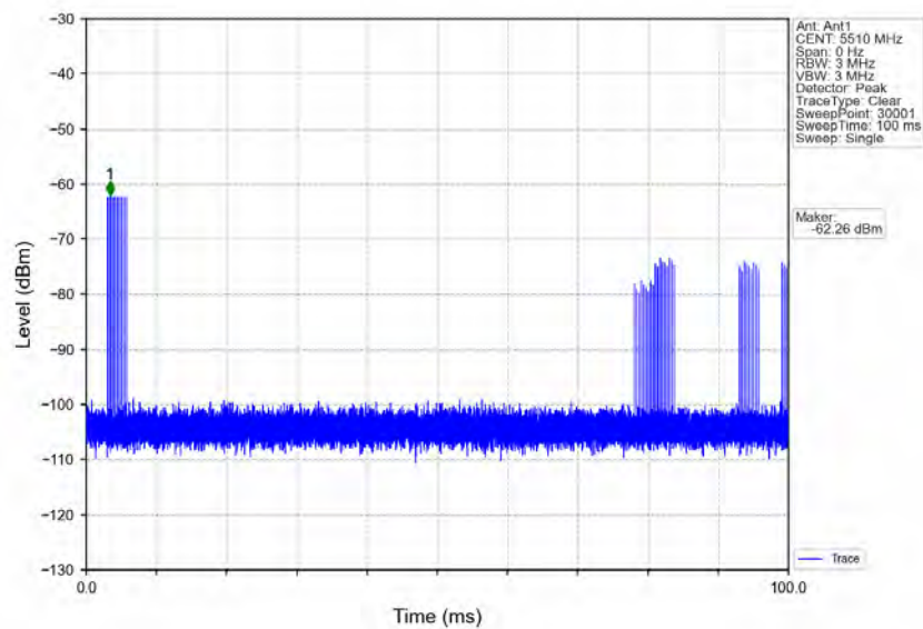
Signal Calibration_802.11n(HT40)_2C_5510MHz_RadarType6_Trial0
