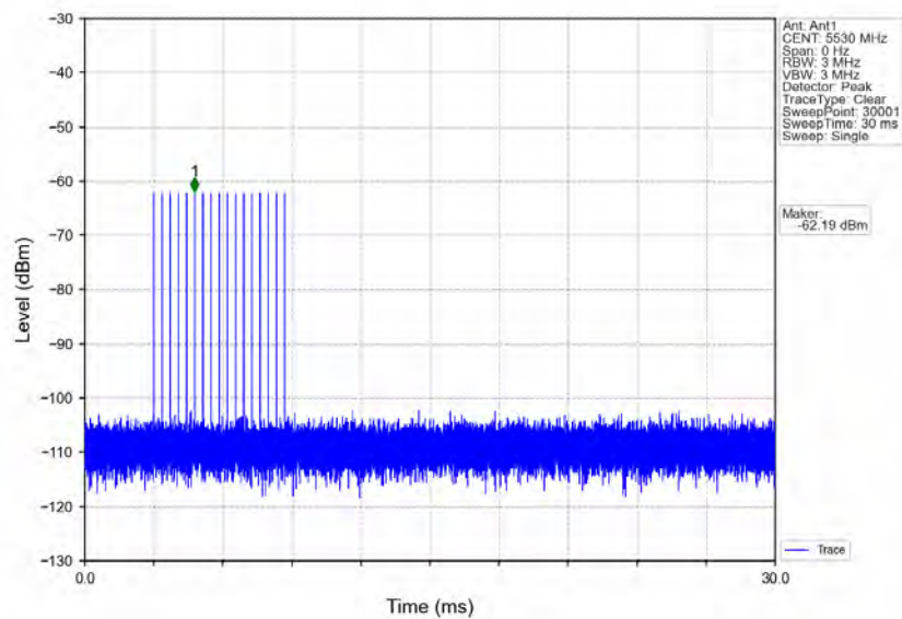
Signal Calibration_802.11ac(VHT80)_2C_5530MHz_RadarType3_Trial0
