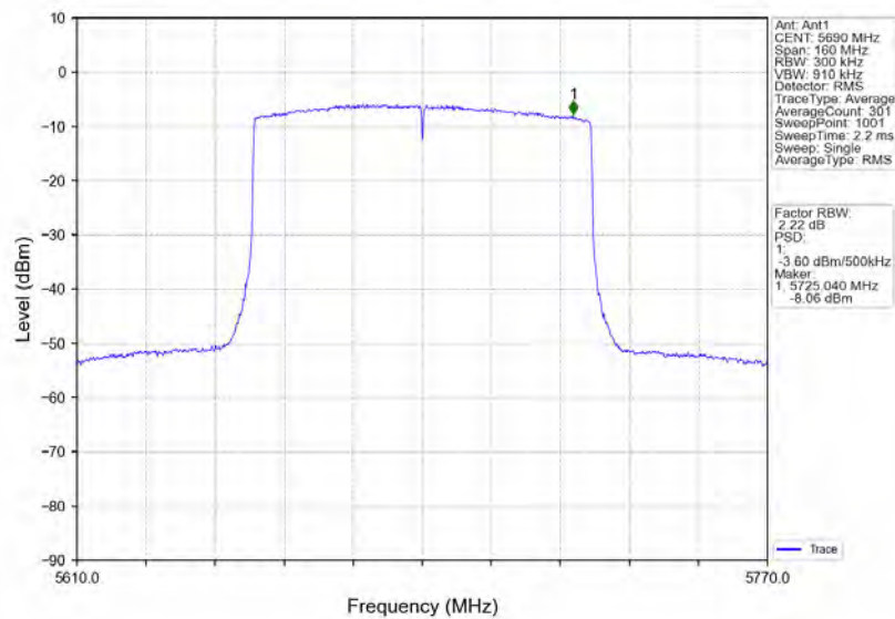
802.11ax(HEW80) HCH 5690MHz RU996 Left Ant1 NTN
