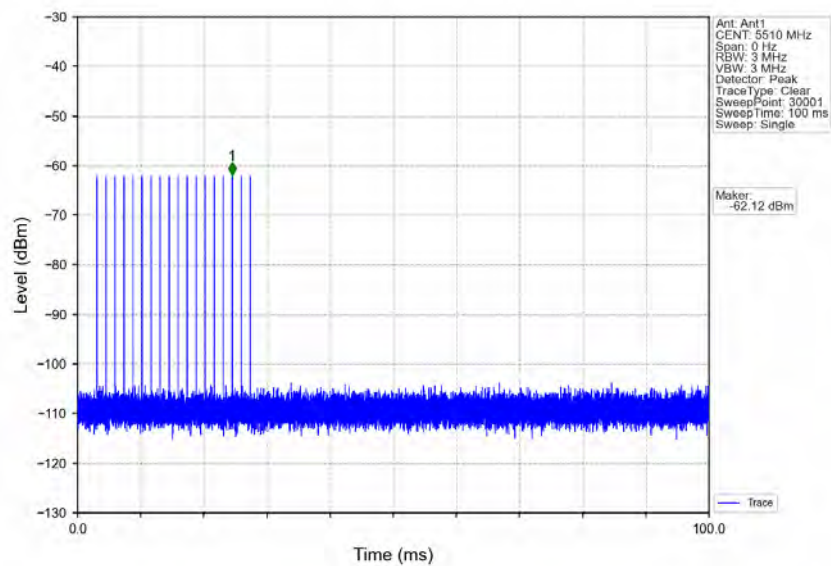
Signal Calibration_802.11n(HT40)_2C_5510MHz_RadarType0_Trial0
