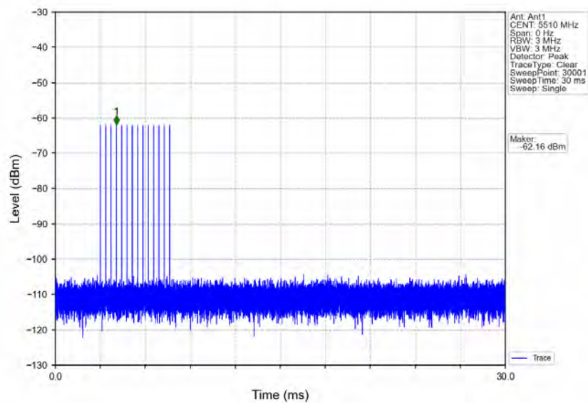
Signal Calibration_802.11n(HT40)_2C_5510MHz_RadarType4_Trial0
