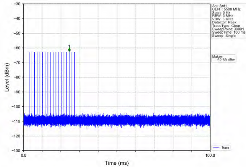
Signal Calibration_802.11a_2C_5500MHz_RadarType1_Trial0
