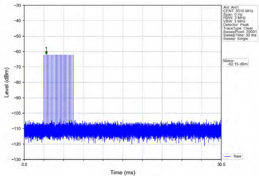
Signal Calibration_802.11n(HT40)_2C_5510MHz_RadarType2_Trial0
