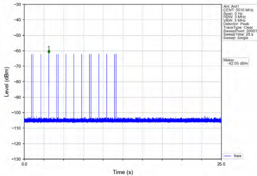
Signal Calibration_802.11n(HT40)_2C_5510MHz_RadarType6_Trial0
