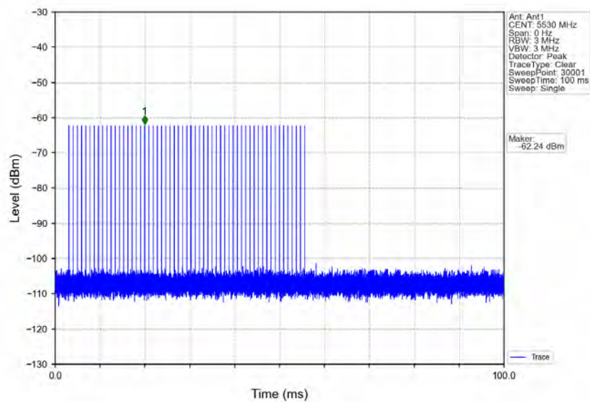
Signal Calibration_802.11ac(VHT80)_2C_5530MHz_RadarType1_Trial0
