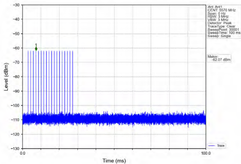
Signal Calibration_802.11ax(HEW160)_2C_5570MHz_RadarType0_Trial0
