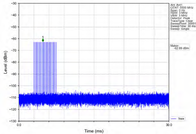
Signal Calibration_802.11a_2C_5500MHz_RadarType3_Trial0
