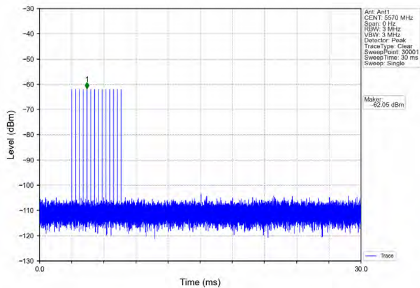
Signal Calibration 802.11ax(HEW160) 2C 5570MHz RadarType4 Trial0
