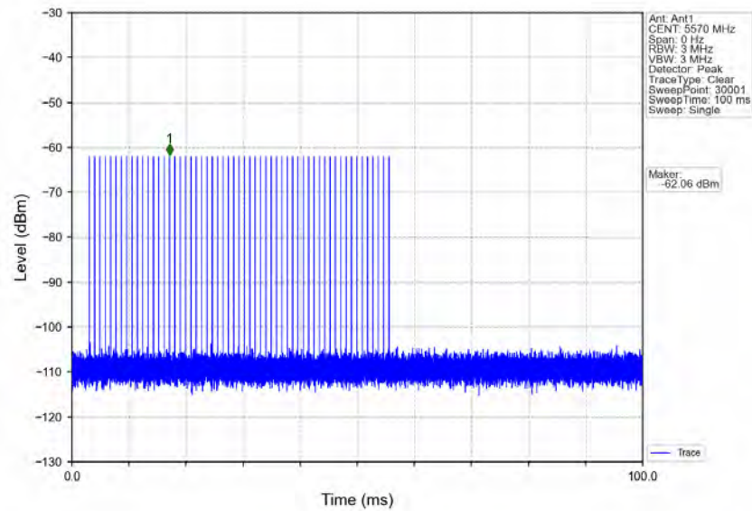
Signal Calibration 802.11ax(HEW160) 2C 5570MHz RadarType2 Trial0
