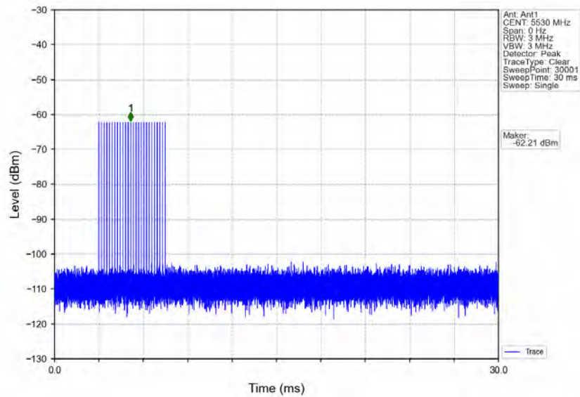
Signal Calibration_802.11ac(VHT80)_2C_5530MHz_RadarType3_Trial0
