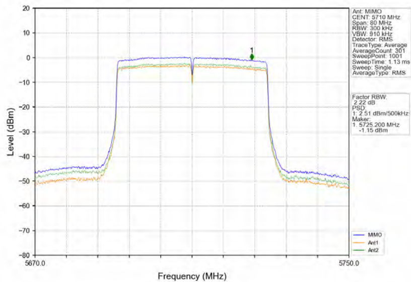
802.11ax(HEW40) HCH 5710MHz RU484 Left MIMO NTN
