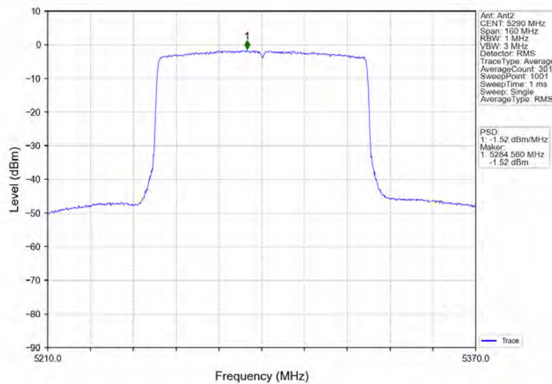
802.11ax(HEW80) MCH 5290MHz RU996 Left Ant2 NTNv
