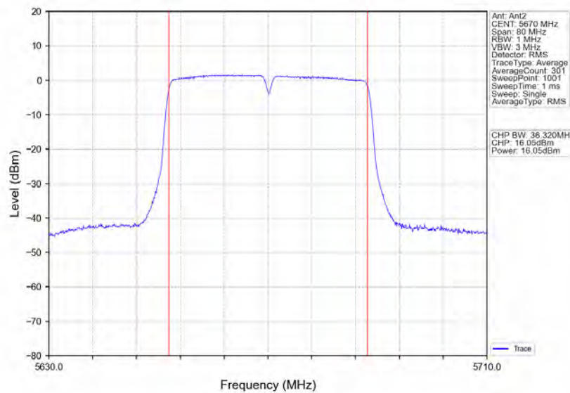
802.11n(HT40)_HCH_5670MHz_Ant2_NTN
