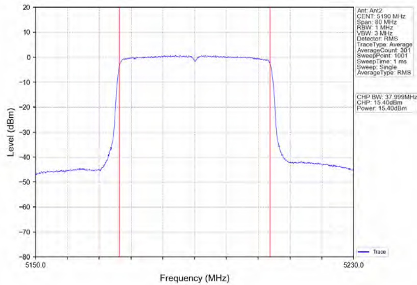
802.11ax(HEW40) LCH 5190MHz RU484 Left Ant2 NTN
