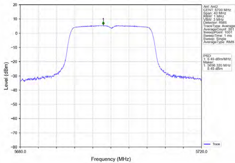
802.11n(HT20)_HCH_5700MHz_Ant2_NTN
