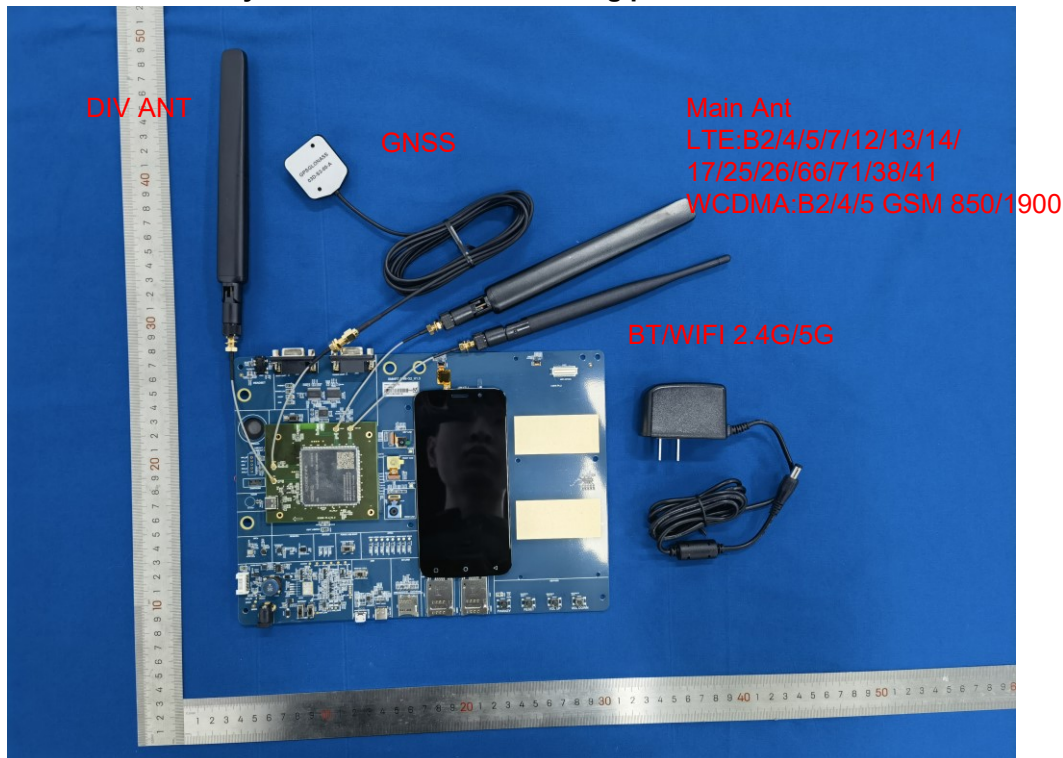
Test auxiliary PCB board and surrounding photos
