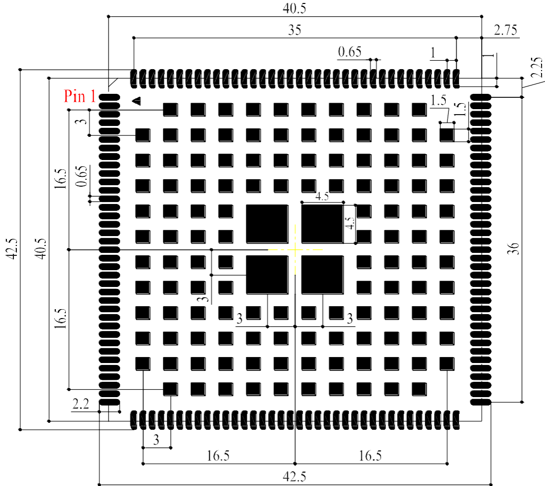
Figure 42: Recommended Footprint
