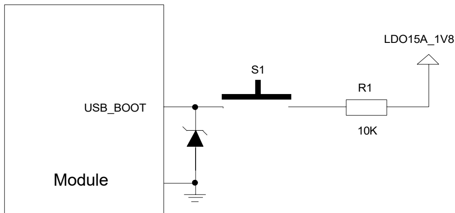
Figure 28: Reference Circuit Design for USB_BOOT Control Interface
