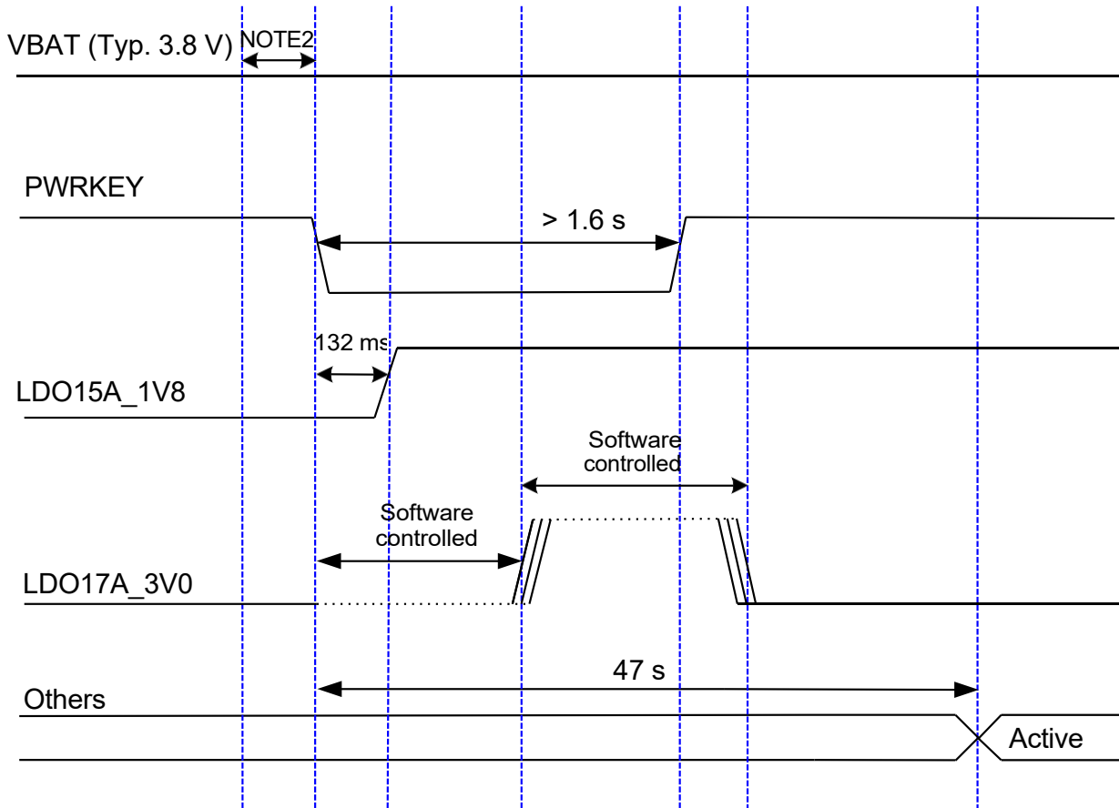
Figure 8: Turn-on Timing
