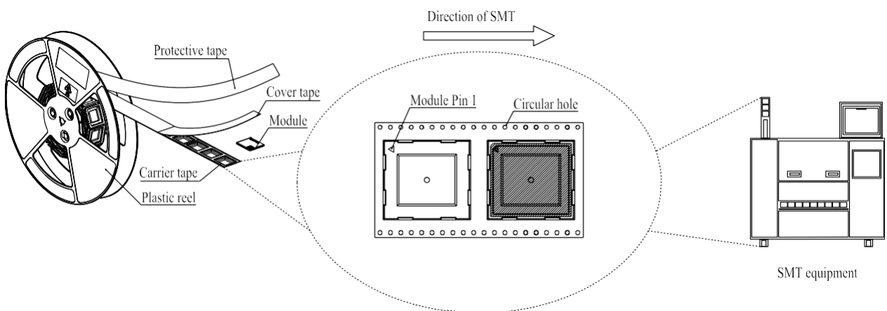
Figure 48: Mounting Direction
