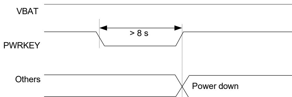
Figure 9: Forced Turn-off Timing
