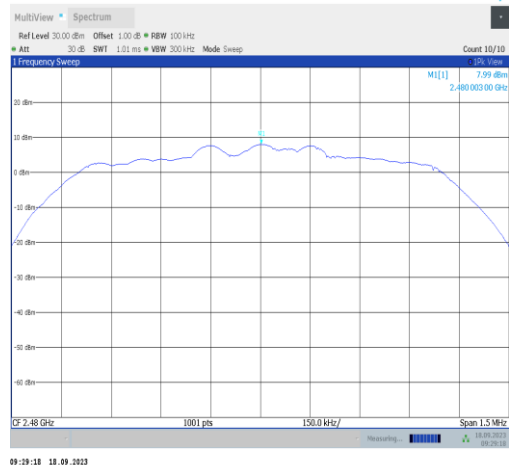
2DH5-Ant1-2480-0~Reference-PASS
