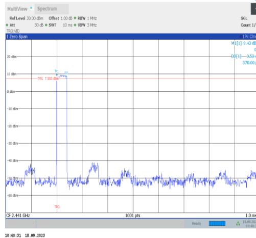
2DH1-Ant1-Hop-PASS
