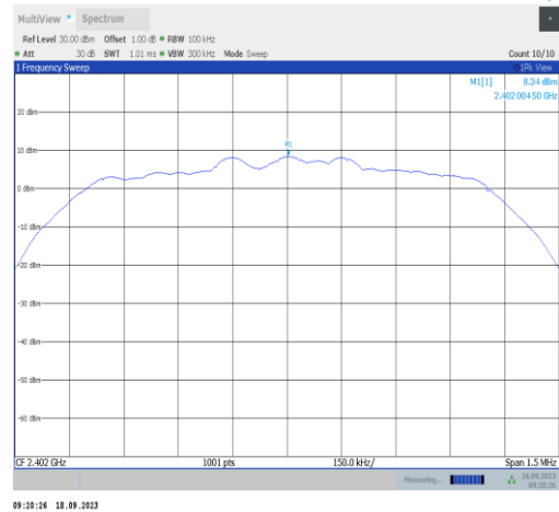
2DH5-Ant1-2402-0~Reference-PASS
