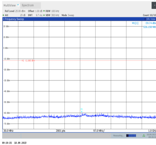
2DH5-Ant1-2402-30~1000-PASS
