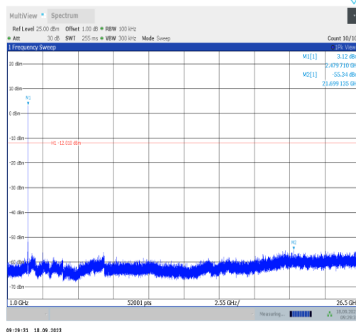
2DH5-Ant1-2480-1000~26500-PASS
