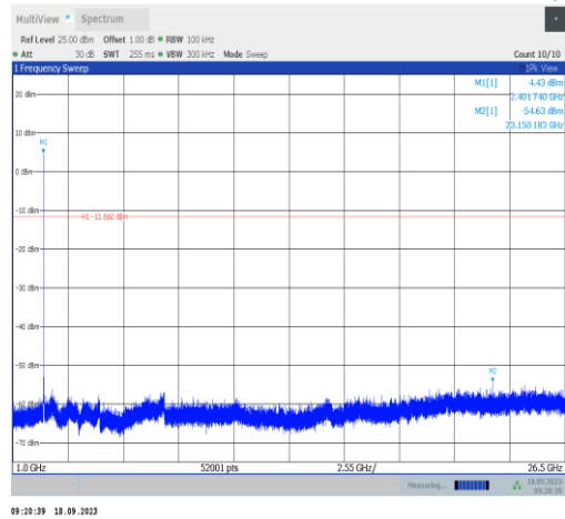
2DH5-Ant1-2402-1000~26500-PASS
