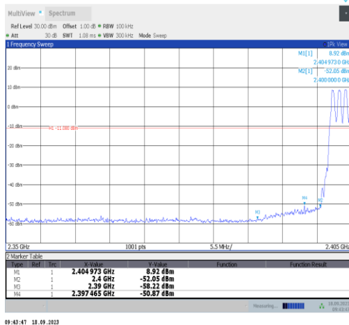
DH5-Ant1-Hop_2402-PASS
