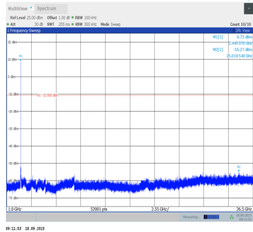
DH5-Ant1-2441-1000~26500-PASS
