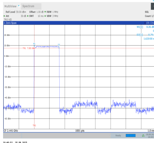
2DH3-Ant1-Hop-PASS
