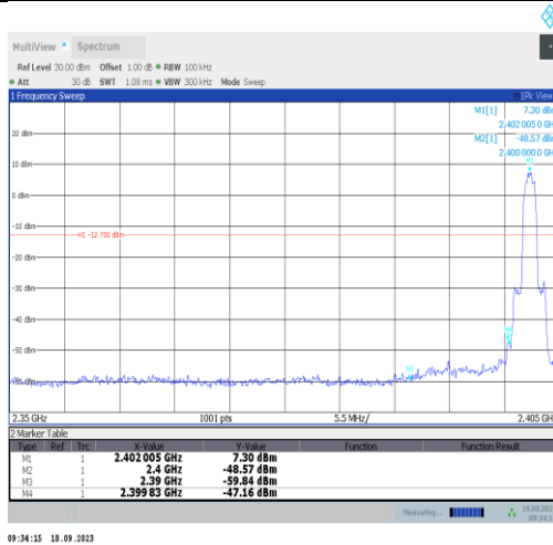
3DH5-Ant1-2402-PASS
