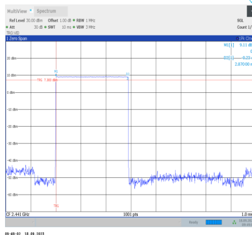
DH5-Ant1-Hop-PASS
