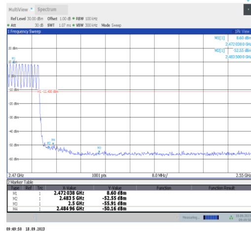
DH5-Ant1-Hop_2480-PASS
