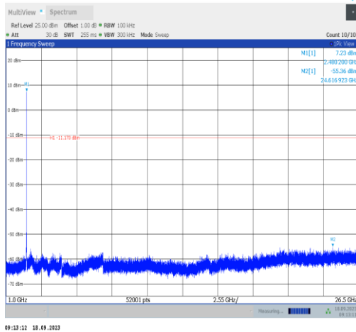
DH5-Ant1-2480-1000~26500-PASS
