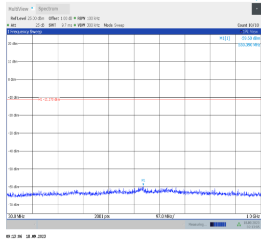
DH5-Ant1-2480-30~1000-PASS
