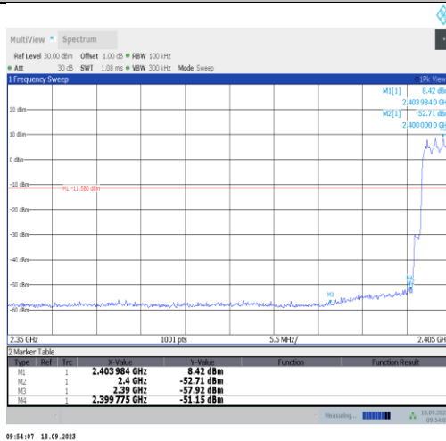
2DH5-Ant1-Hop_2402-PASS
