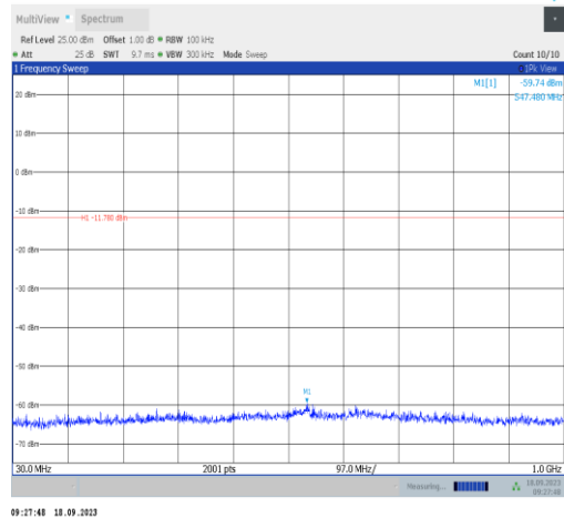
2DH5-Ant1-2441-30~1000-PASS
