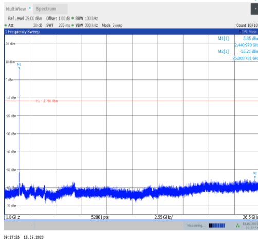
2DH5-Ant1-2441-1000~26500-PASS
