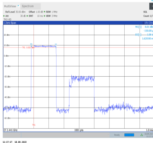
3DH3-Ant1-Hop-PASS
