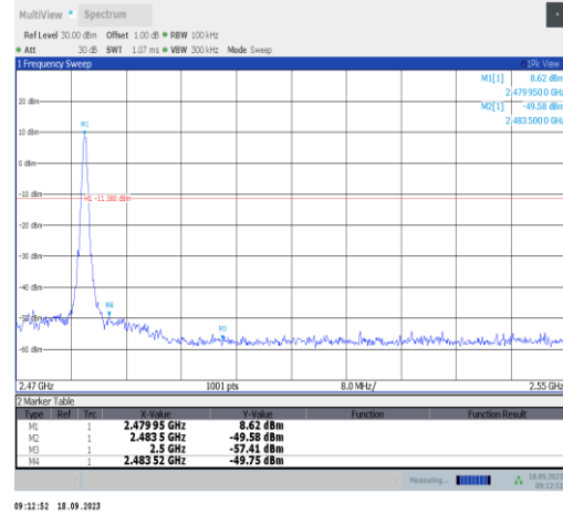
DH5-Ant1-2480-PASS
