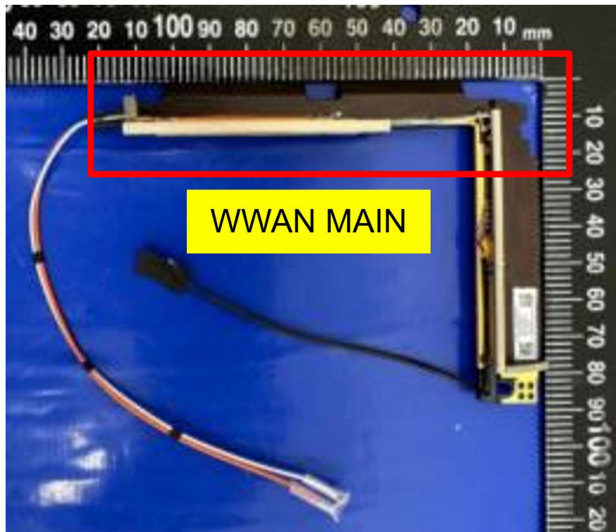
SPEEDWIRE WWAN 5G Antenna
