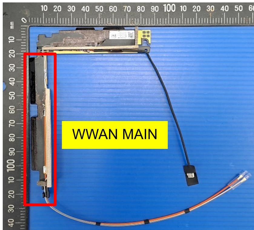
Luxshare-ICT WWAN 5G Antenna
