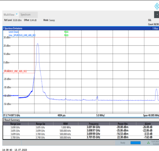
1-N78-3700-3800-PC1-30-40-L-1-DFT-PI2BPSK-Edg_e_1RB_Left-1@0-Ant0-1--PASS-see graph
