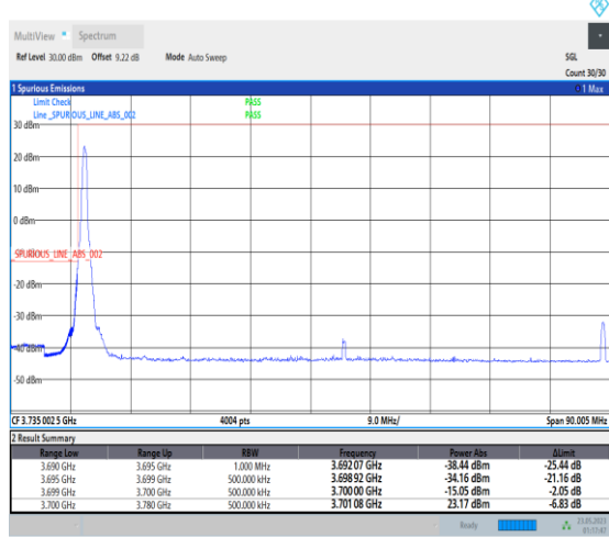
1-N78-3700-3800-PC1-30-80-L-4-CP-QPSK-Edge_1 RB_Left-1@0-Ant0-1--PASS-see graph
