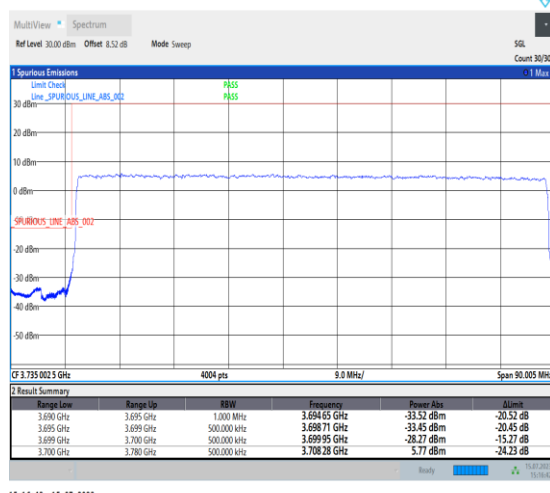
1-N78-3700-3800-PC1-30-80-L-3-DFT-PI2BPSK-O uter_Full-216@0-Ant0-1--PASS-see graph
