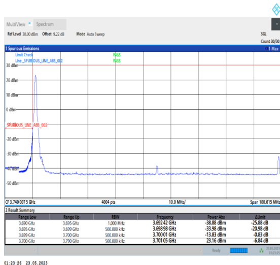
1-N78-3700-3800-PC1-30-90-L-4-CP-QPSK-Edge_1 RB_Left-1@0-Ant0-1--PASS-see graph
