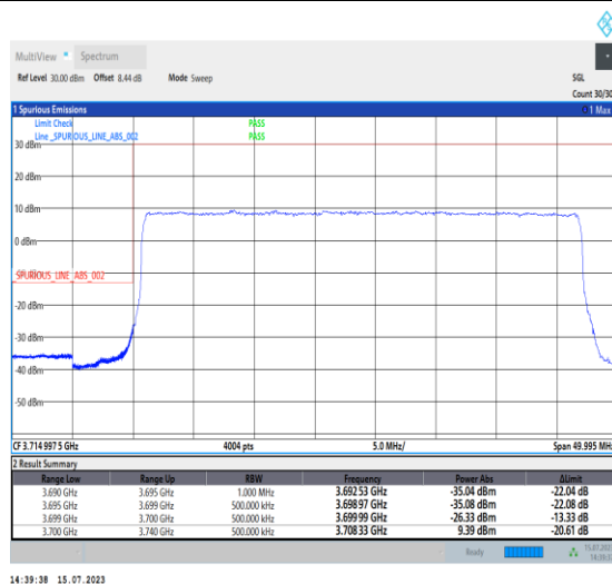
1-N78-3700-3800-PC1-30-40-L-3-DFT-PI2BPSK-Outer_Full-100@0-Ant0-1--PASS-see graph
