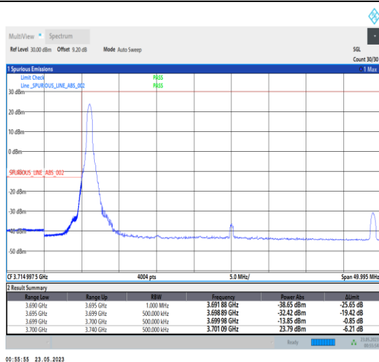
1-N78-3700-3800-PC1-30-40-L-4-CP-QPSK-Edge_1RB_Left-1@0-Ant0-1--PASS-see graph
