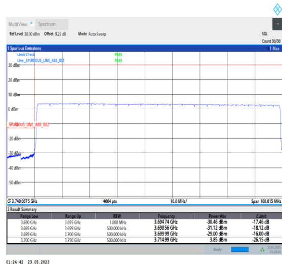
1-N78-3700-3800-PC1-30-90-L-6-CP-QPSK-Outer_ Full-245@0-Ant0-1--PASS-see graph
