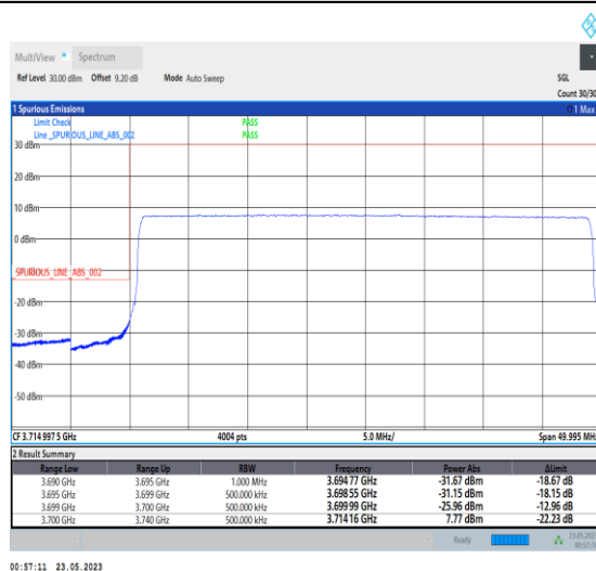
1-N78-3700-3800-PC1-30-40-L-6-CP-QPSK-Outer_Full-106@0-Ant0-1--PASS-see graph
