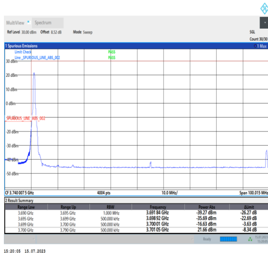
1-N78-3700-3800-PC1-30-90-L-1-DFT-PI2BPSK-Edg e_1RB_Left-1@0-Ant0-1--PASS-see graph
